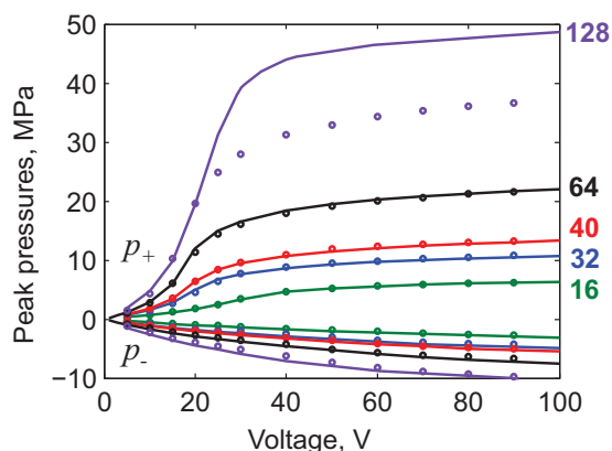
Figure 4.20: Saturation curves for the peak positive and negative pressures obtained in numerical simulation (solid curves) and in hydrophone measurements (markers) for configurations of 16, 32, 40, 64, and 128 active elements of the probe.
