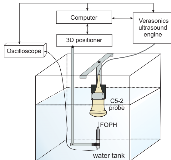
Figure 4.15: Diagram of the experimental arrangement for measurement of acoustic field in water. Fiber optic hydrophone (FOPH) was used for high-power measurements while low-amplitude measurements were performed using a capsule hydrophone.
