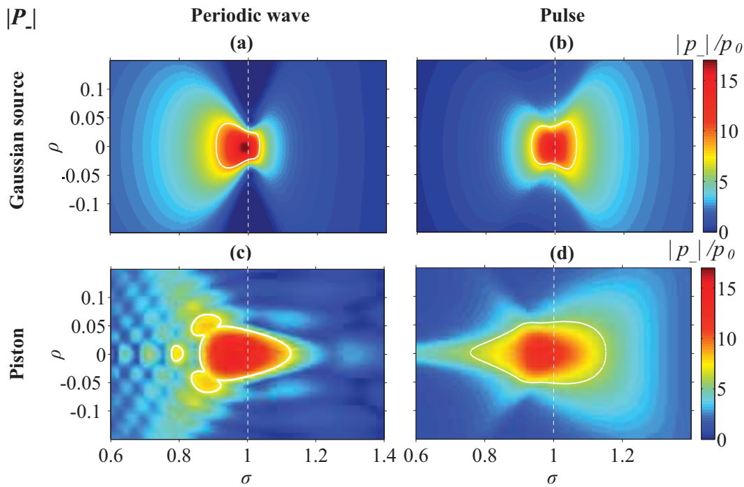
Figure 3.14: 2D spatial distributions of the peak negative pressure in cases of a Gaussian source (upper series a, b) and piston source (lower series c, d). Distributions in left column (a, c) correspond to the periodic field while the right column (b, d) - to the pulsed field. White solid lines indicate sizes of focal areas. White dashed lines show the plane of the geometrical focus. Distributions are plotted for G = 40 , N = 1.0 .
