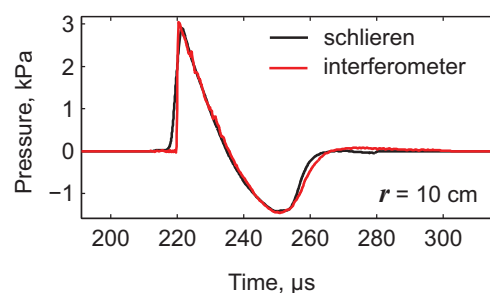
Figure 1.17: Comparison of pressure waveforms obtained using the optical schlieren method (black line) and the Mach-Zehnder interferometry method (red line) at distance r = 10 \text{ cm} from the spark source.
