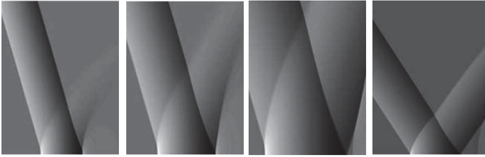
Figure 2.5: Consecutive reflection patterns of the N -wave obtained for different points on the surface. On each pattern reflection of the front shock of the N -wave correspond to the left part of the image while reflection of its rear shock - to the right one. The gradients of a color correspond to the pressure level: white color corresponds to positive pressure, black color - to negative pressure. Figures were taken from (Baskar et al. , 2007).
