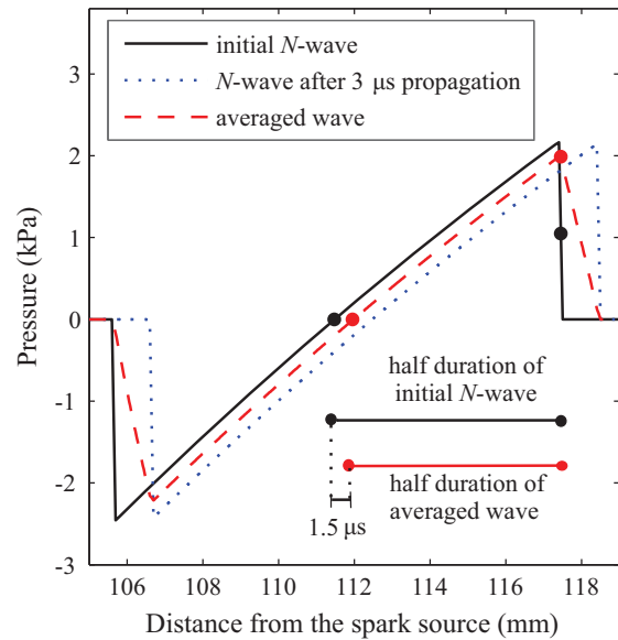
Figure 1.5: Effect of a 3 \mu s exposure time of the camera on the reconstructed waveform. Solid curve is the initial N -wave that was numerically propagated during 3 \mu s ; dotted curve is the wave after propagation; dashed curve is the averaged wave, which imitates the measured waveform. The half duration of the initial wave can be calculated as the half duration of the averaged wave plus the half of the exposure time ( 1.5 \mu s ).
