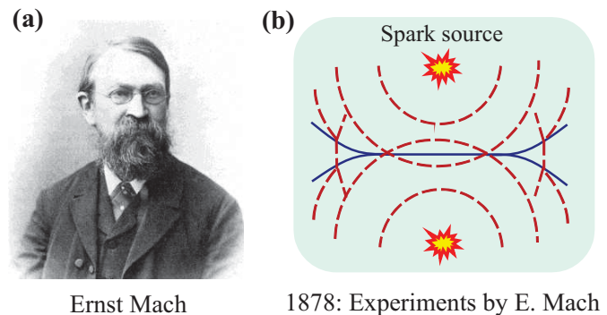
Figure 2.1: (a) Ernst Mach, (b) scheme of an experiment performed by E. Mach to study shock wave reflection, the view is from the top.
