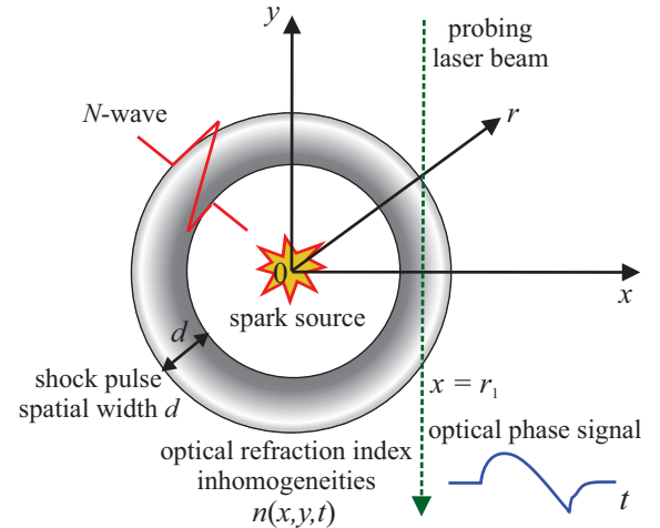
Figure 1.13: Illustration of the optical phase integration along the probing laser beam propagating through a radial distribution of the refraction index inhomogeneities induced by the acoustic wave.
