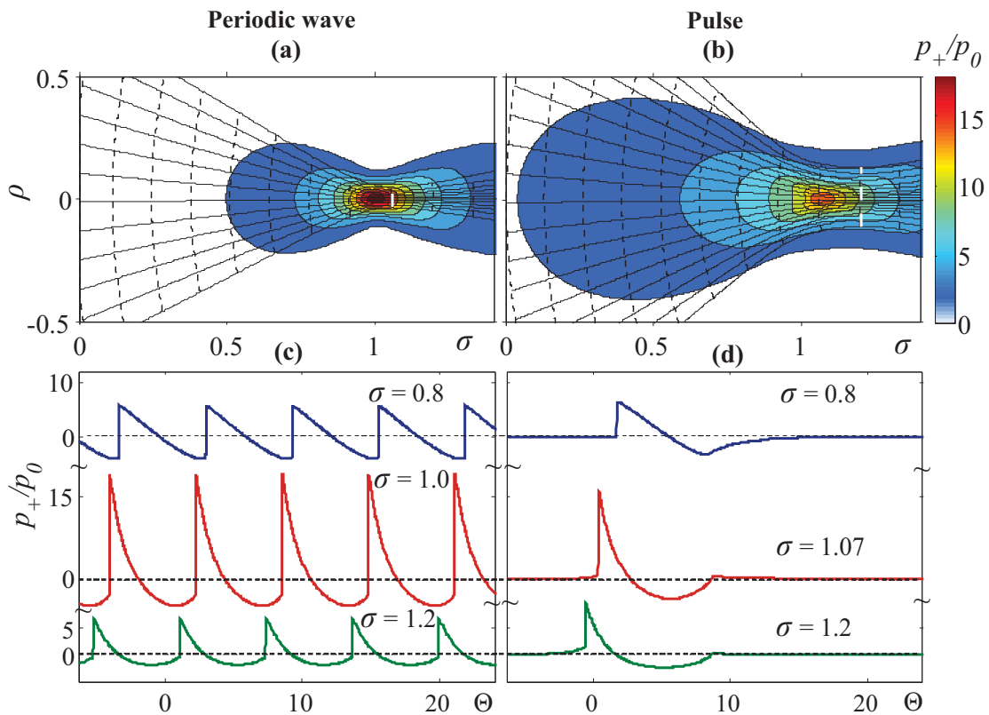
Figure 3.7: The upper series: ray patterns for periodic (a) and pulsed (b) fields. Rays are shown by solid lines and shock fronts – by dashed lines. The white dashed line indicates the front position at the point of its straightening in the paraxial area. Colors indicate levels of the peak positive pressure ( G = 10 , N = 1.0 ). The lower series: waveforms at the source axis of Gaussian transducer at different distances \sigma in the cases of periodic (c) and pulsed (d) fields.
