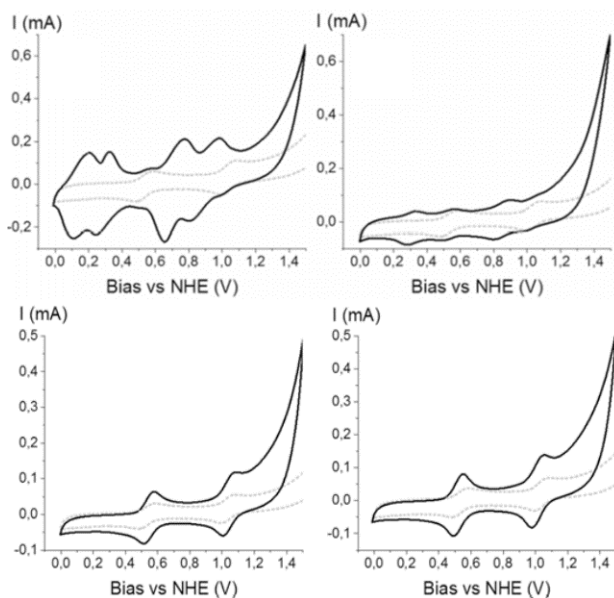
Figure 3.15. Top left, Cyclic voltammograms of 1 , product of direct solvothermal synthesis. Top right, 2 , product of the co-synthesis with edba. Bottom left, octahedral Ru-edba-MOF 5 . Bottom right, interlaced Ru-edba-MOF 6 . Grey dotted lines represent the reference CV of the homogeneous complex for comparison. Reprinted with permission from the Royal Society of Chemistry. T. Liseev et al / Dalton Trans., 2020, 49, 13753 - 13759.
