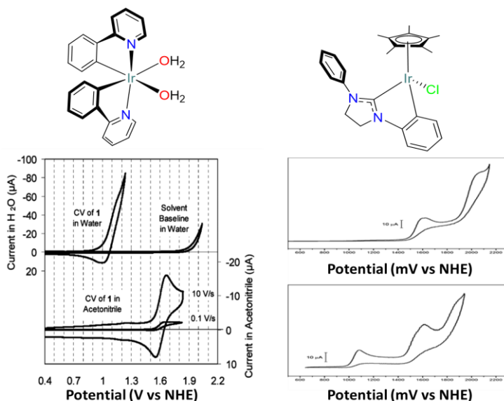
Figure 1.10. Bernhard's Iridium-based WO catalyst containing cyclometalated N,N-bidentate and pentamethylcyclopentadienyl ( cp^* ) ligands. Using Iridium complexes containing carbenes further improves the TOF frequency to up to 10000. Reprinted with permission from American Chemical Society. N. D. McDaniel / J. Am. Chem. Soc. 2008 , 130 , 1, 210 - 217 and T. P. Brewster et al / Organometallics 2011 , 30 , 5, 965 - 973.
