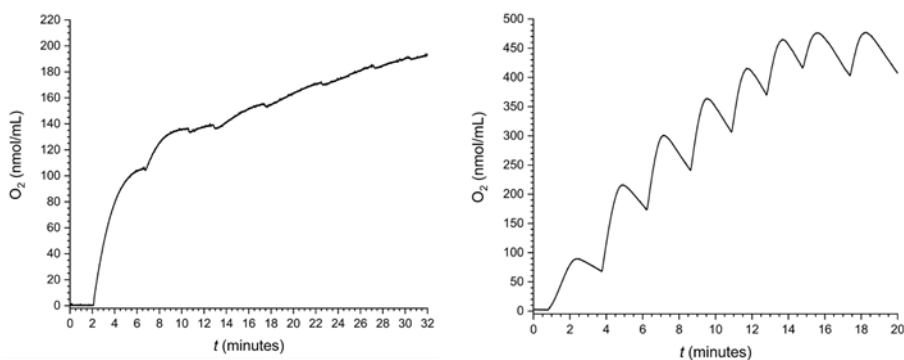
Figure 5.19. Chemical oxidation, 50 \mu L of CAN (0.05 M), multiple additions. Left, II . Right, III . electrode.
