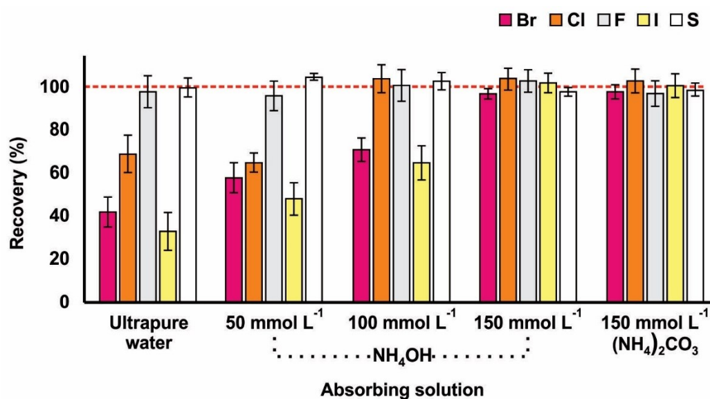
Figure 8. Recoveries obtained from spike tests for bromine, chlorine, fluorine, iodine, and sulfur in D. anceps sample after sample preparation by MIC using different absorbing solutions and analysis by IC-CD-MS (n=3).
