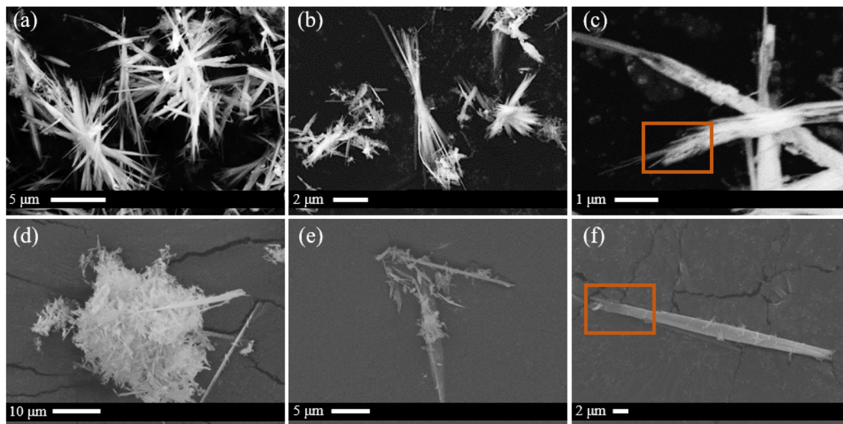
Figure 3.14: SEM images of tobermorite fibres synthesised under supercritical conditions (25 MPa and 400 ^{\circ}\text{C} in 8 s) at different magnifications: both aggregates of small fibres as well as large single fibres are present.
