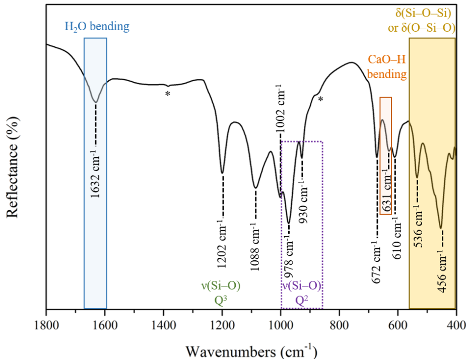
Figure 3.11: IR spectrum of xonotlite synthesised in supercritical water at 25 MPa and 400 °C in 7 s. The asterisk denotes \text{CO}_3^{2-} vibration bands related to carbonate impurity.
