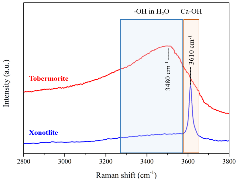
Figure 3.25: Raman spectra of tobermorite (red curve) and xonotlite (blue curve) synthesised under supercritical conditions at 400 °C and 25 MPa [191].
