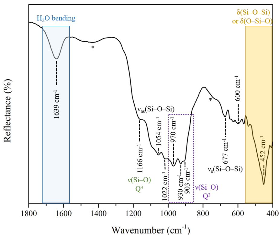
Figure 3.19: IR spectrum, recorded in the range 1800 – 400\text{ cm}^{-1} , of Al-tobermorite synthesised under supercritical conditions at 25\text{ MPa} and 400\text{ °C} in 8\text{ s} . The asterisk denotes C–O stretching mode related to carbonate impurity.
