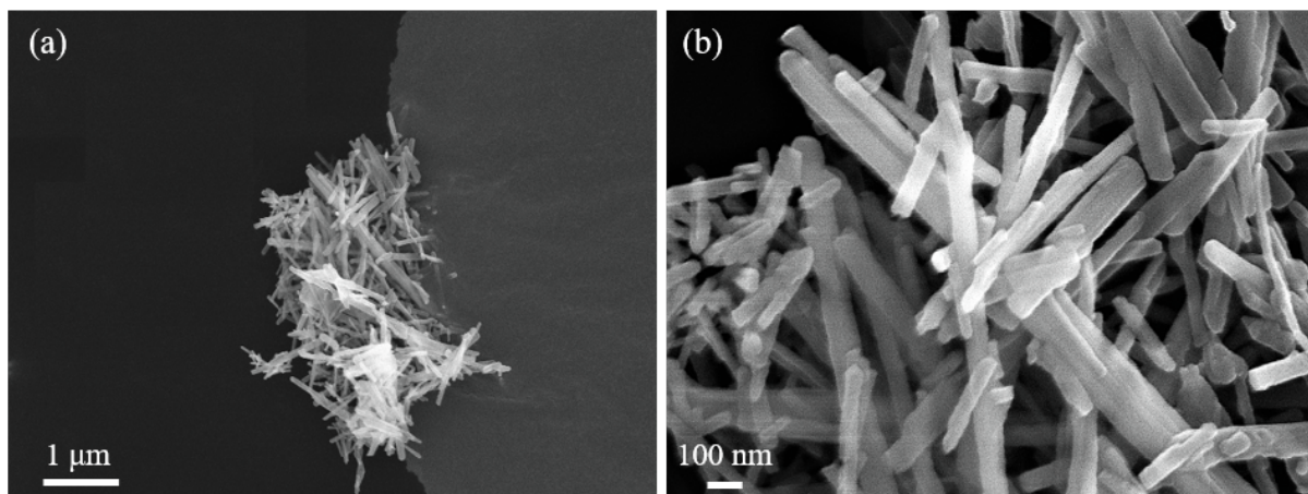
Figure 4.24: HR-SEM images of wollastonite fibres at different magnifications (a) \times 4,000 and (b) \times 65,000 . The images were acquired using acceleration voltage and working distance equal to 15 kV and 3 mm, respectively.
