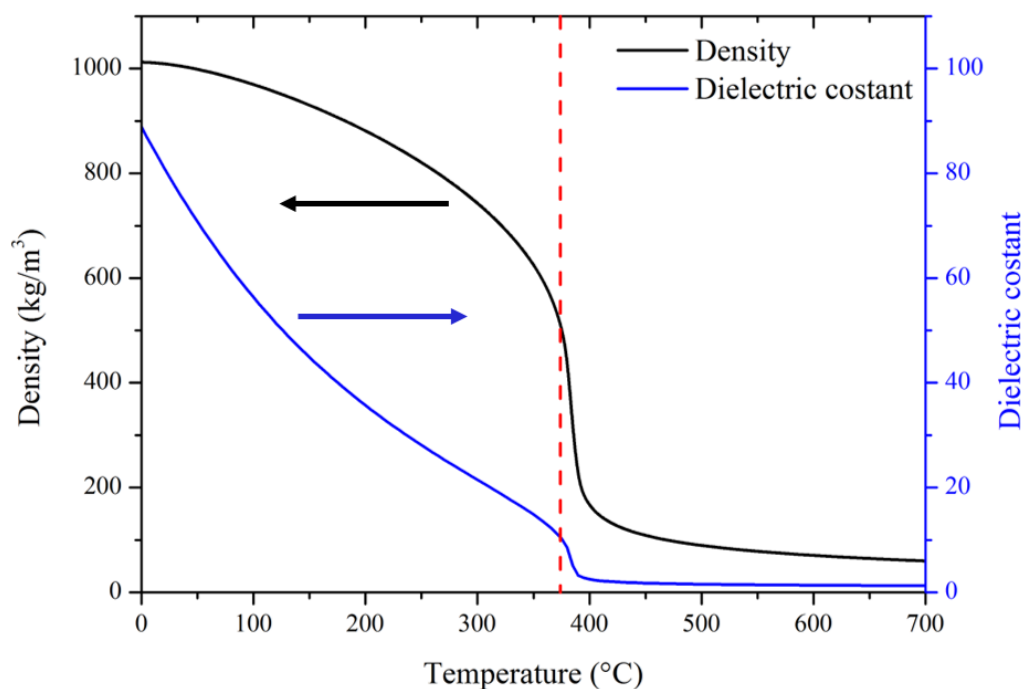
Figure 1.16: Evolution of density (solid black line) and dielectric constant (solid blue line) of pure water as a function of the temperature at 25 MPa. The dotted red line represents the critical temperature. The data were collected from the National Institute for Standards and Technology database, NIST [126].
