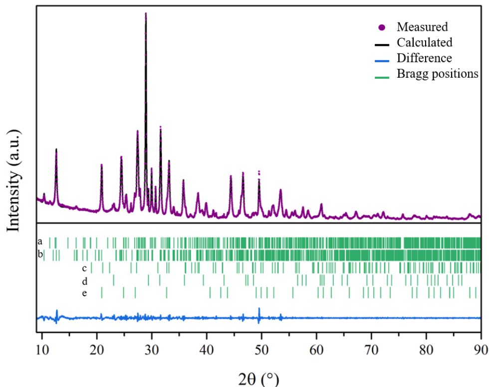
Figure 4.22: Profile Matching plot of sample P2 synthesised at 500^\circ\text{C} and 2 MPa. In the top, the measured (purple circles) and calculated (black curve) patterns are displayed; in the bottom, the difference curve between them is shown (blue line). Five crystalline phases were distinguished: (a) wollastonite-1T, (b) xonotlite, (c) aragonite, (d) calcite, and (e) vaterite, as identified from their respective reflection positions (green bars).
