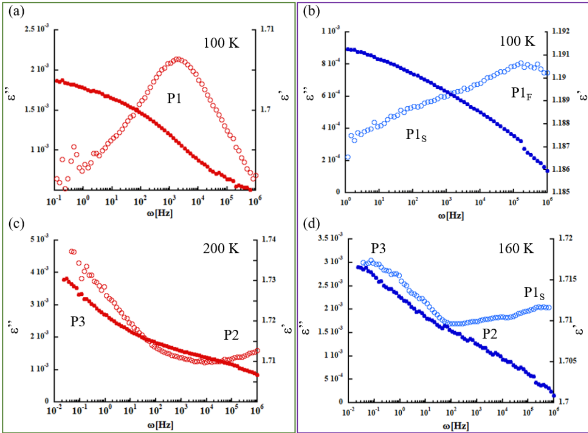
Figure B.1: Comparison between the real part ( \epsilon' ) and the imaginary part ( \epsilon'' ) of the dielectric spectra of nanominerals at different temperatures: tobermorite at (a) 100 K and (c) 200 K and xonotlite at (b) 100 K and (d) 160 K. \epsilon' and \epsilon'' are depicted with full and empty circle lines, respectively.
