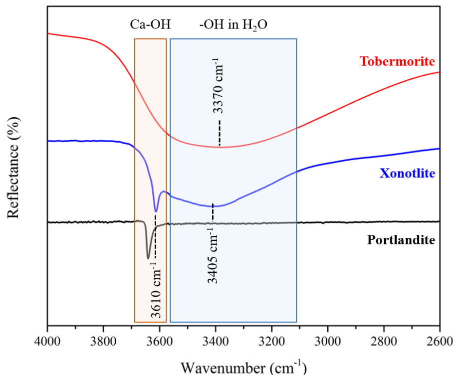
Figure 3.24: IR spectra of tobermorite (red curve) and xonotlite (blue curve) synthesised under supercritical conditions at 400 °C and 25 MPa [191]. For comparison, the IR spectrum of portlandite, collected from the RRUFF database [192], is reported in black.
