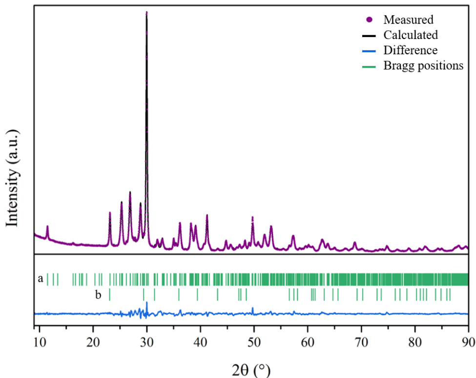
Figure 4.21: Rietveld refinement plot of sample P8 synthesised at 500 °C and 8 MPa. In the top, the measured (purple circles) and calculated (black curve) patterns are displayed; in the bottom, the difference curve between them is shown (blue line). Two crystalline phases were distinguished, (a) wollastonite-2M, and (b) calcite, as identified from their respective reflection positions (green bars).
