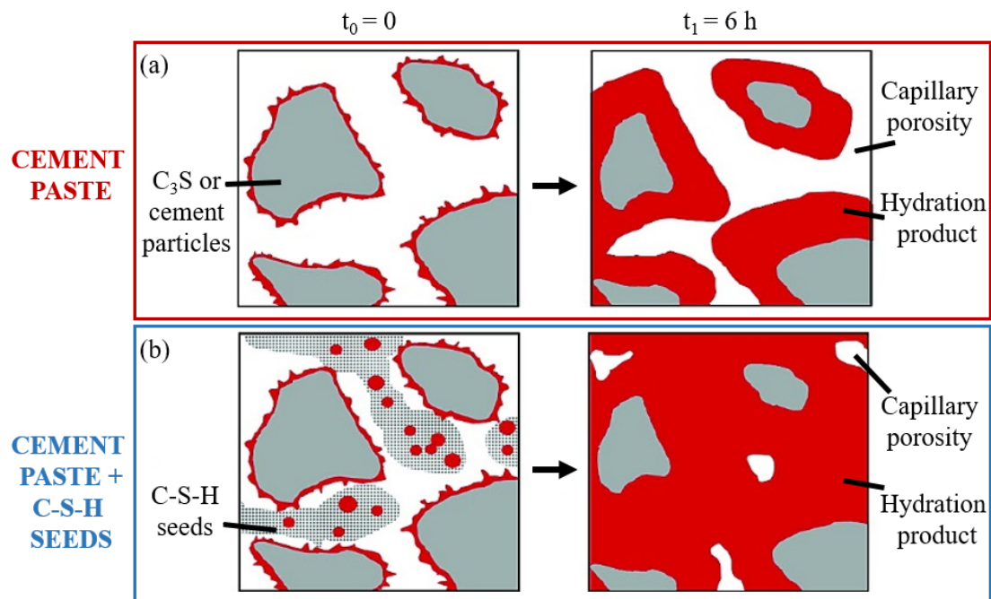
Figure 4.1: Schematic representation of the cement hydration process. (a) Few minutes after mixing an unseeded cement clinker with water, the hydration product (principally the C-S-H gel) nucleates and grows on and around the clinker particle surface. After several hours, further nucleation and growth are limited by the hydrated layer's thickness, leading to capillary porosity. (b) The addition of C-S-H seeds in cement leads to the hydration product to nucleate on both the clinker particles surface and around the seeds present in the region within the clinker particles, promoting the early hydration (adapted from [214]).
