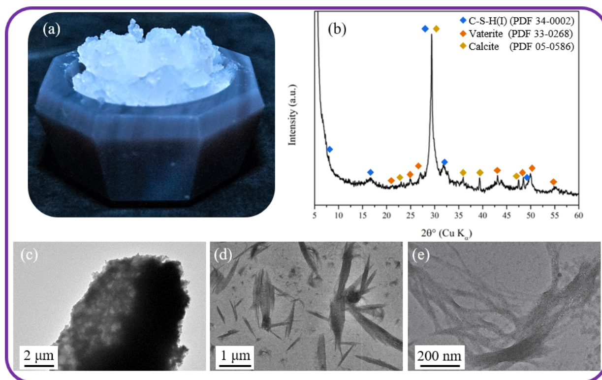
Figure 3.2: (a) Picture, (b) powder X-ray diffraction pattern, and (c)-(e) TEM images of C-S-H compound formed as precipitation product of the Ca- and Si-precursors mixing at the inlet of the reactor and at room temperature. In the PXR pattern, three phases were detected: C-S-H(I) (PDF file no. 34-0002), vaterite (PDF file no. 33-0268), and calcite (PDF file no. 05-0586).
