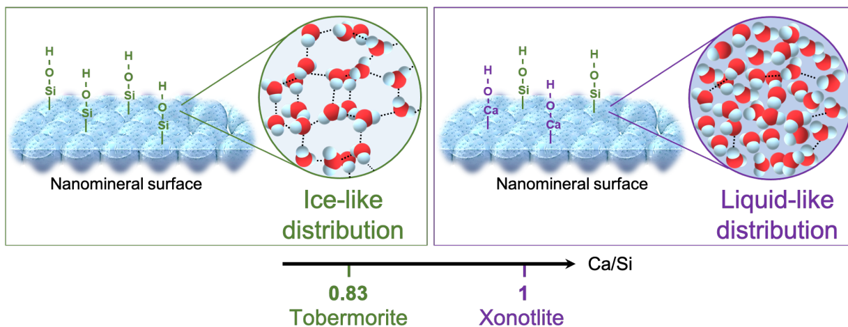
Figure 3.31: Schematic representation of the correlation between the chemical structure of xonotlite and tobermorite and its effect on nanoconfined water dynamics based on the results of this work [191].
