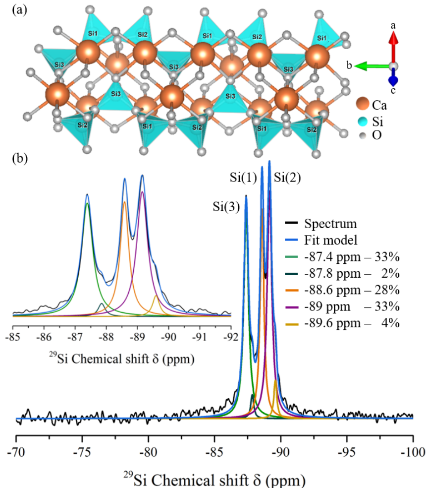
Figure 4.26: (a) Representation of the silicon environments in wollastonite-2M as reported in the crystal structure proposed by Hesse [245]. The CIF file was collected from the ICSD database [160]; (b) 29 Si MAS NMR spectrum of wollastonite synthesised upon hydrothermal dehydration of xonotlite at 8 MPa and 500 °C in 1 h. The fitted curves are presented together with the respective contributions percentage. The assignment of the peaks to the three different silicon sites is the one reported by Florian et al. [267]. The inset shows a zoom-in of the range within -85 and -92 ppm, where the extra shoulders associated with wollastonite-1T are more noticeable.
