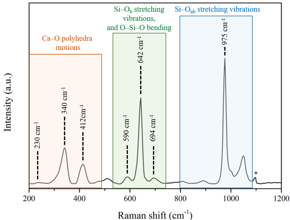
Figure 4.28: Raman spectrum, acquired in the range 200\text{--}1200\text{ cm}^{-1} , of wollastonite synthesised upon hydrothermal dehydration of xonotlite at 500\text{ }^{\circ}\text{C} , 8\text{ MPa} in 1\text{ h} . The asterisk denotes \text{C-O} stretching mode related to carbonate impurity.
