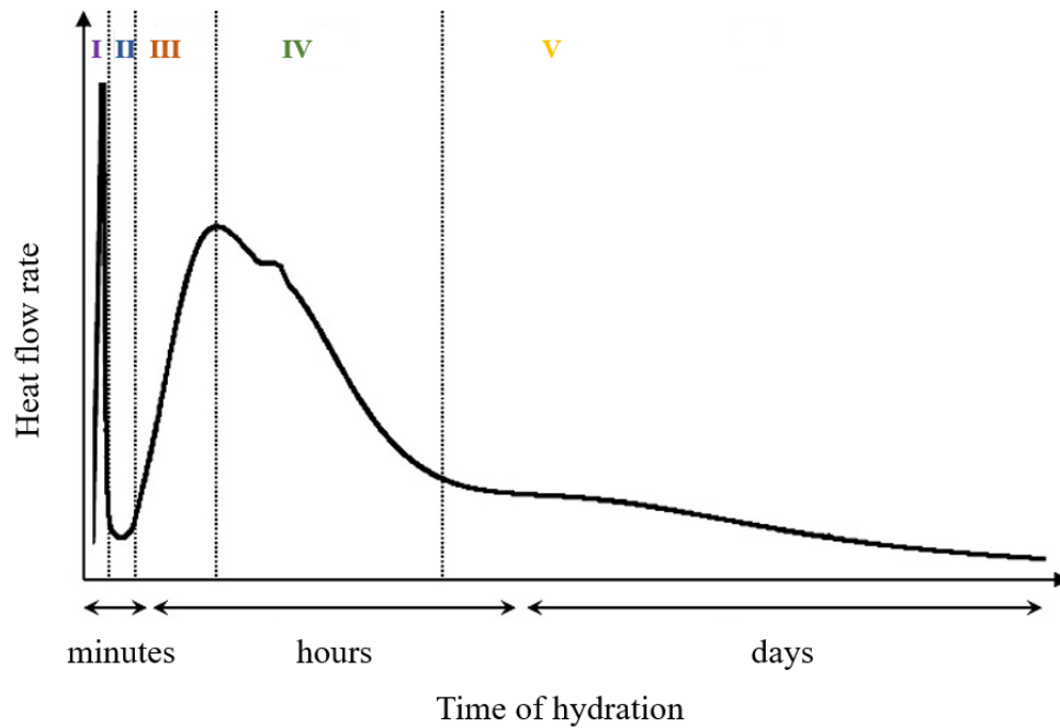
Figure 1.3: Schematic representation of the typical heat release evolution and the proposed classification of different stages during the hydration process of OPC cement [26].
