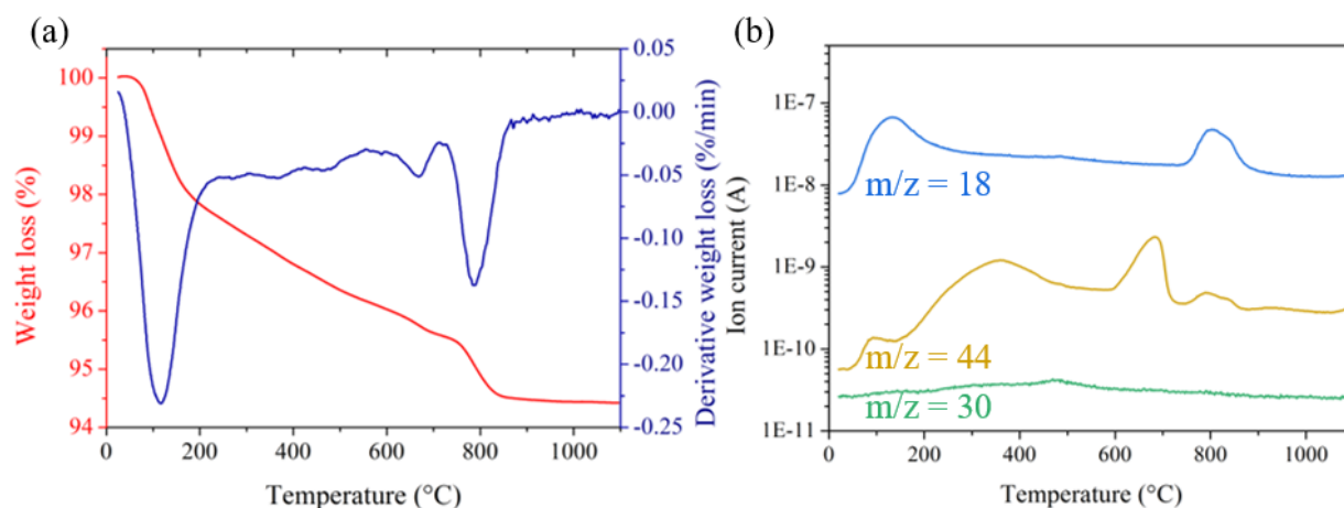
Figure 4.12: (a) Thermogravimetric curves in the range 25 - 1100 °C of weight loss (in red) and derivative weight loss (in blue) of xonotlite synthesised in this work; (b) Mass spectrometry of the exhaust from the TGA experiment for m/z = 18 (water), m/z = 30 ( \text{NO}_x ) and m/z = 44 ( \text{CO}_2 ).
