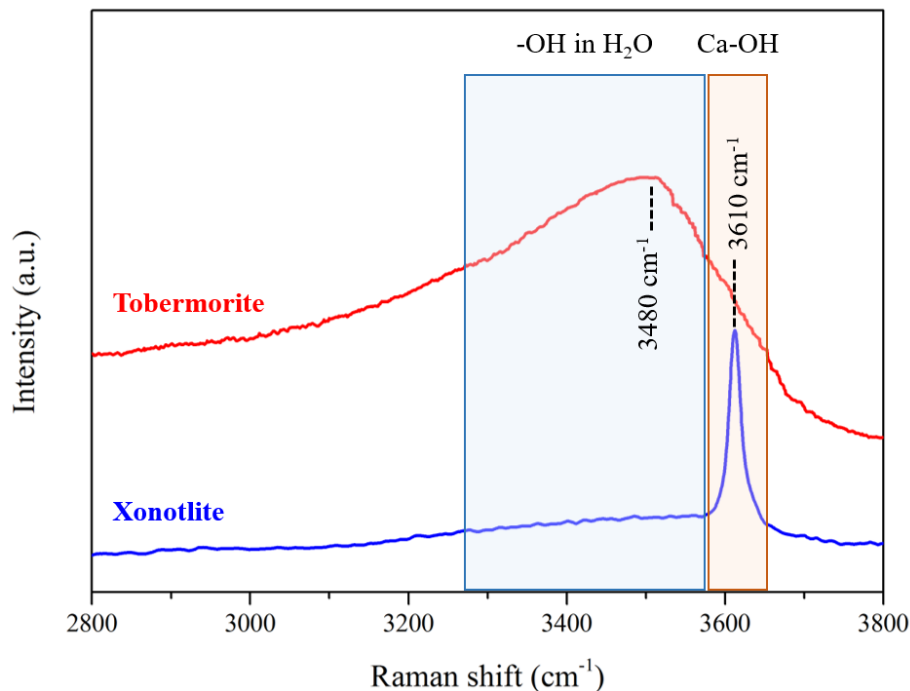
Figure 3.25: Raman spectra of tobermorite (red curve) and xonotlite (blue curve) synthesised under supercritical conditions at 400 °C and 25 MPa [191].
