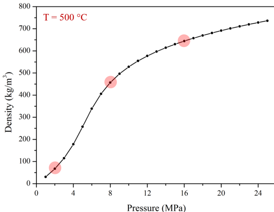
Figure 4.14: Evolution of water density ( \text{kg/m}^3 ) at T = 500\text{ }^\circ\text{C} over the pressure range 1 - 25 MPa. The red circles indicate the values of pressure (density) employed in this study. The data were collected from the NIST database [126].
