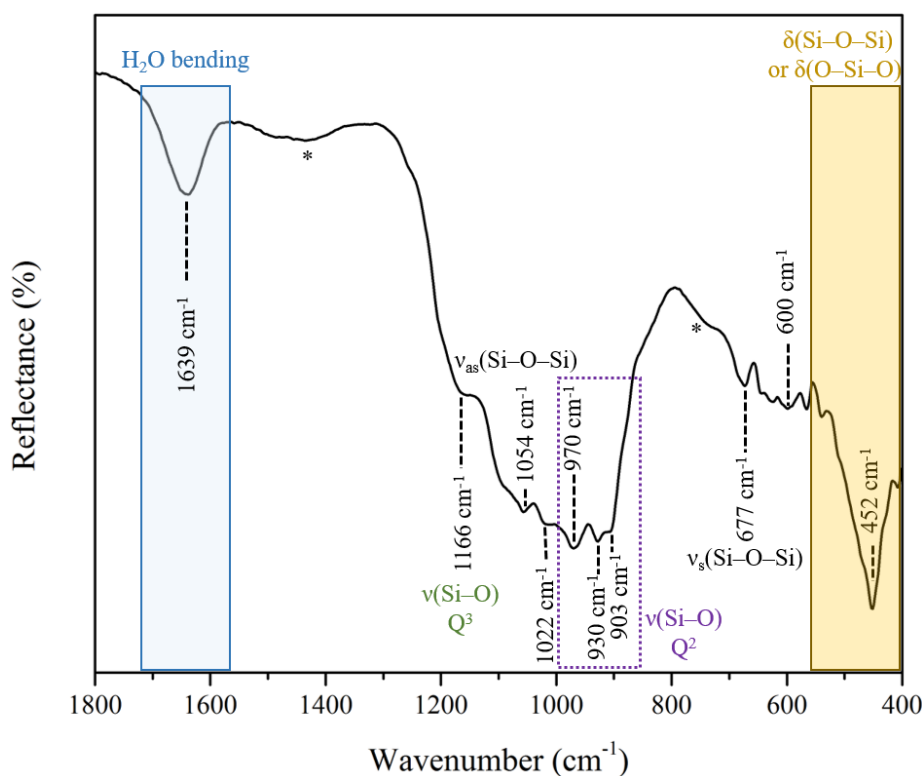
Figure 3.19: IR spectrum, recorded in the range 1800\text{--}400\text{ cm}^{-1} , of Al-tobermorite synthesised under supercritical conditions at 25\text{ MPa} and 400\text{ }^\circ\text{C} in 8\text{ s} . The asterisk denotes C–O stretching mode related to carbonate impurity.
