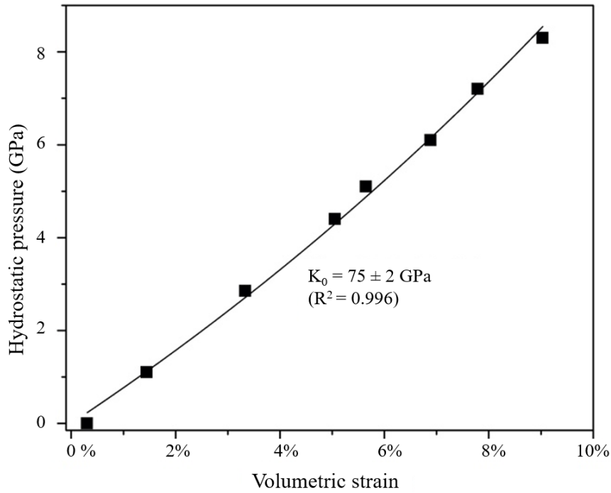
Figure 3.22: Volumetric strain determined at different hydrostatic pressure values. The data were fitted with 2 nd order BM-EoS to determine K_0 . The uncertainty of pressure is estimated to be about \pm 0.15 GPa. R^2 of the fitting is 0.996.
