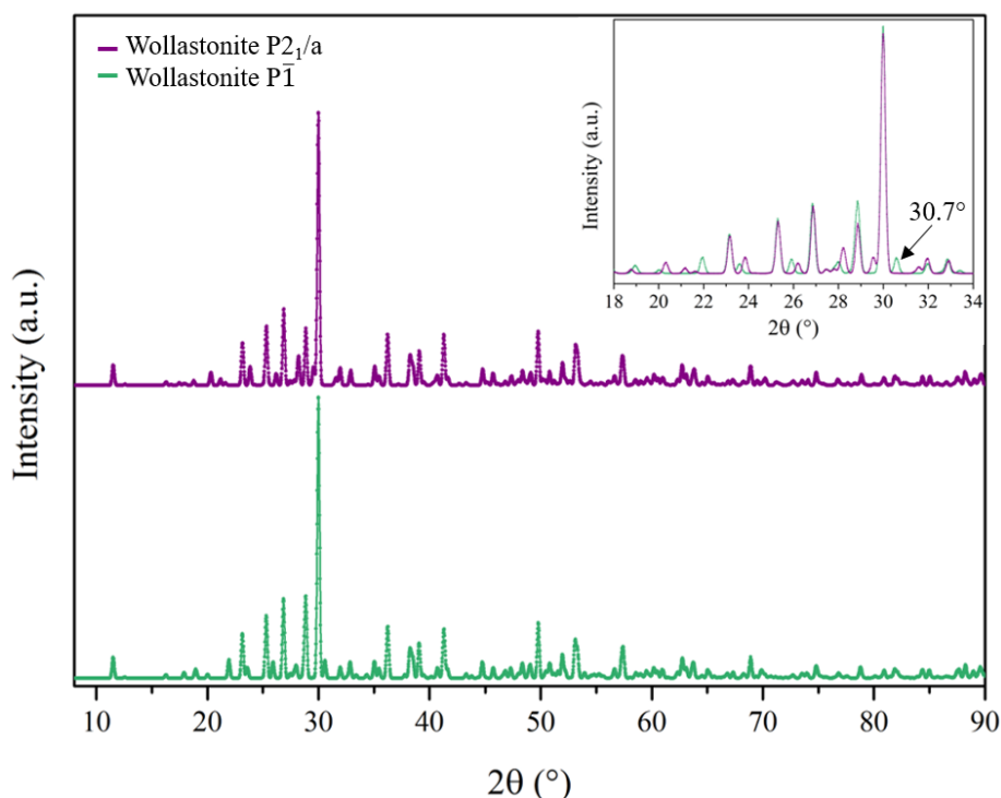
Figure 4.19: Simulation of the XRD patterns of triclinic (space group P\bar{1} ) and monoclinic (space group P2_1/a ) \beta -wollastonite performed with FullProf based on the CIF files of the mineral polytypes. The inset shows a zoom-in of the range 18-34° ( 2\theta^\circ ) where the slight differences between the two patterns are the most noticeable.
