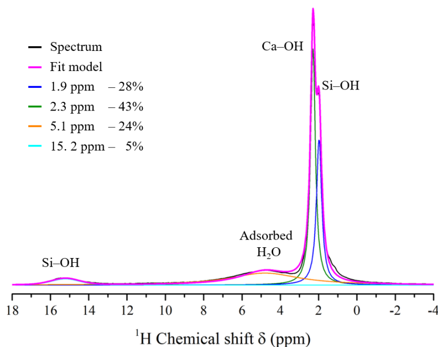
Figure 3.26: ^1\text{H} MAS NMR spectrum of xonotlite. The fitted curves are presented together with the respective contributions percentage [191].
