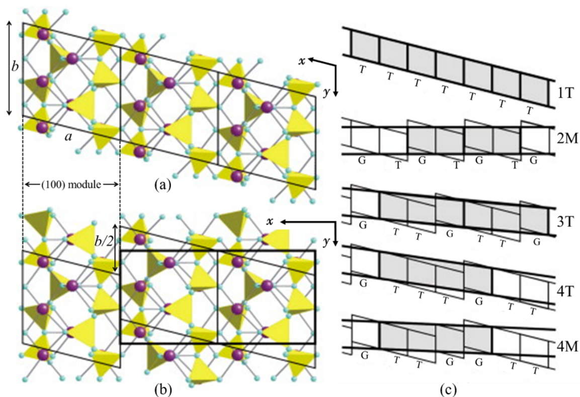
Figure 4.11: Crystal structures of wollastonite polytypes along the c -axis: (a) wollastonite-1T and (b) wollastonite-2M; (c) Schematic representation of stacking sequences of the a[(100) module] slabs for wollastonite polytypes according to Henmi et al. [242]. The unit cells are delimited by thick lines. Si tetrahedra, Ca and O atoms are depicted in yellow, purple and light blue, respectively [238].
