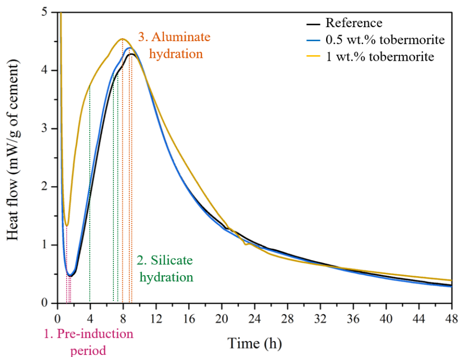
Figure 4.4: Heat flow measured over time during the hydration of reference cement paste and seeded cement pastes (tobermorite addition 0.5 and 1 wt.%).
