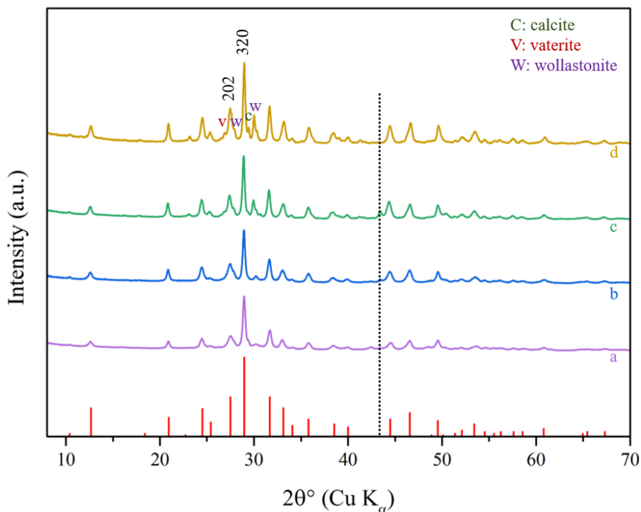
Figure 3.3: Powder X-ray diffraction patterns of samples T250, T300, T350 and T400 synthesised under near- and supercritical conditions at 23.5 MPa and (a) 250 °C, (b) 300 °C, (c) 350 °C and (d) 400 °C, respectively. In red, the positions and intensities of the diffraction peaks as reported in PDF file no. 00-023-0125 of monoclinic xonotlite (space group P2/a) are shown. The letters C, V, and W indicate diffraction peaks of calcite, vaterite or wollastonite phases, respectively. The vertical black dot line indicates diffraction from the stainless steel sample holder.
