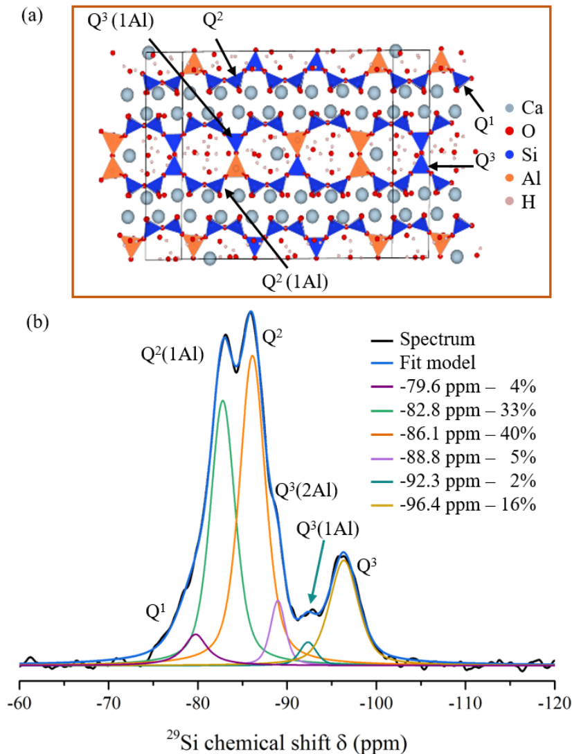
Figure 3.16: (a) Structural model proposed for Al-anomalous tobermorite, thanks to a combination of NMR and simulation results, by Dupuis et al. [170]. (b) 29 Si MAS NMR spectra of Al-tobermorite synthesised under supercritical conditions at 25 MPa and 400 °C in 8 s. The fitted curves are presented together with the respective contributions percentage.
