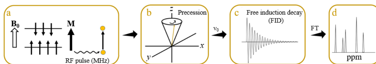
Figure A.2: Schematic representation of NMR working principle. (a) The whole spin system at equilibrium shows a net magnetisation, M , aligned along the direction of the external magnetic field B_0 ; a radio frequency (RF) pulse excites the nuclei generating a transition in the spin energy levels. (b) The magnetisation is subjected to a precessional motion, which in turn gives rise to the emission of a (c) free induction decay signal. (d) The Fourier Transform (FT) of such signal provides the NMR spectrum.
