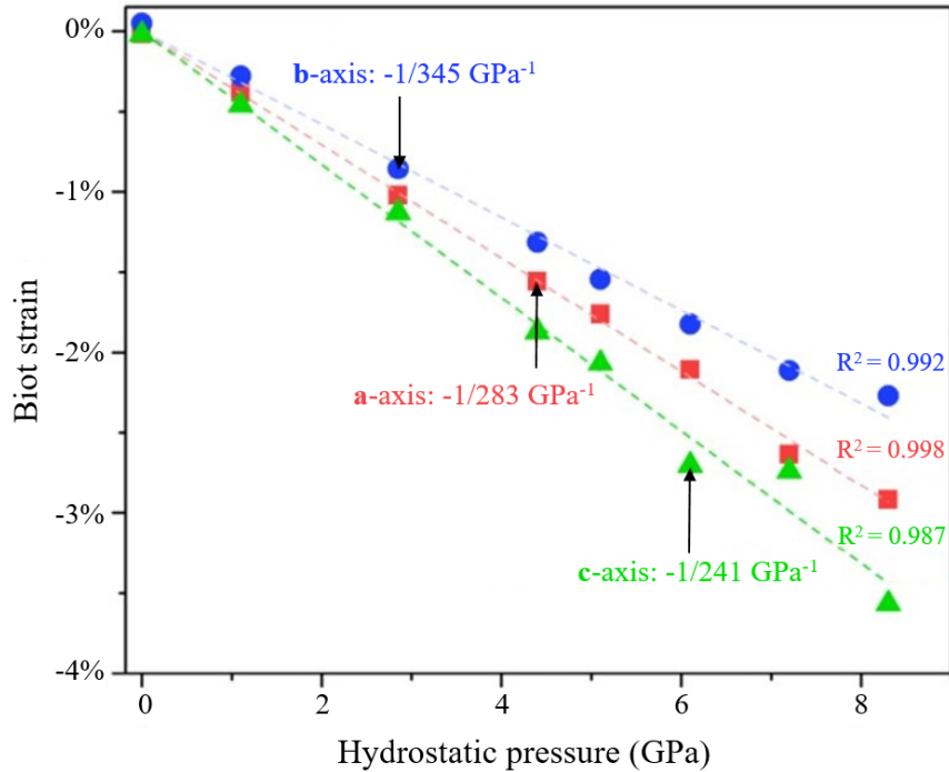
Figure 3.21: (a) Biot strain as a function of applied hydrostatic pressure along the a-, b-, and c-axes. The uncertainty of pressure is estimated to be about \pm 0.15 GPa. The uncertainty of the Biot strain is below \sim 0.15\% . R^2 of the fittings are above 0.987.
