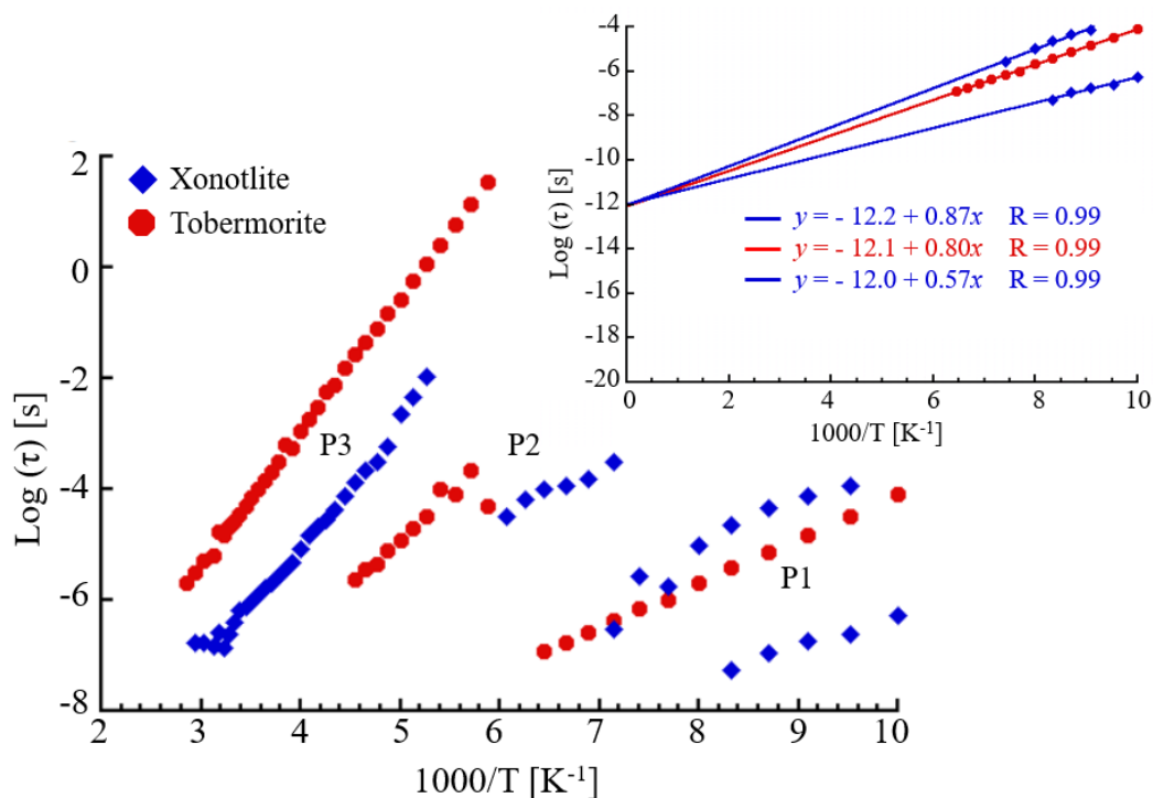
Figure 3.30: Temperature dependence of relaxation times related to the observed dynamics in tobermorite (in red) and xonotlite (in blue) synthesised in SCW. The inset shows the fit for each P1 process, together with the calculated fit equations used to determine the \tau_0 and E_a values [191].
