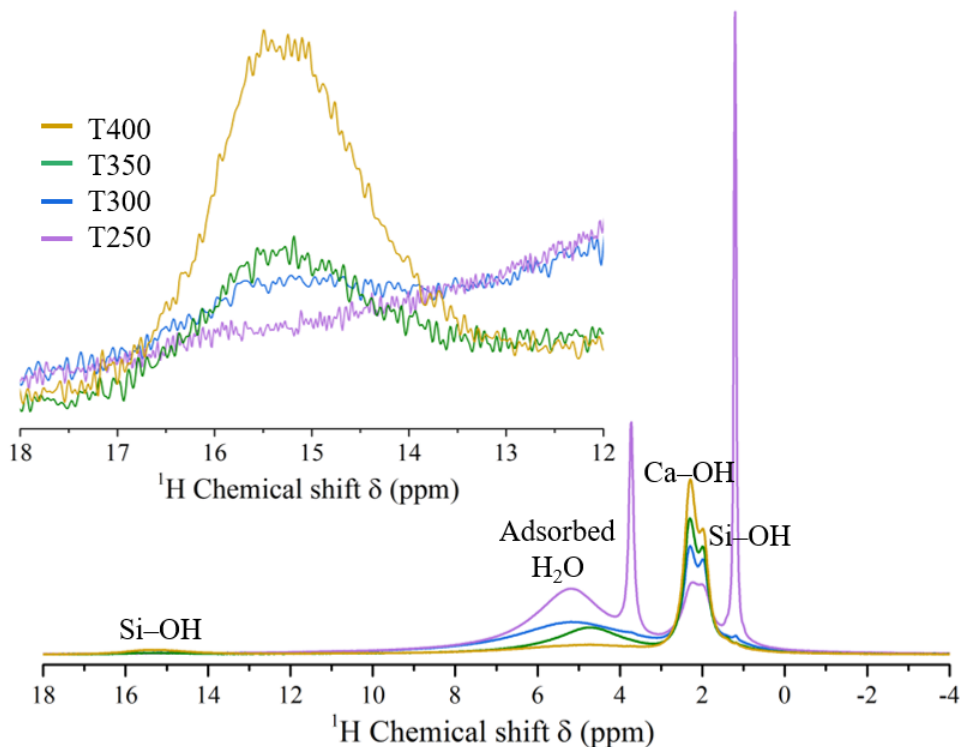
Figure 3.4: ^1\text{H} MAS NMR spectra of samples T250, T300, T350, and T400 synthesised under near- and supercritical conditions at 23.5 MPa and 250, 300, 350 and 400 ^{\circ}\text{C} , respectively. The spectra are normalised for the material mass and the number of scans, and thus comparable to each other. The inset shows a zoom in the range within 12 and 18 ppm of the spectra.
