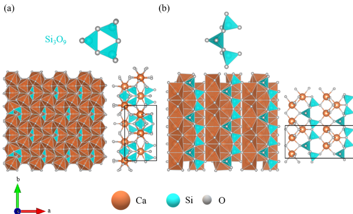
Figure 4.10: Structure of (a) \alpha -wollastonite and (b) \beta -wollastonite. The black rectangle represents the limits of the unit cell. The CIF files with the reference structures were collected from the ICSD database [160].
