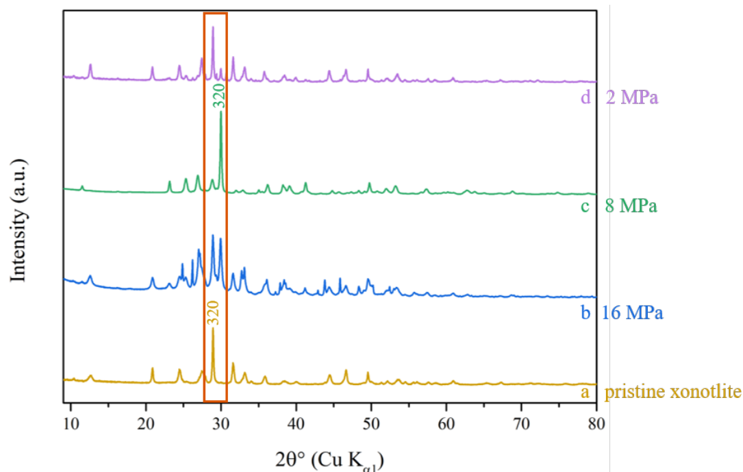
Figure 4.17: (a) PXRD pattern of pristine xonotlite phase. PXRD patterns of samples synthesised upon hydrothermal dehydration at 500^{\circ}\text{C} for 1 h at different pressure values: (b) 16 MPa, (c) 8 MPa and (d) 2 MPa. The pattern of pristine xonotlite in (a) shows the characteristic (320) diffraction peak at 28.9^{\circ} ( 2\theta^{\circ} ), while the characteristic (320) diffraction peak of wollastonite appears at 30.1^{\circ} ( 2\theta^{\circ} ) in the other diffraction patterns.
