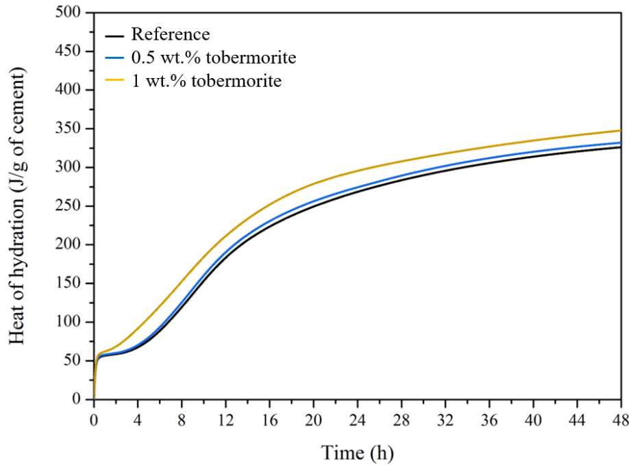
Figure 4.5: Cumulative heat measured over time during the hydration of reference cement paste and seeded cement pastes (tobermorite addition 0.5 and 1 wt.%).
