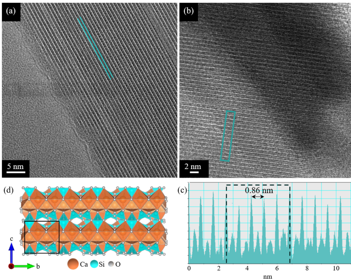
Figure 3.9: (a) and (b) HR-TEM images of xonotlite fibres, synthesised under supercritical conditions, showing the ordered and well-arranged crystal lattice of the material. (c) Distance profile derived from the light blue region in (b) to measure the interlayer distance between planes related to reflection (200) and perpendicular to the fibre's length. (d) Crystal structure of xonotlite as reported in the CIF file of the ICSD database [160] by Hejny et al. [44].
