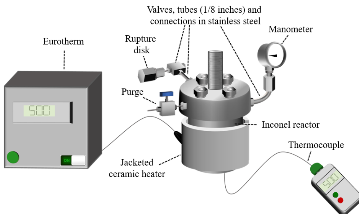
Figure 4.15: Experimental set-up for the synthesis of wollastonite upon xonotlite dehydration. The principal part of the system is a batch reactor made in Inconel. All the connections, tubes (external section 1/8 inch, i.e. 3.175 mm) in the upper part of the set-up, and the manometer are built-in stainless steel.
