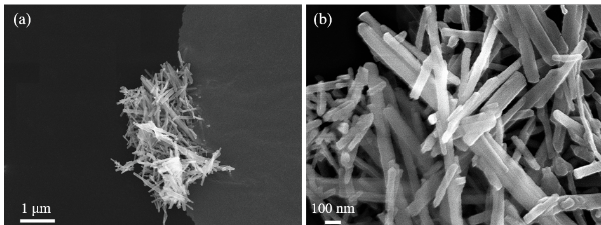
Figure 4.24: HR-SEM images of wollastonite fibres at different magnifications (a) \times 4,000 and (b) \times 65,000 . The images were acquired using acceleration voltage and working distance equal to 15 kV and 3 mm, respectively.
