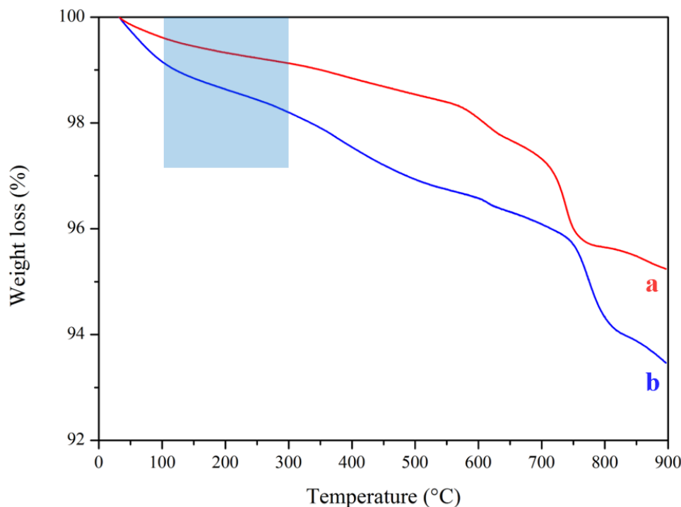
Figure 3.28: Thermogravimetric curves of (a) tobermorite and (b) xonotlite synthesised under supercritical conditions [191].
