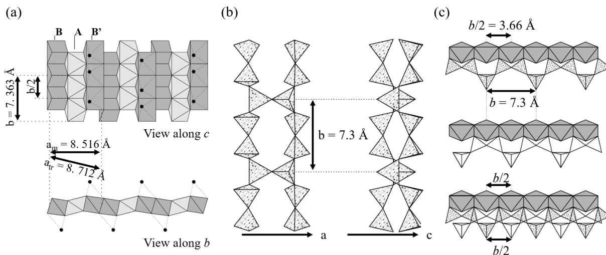
Figure 1.8: Representation of (a) CaO-polyhedral sheet in the structure of xonotlite. Chains of Ca atoms seven-fold coordinated, type B and B', Ca atoms octahedrally coordinated, type A, are represented in dark grey and light grey, respectively. The seven-fold coordination structure forms a trigonal prism where black dots represent a seventh oxygen atom; (b) \text{Si}_6\text{O}_{17} -dreier-doppelkette double chain in the structure of xonotlite seen along the c -axis (left) and along the a -axis (right); (c) the two different possibilities of connecting a silicon tetrahedra chain (with a periodicity of three \text{SiO}_4 ) to a column of calcium octahedra (type A) in xonotlite (top and middle) and column of calcium octahedra with two superimposed \text{SiO}_4 chains (bottom) [44].
