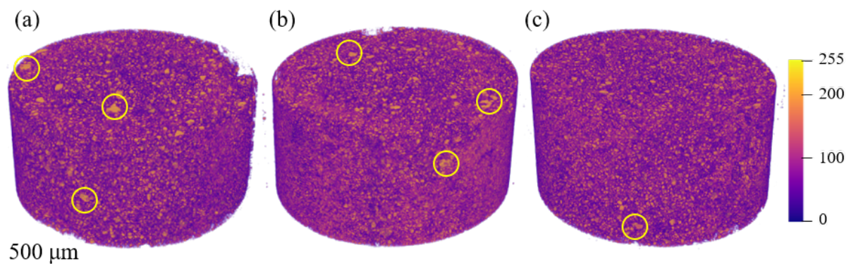
Figure 4.8: Visualisation of the reconstructed 3D \mu CT images of (a) reference sample, (b) 1 wt.% tobermorite, and (c) 1 wt.% xonotlite seeded cement pastes obtained with Tomviz . The \mu CT tomograms were acquired at 7 h of hydration for all samples. Yellow circles indicate unhydrated clinker particles, which appear bigger in size in the reference sample than in the seeded pastes.
