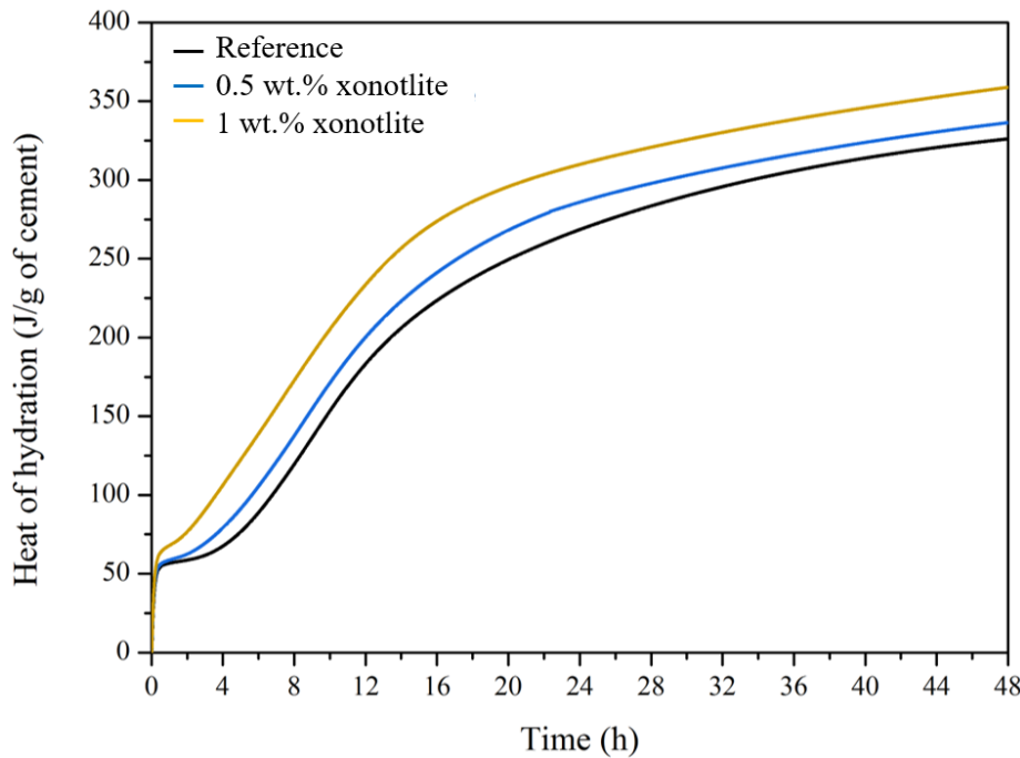
Figure 4.3: Cumulative heat measured over time during the hydration of reference cement paste and seeded cement pastes (xonotlite addition 0.5 and 1 wt.%).
