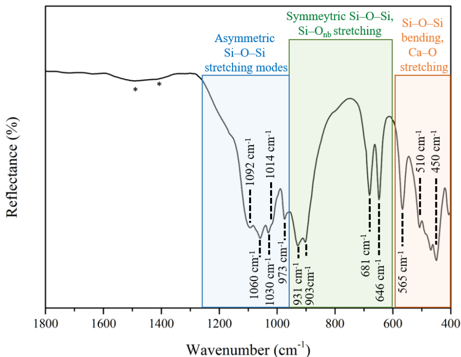
Figure 4.27: IR spectrum, acquired in the range 1800-400 cm -1 , of wollastonite synthesised upon hydrothermal dehydration of xonotlite at 500 °C, 8 MPa in 1 h. The asterisk denotes C–O stretching mode related to carbonate impurity.
