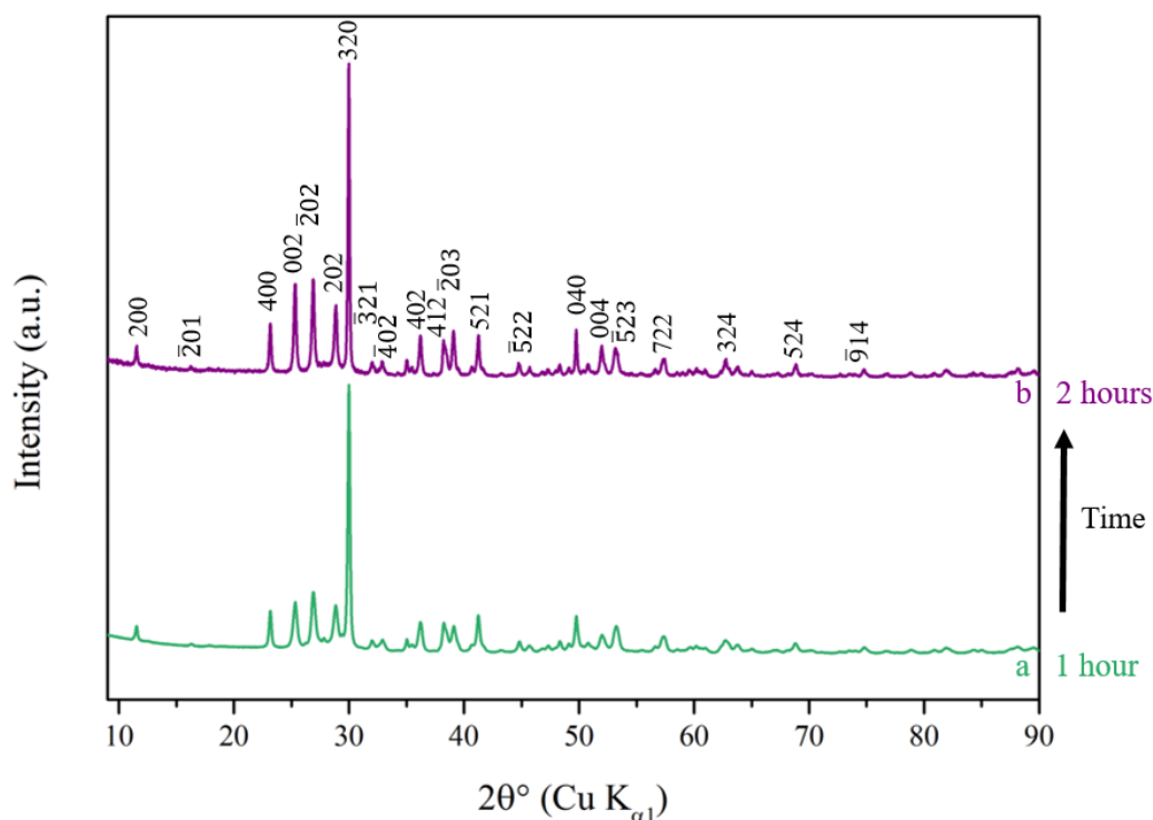
Figure 4.23: PXRD patterns of wollastonite samples synthesised upon hydrothermal dehydration treatment of xonotlite at 500 °C and 8 MPa for (a) 1 h and (b) 2 h. The principal diffraction peaks are identified by the corresponding Miller indices, according to PDF no. 43-1460 of wollastonite-2M reported in the ICDD database.
