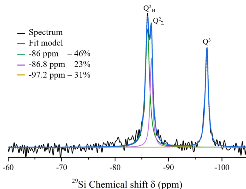
Figure 3.10: ^{29}\text{Si} MAS NMR spectrum of xonotlite synthesised under supercritical conditions at 25 MPa and 400 °C in 7 s.
