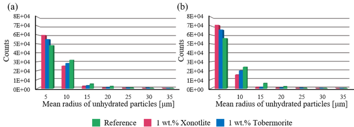
Figure 4.9: Distribution of mean radius of unhydrated particles ( \mu\text{m} ) determined for reference and seeded cement pastes at (a) 7 h and (b) 36 h.
