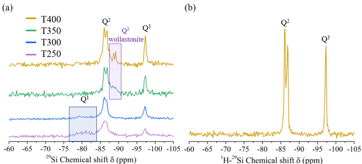
Figure 3.6: (a) ^{29}\text{Si} MAS NMR spectra of samples T250, T300, T350, and T400 synthesised under near- or supercritical conditions at 23.5 MPa and 250, 300, 350, and 400 °C, respectively.
