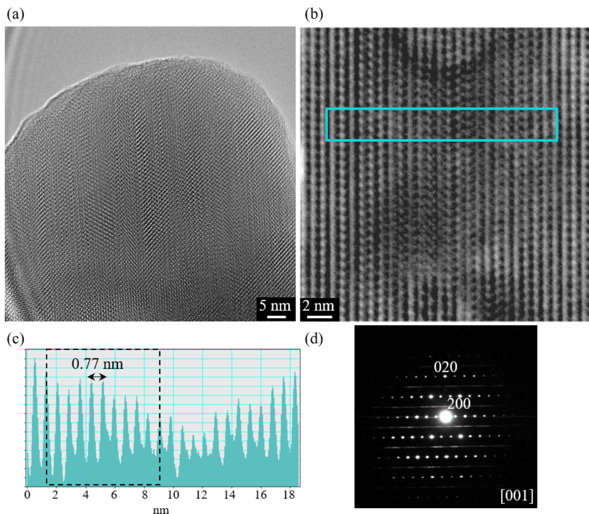
Figure 4.25: (a) and (b) HR-TEM images showing the ordered and well arranged crystal lattice of wollastonite fibres. (c) Distance profile, derived from the light blue region in (b), representing the interplanar spacing of 0.77 nm between (200) planes. (d) SAED pattern, obtained from the region marked in (b), indicates the characteristic reflection of wollastonite from (200) and (020) families of lattice planes.
