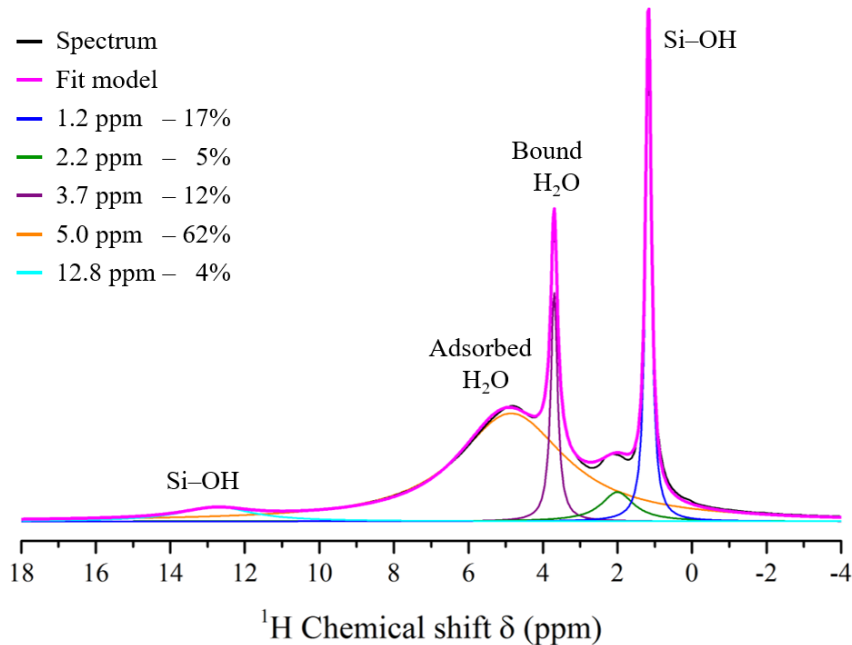
Figure 3.27: ^1\text{H} MAS NMR spectrum of tobermorite. The fitted curves are presented together with the respective contributions percentage [191].
