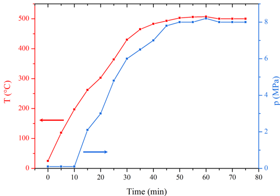
Figure 4.16: Temperature-pressure profiles show the evolution of temperature T and pressure p over time. The data were acquired during the heating step of a synthesis in which 6 mL of water were loaded into the batch reactor.
