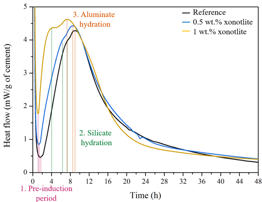
Figure 4.2: Heat flow measured over time during the hydration of reference cement paste and seeded cement pastes (xonotlite addition 0.5 and 1 wt.%).
