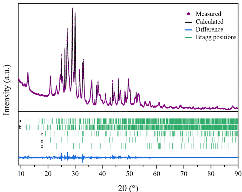
Figure 4.20: Profile Matching plot of sample P16 synthesised at 500 °C and 16 MPa. In the top, the measured (purple circles) and calculated (black curve) patterns are displayed; in the bottom, the difference curve between them is shown (blue line). Five crystalline phases were distinguished: (a) wollastonite-2M, (b) xonotlite, (c) aragonite, (d) vaterite, and (e) calcite, as identified from their respective reflection positions (green bars).
