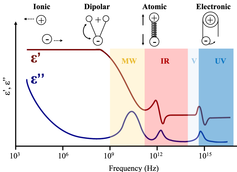
Figure 2.7: Illustration of dielectric response over a wide range of frequencies. \epsilon' and \epsilon'' indicate the real and the imaginary part of the permittivity, respectively. Several processes are pictured as a function of the frequency: ionic and dipolar relaxations, and atomic and electronic resonances (adapted from [138]).
