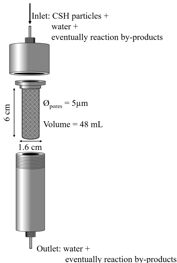
Figure 2.4: Schematic representation of the product recovery system employed in this work.
