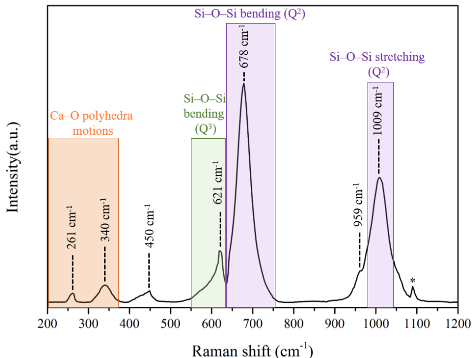
Figure 3.18: Raman spectrum, acquired in the range 200–1200 \text{cm}^{-1} , of Al-tobermorite synthesised under supercritical conditions at 25 MPa and 400 °C in 8 s. The asterisk denotes C–O stretching mode related to carbonate impurity.
