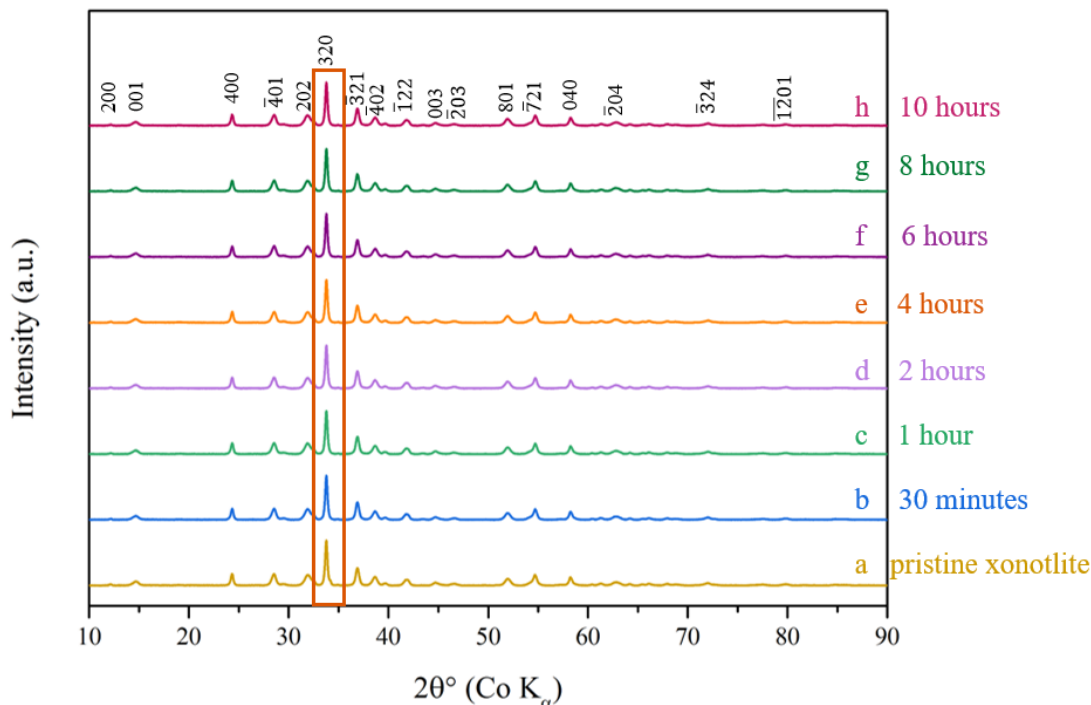
Figure 4.18: (a) PXRD pattern of pristine xonotlite acquired at room temperature before starting heating. Isothermal HT-PXRD patterns acquired in situ during a conventional heating treatment at 500 °C and different times: (b) 30 min, (c) 1 h, (d) 2 h, (e) 4 h, (f) 6 h, (g) 8 h, and (h) 10 h. Each peak is identified by the corresponding Miller indices as reported in the PDF file no. 00-023-0125 of monoclinic xonotlite (space group P2_1/a ).
