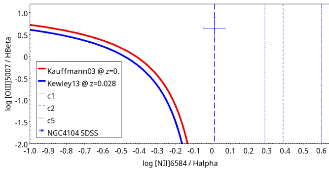
Fig. 13. \log([OIII]5007/H\beta) versus \log([NII]6584/H\alpha) for the SDSS spectrum (central area, see e.g. Fig. B.1) and the c1, c2, and c5 MISTRAL regions. Regions under the red and blue curves are normal galaxies, according to Kauffmann et al. (2003) and Kewley et al. (2013) respectively, while regions above these curves are active objects (AGN, LINERS).
