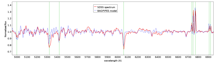
Fig. 12. A modelisation of the normalized SDSS spectrum of NGC 4104 with the pipes_vis tool.
