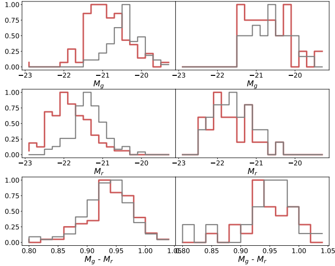
Fig. 4. Normalized histograms of the absolute magnitudes of the BGGs in the g (top) and r (middle) bands, and of the (g-r) colour (bottom), for FGs (red) and non-FGs (grey). Left: the 87 FGs and 100 non-FGs. Right: 25 FGs and 30 non-FGs analysed morphologically.
