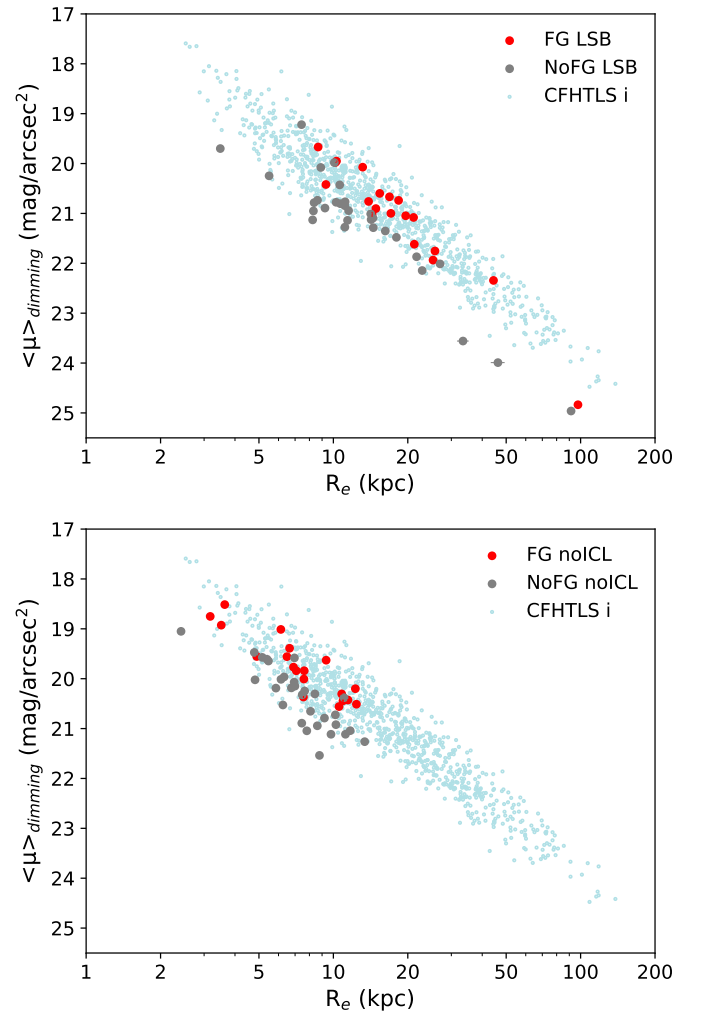
Fig. 7. Kormendy relation for FGs in red and Non-FGs in grey, superimposed on the relation found for almost one thousand BCGs by Chu et al. (2022) in cyan. Both plots are obtained in the rLSB band, the top plot without ICL subtraction and the bottom plot after ICL subtraction. The points for FGs and non-FGs have been shifted from the r to the i band, and all points are corrected for cosmological dimming.
