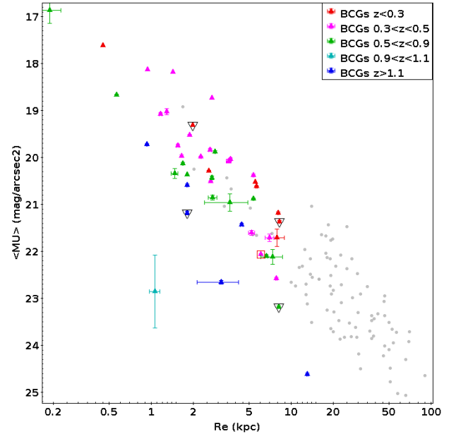
Fig. 17. Same as Fig. 16, but for the inner component of BCGs fitted with two components. The gray points are the same as in Fig. 16.
