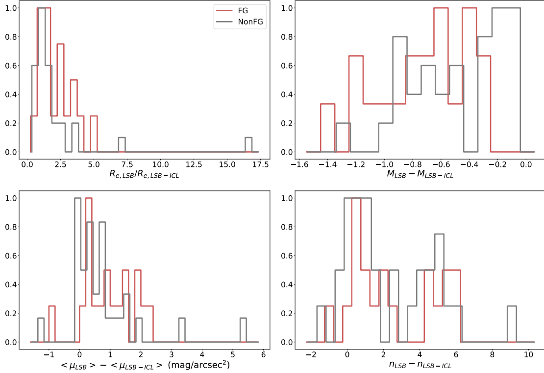
Fig. 8. Normalized histograms of the difference between the values obtained before and after subtraction of the ICL for the 19 candidate FGs (in red) and 30 non-FGs (in grey): effective radius (top left), absolute magnitude (top right), mean surface brightness (bottom left), and Sérsic index n (bottom right).
