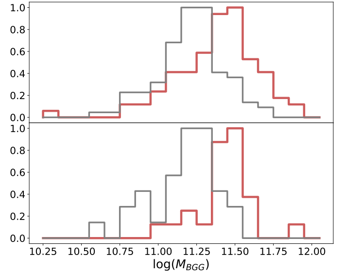
Fig. 2. Same as Fig. 1 for the normalized histograms of the logarithms of the BGG stellar masses.
