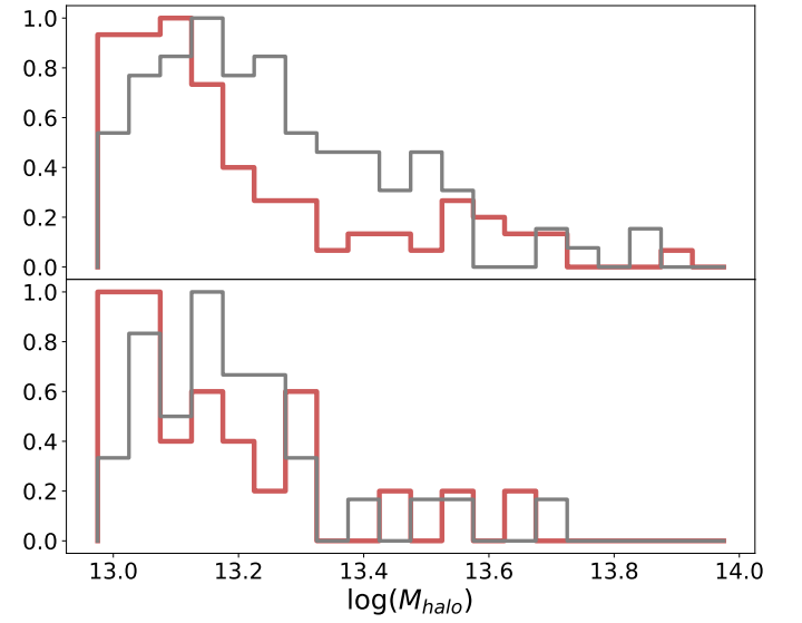
Fig. 1. Normalized histograms of the logarithms of the halo masses for FGs (red) and non-FGs (grey). Top: the 87 FGs and 100 non-FGs. Bottom: 25 FGs and 30 non-FGs analysed morphologically.
