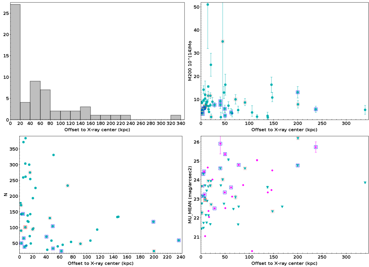
Fig. 21. Top left: histogram of the offsets between the BCG and the X-ray center. Top right: masses M_{200,c} of the clusters as a function of the offsets between the BCG and the cluster X-ray center. Bottom left: richness of the cluster as a function of the offsets between the BCG and the cluster X-ray center. Bottom right: mean effective surface brightness of the BCGs as a function of the offsets between the BCG and the cluster X-ray center.
