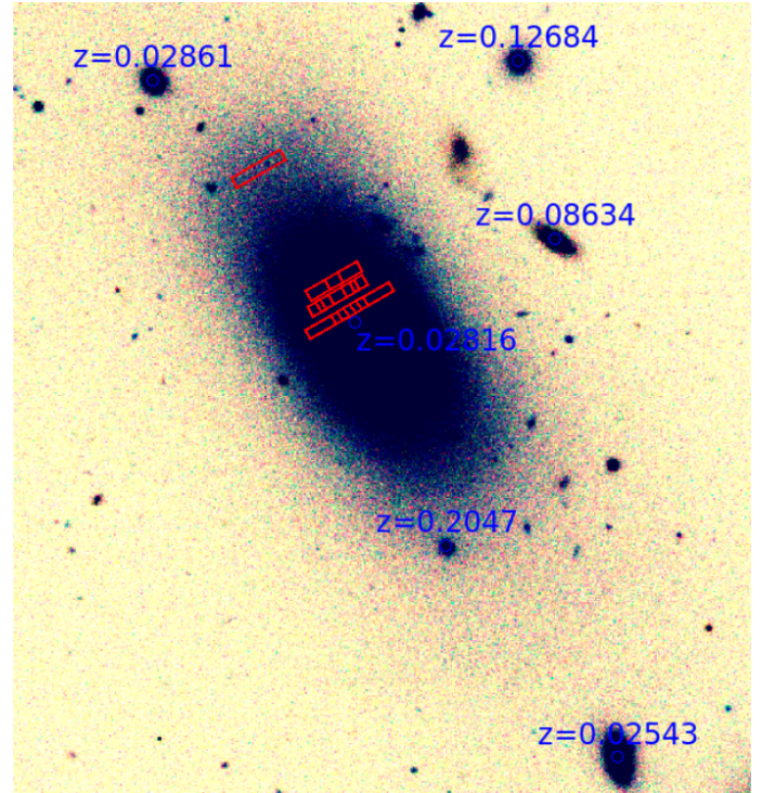
Fig. 10. SDSS g' , r' , i' trichromatic image ( \sim 2.9' \times 3.5' ) of NGC 4104. The redshifts indicated come from the SDSS. The red rectangles show the regions where we extracted MISTRAL spectra.
