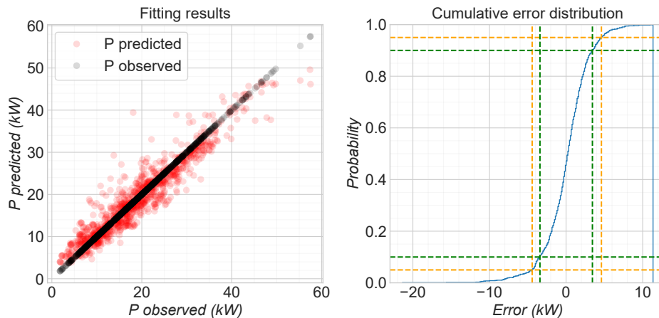
Figure 5.12: Power consumption forecasting accuracy on selected preheating timesteps.
