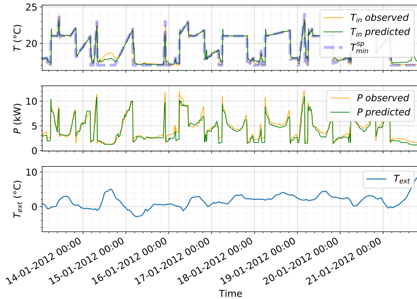
Figure 4.29: RF estimators for indoor temperature: T_{in,t} \approx f_{RF}(X_t, \bar{X}_{t-1,\dots,t-N}) , where X = (T_{sp}^{min}, T_{ext}, \Phi_{irr}, TOD, DOW)^T and N=8 (2 hours), and power consumption: P_t \approx f_{RF}(X_t) , X = (T_{in}, T_{sp}^{min}, T_{ext}, \Phi_{irr}, TOD, DOW)^T . Validation on IDA ICE building simulated using ramp preheating setpoints.
