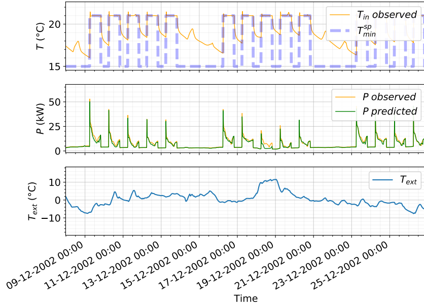
Figure 4.32: RF power consumption forecasting results based on past and current feature values: y_t \approx f_{RF}(X_t, \bar{X}_{t-1, \dots, t-N}) , where X = (T_{sp}^{min}, T_{ext}, \Phi_{irr}, TOD, DOW)^T and N=8 (2 hours). Validation on IDA ICE building with night setback temperature control.
