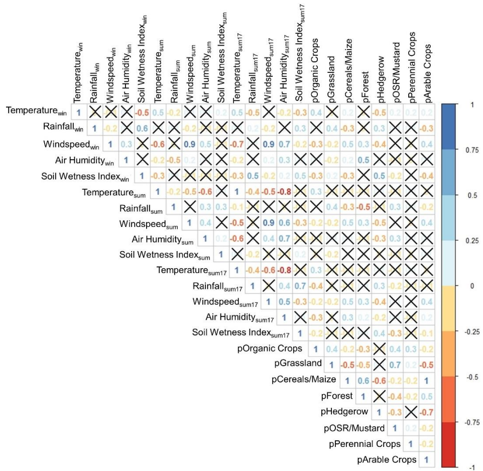
Figure S4. Matrix of correlations between all explanatory weather and landscape variables.
