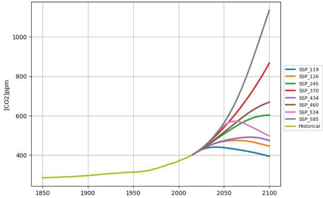
Figure A 2 - CO 2 annual global-mean surface concentration (ppm) was obtained from the consolidated database of historical and projected atmospheric greenhouse gases concentration from the climate-carbon-cycle model MAGICC7.0 adapted from (Meinshausen et al., 2020).
