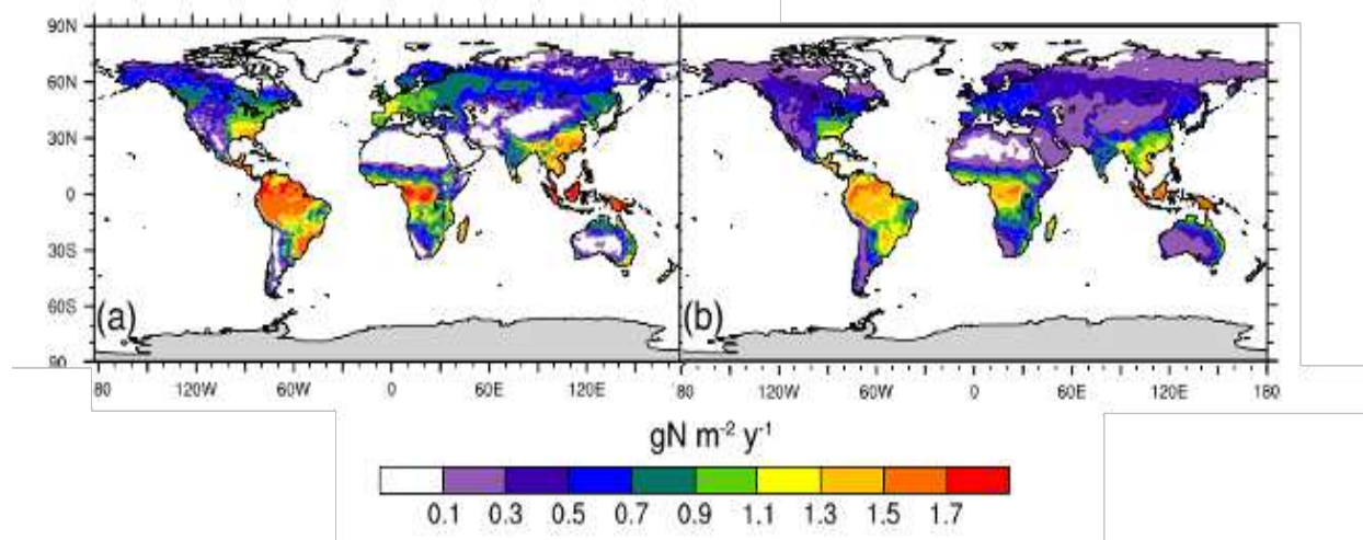
Figure 5.5 - Results for modeled BNF in \text{gN m}^{-2} \text{yr}^{-1} for (a) CLM4.5 using the standard NPP structure, (b) CLM4.5 using the standard evapotranspiration structure and (Wieder et al., 2015).
