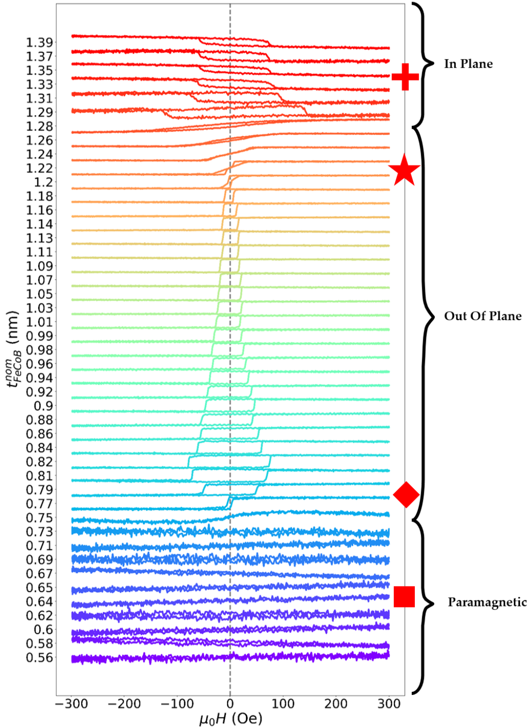
Figure 4.5: Hysteresis loops versus ferromagnetic thickness after sample annealing: Normalized hysteresis loops at t_{Ta} \simeq 0.98 nm (optimally oxidized FeCoB/TaO x interface after annealing) for various nominal ferromagnetic thickness, indicated on the y -axis. The symbols corresponds to the different locations indicated in Fig. 4.4a. It allows to distinguish three different magnetic states : the paramagnetic state (bottom part of the graph, square symbol) corresponds to a noisy signal, while square-shaped hysteresis loop are observed in the out of plane region (middle part of the graph, between diamond and star symbols). In the in plane region (top part of the graph, cross symbol), the signal is weaker and the loop is inverted, due to the opposite sign of polar and longitudinal signals in the setup.
