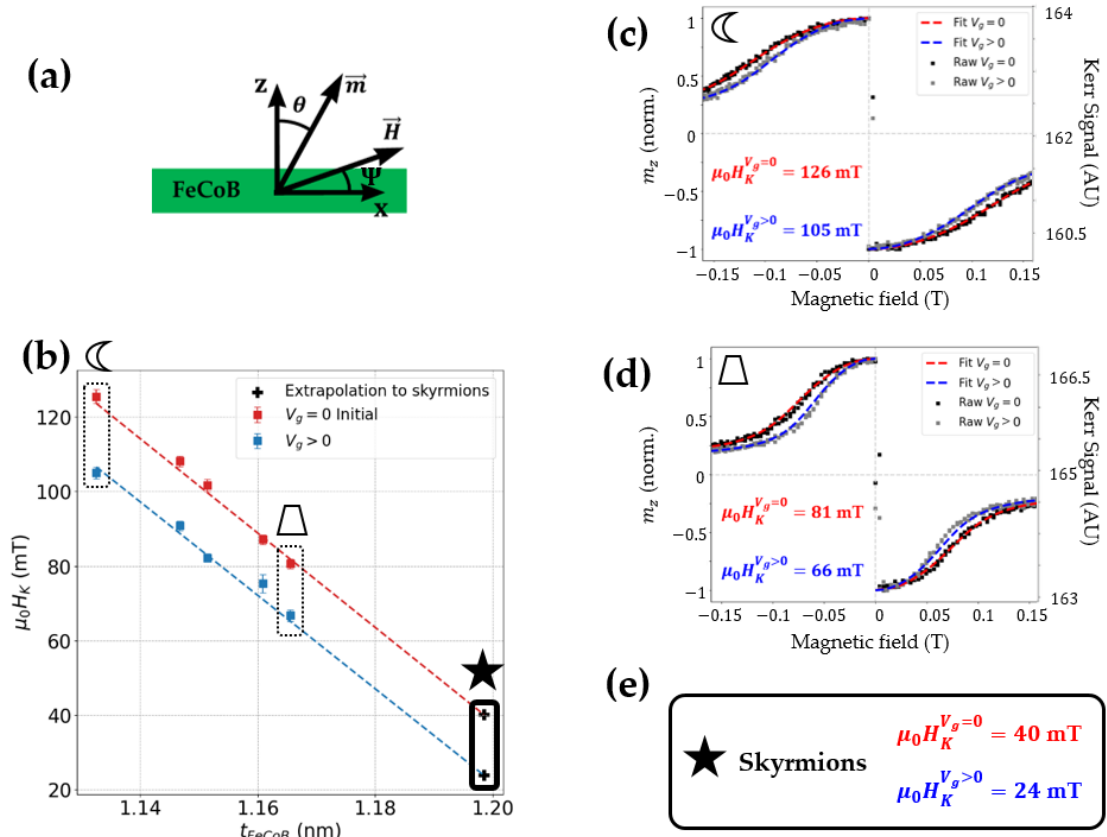
Figure 5.11: Variation of the magnetic anisotropy under gate voltage: (a) Geometry considered in our energetic model. (b) Anisotropy fields measured at V_g = 0 (red data points) and V_g > 0 (blue data points). It is possible to extrapolate values for skyrmions, as depicted by the dashed lines and the "+" symbols. (c,d) Raw data and their fit respectively for thinner and thicker FeCoB thickness. (e) An extrapolation at the FeCoB thickness at which skyrmions are observed allows to extract the values of anisotropy field and its variation under gate voltage in the region of interest.
