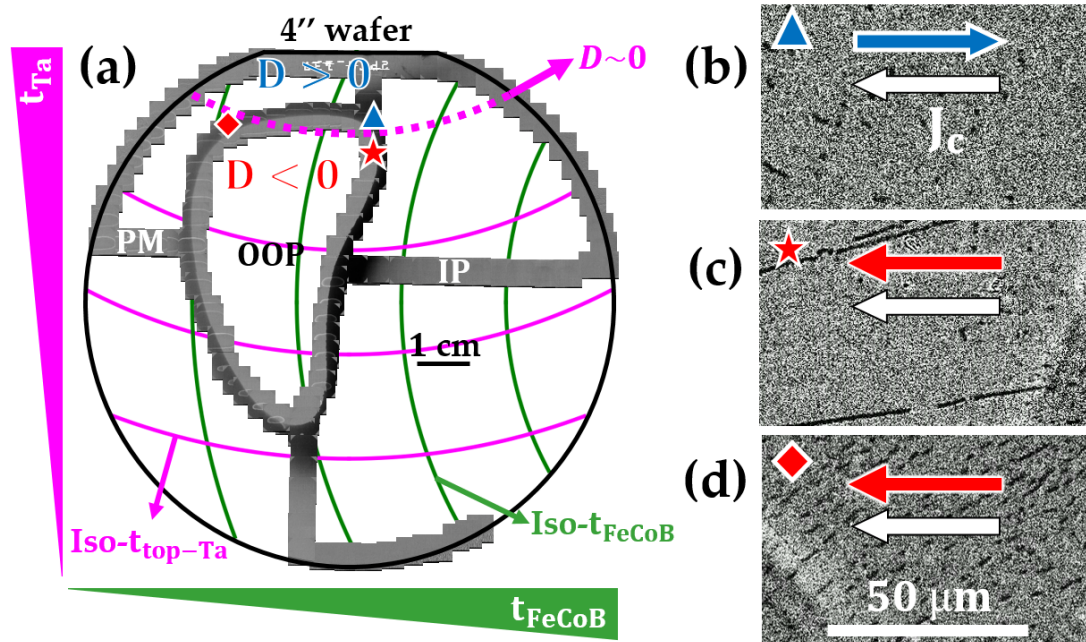
Figure 4.13: Possible influence of the deposition geometry: (a) Real scale representation of the iso-thickness curves on the sample. The D = 0 curve could correspond to an iso-thickness of the top-Ta layer which could explain our observation of iDMI and CIM inversion by moving horizontally. (b)-(c)-(d) CIM measurements.
