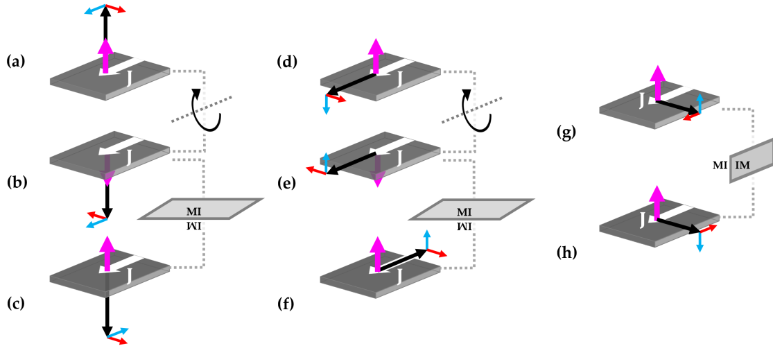
Figure 2.20: SOT vs magnetization direction: The torques directions as a function of the magnetization direction can be obtained by using the system symmetries. For an electric field pointing along +z , (a) shows the torque directions for magnetization pointing along +z , (c) along -z , (d) along x , and (f) along -x . (b,e) Moreover, using the systems symmetries, the torques directions can also be determined when the electric field points along -z . (g,h) If the magnetization is in-plane and perpendicular to the current density (here y axis), the system acquires a (x,z) mirror symmetry which leads to zero net SOT by compensation.
