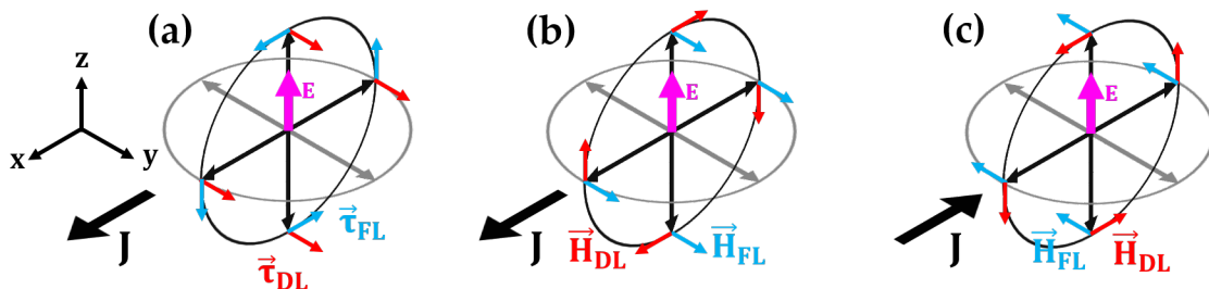
Figure 2.21: Spin orbit torques direction determined from symmetry consideration in a system lacking inversion symmetry: (a) Direction of the field-like (blue arrows) and damping-like (red arrows) torques under \vec{j} = J\vec{x} (black arrow in the bottom left) as a function of magnetization direction. (b) direction of the corresponding effective magnetic field for \vec{j} = J\vec{x} and (c) for \vec{j} = -J\vec{x}
