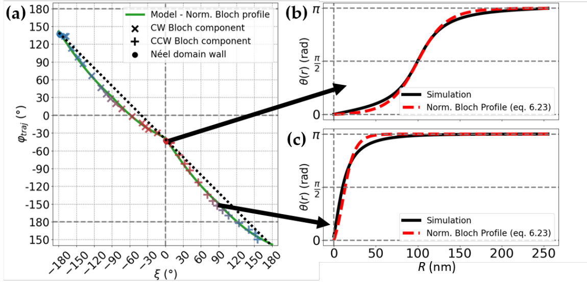
Figure 6.15: Skyrmion trajectory angle versus helicity - comparison model / simulations: (a) Comparison between the simulation data point and the model prediction (green curve) for the adjusted Bloch DW profile from eq. 6.22. (b) (resp. (c)) Comparison of the DW profile extracted from simulations (black curve) and the Bloch profile (dashed red curve) for the data point at \xi \simeq 0 (resp. \xi \simeq \frac{\pi}{2} ). In this case (c), the adjusted Bloch DW profile from eq. 6.23 is convenient for small skyrmion, since it respects \theta(r = 0) = 0 .
