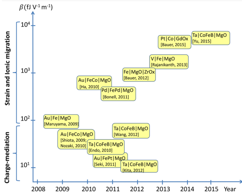
Figure 1.13: Efficiency parameter \beta for the voltage control of magnetic anisotropy : Summary of efficiency parameters value for the electric-field control of magnetic anisotropy at FM/oxide interfaces and in magnetic tunnel junctions. The effect associated to ionic migration (and strain) is larger than the one related to charge effects. (Extracted from [85])
