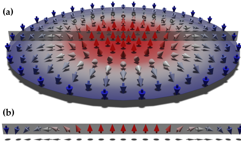
Figure 2.12: The skyrmionic bubble spin texture: (a) Schematic representation of a clockwise Néel skyrmionic bubble, that has to be compared to the corresponding skyrmion from Fig. 2.6a. (b) represents a cut section view of (a) across the skyrmionic bubble diameter. It shows the magnetic domain in the center, surrounded by the CW Néel DW.
