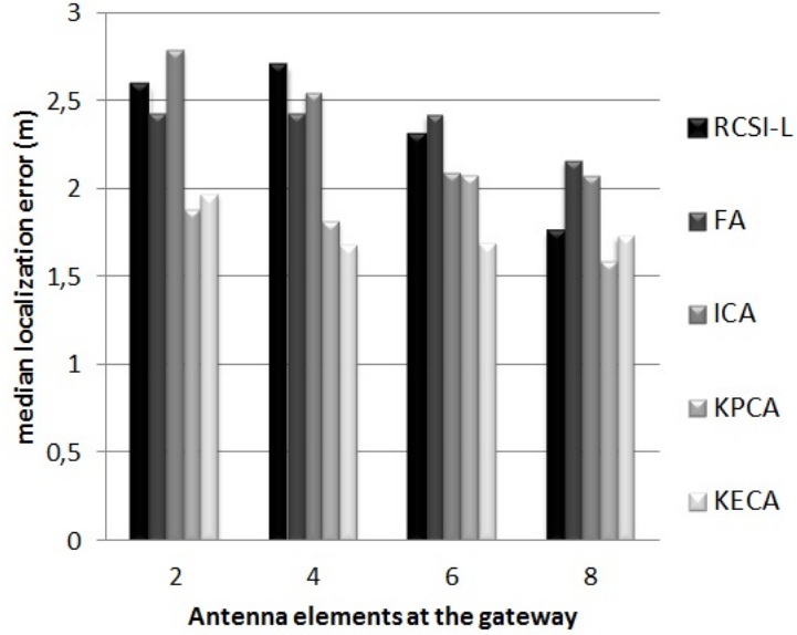
Figure 5.2 – Median localization errors with R = 2, 4, 6, 8 with the training phase in SA scenario and the testing phase in SE scenario.
