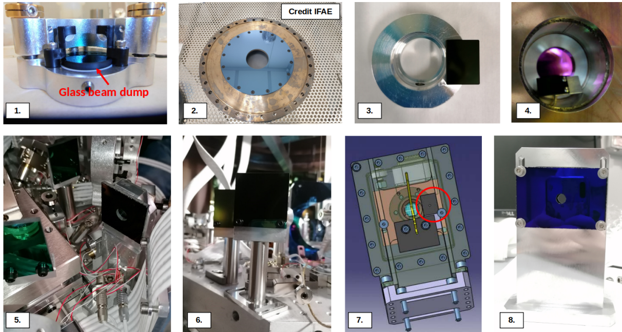
Figure 7.3.: Some of the dumping strategies implemented in AdV+ during the commissioning: (1) absorbing glass behind mirrors, (2) baffles inside tubes, (3) absorbing glass glued on a lens mount, (4) beam dump in front of a viewport, (5) absorbing glass glued on a quadrant and few other beam dumps, (6) small beam dump with black absorbing screws, (7) beam dump glued on the photodiode box, (8) diaphragm.
