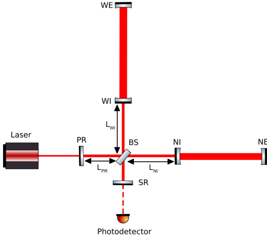
Figure 2.7.: Michelson interferometer with Fabry-Perot cavities along the arms and two additional mirrors: the Power Recycling (PR) and the Signal Recycling (SR). The PR amplifies the light circulating in the interferometer. L_{PR} is the distance between the the PR mirror and the Beam Splitter (BS). L_{NI} and L_{WI} are the distances between the North Input and the West input mirrors from the BS. The SR amplifies the signal arriving at the detection port.
