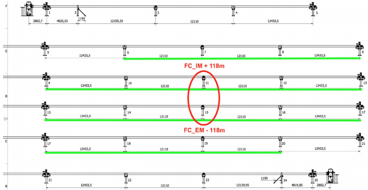
Figure 7.14.: Filter cavity structure with the proposed position for the baffles, placed at z_{IM} + 118 m and z_{EM} - 118 m, in correspondence of the supports 11 and 15 respectively.
