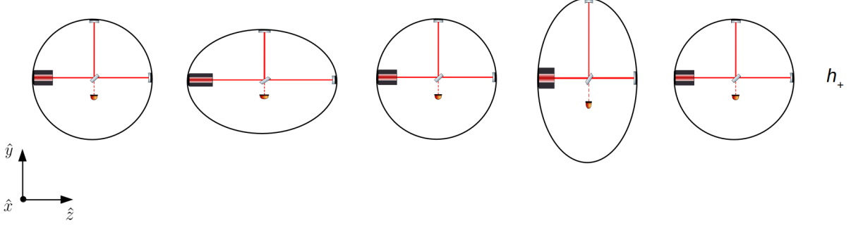
Figure 2.1.: The effect of a passing gravitational wave polarized h_+ which arrives perpendicular to the interferometer plane.
