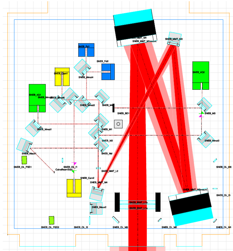
Figure 6.12.: Optocad scheme of SNEB bench. SWEB is similar. The blue boxes represent the photodiodes, the green boxes represent the quadrants and the yellow boxes represent the cameras. The black box near the center of the bench is the Silicon beam dump catching most of the power going to the quadrant. The L1a and L1b lenses are the first elements passed by the beam, at the entrance of the bench.
