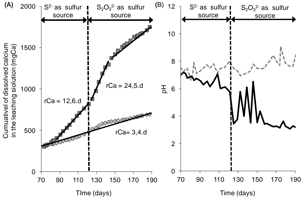
Figure 42: total calcium in the leaching solution for the abiotic pipe reactor and the biotic pipe reactor, with the pH evolution of the leaching solutions. \blacksquare : total calcium in the leaching solution of the biotic pipe reactor (mgCa); \blacklozenge : total calcium in the leaching solution of the biotic pipe reactor (mgCa); \diamond : total calcium in the leaching solution of the abiotic pipe reactor (mgCa); \text{—} : pH of the leaching solution of the biotic pipe reactor; \text{---} : pH of the leaching solution of the abiotic pipe reactor,
