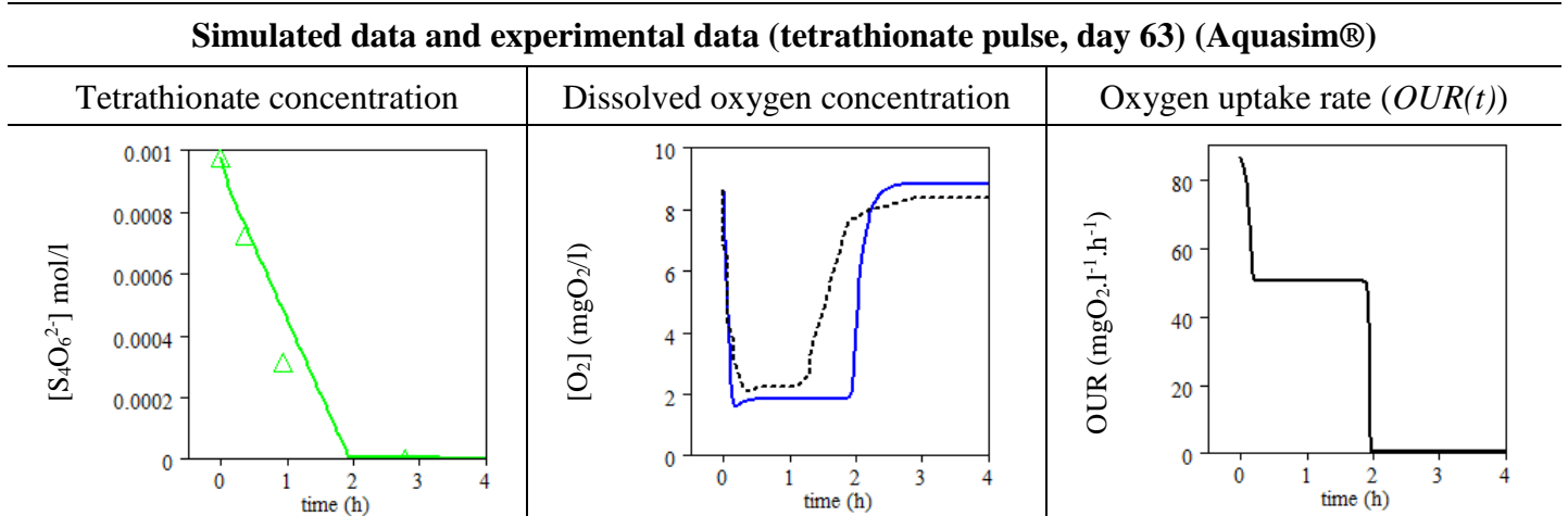
Figure 71: experimental and numerical data for tetrathionate pulse. \Delta : experimental data for tetrathionate concentration (mol/l); \text{—} : numerical data for tetrathionate concentration (mol/l); \text{---} : experimental data for oxygen concentration (mgO 2 /l); \text{—} : numerical data for oxygen concentration (mgO 2 /l); \text{—} : experimental data for OUR(t) (mgO 2 .l -1 .h -1 ); \text{---} : numerical data for OUR(t) (mgO 2 .l -1 .h -1 ).
