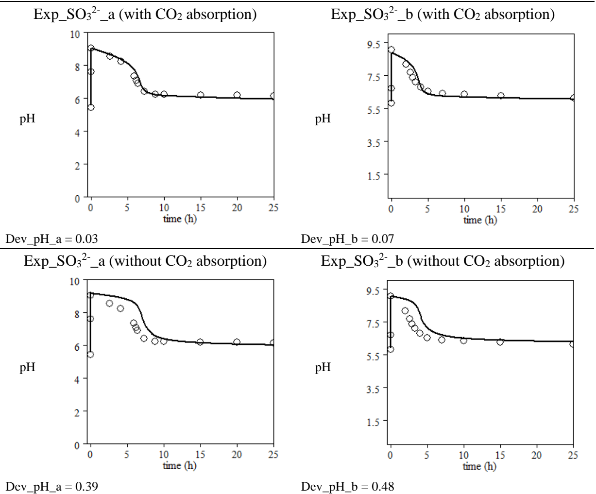
Figure 117: the implication of the carbon dioxide absorption in the definition (Compartement 3) of the sulfite oxidation (Compartement 2a). Comparison in the pH simulation for the experiments Exp_SO 3 2- _a, and Exp_SO 3 2- _b, with and without the simulation of the carbon dioxide absorption. The dissolved oxygen concentration was not modified.
