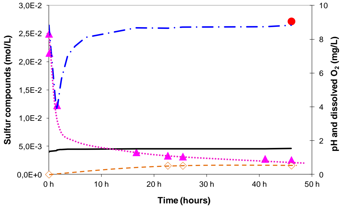
Figure 48: Exp_S 2 O 3 2- _b – time course of the different parameters measured. \blacktriangle : the thiosulfate concentration (S 2 O 3 2- ) (mol/l); \diamond : the sulfate concentration (SO 4 2- ) (mol/l); \bullet : the mass of precipitate expressed as equivalent of loss sulfur (molS/l); -\cdot- : dissolved oxygen concentration (mgO 2 /l); — : pH measurement.
