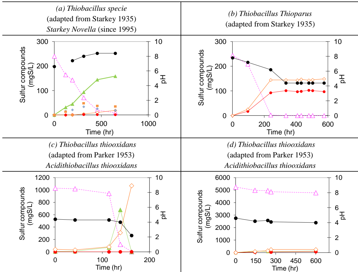
Figure 58: adaptation of results obtained by Starkey in 1935 and Parker 1953 during batch culture of thiobacilli species (neutrophil and acidophil) with thiosulfate as sulfur substrate. \text{---}\triangle\text{---} : thiosulfate concentration [ \text{S}_2\text{O}_3^{2-} ] (mgS/l); \text{---}\diamond\text{---} : S(VI) oxides concentration (mgS/l); \text{---}\triangle\text{---} : tetrathionate concentration [ \text{S}_4\text{O}_6^{2-} ] (mgS/l); \text{---}\square\text{---} : trithionate concentration (mgS/l); \text{---}\diamond\text{---} : pentathionate concentration (mgS/l); \text{---}\bullet\text{---} : pH measurements.
