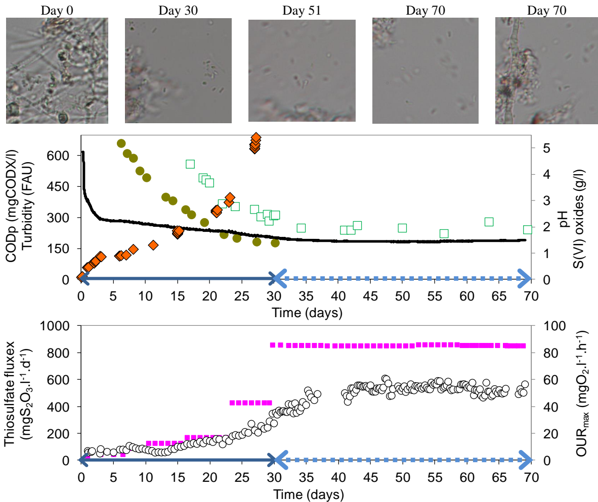
Figure 59: Sequenced-batch culture (inoculated by activated sludge consortium) feeding by thiosulfate as only sulfur substrate. \blacksquare : inlet thiosulfate fluxes ( \text{mgS}_2\text{O}_3 \cdot \text{l}^{-1} \cdot \text{d}^{-1} ); \circ : \text{OUR}_{\text{max}} for each pulse ( \text{mgO}_2 \cdot \text{l}^{-1} \cdot \text{h}^{-1} ); \text{—} : pH measurements; \blacklozenge : S(VI)-oxides (g/l); \square : particulate COD ( \text{mgCOD-X/l} ); \bullet : Turbidity (FAU = OD at 860 nm); \longleftrightarrow : period with HRT = 14.6 d ; \dashrightarrow : period with HRT = 7.3 d.
