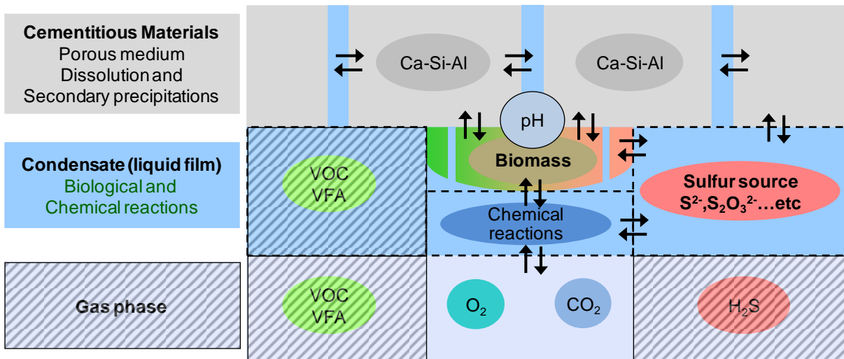
Figure 36: Simplified schema of the biotdeterioration system adapted to study the interaction between sulfur-oxidizing activity and cementitious materials (based on the schema described at figure 17 of the chapter I).
