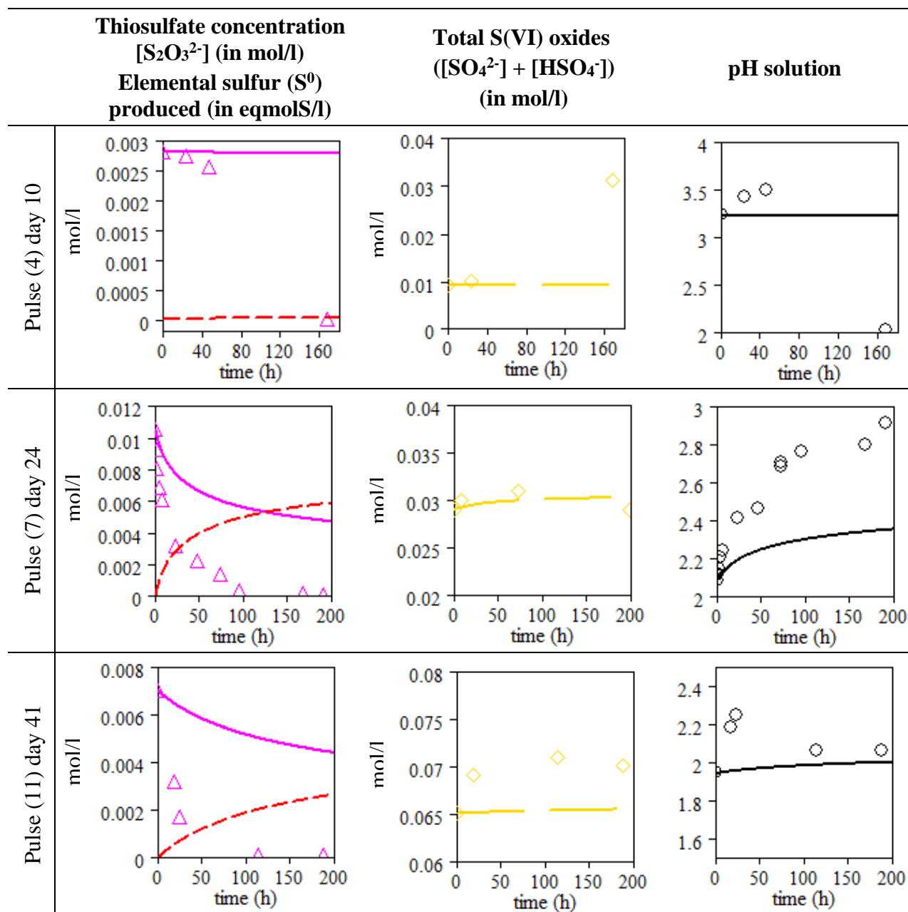
Figure 120: Simulations of thiosulfate pulses (4) (7) (11) by the abiotic model developed in the chapter V of this document. Experimental data: \blacktriangle : thiosulfate concentration [S 2 O 3 2- ] (mol/l); \blacklozenge : S(VI)-oxides (mol/l); \circ : pH measurements. Numerical data: \text{---} : thiosulfate concentration [S 2 O 3 2- ] (mol/l); \text{---} : elemental sulfur produced [S 0 ] (eqmolS/l); \text{---} : S(VI)-oxides concentration (mol/l); \text{---} : solution pH.
