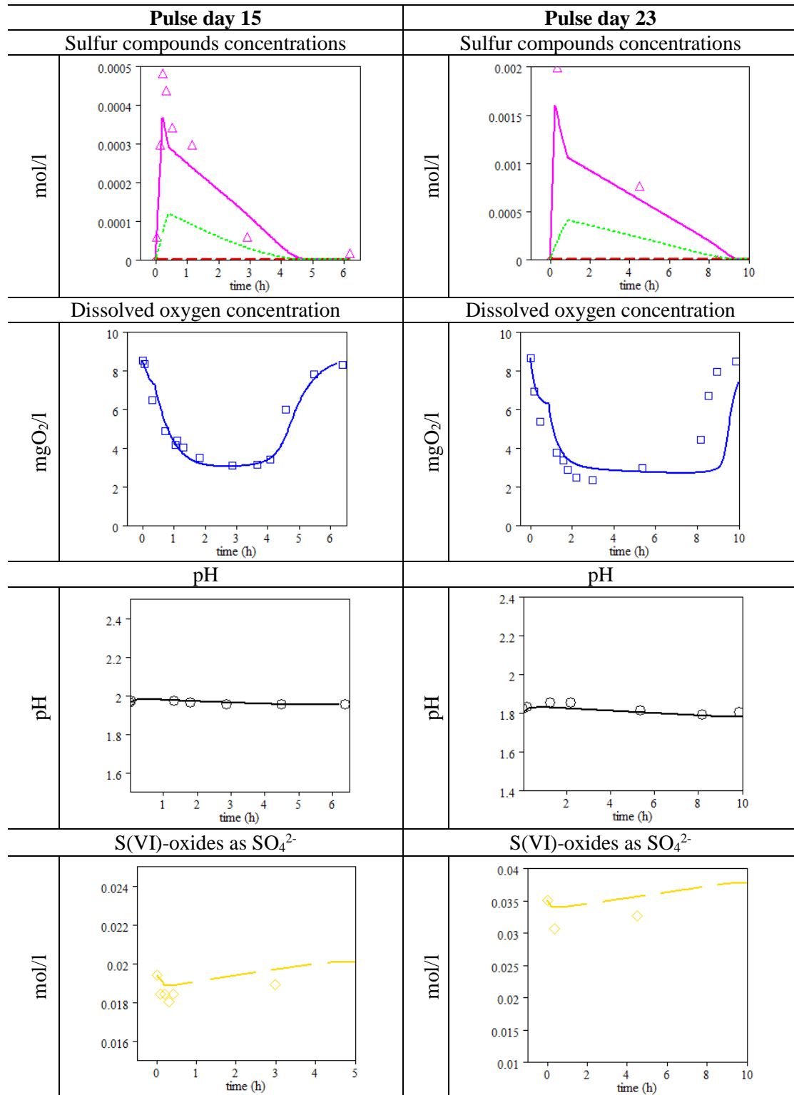
Figure 76: coupled chemical and biological processes experimental and numerical data for two thiosulfate pulses (pulse day 15 and pulse days 23).
