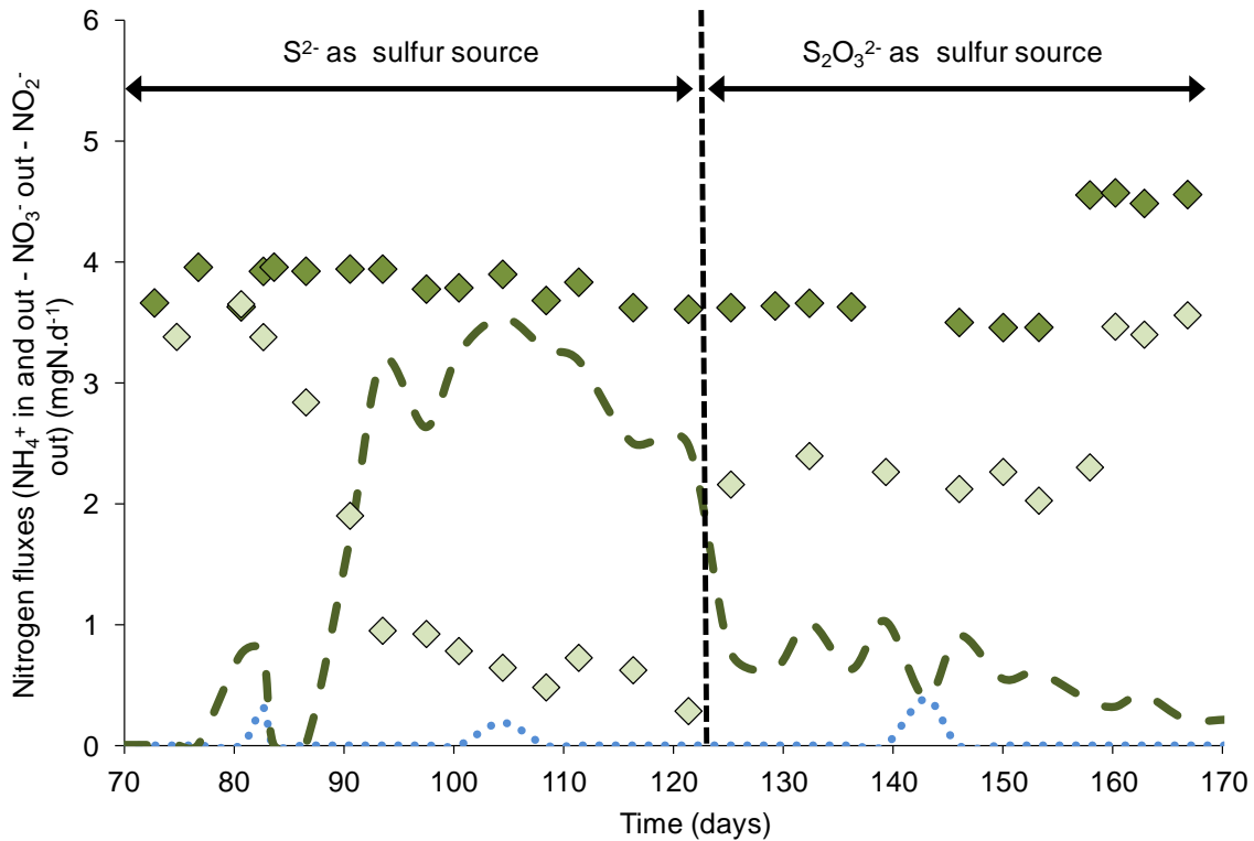
Figure 41: Analyses of nitrogen compounds in the leaching solution for the biotic-pipe reactor. \blacklozenge : ammonium inlet fluxes ( \text{mgN}\cdot\text{d}^{-1} ); \diamond : ammonium outlet fluxes in the leaching solution ( \text{mgN}\cdot\text{d}^{-1} ); -\text{---} : nitrate fluxes produced in the leaching solution ( \text{mgN}\cdot\text{d}^{-1} ); \bullet\bullet\bullet : nitrite fluxes produced in the leaching solution ( \text{mgN}\cdot\text{d}^{-1} ).
