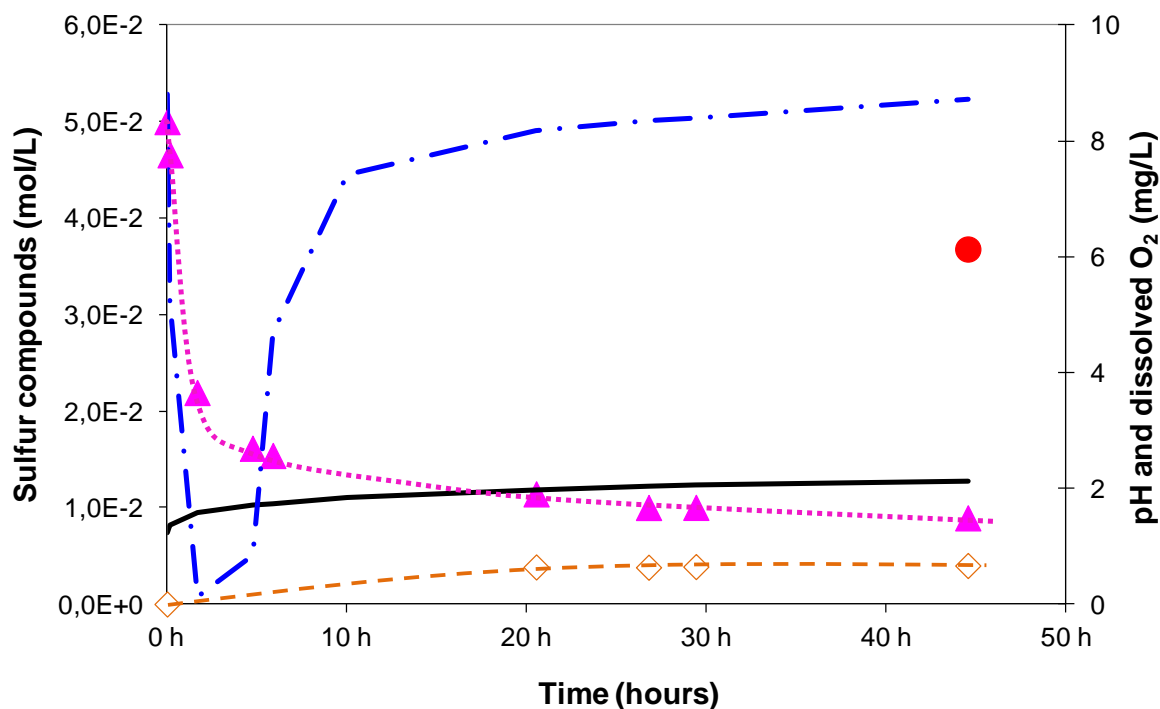
Figure 50: Exp_S 2 O 3 2- _a – time course of the different parameters measured. ..▲.. : the thiosulfate concentration (S 2 O 3 2- ) (mol/l); -◇- : the sulfate concentration (SO 4 2- ) (mol/l); ● : the mass of precipitate expressed as equivalent of loss sulfur (molS/l); -.- : dissolved oxygen concentration (mgO 2 /l); — : pH measurement.
