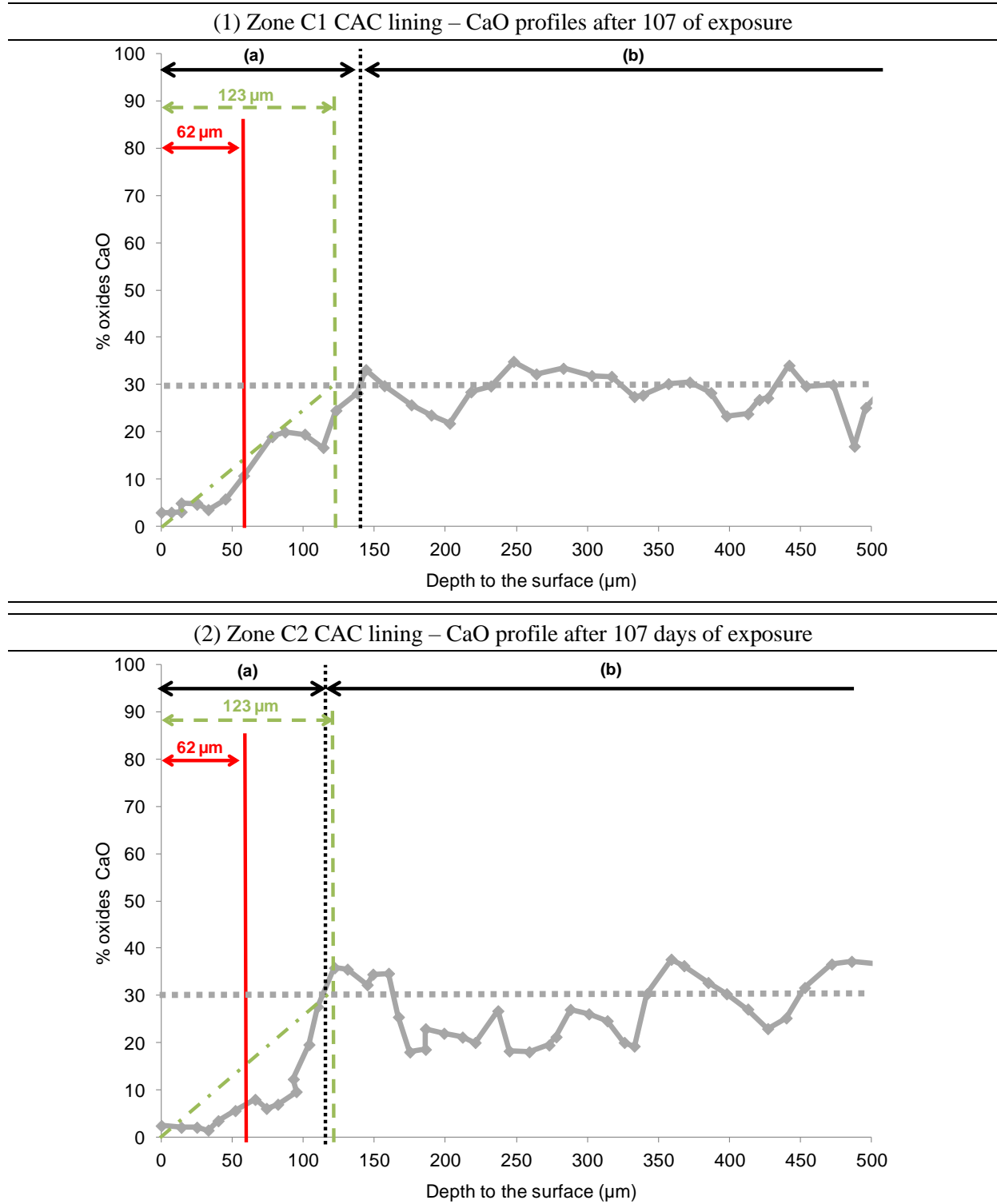
Figure 98: CaO EPMA profiles on zone C1(1) and C2(2) of CAC lining after exposure and calculation of theoretical decalcified depths by the cumul of the calcium in the leaching solution. \blacklozenge : CaO (in %); \bullet\bullet\bullet : mean value of CaO for initial cement paste (in %); \dots\dots : depth of the decalcified zone by comparison of the CaO content of the control specimen and EPMA profiles; \color{red}\rule{0.5pt}{1cm} : calculated depth of decalcified zone for homogenous total decalcification; \color{green}\rule{0.5pt}{1cm} : calculated depth of decalcified zone for homogenous semi-decalcification; \color{green}\rule{0.5pt}{1cm} : theoretical CaO profile for zone with semi-decalcification; (a): decalcified zone; (b) zone of sane paste cement + anhydrous; (c) mortar zone.
