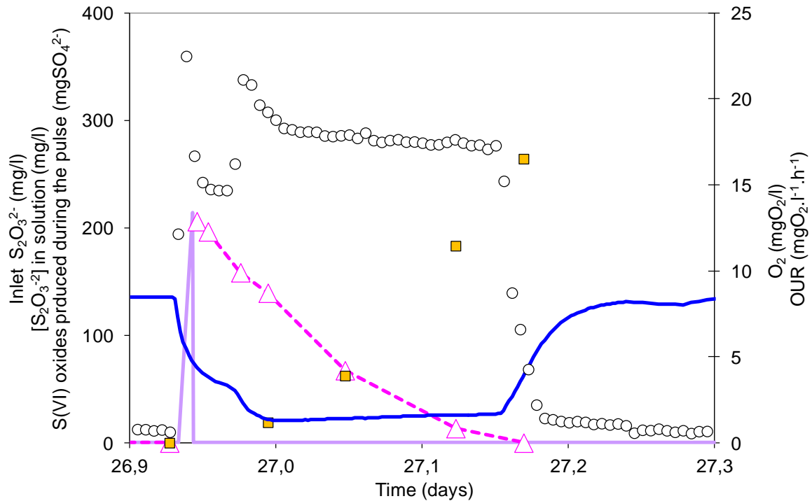
Figure 64: Sequenced-batch culture – HRT = 14.6 days – thiosulfate pulse (214 mgS_2O_3^{2-}/l per pulse). — : thiosulfate pulse; —△— : thiosulfate concentration ( mgS_2O_3/l ); ■ S(VI)-oxides produced during the pulse ( mgSO_4^{2-} ); — : dissolved oxygen concentration ( mgO_2/l ); ○: OUR ( mgO_2 \cdot l^{-1} \cdot h^{-1} ).
