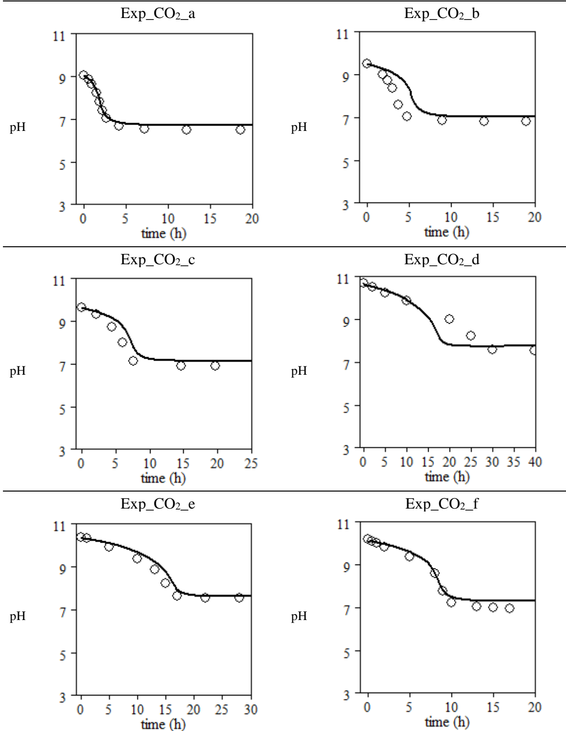
Figure 106: Simulation results for the pH calculation during the carbon dioxide absorption in aqueous solution. The kla_{O_2} was fixed for all the experience ( 0.7 \text{ h}^{-1} ). \circ : the pH values from experimental data; \text{—} : the pH simulation results.
