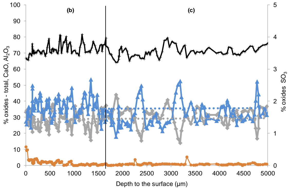
Figure 95: EPMA profiles of cement paste on zone B1 of CAC lining after exposure. + : total oxides (in %); \blacklozenge : CaO (in %); \blacktriangle : Al 2 O 3 (in %); \bullet : SO 3 (in %). \dots : mean value of CaO for initial cement paste (in %); \dots : mean value of Al 2 O 3 for initial cement paste (in %). (b) zone of sane paste cement + anhydrous; (c) mortar zone.
