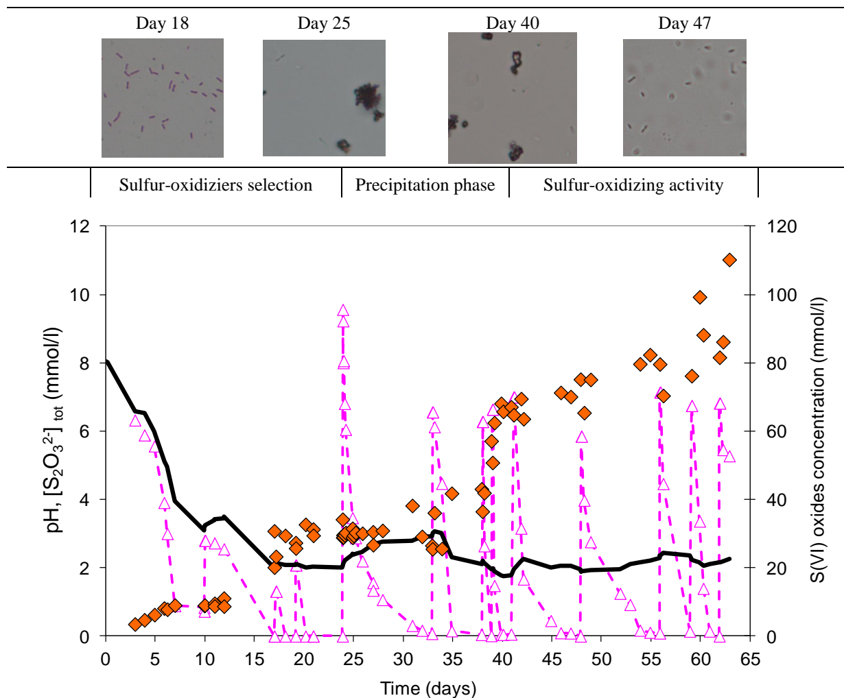
Figure 118: Fed-Batch culture of activated sludge inoculum on thiosulfate as only sulfur substrate (surface aeration). \text{---}\triangle\text{---} : thiosulfate concentration measured [S_2O_3^{2-}] (mmol/l); \text{---}\diamond\text{---} : S(VI) oxides (mol/l) (mmol/l); \text{---} : pH measurements.
