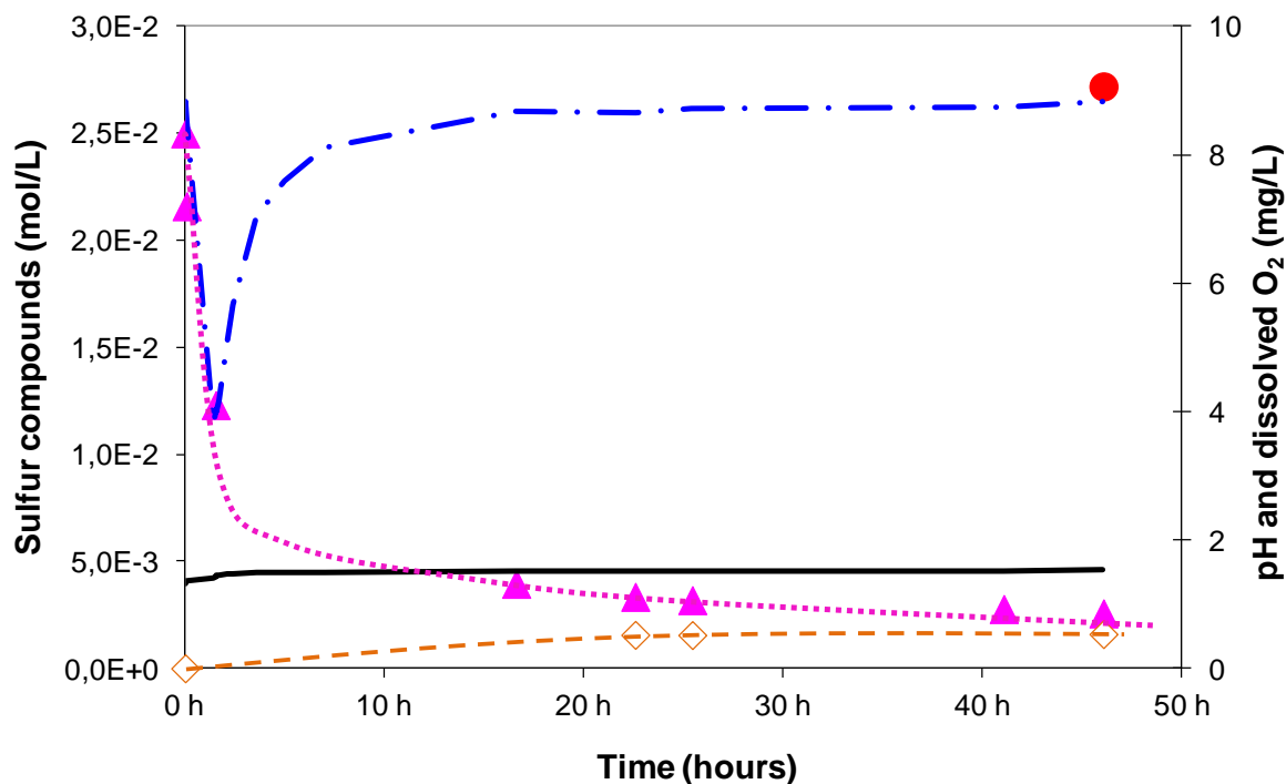
Figure 48: Exp_S 2 O 3 2- _b – time course of the different parameters measured. \dots\blacktriangle\dots : the thiosulfate concentration (S 2 O 3 2- ) (mol/l); \text{---}\blacklozenge\text{---} : the sulfate concentration (SO 4 2- ) (mol/l); \bullet : the mass of precipitate expressed as equivalent of loss sulfur (molS/l); \text{---}\cdot\text{---} : dissolved oxygen concentration (mgO 2 /l); \text{---} : pH measurement.
