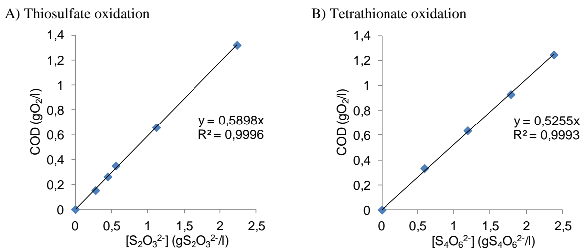
Figure 30: equivalent COD values for the oxidation of thiosulfate (S 2 O 3 2- ) and tetrathionate (S 4 O 6 2- )
