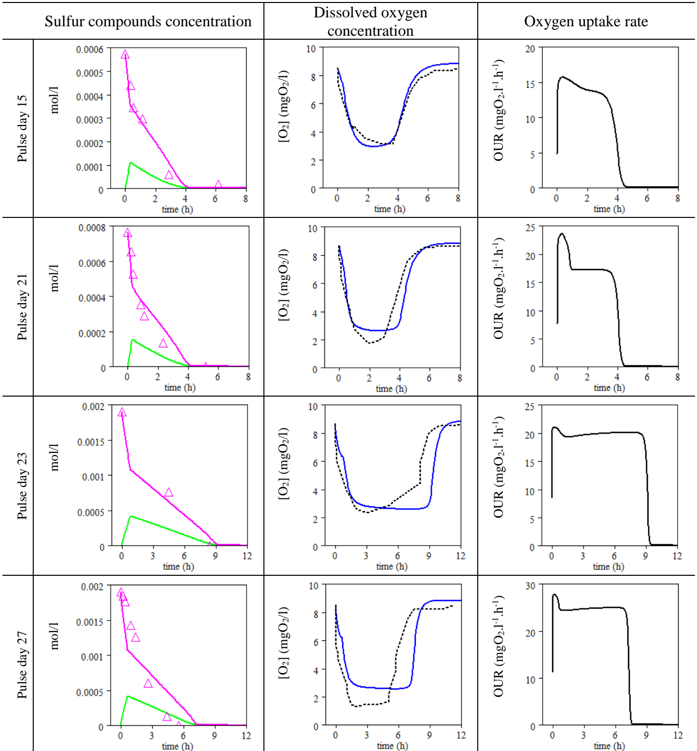
Figure 73: experimental and numerical data for four thiosulfate pulses.
