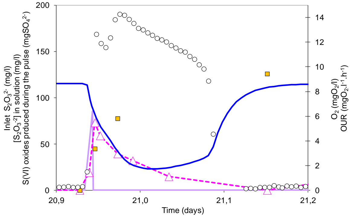
Figure 63: Sequenced-batch culture – HRT = 14.6 days – thiosulfate pulse (86 mgS_2O_3^{2-}/l per pulse). — : thiosulfate pulse; —△— : thiosulfate concentration ( mgS_2O_3/l ); ■ S(VI)-oxides produced during the pulse ( mgSO_4^{2-} ); — : dissolved oxygen concentration ( mgO_2/l ); ○: OUR ( mgO_2 \cdot l^{-1} \cdot h^{-1} ).
