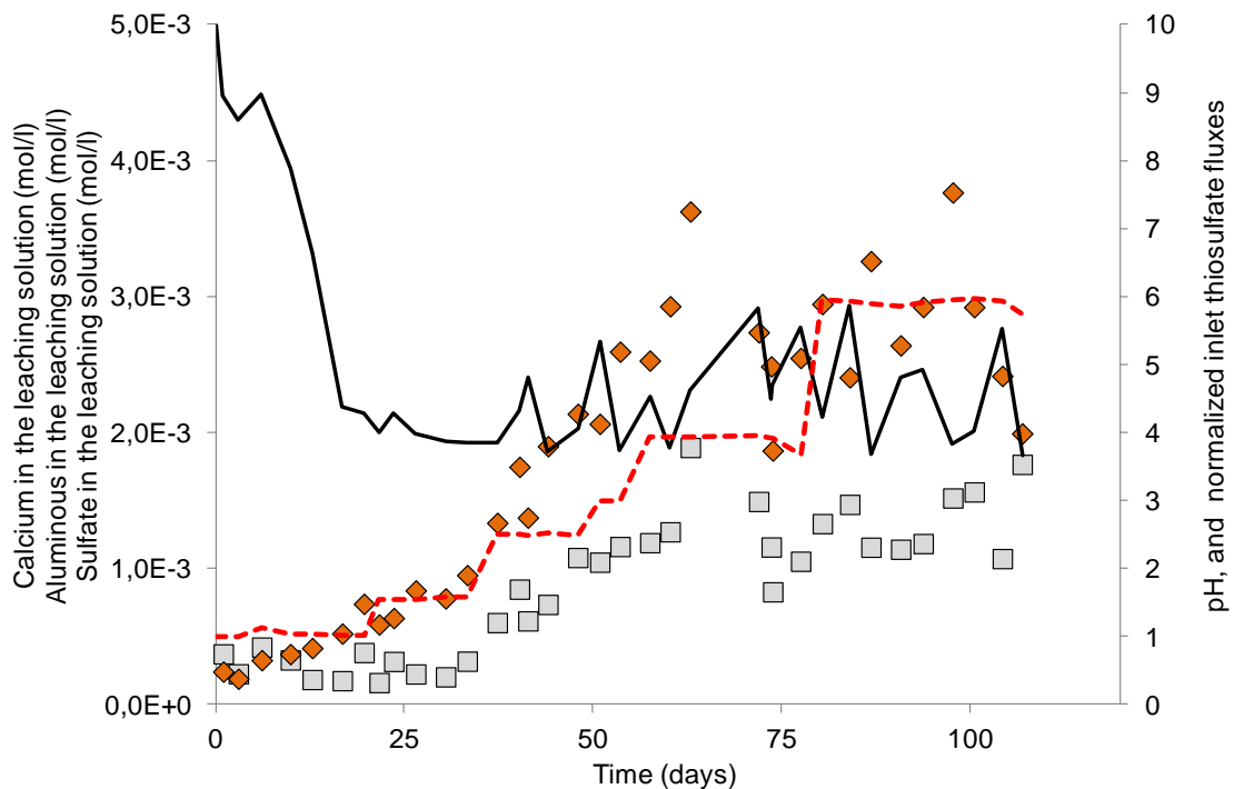
Figure 86: (a) for CAC lining, (b) for BFSC. — : pH of the leaching solution; \blacklozenge : sulfate concentration in the leaching solution (mol/l); \blacksquare : calcium concentration in the leaching solution (mol/l); \blacktriangle : alumina concentration in the leaching solution (mol/l); - - - : normalized thiosulfate inlet fluxes.
