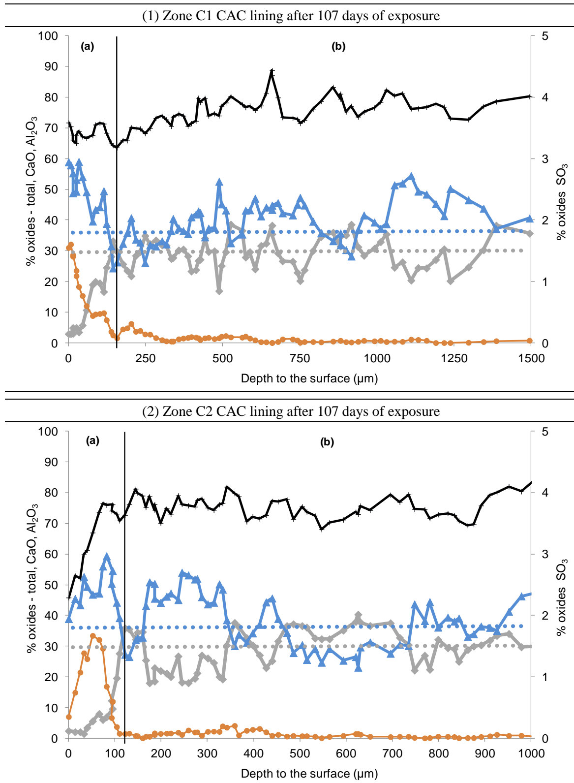
Figure 96: EPMA profiles of cement paste on zone C1(1) and C2(2) of CAC lining after exposure. + : total oxides (in %); ♦ : CaO (in %); ▲ : Al 2 O 3 (in %); ● : SO 3 (in %); ..... : mean value of CaO for initial cement paste (in %); ..... : mean value of Al 2 O 3 for initial cement paste (in %). (a): decalcified zone; (b) zone of sane paste cement + anhydrous; (c) mortar zone.
