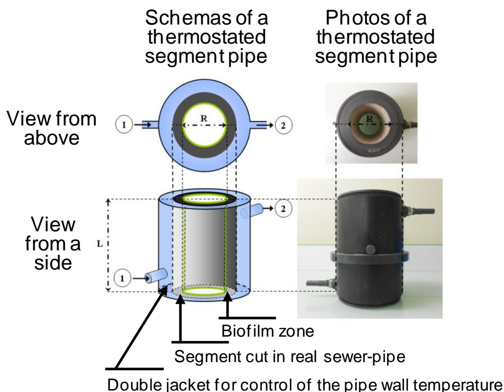
Figure 28: schema and photos of the segment-pipe (D = 80 mm and L = 200 mm) with his double jacket of PVC for the control of the temperature applied at the pipe-wall.
