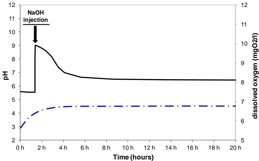
Figure 105: Exp_CO 2 _a – time course of the different parameters measured. — . — : dissolved oxygen concentration (mgO 2 /l); — : pH measurement.
