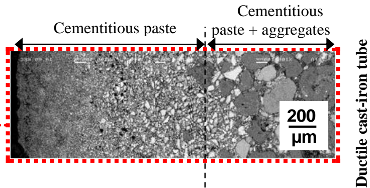
B) Cementitious lining section observed by SEM
