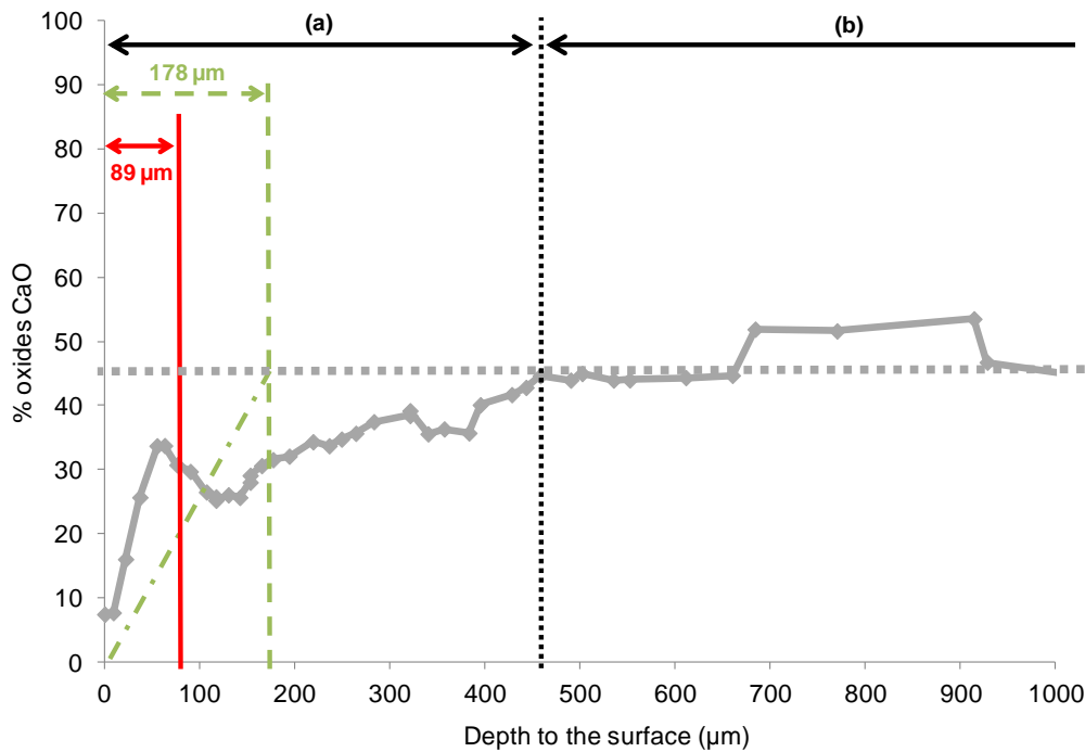
Figure 99: CaO EPMA profiles on zone D2 of BFSC lining after exposure and calculation of theoretical decalcified depths by the cumulated calcium in the leaching solution. \blacklozenge : CaO (in %); \bullet\bullet\bullet : mean value of CaO for initial cement paste (in %); \bullet\bullet\bullet\bullet : depth of the decalcified zone by comparison of the CaO content of the control specimen and EPMA profile; \color{red}\rule{0.5pt}{1cm} : calculated depth of decalcified zone for homogenous total decalcification; \color{green}\rule{0.5pt}{1cm} : calculated depth of decalcified zone for homogenous semi-decalcification; \color{green}\rule{0.5pt}{1cm} : theoretical CaO profile for zone with semi-decalcification; (a): decalcified zone; (b) zone of sane paste cement + anhydrous; (c) mortar zone.
