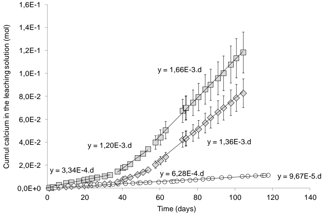
Figure 87: total calcium in the leaching solution during the experiments with inoculated CAC and BFSC lining, and with abiotic CAC lining. \blacklozenge : total calcium in the leaching solution for inoculated CAC lining (mol); \blacksquare : cumul of calcium in the leaching solution for inoculated BFSC lining (mol); \circ : total calcium in the leaching solution for abiotic CAC lining (mol).
