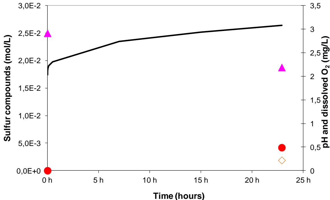
Figure 49: Exp_S 2 O 3 2- _d – time course of the different parameters measured. \blacktriangle : the thiosulfate concentration (S 2 O 3 2- ) (mol/l); \blacklozenge : the sulfate concentration (SO 4 2- ) (mol/l); \bullet : the mass of precipitate expressed as equivalent of loss sulfur (molS/l); \text{---} : pH measurement..
