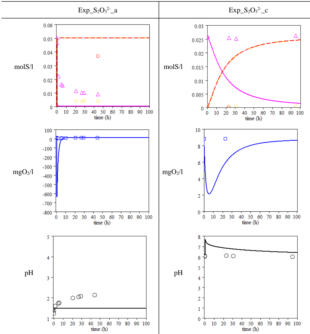
Figure 53: Simulation results with Johnston and Connick kinetic definition (Exp_S 2 O 3 2- _a and – Exp_S 2 O 3 2- _c). Experimental data: \triangle : the thiosulfate concentration (S 2 O 3 2- ) (mol/l); \diamond : the sulfate concentration (SO 4 2- ) (mol/l); \circ : the mass of precipitate expressed as equivalent of loss sulfur (molS/l); \square : the dissolved oxygen concentration; \circ : the pH. Numerical data: \text{—} (magenta): the thiosulfate concentration (S 2 O 3 2- ) (mol/l); \text{—} (yellow): the sulfate concentration (SO 4 2- ) (mol/l); \text{-- --} (red): the colloidal sulfur (eqmolS/l); \text{—} (blue): dissolved oxygen concentration (mgO 2 /l); \text{—} (black): pH measurement.
