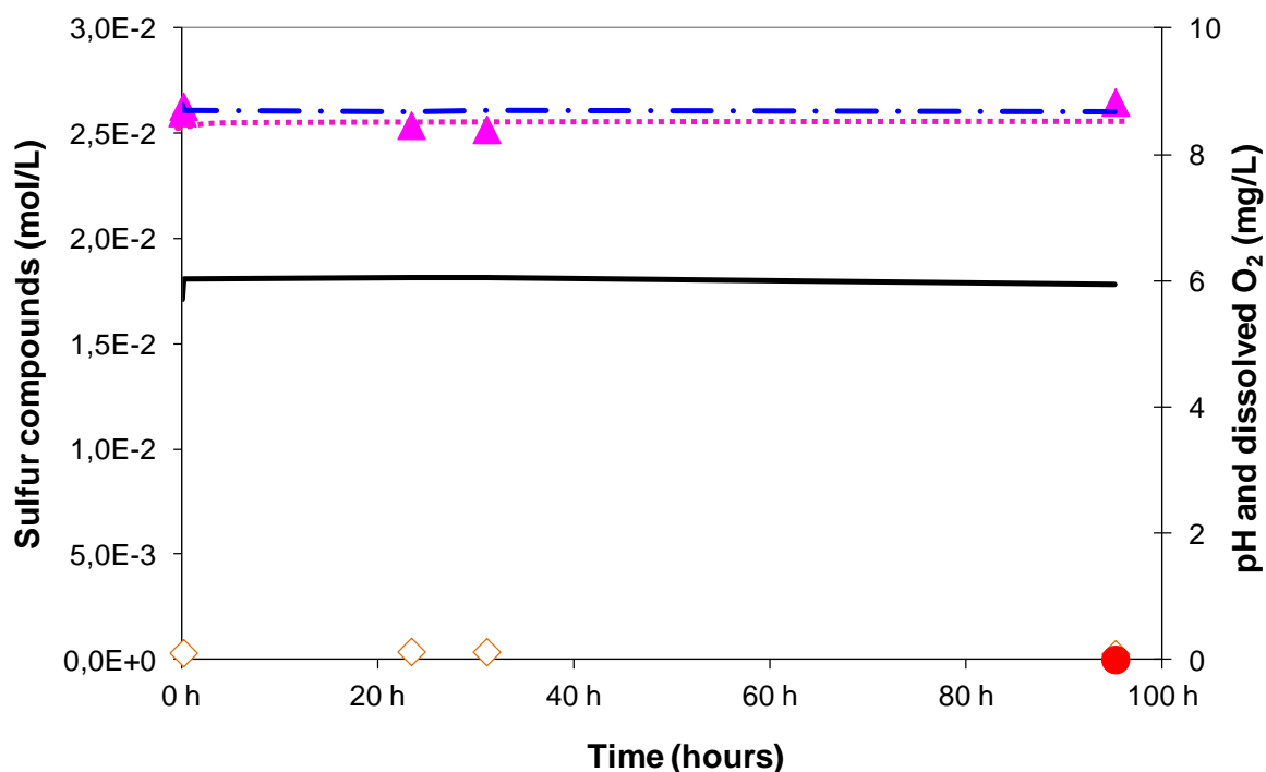
Figure 47: Exp_S 2 O 3 2- _c – time course of the different parameters measured. \dots \blacktriangle \dots : the thiosulfate concentration (S 2 O 3 2- ) (mol/l); \diamond : the sulfate concentration (SO 4 2- ) (mol/l); \bullet : the mass of precipitate expressed as equivalent of loss sulfur (molS/l); -\cdot-\cdot- : dissolved oxygen concentration (mgO 2 /l); — : pH measurement.
