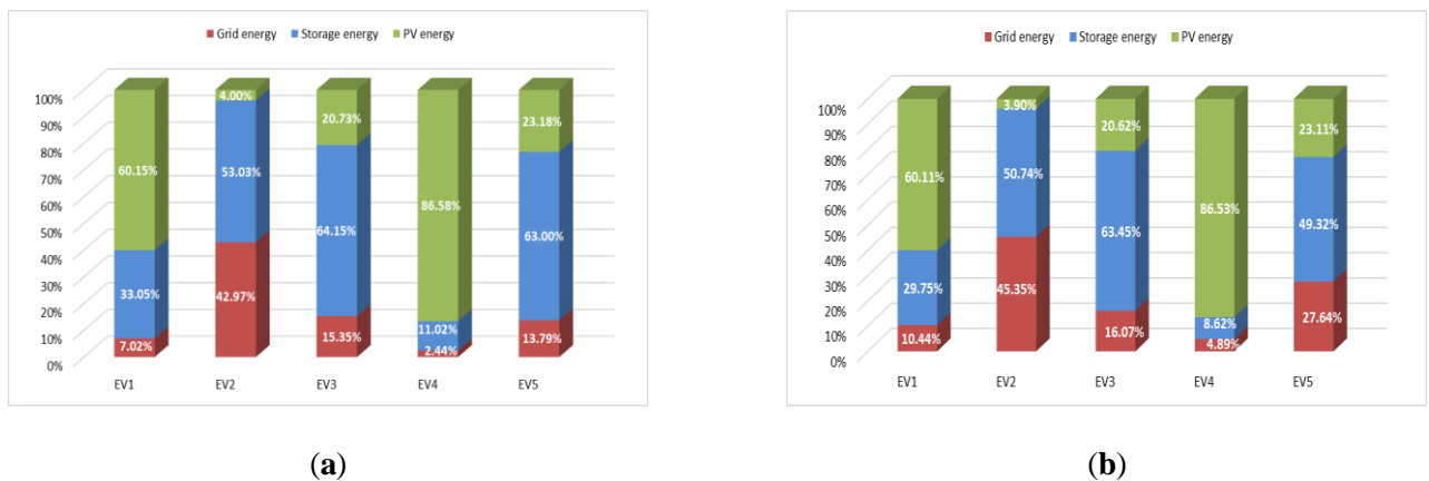
Figure 94: EV energy distribution for “real-time exp” (a) without opt and (b) with opt—experimental test 5.
