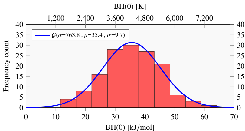
Figure 2. BSSE corrected BH(0) distribution at DLPNO-CCSD(T) level. Structures and ZPEs are calculated at the ONIOM(B97-3c:xTB-GFN2) level. The solid blue curve is the \mathcal{G}(\text{hist}(\text{BH}(0)), \alpha, \mu, \sigma) unnormalized Gaussian best fit function for the histogram (see Eq. 6).
