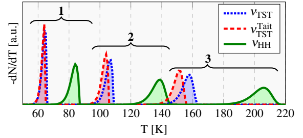
(c) Methanol
