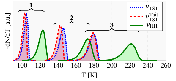
(a) Water
