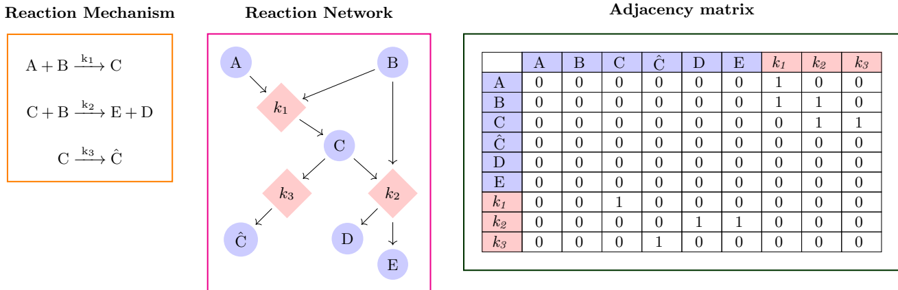
Figure 1. Three different ways to visualize and work with a reaction network: reactions list ( left panel ), colored directed graph (or colored di-graph), where circles correspond to chemical species, while squares indicate rate constants ( middle panel ), and non symmetric adjacency (or connectivity) matrix representation of the colored di-graph ( right panel ).
