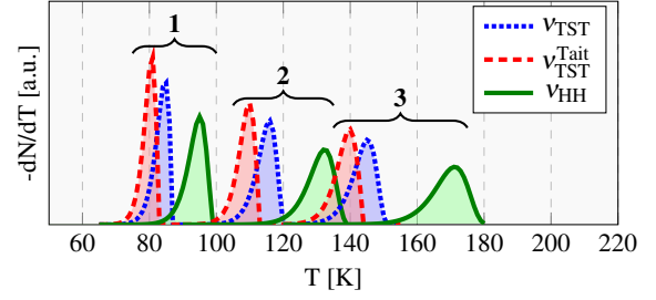
(b) Ammonia
