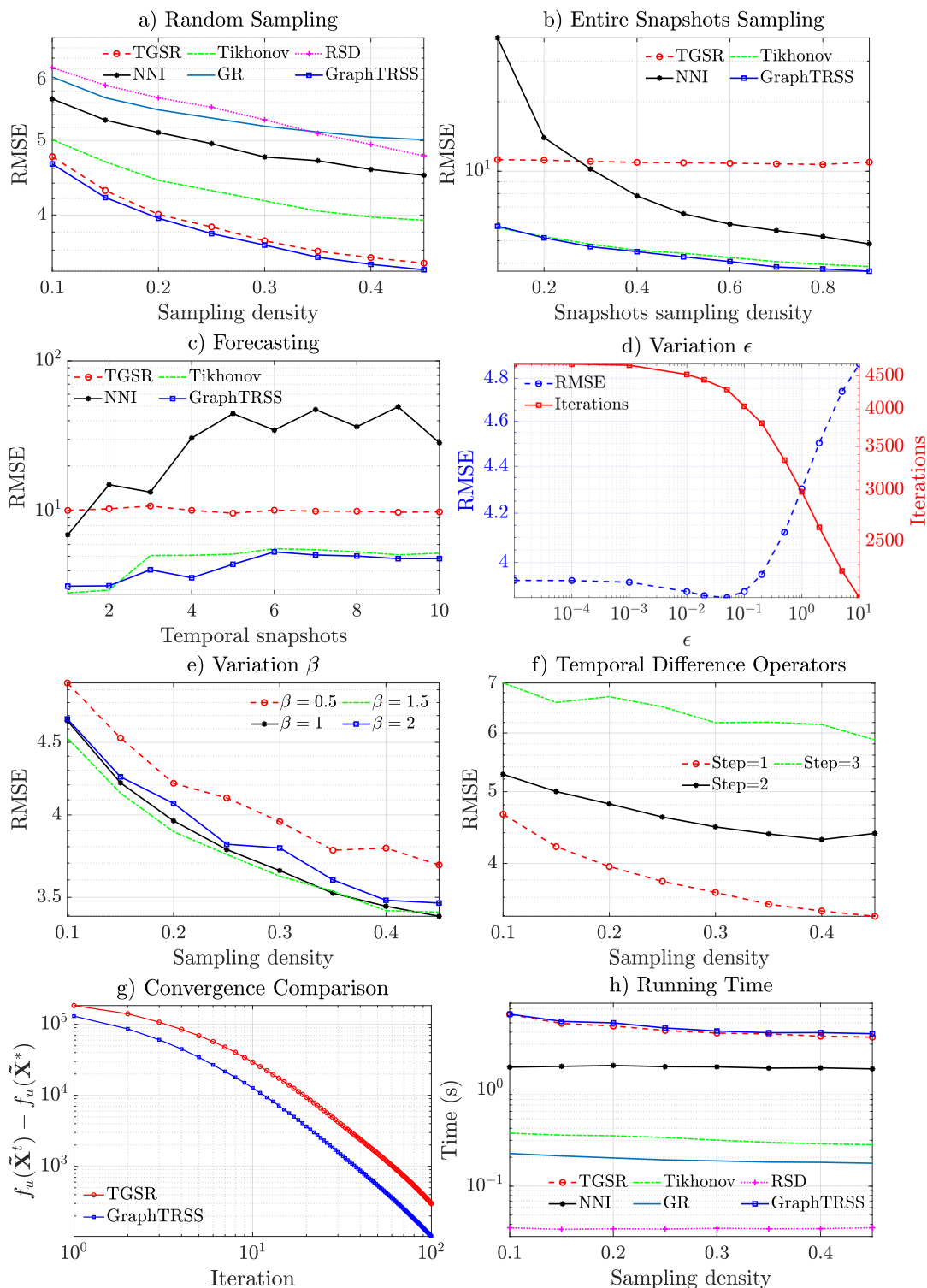
Figure 8-10: Comparison of GraphTRSS with several methods in the literature in the PM 2.5 dataset for several experiments in terms: a) random sampling, b) entire snapshots sampling, c) forecasting, d) variation of parameter \epsilon , e) variation of parameter \beta , f) several temporal difference operators, g) convergence comparison, and h) running time.
