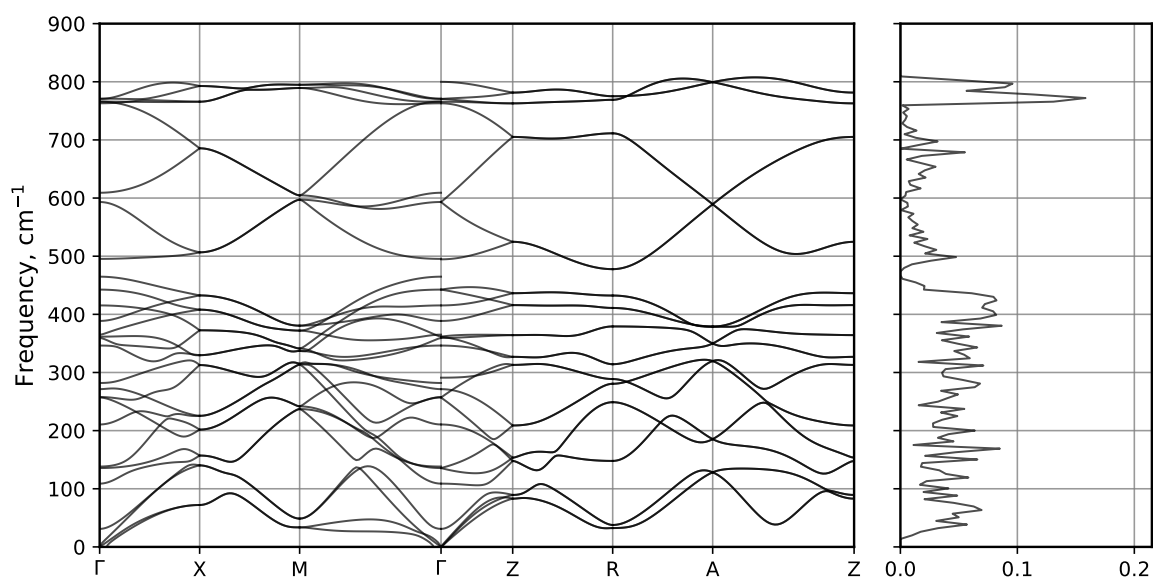
(b) Crystobalite \alpha -SiO 2
