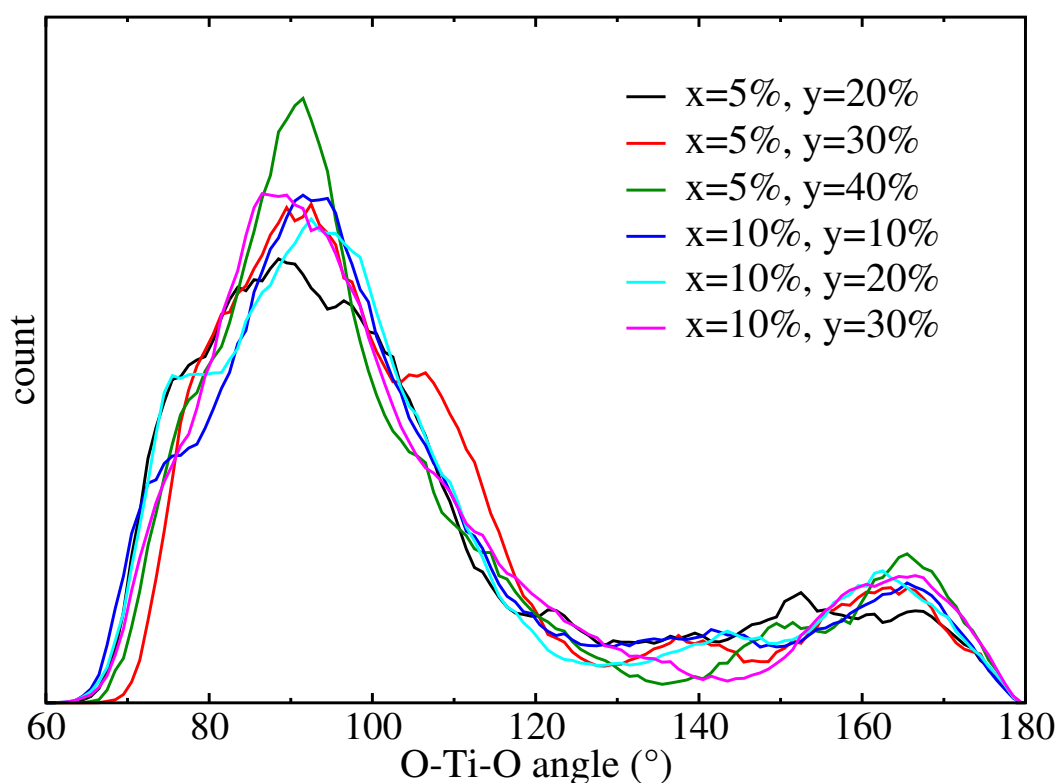
Figure 5.14: Angles O-Ti-O in (\text{TiO}_2)_x - (\text{TlO}_{0.5})_y - (\text{TeO}_2)_{1-x-y}
