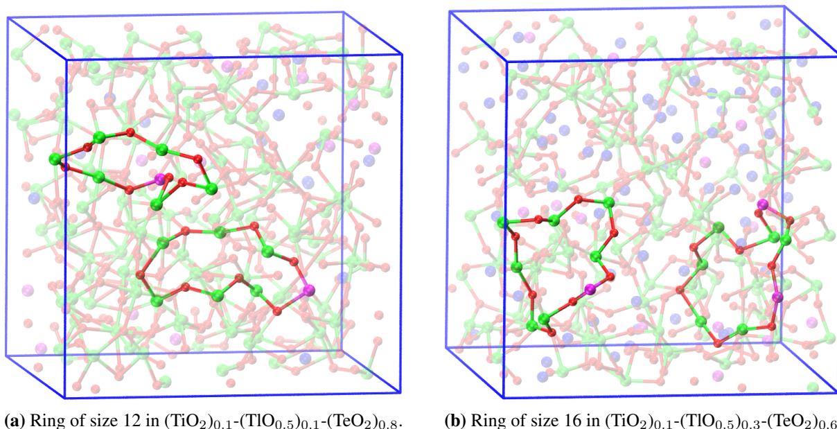
Figure 5.18: Visualization of n -size rings in (\text{TiO}_2)_x - (\text{TlO}_{0.5})_y - (\text{TeO}_2)_{1-x-y} ternary glass. Red sphere: Oxygen, Magenta sphere: Titanium, Green sphere: Tellurium, Blue sphere: Thallium
