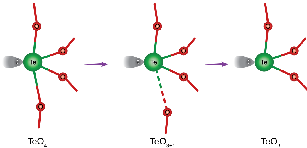
Figure 1.11: Depolymerization of TeO 4 unit into TeO 3 unit via TeO 3+1 (1 long and 3 short bonds).
