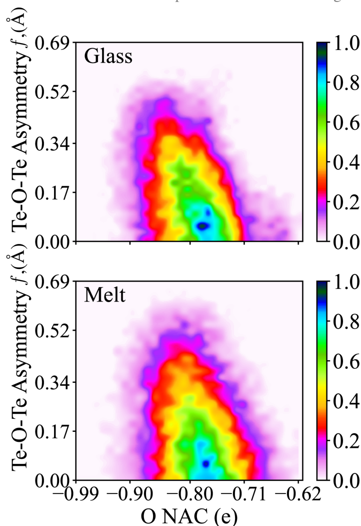
Figure 3.14: 2-D Histogram distribution of 2-fold bridging oxygen (Te-O-Te) asymmetry vs the NACs f for glassy and melt phases of \text{TeO}_2 system.
