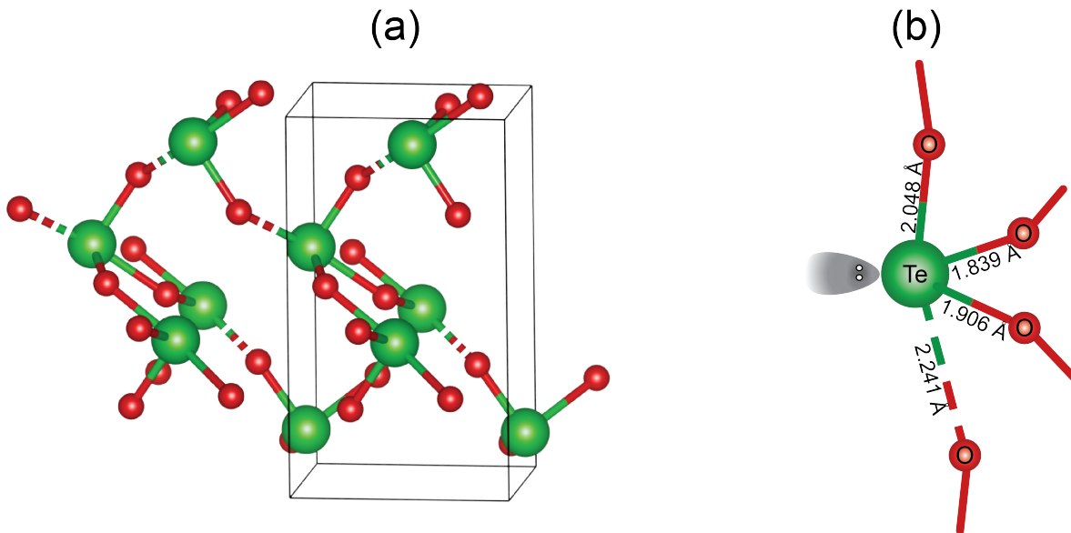
Figure 1.5: (a) Three dimensional lattice of \gamma -TeO 2 and (b) representation of the basic TeO 3+1 structural unit. Bond length are in \text{\AA} .
