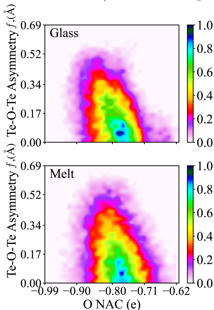
Figure 3.14: 2-D Histogram distribution of 2-fold bridging oxygen (Te-O-Te) asymmetry vs the NACs f for glassy and melt phases of TeO 2 system.
