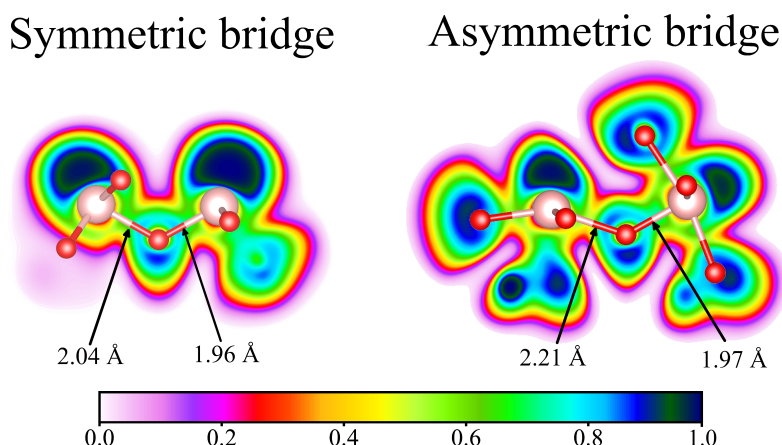
Figure 3.15: ELF was calculated for symmetric and asymmetric bridges in representative \text{TeO}_2 network glass fragments on the Te-O-Te plane. The ELF map is overlaid with the atomic structure of each component. Above the Te-O-Te plane, only Te (brown) and O (red) are depicted. For the sake of clarity, H atoms were employed but not shown to passivate O atoms.
