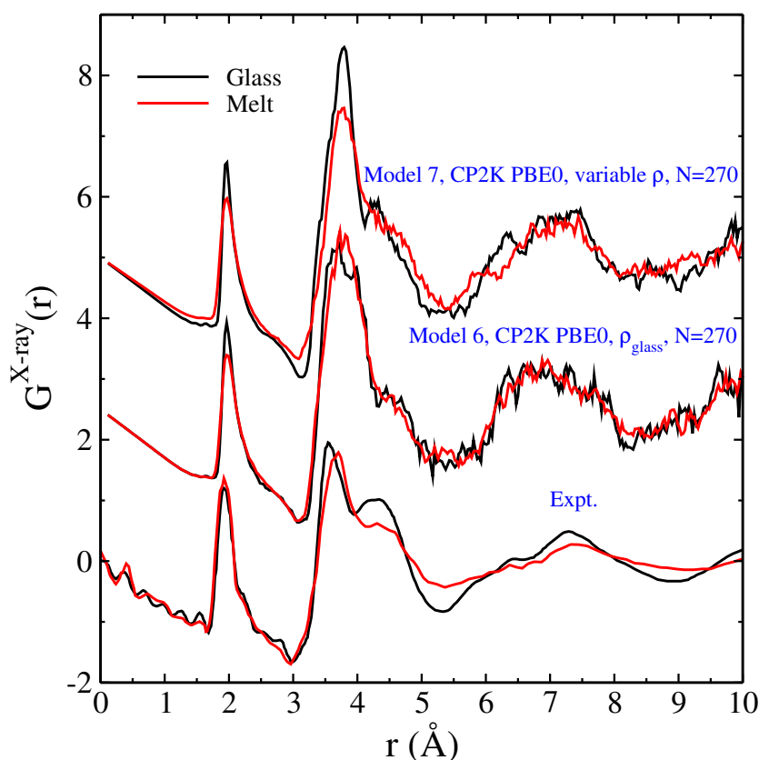
Figure 3.2: Comparison of total X-ray PDF for amorphous (black lines) and melt (red lines) phases of \text{TeO}_2 systems obtained from Model 6 and 7 to experimental results [38]. The curves are shifted vertically for better clarity.
