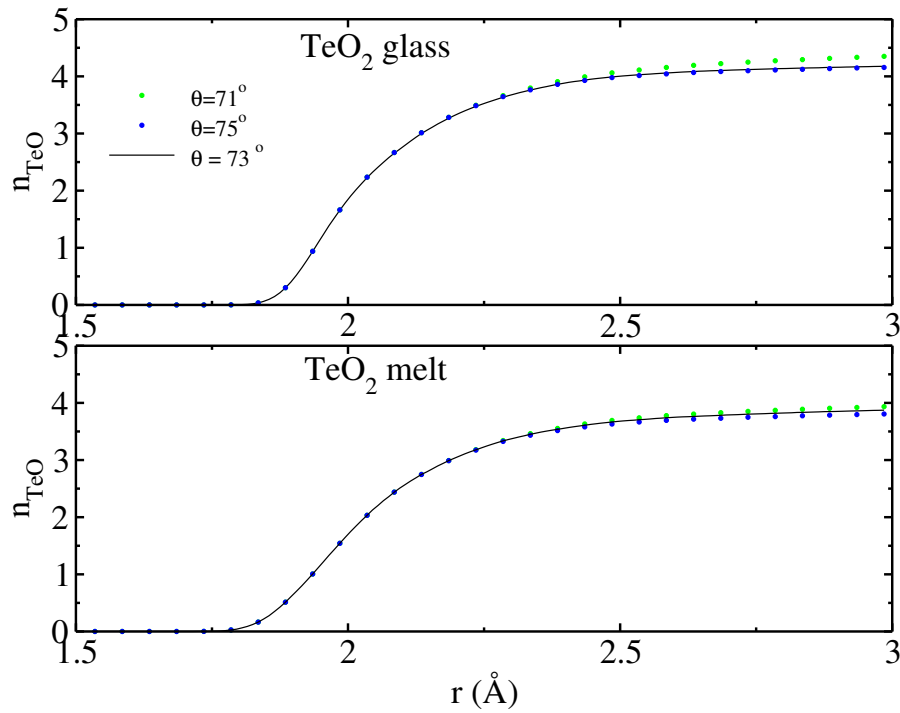
Figure 3.9: Running Te-O coordination number ( n_{\text{TeO}} ) of glassy (top panel) and melt (bottom panel) \text{TeO}_2 . Results obtained based on Wannier centers with variable angular constraint thresholds.
