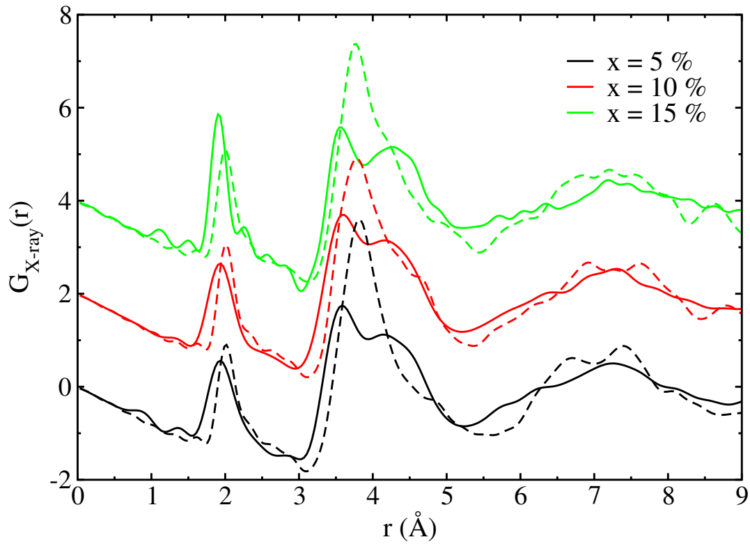
Figure A.10: Comparison of total X-ray scattering PDF G(r) between experiments (solid lines) [113] and ab-initio MD simulation (dashed lines) for (\text{TiO}_2)_x - (\text{TeO}_2)_{1-x} binary glassy system with various concentrations ( x ). A shift of 2 units in the y-axis is given to various concentrations for better clarity of the graph.
