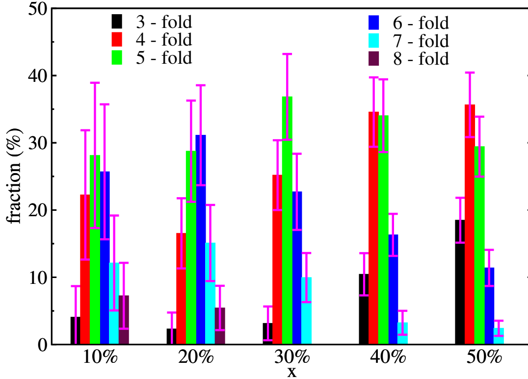
Figure 4.16: Percentage of l -fold coordinated Ti atoms in all the considered composition of (\text{TiO}_{0.5})_x - (\text{TeO}_2)_{1-x} binary glasses. Further, values less than 2% are ignored.
