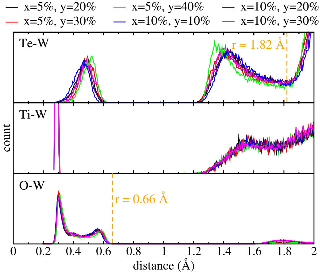
Figure 5.7: Histogram distribution of Te-W (top panel), Ti-W (middle panel) and O-W (bottom panel) pair distances (\text{TiO}_2)_x - (\text{TiO}_{0.5})_y - (\text{TeO}_2)_{1-x-y} .
