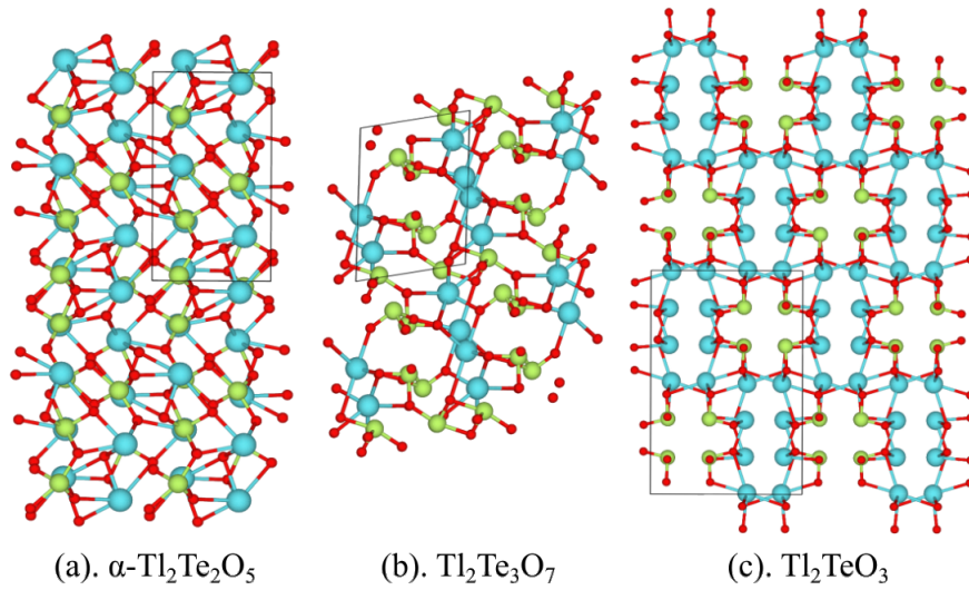
Figure A.2: Three crystalline thallium tellurite crystal structures used in the fit of IAP. (a) \alpha - \text{Tl}_2\text{Te}_2\text{O}_5 : space group - \text{P2}_1/\text{n} , (b) \text{Tl}_2\text{Te}_3\text{O}_7 : space group - \text{P1} , (c) \text{Tl}_2\text{TeO}_3 : space group - \text{Pbn} . Color code: oxygen (red), tellurium (green) and thallium (cyan).
