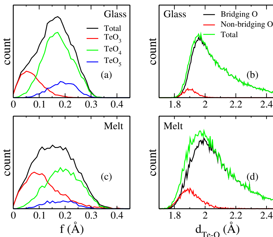
Figure 3.11: Distribution of the average bond asymmetry function calculated on amorphous (a) and melt (c) \text{TeO}_2 system and its breakdown into contributions from \text{TeO}_n units ( n=3,4 and 5). Distribution of Te-O distances calculated on glass (b) and melt (d) \text{TeO}_2 where O atoms are either bridging or non-bridging.
