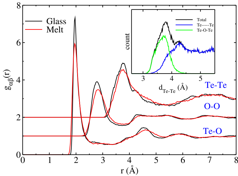
Figure 3.4: The partial distribution functions of g_{\text{TeTe}}(r) , g_{\text{TeO}}(r) , and g_{\text{OO}}(r) for glass (black lines) and melt (red lines) \text{TeO}_2 . In the inset, the Te-Te distance distribution is decomposed into contributions from Te atoms linked by bridging O (green hue) and contributions from nearby Te atoms not directly sharing any O (blue color). Various pair distributions are shifted vertically to depict a clear representation.
