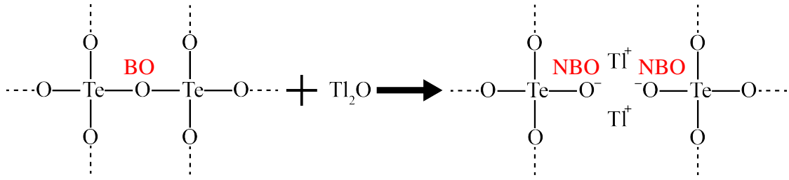
Figure 4.11: Structural depolymerization of Te-O-Te bridge by addition of \text{Tl}_2\text{O} modifier. Text in the red categorizes oxygen atom into bridging oxygen (BO) or non-bridging oxygen (NBO).
