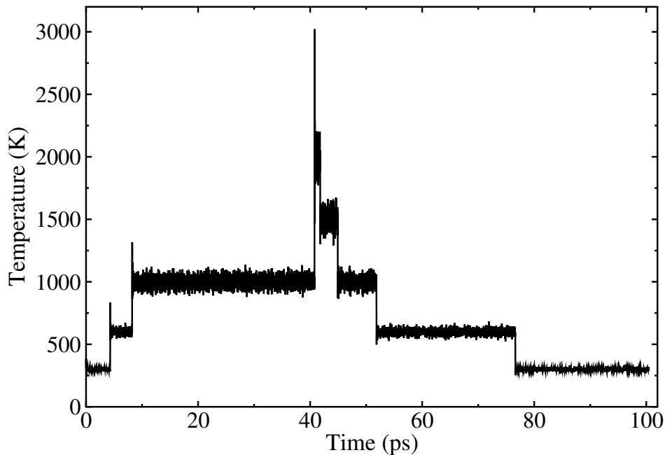
Figure A.9: Thermal cycle for x = 5\% in (\text{TiO}_2)_x - (\text{TeO}_2)_{1-x} binary glass.
