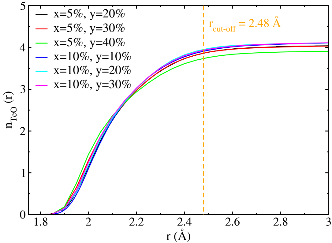
Figure 5.8: For all the compositions in the (\text{TiO}_2)_x - (\text{TiO}_{0.5})_y - (\text{TeO}_2)_{1-x-y} ternary glasses taken into consideration, the running coordination number ( n_{\text{Te-O}} ) using MLWF formalism as a function of TeO pair distance.
