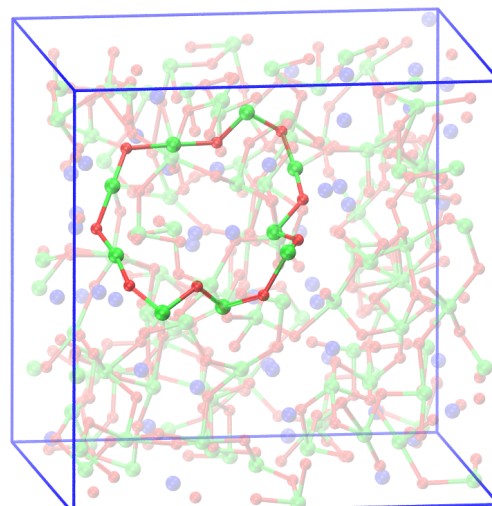
(b) Ring of size 18 in 30%- \text{TlO}_{0.5} -70% \text{TeO}_2 .
