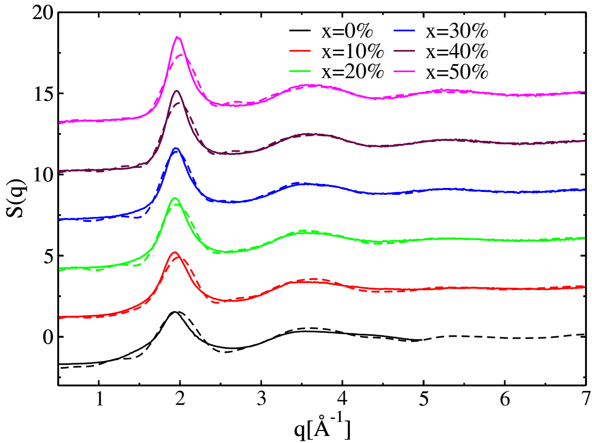
Figure 4.2: Comparison of total X-ray structure factor computed (dashed lines) for various (\text{TiO}_{0.5})_x - (\text{TeO}_2)_{1-x} binary glasses with experimental data (solid lines) [113]. Experimental and simulated data for x = 0\% are taken from Alderman et. al. [38] and calculated from PBE0 hybrid XC functional (see chapter [3])
