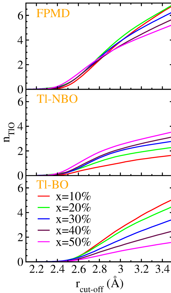
Figure 4.14: Running coordination of considered binary glasses. Top panel represents the coordination number n_{\text{Tl-O}} as a function of distance obtained using integration of partial Tl-O PDF. Middle panel represents running n_{\text{Tl-NBO}} with respect to non-bridging oxygen (NBO). Bottom panel shows running n_{\text{Tl-BO}} with respect to bridging oxygen (BO).
