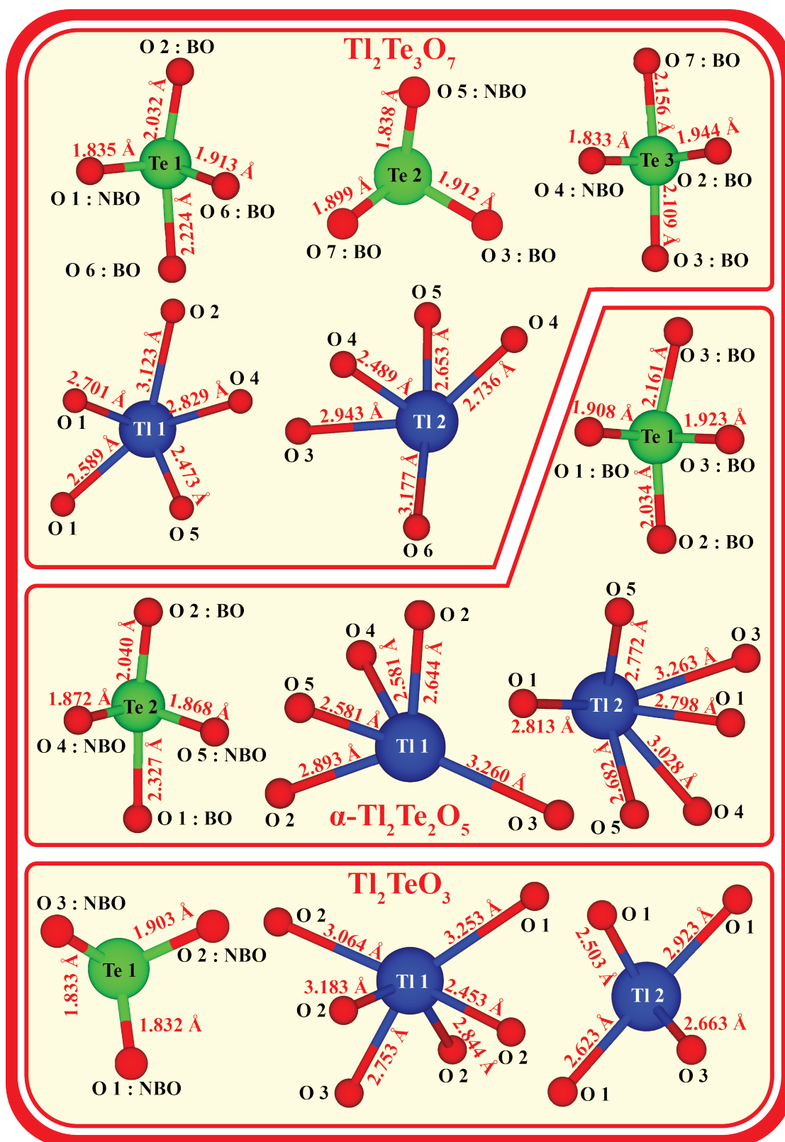
Figure 4.12: Various Tl and Te center environments in \text{Tl}_2\text{Te}_3\text{O}_7 , \text{Tl}_2\text{Te}_2\text{O}_5 , and \text{Tl}_2\text{TeO}_3 crystalline polymorphs.
