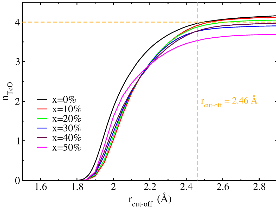
Figure 4.10: For all the (\text{TiO}_{0.5})_x - (\text{TeO}_2)_{1-x} binary glasses taken into consideration, the running coordination number ( n_{\text{Te-O}} ) using MLWF formalism as a function of TeO pair distance. Vertical dashed lines indicate distance cut-offs, and the dashed horizontal line indicates the ideal \text{Te}^{4+} coordination number.
