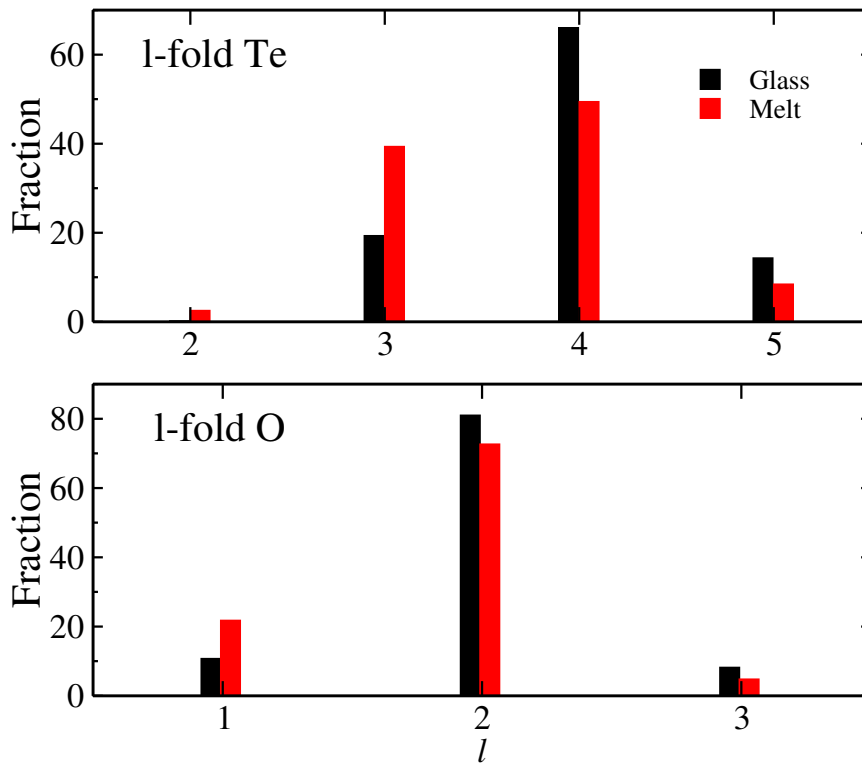
Figure 3.10: Decomposition of l -fold fractions of Te ( l = 2, 3, 4 and 5 ) and O ( l = 1, 2 and 3 ) evaluated on glass (black) and melt (red) \text{TeO}_2 .
