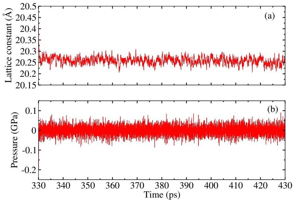
Figure A.5: (a) Lattice constant of the smallest cell vector and (b) Pressure variation as a function of Time during NPT ensemble run.
