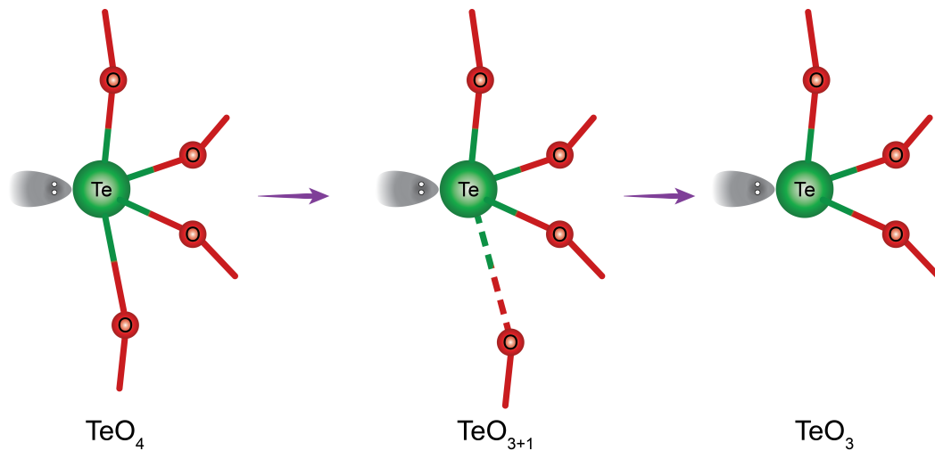
Figure 1.11: Depolymerization of \text{TeO}_4 unit into \text{TeO}_3 unit via \text{TeO}_{3+1} (1 long and 3 short bonds).
