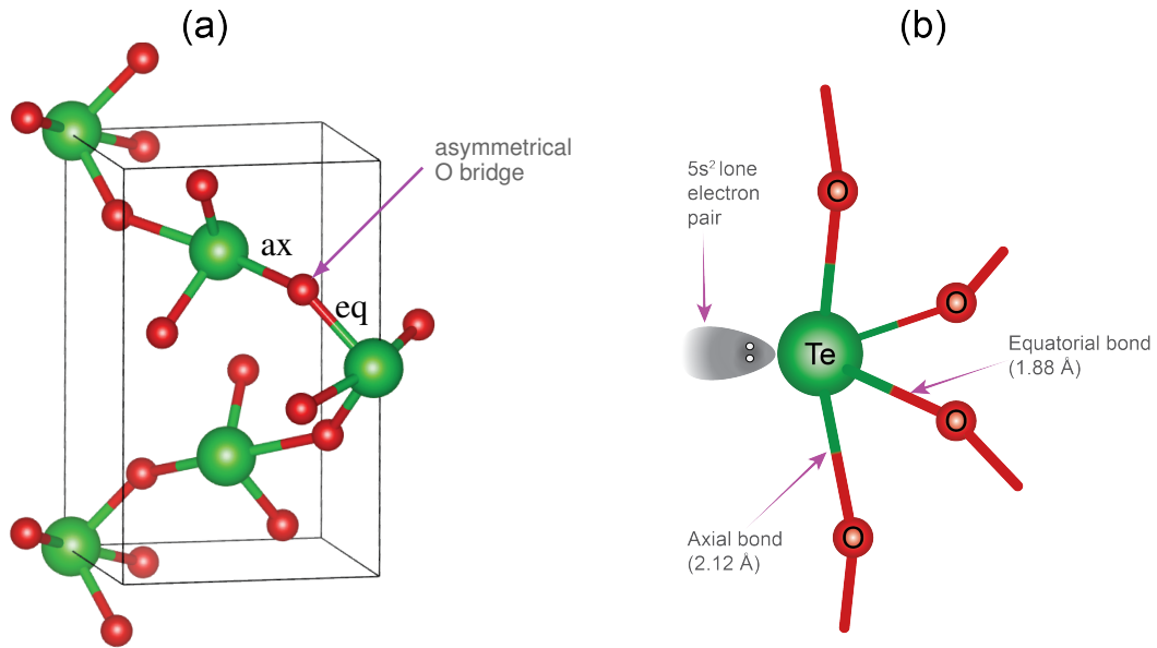
Figure 1.3: (a) \alpha -TeO 2 unit cell in perspective view showing a single sinusoidal "Te-O-Te" chain and (b) representation of TeO 4 disphenoid (or, TeO 4 E trigonal bipyramid) structural unit in \alpha -TeO 2 crystal where E represents lone pair (5s 2 ).
