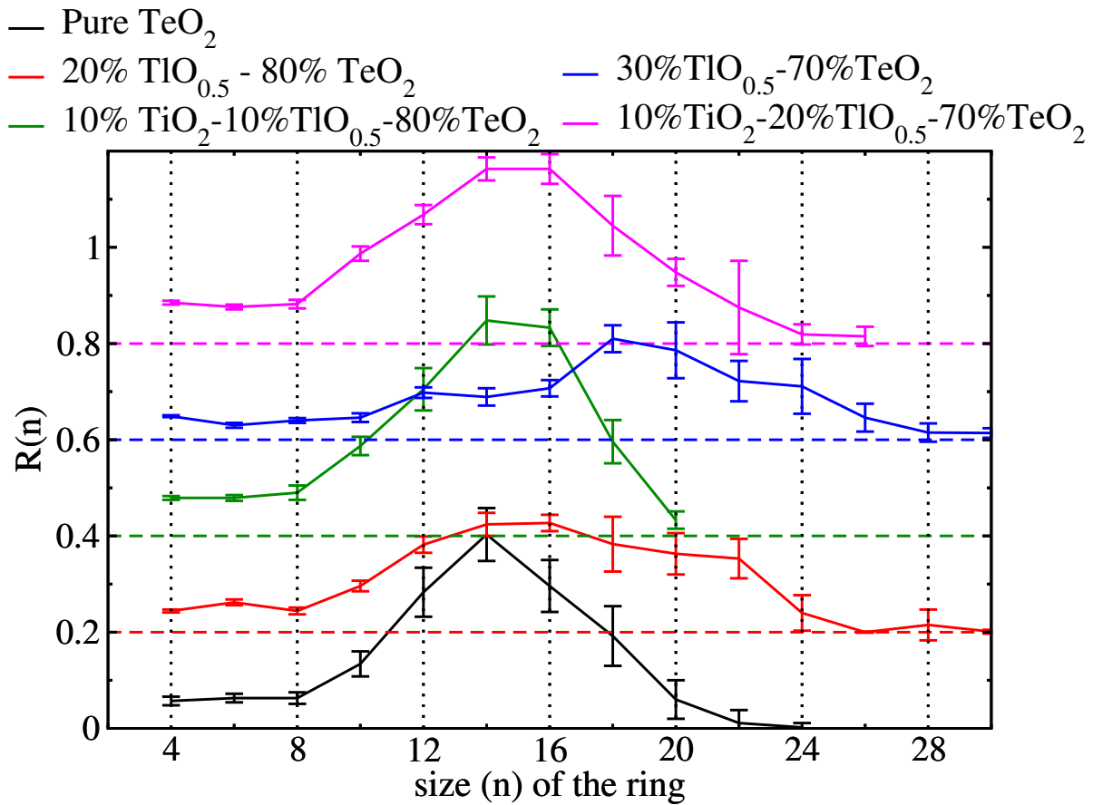
Figure 5.17: Connectivity profiles of various compositions in (\text{TiO}_2)_x - (\text{TlO}_{0.5})_y - (\text{TeO}_2)_{1-x-y} ternary glass. Y-axis, represents, R(n) , number of rings with size (n) , and is normalized to total number of atoms in each model. Vertical bars represent the standard deviation in the obtained values. For clarity, a shift of 0.2 units between each composition along with dashed horizontal lines showing zeros for particular curve are provided.
