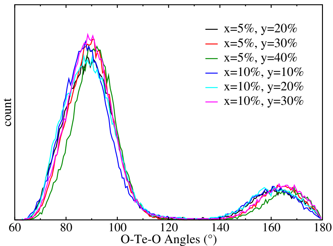
Figure 5.12: Bond-angles distribution of O-Te-O angles in (\text{TiO}_2)_x - (\text{TiO}_{0.5})_y - (\text{TeO}_2)_{1-x-y} ternary glasses.
