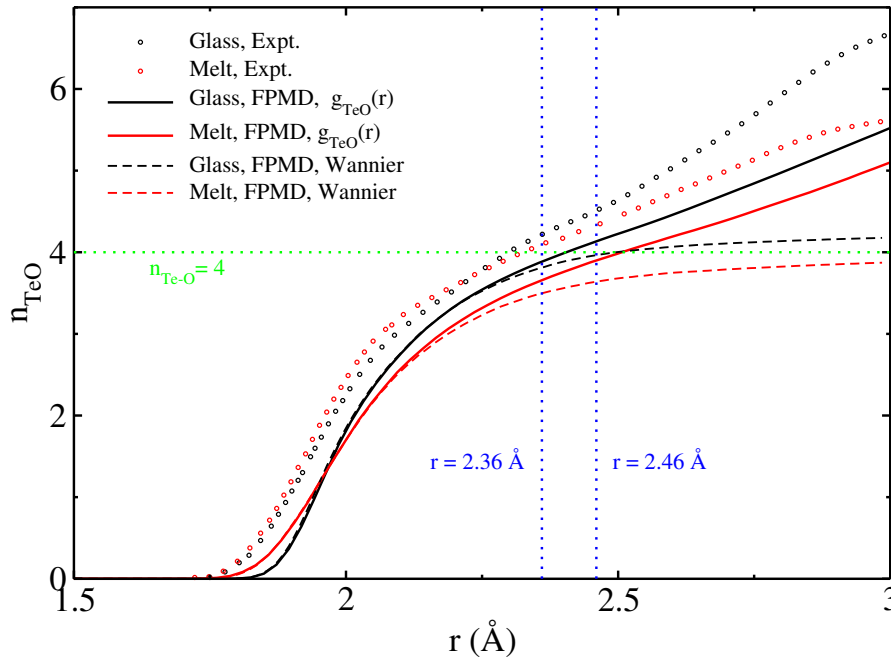
Figure 3.5: Running Te-O coordination number ( n_{\text{TeO}}(r) ) of glassy (black color) and melt (red color) \text{TeO}_2 system. Results obtained by integration of the Te-O partial PDF (solid lines) and based on Wannier centers (dashed lines) are compared to experimental results (circles) from Ref. [38]. Vertical dashed lines indicate distance cut-offs, and the dashed horizontal line indicates the ideal \text{Te}^{4+} coordination number.
