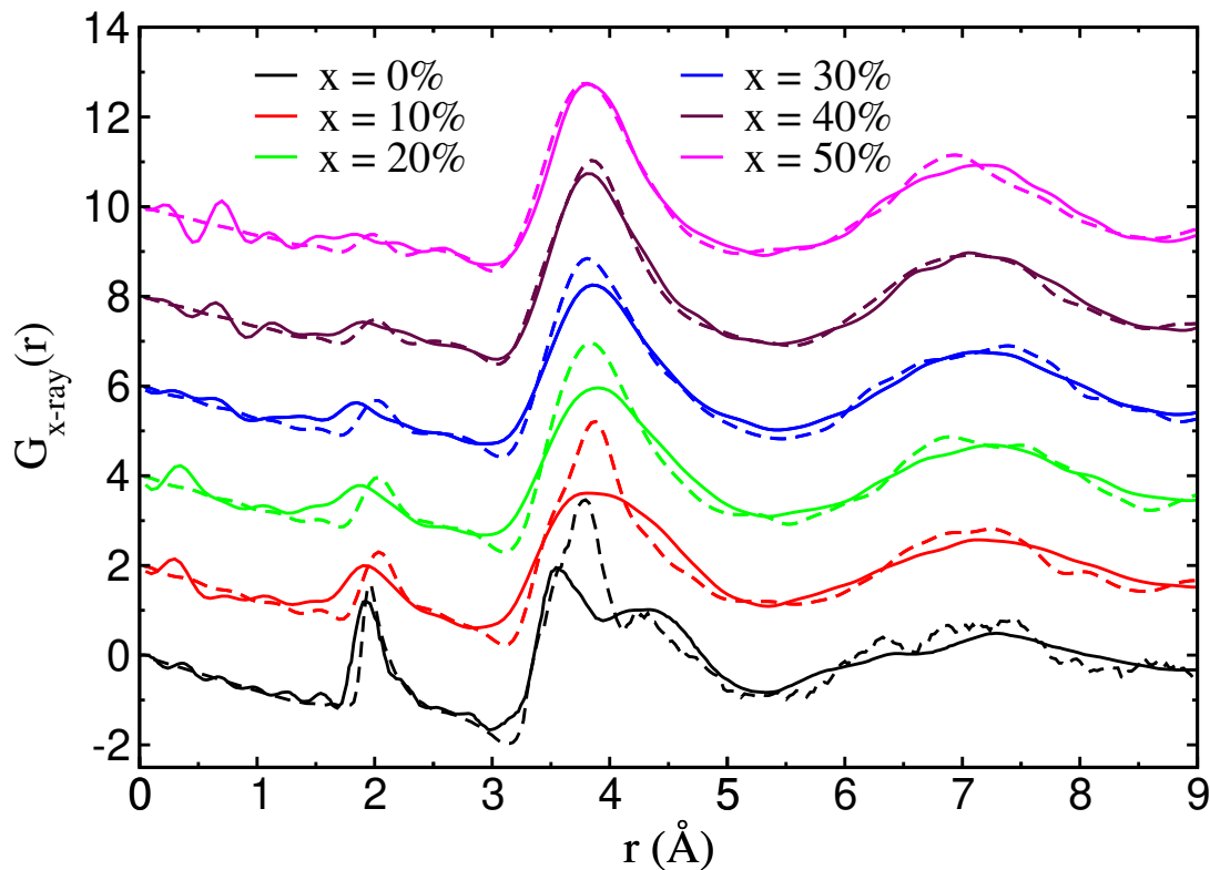
Figure 4.1: Comparison of total X-ray scattering PDF G(r) between experiments (solid lines) [113] and ab-initio MD simulation (dashed lines) for (\text{TiO}_{0.5})_x - (\text{TeO}_2)_{1-x} binary glassy system with various concentrations ( x ). Experimental and simulated data for x = 0\% are taken from Alderman et. al. [38] and calculated from PBE0 hybrid XC functional (see chapter [3])
