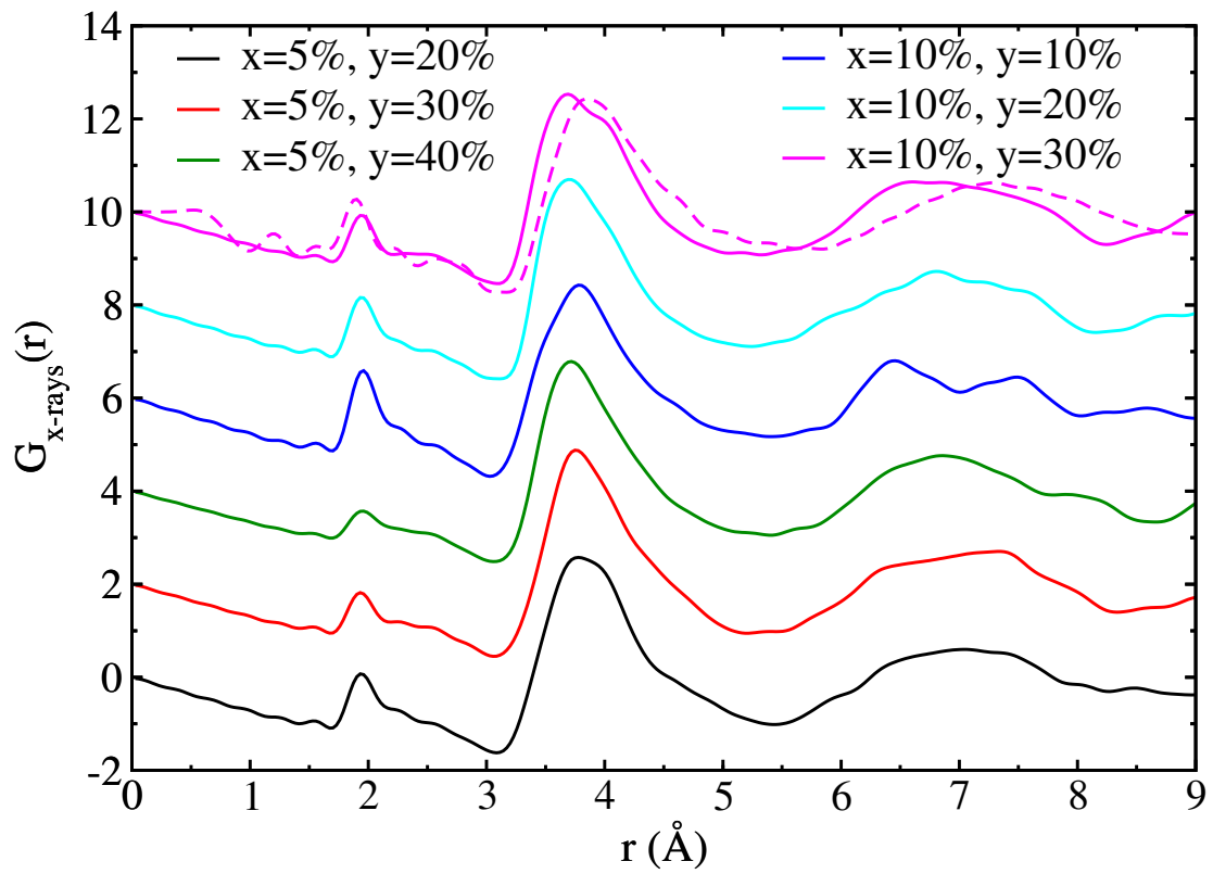
Figure A.8: Description of total G(r) PDF for various compositions in (\text{TiO}_2)_x - (\text{TiO}_{0.5})_y - (\text{TeO}_2)_{1-x-y} glassy system. Solid lines represent the computed G(r) from classical MD simulations while the dashed line shows experimental data [131]. For clarity, a vertical shift of 2 units is provided between various compositions.
