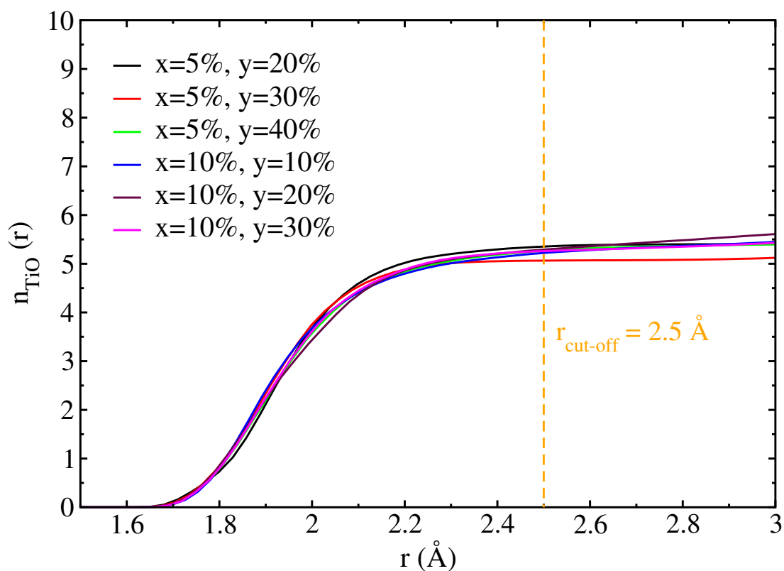
Figure 5.9: Running coordination ( n_{\text{Ti-O}} ) in (\text{TiO}_2)_x - (\text{TiO}_{0.5})_y - (\text{TeO}_2)_{1-x-y} ternary glass. Vertical dashed line represents the considered radius of the first coordination shell around Ti.
