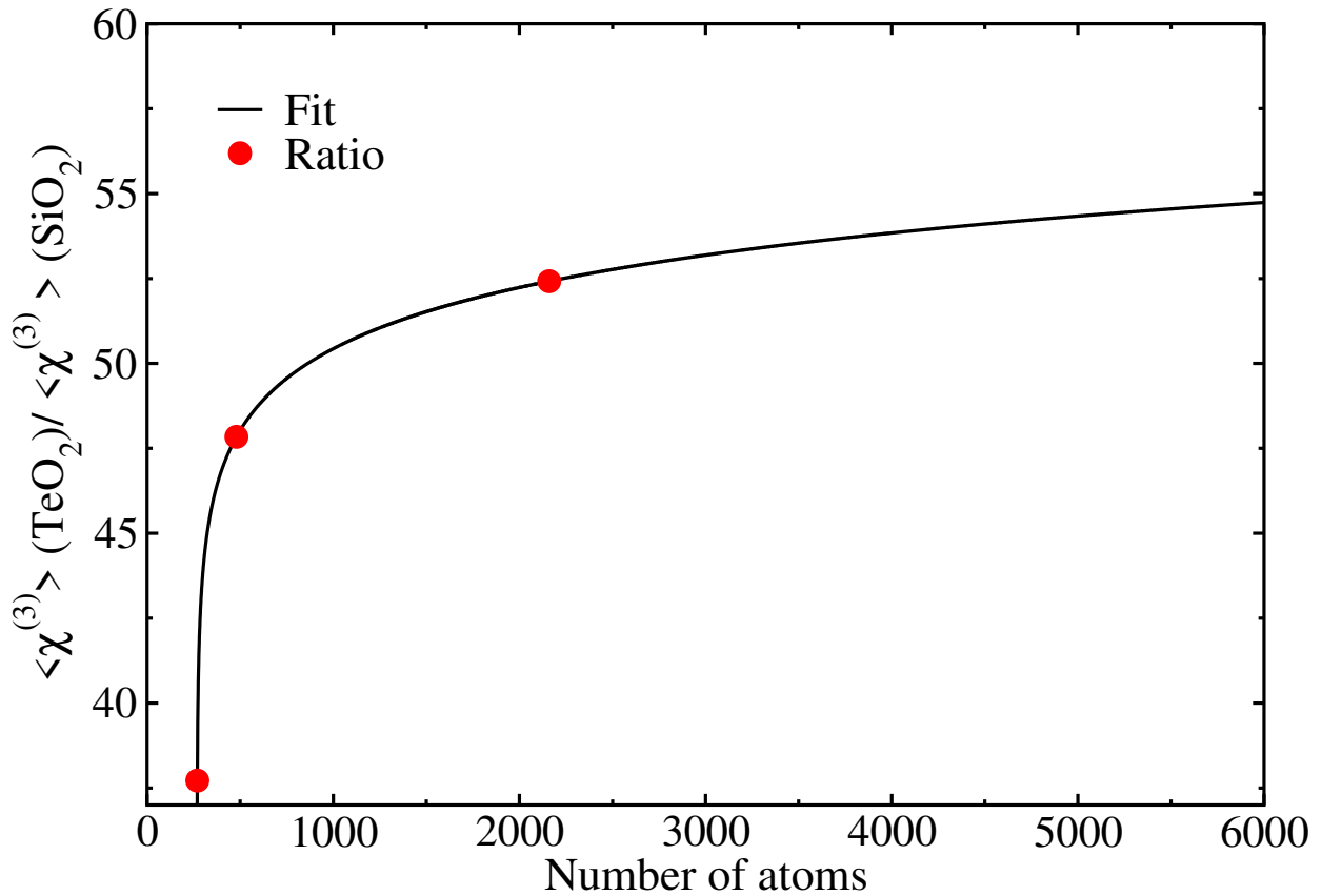
Figure 6.10: Ratio of non-linear susceptibility planar average \langle \chi^{(3)} \rangle of pure TeO 2 and SiO 2 dependence on system size. Convergence of the fit is performed by log function (a \times \ln(x - b) + c) .
