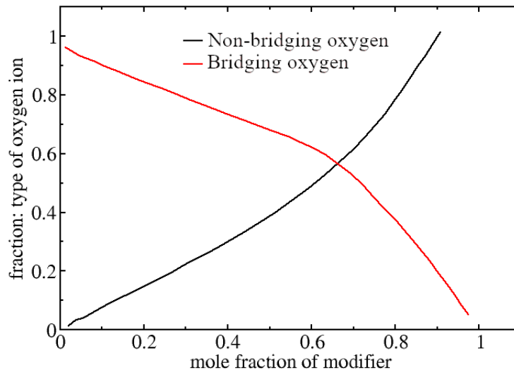
Figure 1.12: Variation of fraction of BO/NBO with the mole fraction of the modifier content. Picture source [42]
