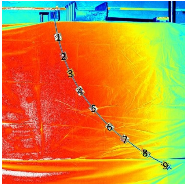
Figure 3.12: Trajectories of targets 1,2,3,4,5 and 8 obtained with a high speed camera (solid line —) and with FEM (solid line —)
