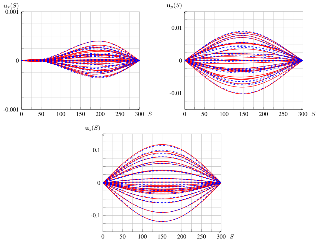
Figure 4.11: Displacement (mm) versus curvilinear abscissa (m) for the x direction, y direction and z direction obtained via FEM (solid line —) and via ROM (dashed line ---) for a transient dynamics in a quasi-linear regime- Parameters are given in Table 4.3
