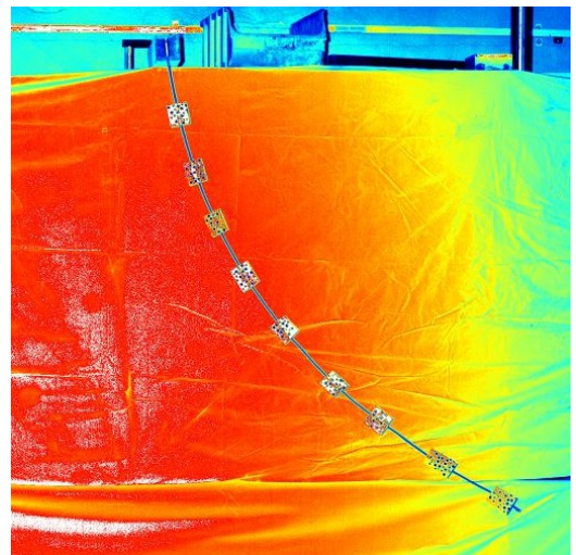
Figure 3.10: Hinge and target used for the experiment - Cable with targets mounted on
