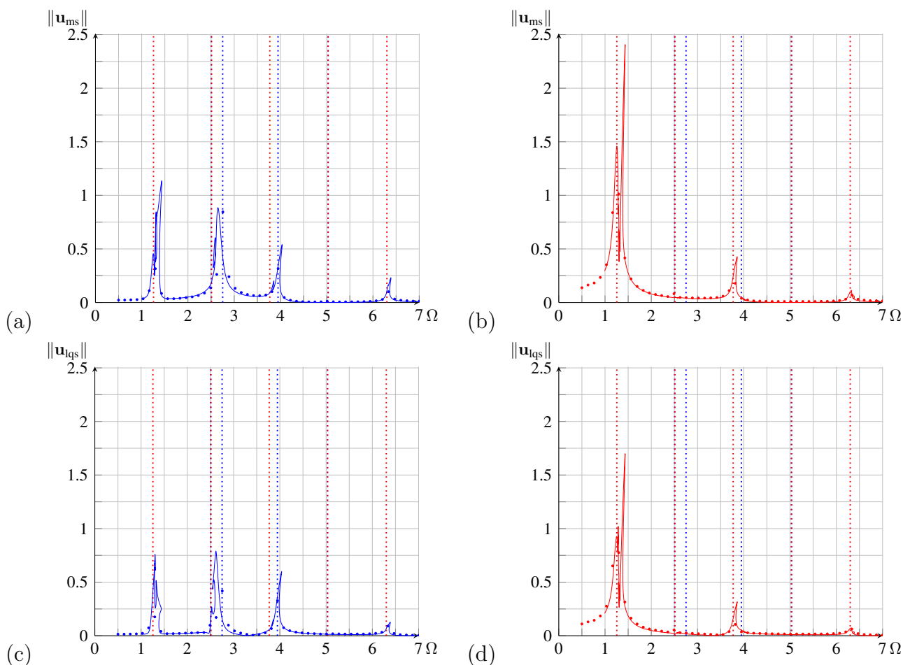
Figure 4.15: Displacement (m) versus frequency of forcing (rad/s) for the \mathbf{y} direction and \mathbf{z} direction obtained via FEM (dots \bullet ) and (dots \cdot ) and via arc-length continuation endowed in the ROM (solid line \text{---} ) and (solid line \text{---} ) in a nonlinear regime - (a) Vertical amplitude at midspan (b) Transversal amplitude at midspan (c) Vertical amplitude at last quarter span (d) Transversal amplitude at last quarter span - Undamped frequencies are plotted vertically - Parameters are given in Table 4.4
