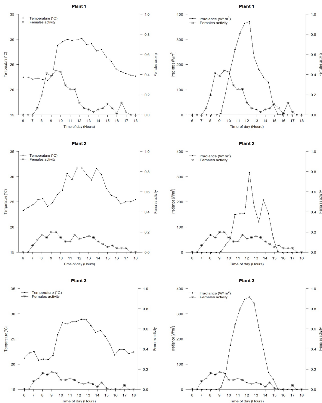
Figure 2.6 – Circadian patterns of both oviposition and searching activities of females (ratio between the number of females in activity and the female population size) on three potted Rubus alceifolius in insect-proof cages using for each of them a cohort of 75 Cibdela janthina female adults. Temperature and irradiance are means per half an hour.
