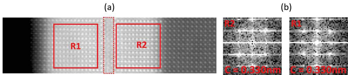
Figure IV-18 (a) STEM image of a 10 nm thick NSNO 2 (0) uncapped thin film (b) FFT of the 2 regions indicated by red boxes in (a) exhibiting c-axis parameter of 0.330 nm for both regions.
