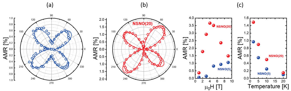
Figure V-22 Polar plots of in-plane AMR as a function of the \varphi angle for measurements performed at 2 K under a magnetic field of 9 T for (a) \text{NSNO}_2(5) and (b) \text{NSNO}_2(20) capped-experimental data as dots and fitting represented with lines, (c) temperature- and field-depend with \text{NSNO}_2(5) in blue and \text{NSNO}_2(20) in red.
