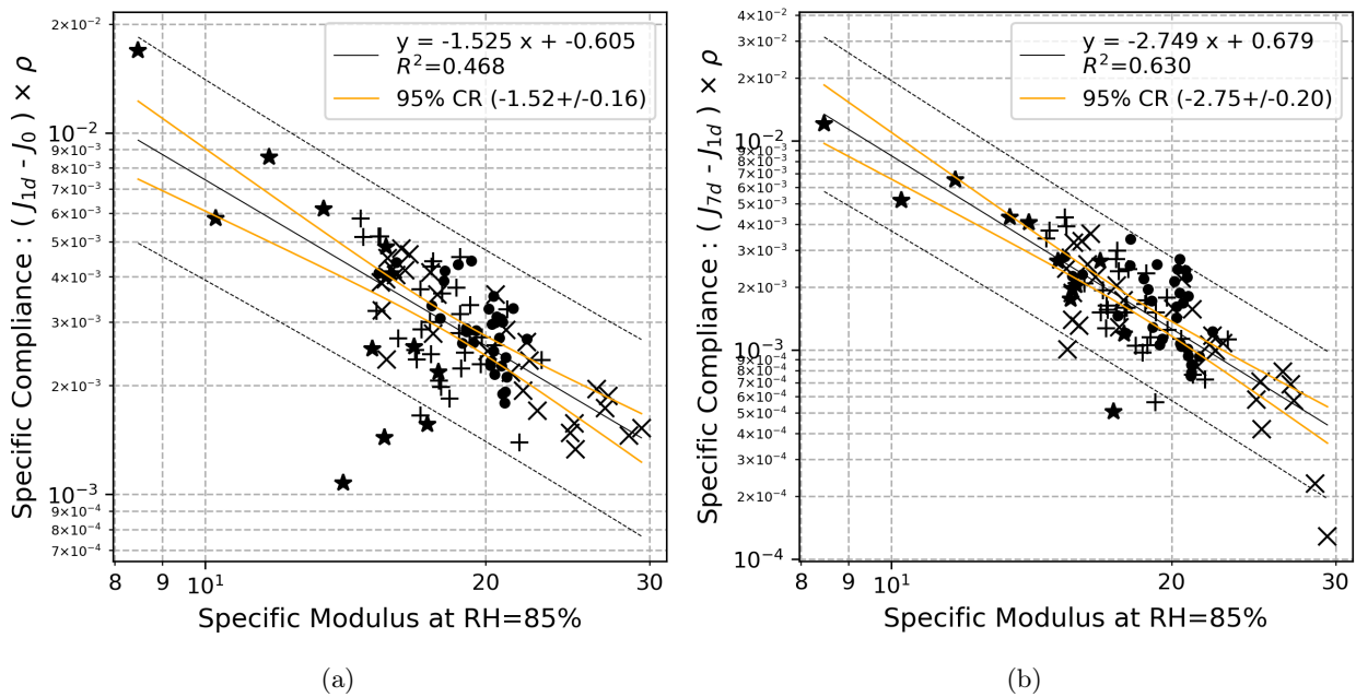
Figure 5.17: The relation between specific compliance and specific modulus. (a) primary creep (b) secondary creep. \times : Douglas fir, \bullet : Poplar, \star : Oak, + : Beech, — : 95% confidence region (CR), - - - : 95% prediction band
