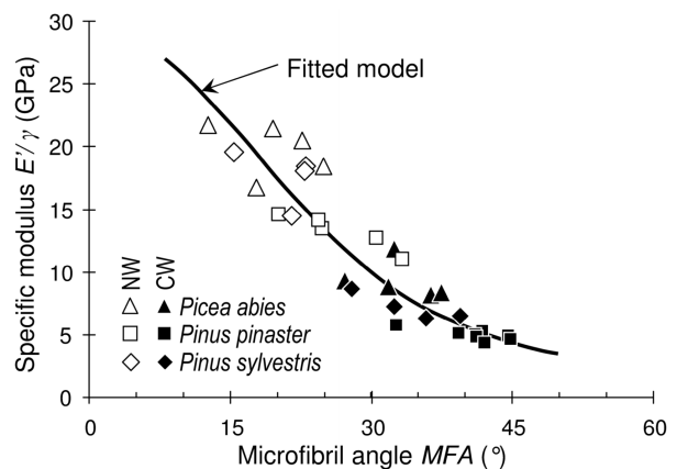
(b) Relationship between microfibril angle (MFA) and specific modulus (Brémaud et al., 2013). Fitting equation is equation 3.8.
