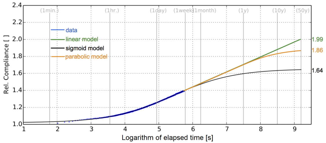
Figure 4.6: Relative compliance of 1 week creep test data at moisture content = 26% and predictive models toward 50 years (Montero and Gril, 2016).
