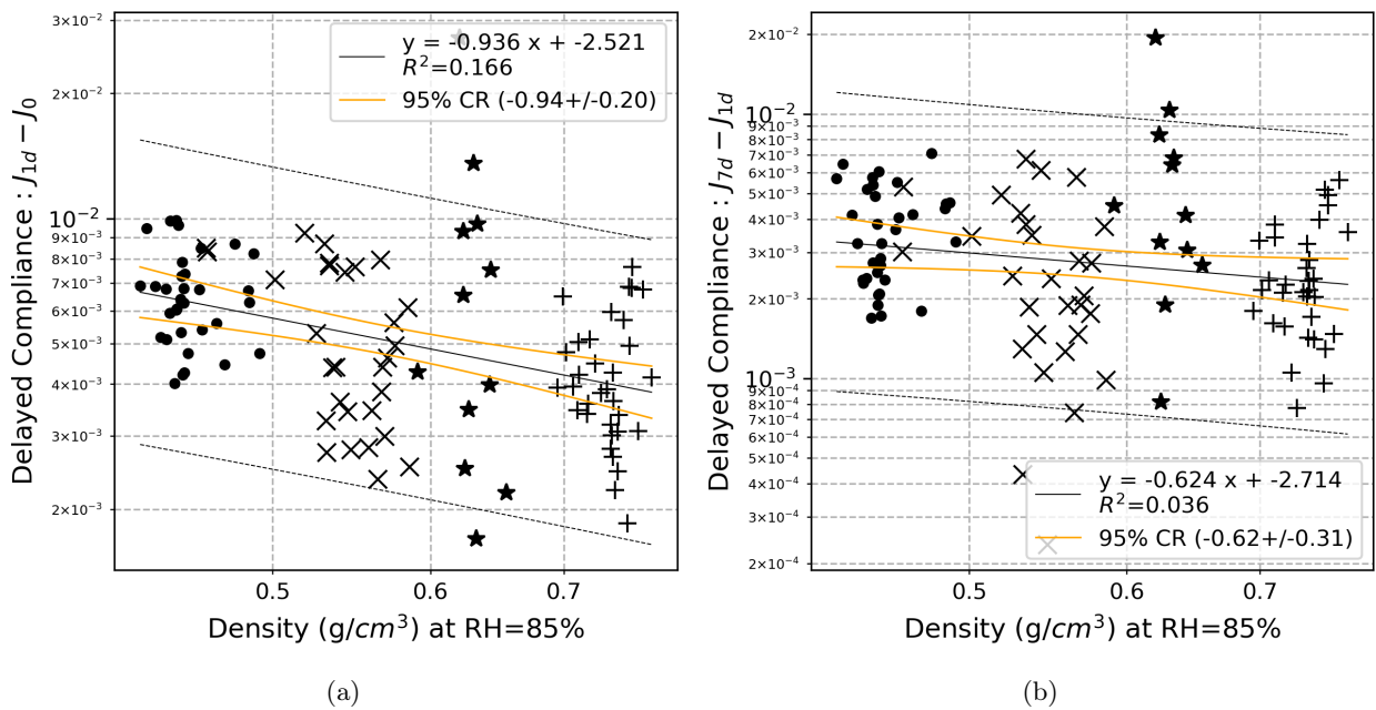
Figure 5.15: The relation between delayed compliance and density. (a) primary creep (b) secondary creep. ×: Douglas fir, ●: Poplar, ★: Oak, +: Beech, —: 95% confidence region (CR), - - -: 95% prediction band
