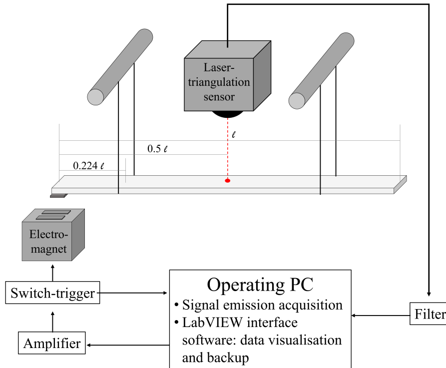
Figure 3.12: Vybris system
