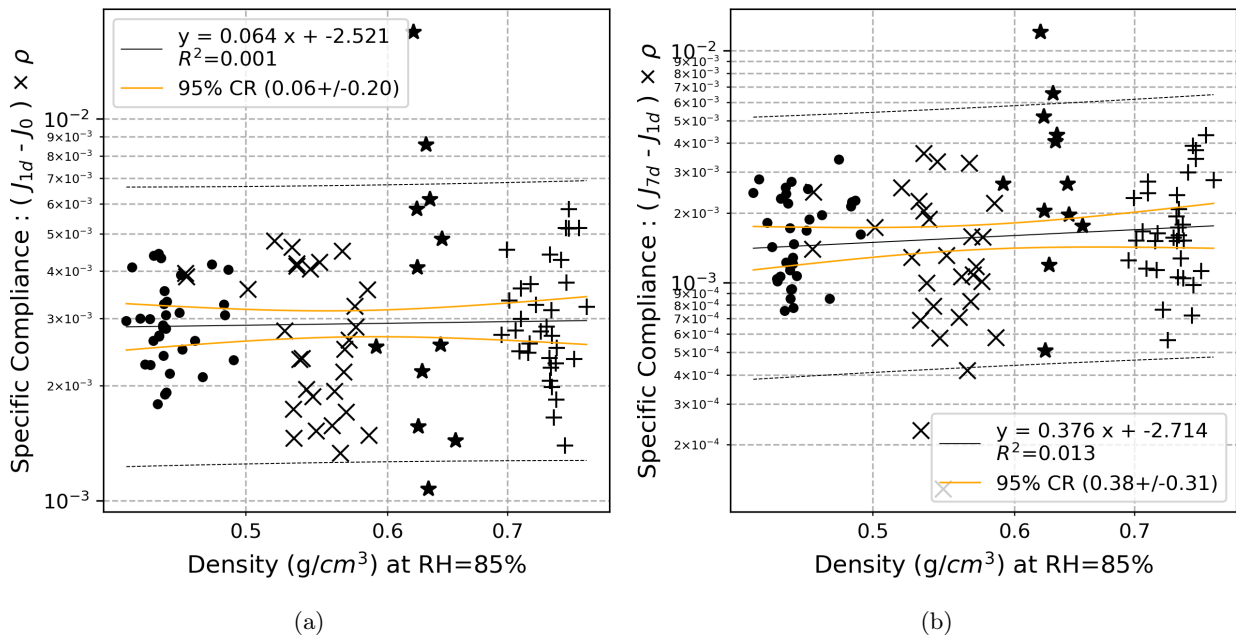
Figure 5.16: The relation between specific compliance and density. (a) primary creep (b) secondary creep. \times : Douglas fir, \bullet : Poplar, \star : Oak, + : Beech, \text{---} : 95% confidence region (CR), \text{---} : 95% prediction band
