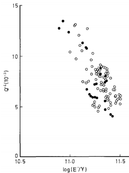
(b) Solid circles show ring-porous wood, open circles diffuse-porous wood. (Ono and Norimoto, 1984)
