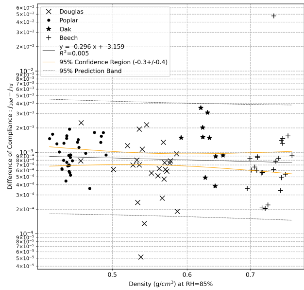
(f) J_{10d} - J_{7d}
