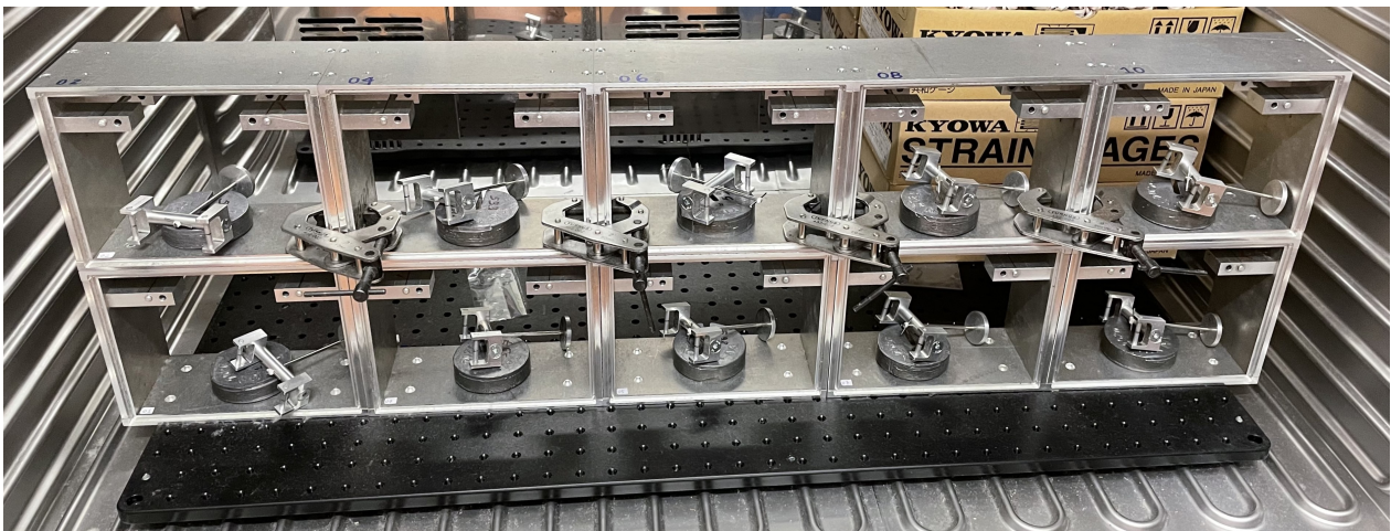
Figure 4.2: Creep boxes in chamber before installing the specimens. The boxes are connected by C-clamps and fixed at the bottom of the chamber.
