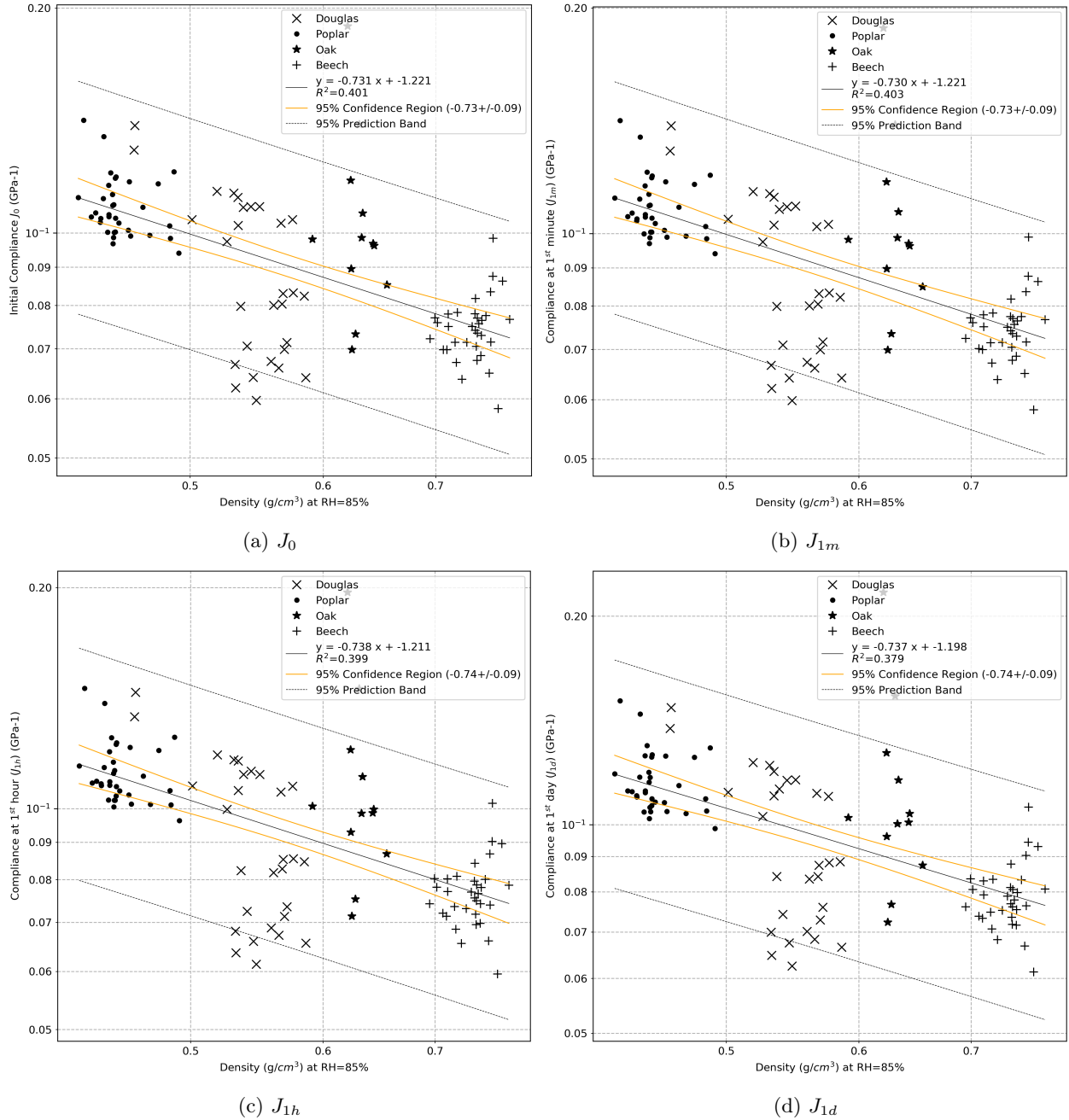
Figure 4.19: Correlation between density at RH=85% and compliance. (a) initial compliance J_0 . (b) compliance at 1 st minute J_{1m} . (c) compliance at 1 st hour J_{1h} . (d) compliance at 1 st day J_{1d} .
