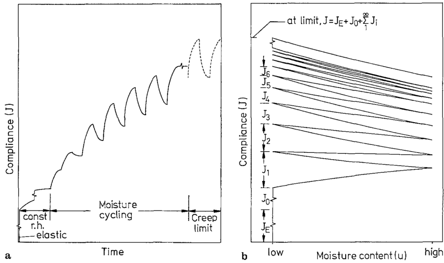
Figure 1.11: Schematics representation of mechano-sorptive creep over time (left) and moisture content (right) (Hunt, 1989)
