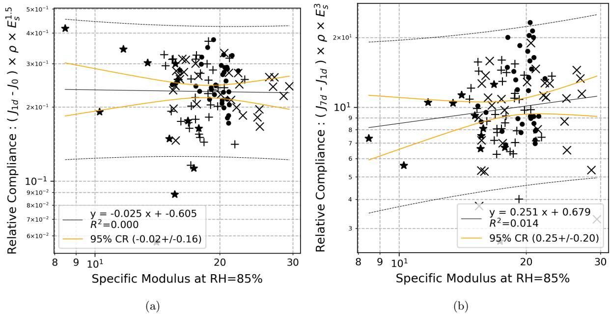
Figure 5.18: The relation between adjusted relative compliance and specific modulus. (a) primary creep (b) secondary creep. \times : Douglas fir, \bullet : Poplar, \star : Oak, + : Beech, \text{---} : 95% confidence region (CR), \text{---} : 95% prediction band
