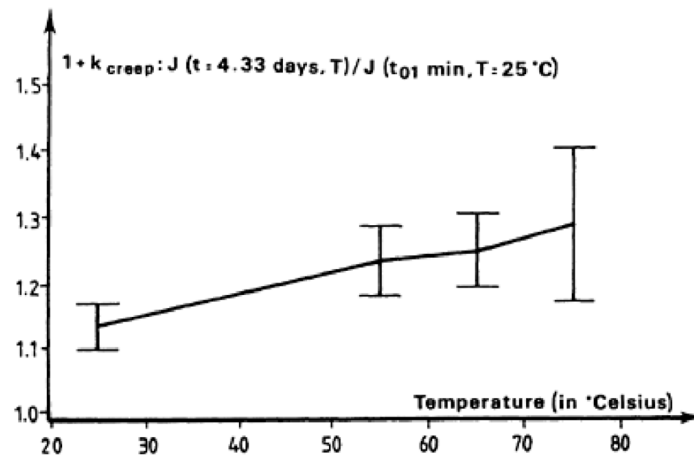
Figure 4.4: Creep behavior at different testing temperature. (Morlier, 1994)
