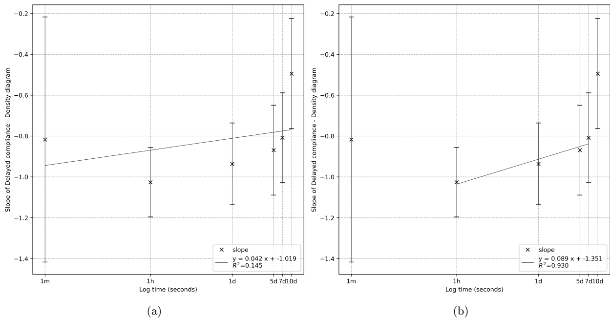
Figure 5.9: Regression slope of delayed compliance and density. (a) The linear regression result from J_{1m} - J_0 to J_{10d} - J_0 . (b) The linear regression result from J_{1h} - J_0 to J_{7d} - J_0 .
