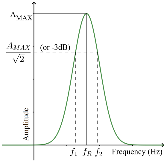
(a) Calculation method of \Delta f/f_R by forced-vibration
