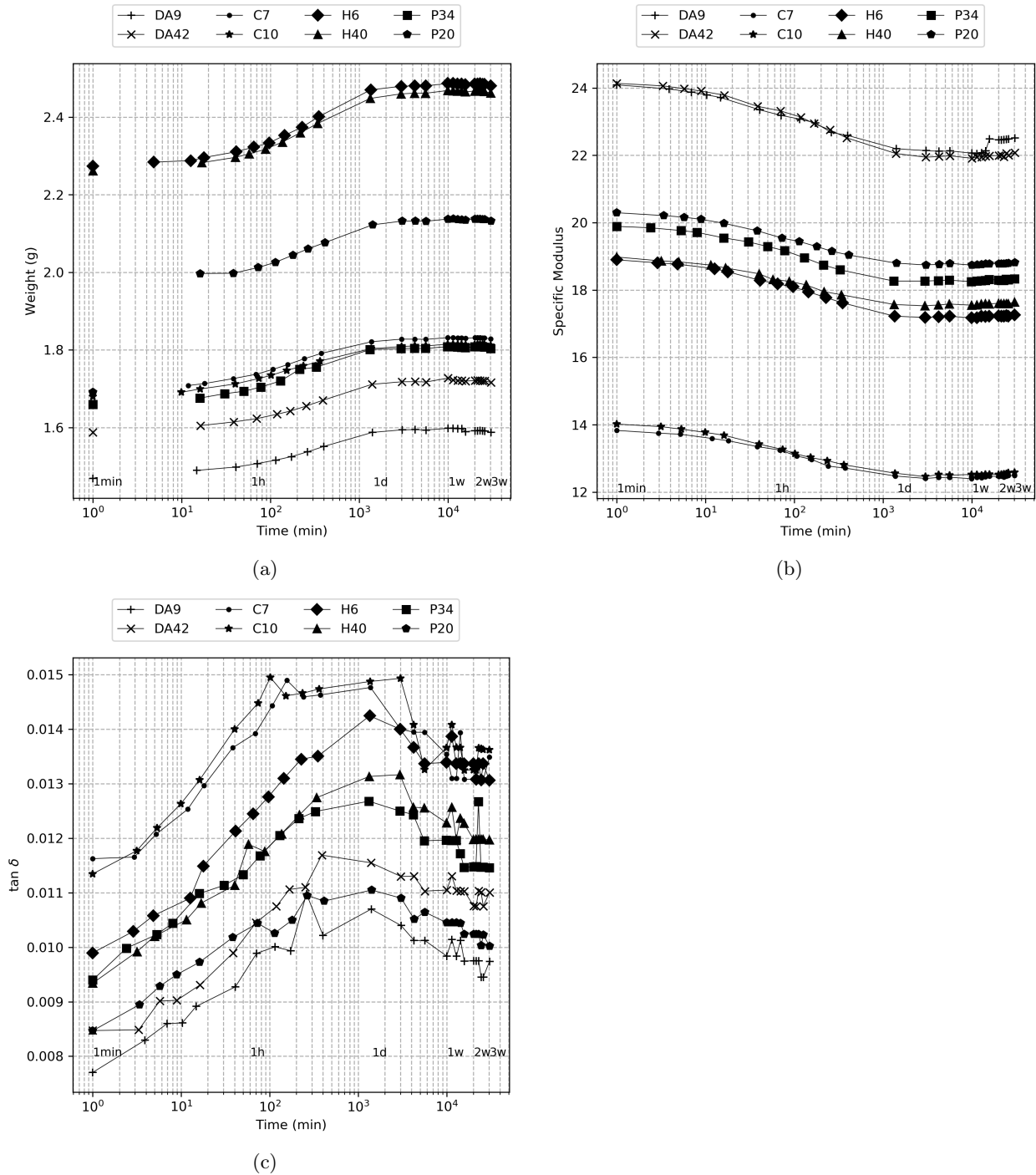
Figure 3.13: The record of weight, specific modulus and damping coefficient during the equilibrium process
