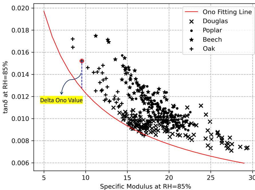
Figure 3.16: Definition of delta Ono value
