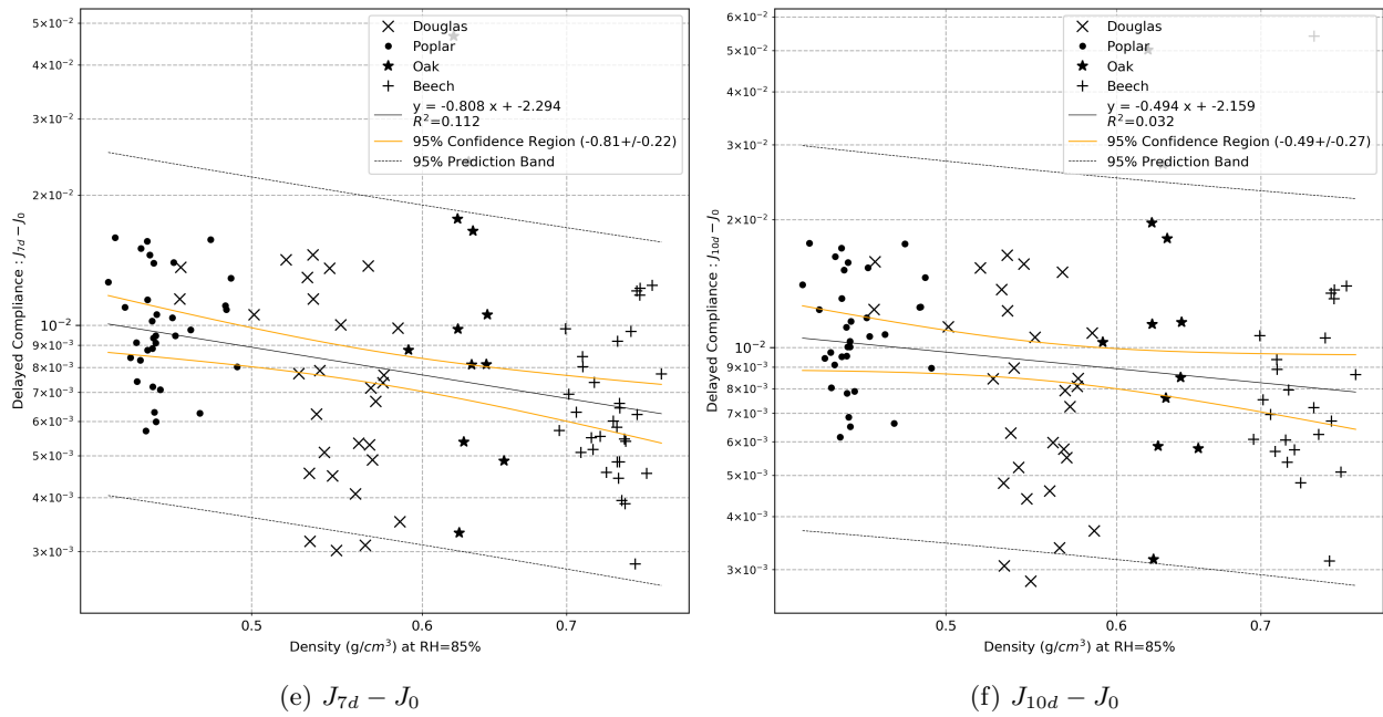
Figure 5.8: Correlation between delayed compliance and density (Continue). (e) Compliance at 7 th day minus initial compliance. (f) Compliance at 10 th day minus initial compliance.
