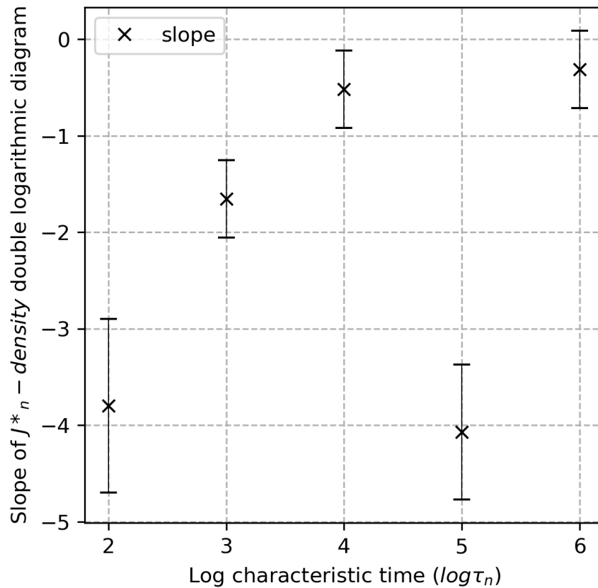
Figure 5.22: Linear regression result of J_i and density
