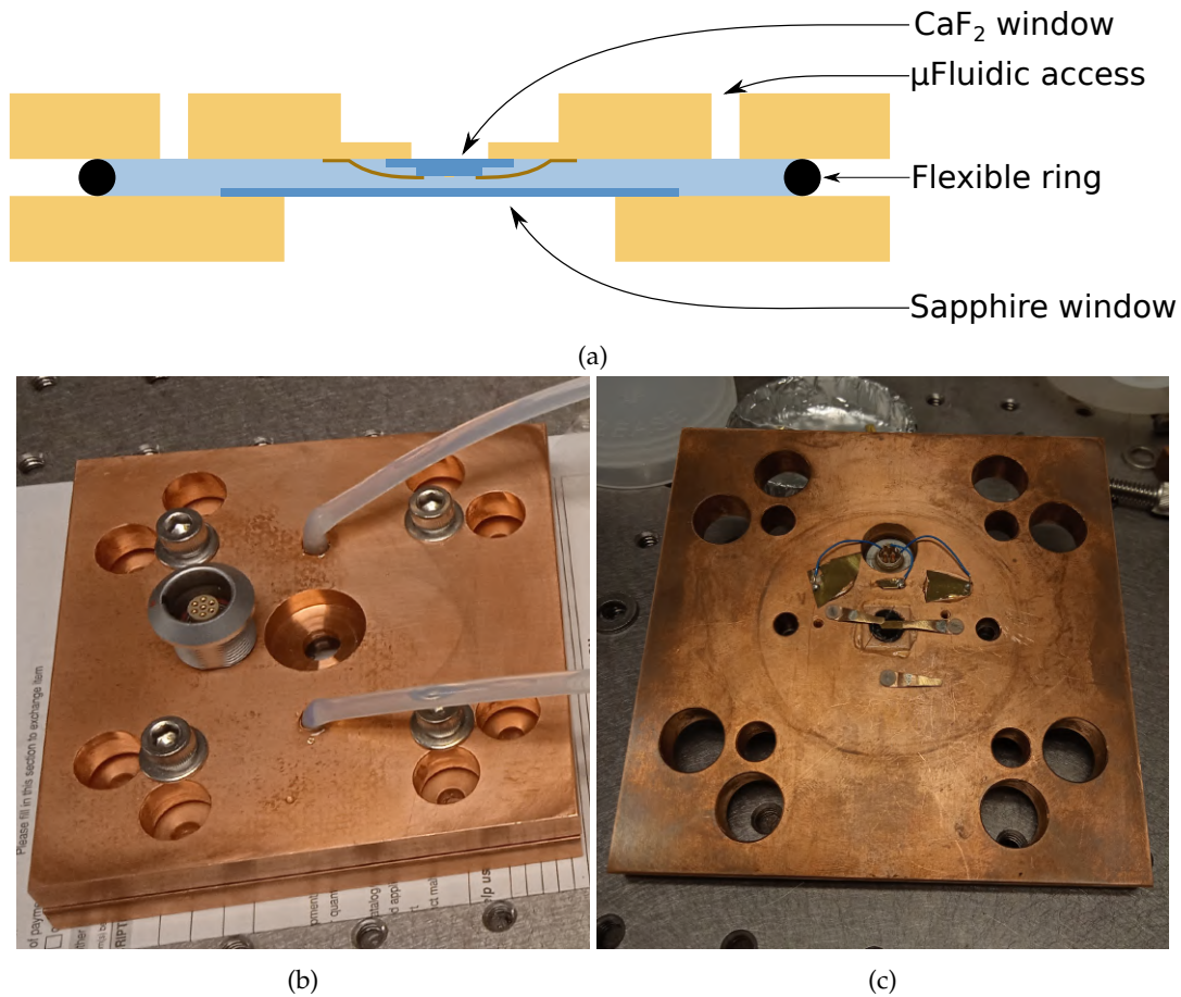
Figure 5.22: (a) : Schematic cross section of the sample holder. The sample is held in place against the CaF 2 window with metal clips. The top copper plate is shaped to facilitate mid-IR access at 45°. Electrical connections are not represented in this schematic. (b) : Assembled sample holder. (c) : Inside view of the top plate with a mounted test sample. The electrical connection is done with wire bonding with the gold coated glass slides glued to the copper and soldered to the external electrical connection.
