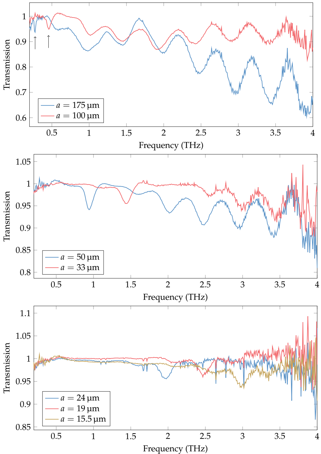
Figure 4.11: Transmission spectra of 7 individual SRRs, with sizes ranging from 15.5 \mu\text{m} to 175 \mu\text{m} normalized with the quartz transmission. The lowest resonance is measured at 275 \text{ GHz} , and the highest at 3 \text{ THz} . In each spectra from 33 \mu\text{m} to 175 \mu\text{m} , we see a broadband modification of the reflectivity starting at roughly twice the resonance frequency.
