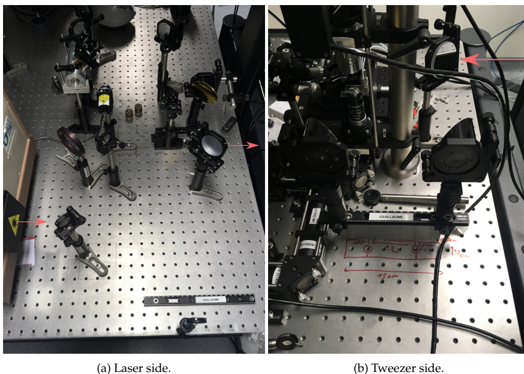
Figure 5.8: THz optical setup. (a) : The beam goes through a polarization rotator made of three planar mirrors. It is then enlarged with two confocal parabolic mirrors and directed toward the tweezer optical table. (b) : The beam diameter is reduced with two confocal parabolic mirrors and focused on the sample with another parabolic mirror.
