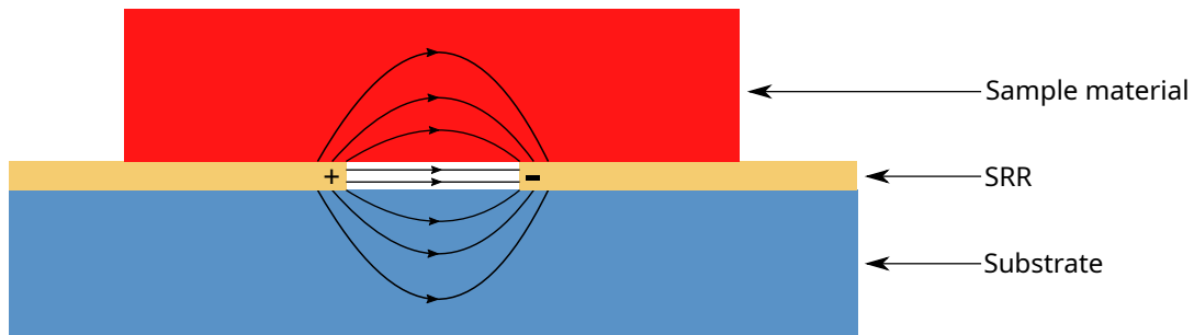
Figure 4.26: Schematic cross section of a SRR gap and its field line coupled with a crystal. The electric field is polarized out of plane above the metal, but the vertical component is anti-symmetric and has a zero mean value. A mode that couples with a vertically polarized electric field should couple to the SRR, unless the mode is delocalized over a distance larger than the gap.
