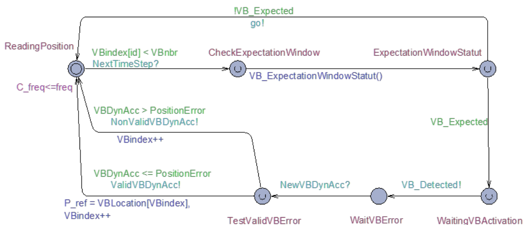
Figure 4.12: Virtual Balise Reader module (VBR) representing VB activation
