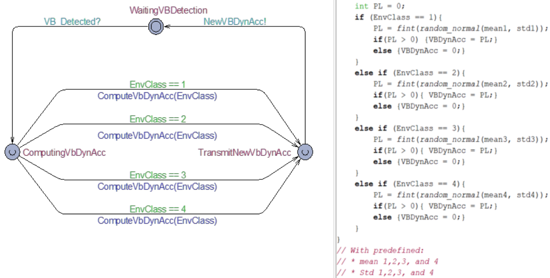
Figure 4.16: Module representing the PL generation according to the active environment class.
