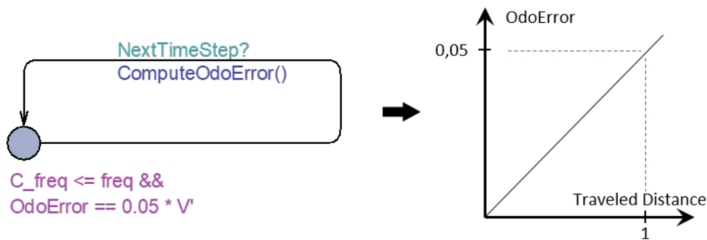
Figure 4.10: Preliminary representation of the odometer accumulated error on the estimated traveled distance.
