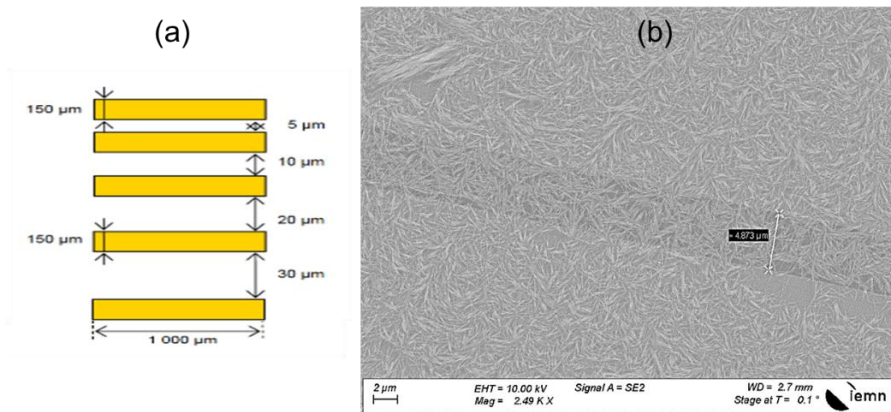
Figure 4.22. (a) Scheme of the TLM pattern with 5 gold lithographed electrodes and (b) SEM image of the deposited NW network.
