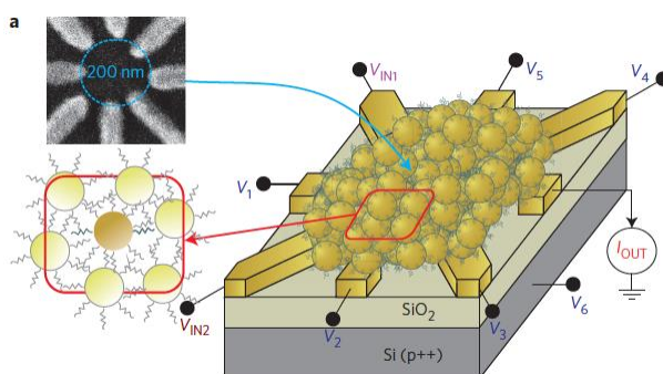
Figure 1.18. Schematic of the device layout of reconfigurable logic. 99
