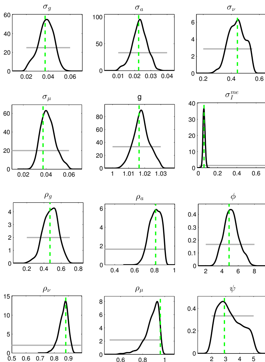
FIGURE 1.6: Posterior distributions
