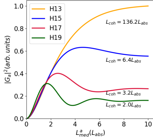
Figure 11.7: Phase matching along the propagation direction in NCHHG. Harmonic yield ( |G_a(\Delta\vec{k}_{q_s})|^2 ) for p=0 as a function of the medium length, along \vec{a} . The solid lines represent the harmonic signal for four different harmonics which give four different values of L_{\text{coh}} along \vec{a} . The intensity of the main beam is 0.5 * 10^{14} W/cm 2 , with \alpha = 0.2 . The two beams cross at an angle of 30 mrad.
