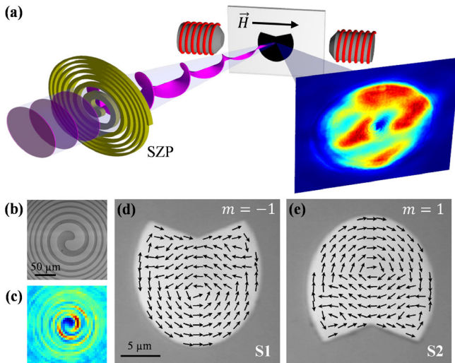
FIG. 1. (a) Schematics of the experimental setup at the DiProI beam line, showing the incoming FEL beam with planar wave front, a SZP that imparts OAM to the FEL beam, the sample placed between the poles of the electromagnet and the image of the scattered beam. (b) Scanning electron microscope image of one SZP ( \ell = +1 ). (c) Far field image of the interference pattern of the corresponding OAM beam and the undiffracted, OAM-free beam, featuring a spiraling intensity pattern. (d),(e) Magnetic dots S1 and S2 with corresponding remanent magnetization after applying a pulse of saturating external field \vec{H} as in (a). An opposite field reverses the curling direction m of the remanent magnetization in both samples.
