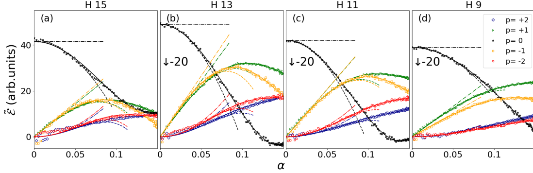
Figure 7.6: The magnitude of the electric fields of the diffraction orders p = 0, \pm 1 and \pm 2 for harmonics 15, 13, 11 and 9 as obtained from the experiment. The solid lines are the fitting of the data with the first 3 terms in the expansion of equation 7.13. The dashed lines are fits with two terms and the dot-dashed lines with just one term.
