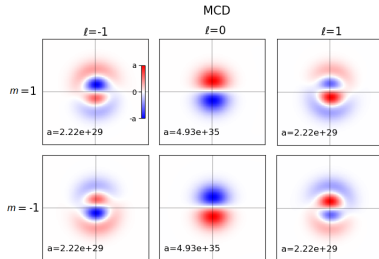
FIG. S14: Magnetic circular dichroism, obtained changing the circular polarization at fixed light OAM and the curling direction of the MV.
