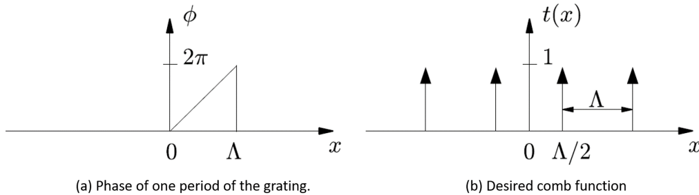
Figure 6.5: Blazed grating: The complex transparency of the grating can be constructed by the convolution of a triangular phase profile and a comb function.
