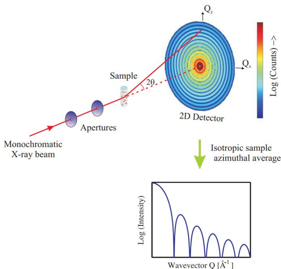
Figure 2.5 Schematic layout of a Small-Angle X-ray scattering beamline from ref. 5. An incident monochromatic X-ray beam is collimated using a set of apertures (placed at collimation distance, usually of the order of the sample-detector distance) and interacts with the sample. The scattered beam is detected on a two-dimensional XY detector. The measured signal is proportional to the incident flux, the “illuminated” area of the sample, its transmission. For isotropic samples, the scattering is azimuthally averaged to obtain the scattering intensity versus the modulus of the scattering vector q .
