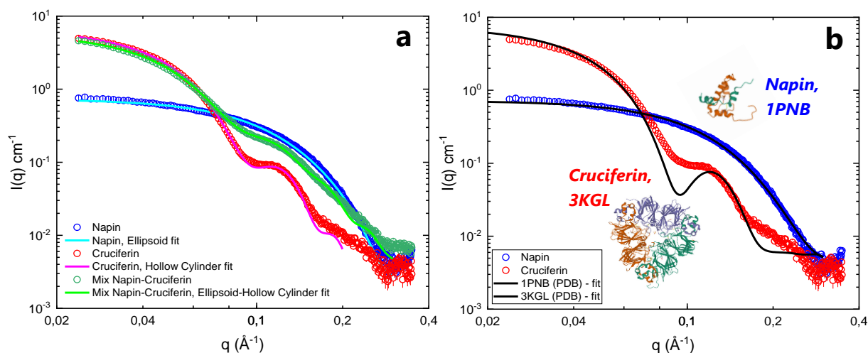
Figure 3.1 SAXS of “native” canola protein solutions (pH \sim 7.5, c=0.1 \text{ g/cm}^3 ): a ) napin (blue), cruciferin (red), their mixture (green). Lines represent the best fits: ellipsoid for napin (with R= 22 \text{ \AA} and r= 12 \text{ \AA} ), hollow cylinder for cruciferin (with R= 46 \text{ \AA} , r= 10 \text{ \AA} and L= 55 \text{ \AA} ) and the mix of both form factors (with volume fractions 47% - 53%). b ) The same data for napin and cruciferin with the simulations of the corresponding 1PNB and 3KGL Protein Data Bank (PDB) structures from CRYSOLOG software.
