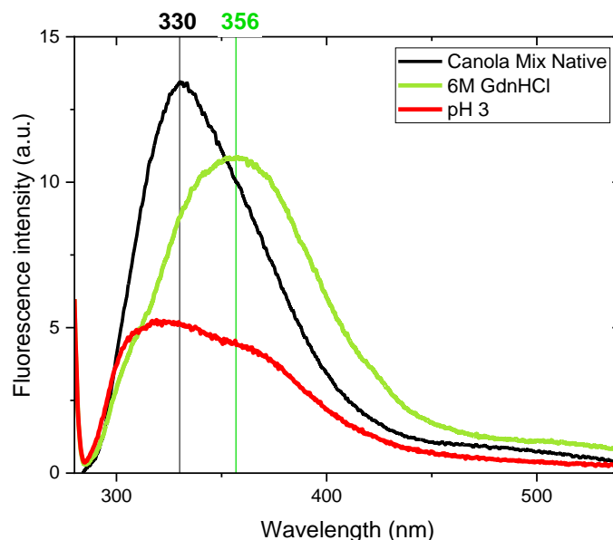
Figure 3.9 Fluorescence emission spectra for canola protein mix solutions (1g/L): native pH ~8 (black), at pH 3 (red) and in 6 M GdnHCl solution (green).
