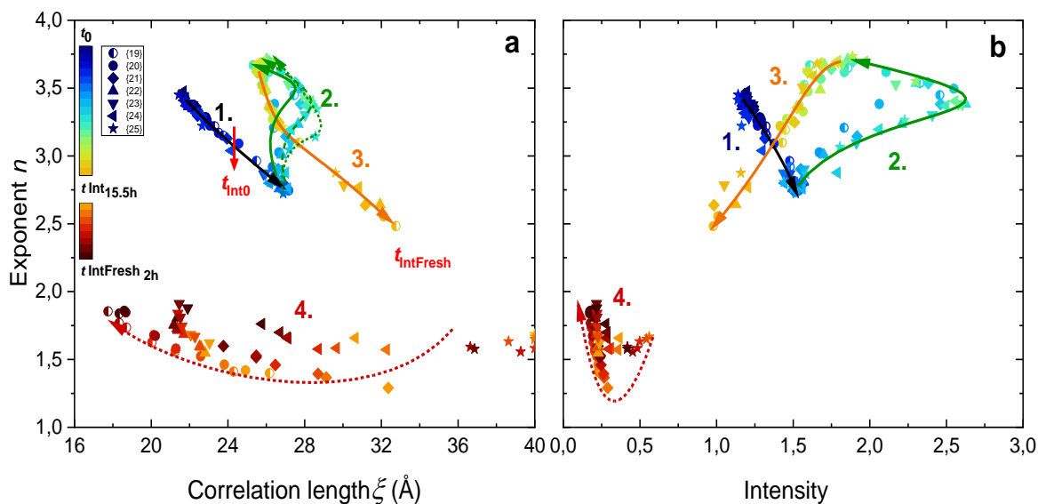
Figure 4.16 Diagrams presenting the evolution during gastro-intestinal digestion (gastric only until 3.5 h = t_{\text{int}0} , after which intestinal juice was added - red arrow, up to 15.5 h) of pH 11 gel , with the fitting parameters ( \xi , n , intensity ) describing the structural changes at the scale of proteins. a) exponent n as a function of correlation length \xi . b) exponent n as a function of intensity . The shapes of the symbols correspond to 7 different z positions in the capillary (19-25, with a 150 \mu\text{m} interval) and colors correspond to the digestion time as in Figure 4.15a . Numbers indicate the 4 characteristic steps of digestion and arrows - the evolution directions. (Figure 2 in ref. 2).
