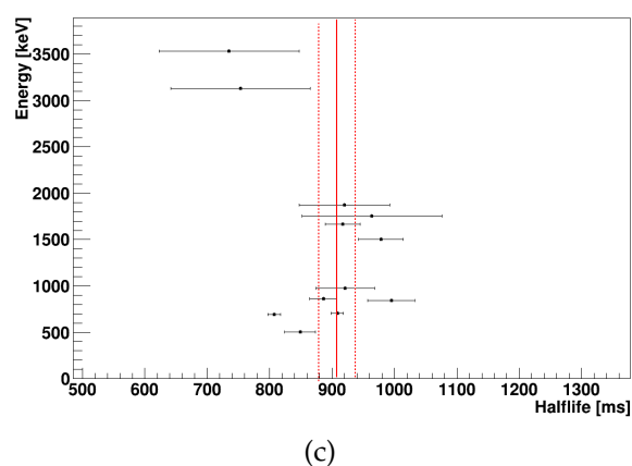
Figure 6.36: Measured half-lives of all \gamma -ray transitions associated with the beta decays of ^{82}\text{Ga} (a), ^{83}\text{Ga} (b) and ^{86}\text{As} (c). The red lines represent the half-lives of the strongest \gamma -ray transition in each nucleus \pm 3\sigma (dashed lines).
