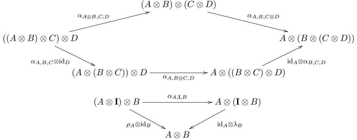
FIGURE 4.1.1. Coherence conditions for monoidal categories
