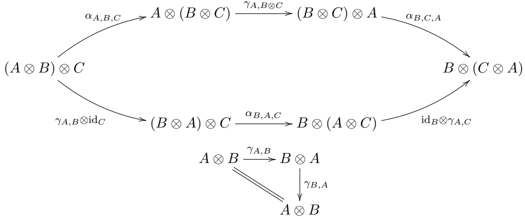
FIGURE 4.1.2. Coherence conditions for symmetries
