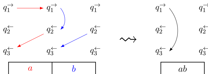
FIGURE 1.1.1. The behavior of a 2DFA with 3 states on the inputs a and b determines, by monoid multiplication, its behavior on the concatenation ab .
