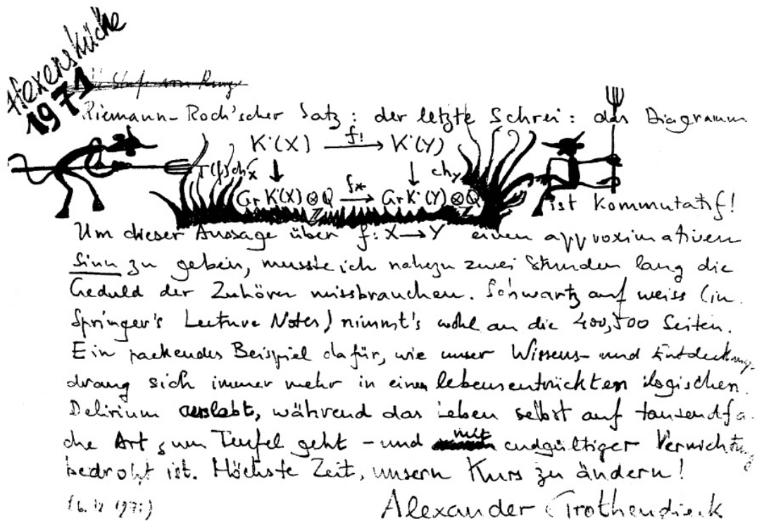
FIGURE 1.1.3. A commutative diagram hand-drawn by A. Grothendieck. Translation of the letter: “Witches’ Kitchen 1971. Riemann–Roch Theorem: The final cry: The diagram [...] is commutative! To give an approximate sense to the statement about f: X \rightarrow Y , I had to abuse the listeners’ patience for almost two hours. Black on white (in Springer lecture notes) it probably takes about 400, 500 pages. A gripping example of how our thirst for knowledge and discovery indulges itself more and more in a logical delirium far removed from life, while life itself is going to Hell in a thousand ways and is under the threat of final extermination. High time to change our course!” (Image and translation both from http://math.stanford.edu/~vakil/11-245/ )
