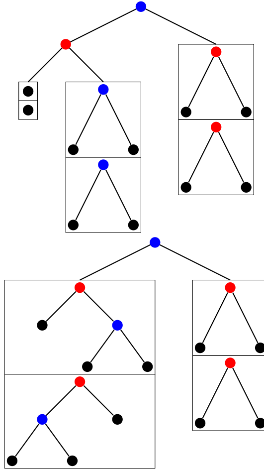
FIGURE 2.6.1. Two consecutive steps of the run of the bottom-up ranked tree transducer of Example 2.6.7 over a tree whose alphabet of node labels is \Sigma = \{\bullet, \bullet\} \cong \{a, b\} .
