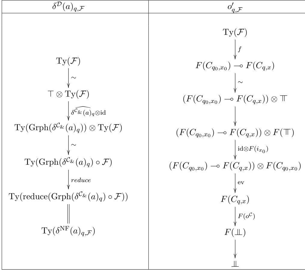
FIGURE 4.8.4. Definition of \delta^{\mathcal{D}}(a)_{q,\mathcal{F}} and o'_{q,\mathcal{F}} .
