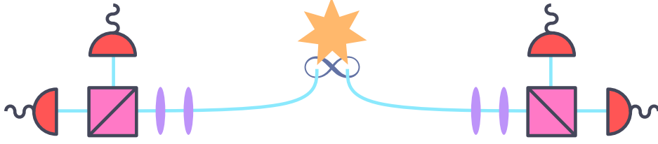
Figure 8.1: SPDC setup. A SPDC source (yellow star) sends photons entangled in polarization (blue lines), with one part sent to Alice and one sent to Bob. Locally, each party disposes of wave plates (purple ellipses) used to choose the measurement basis according to the measurement setting. This is followed by a polarising beamsplitter (pink sliced square) with each of the two outputs measured by NPNR detectors.
