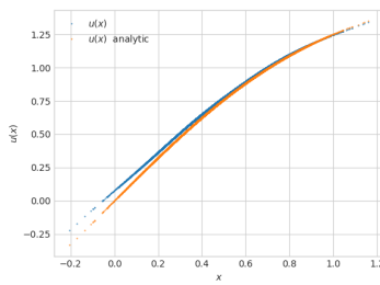
Y at date t = 0.006125 .
