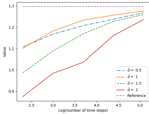
Convergence of D_x u depending on \hat{\sigma}
