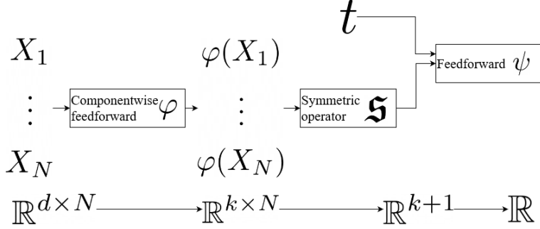
Figure 7.2: Architecture of time dependent symmetric network.
