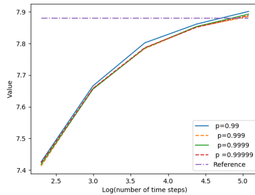
Figure 5.10: Function value convergence in 7D of the linear quadratic case with 2 layers, 100 neurons, testing p , using \hat{\sigma} = 2
