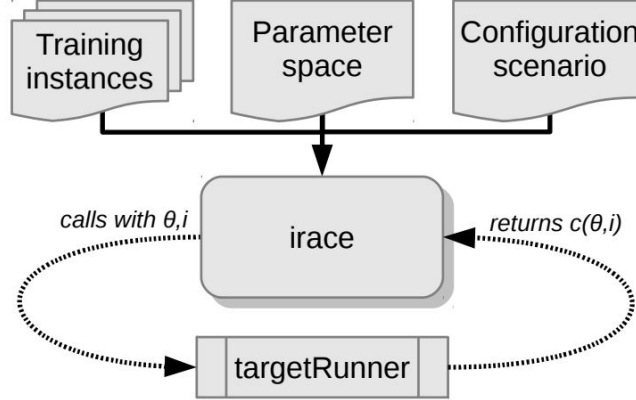
Figure 2.20 Flowchart of irace workflow [94].
