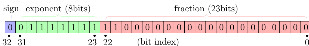
Figure 2.13: IEEE 754 single-precision format on 32 bits
