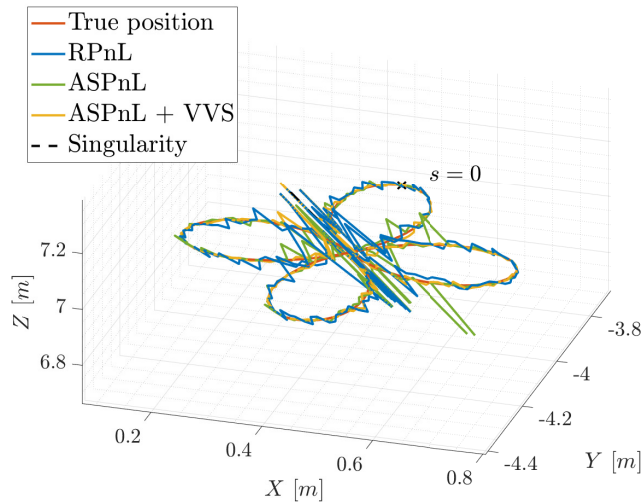
Figure 4.19: Pose computation from RPnL , ASPnL and ASPnL refined by VVS using five image lines along a quadrifolium trajectory centred at a point on the line singularity \mathcal{L}_M . In the proximity of the singularity the error in the estimation grows unbounded.
