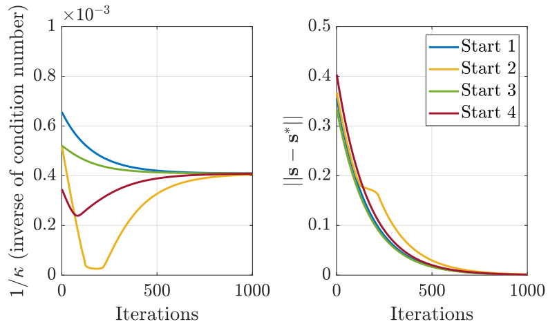
Figure 4.7: Inverse of the condition number \kappa of the interaction matrix \mathbf{M}_{(4)} (left) and norm of the error vector \|\mathbf{s} - \mathbf{s}^*\| (right).
