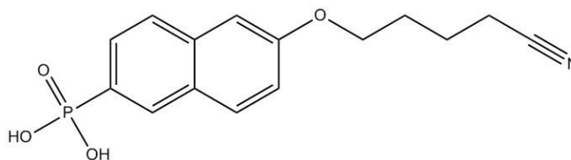
(6-(4-cyanobutoxy)naphtalen-2-yl)phosphonic acid
