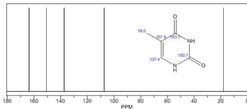
Figure 37: Simulated ^{13}\text{C} NMR of Thymine.
