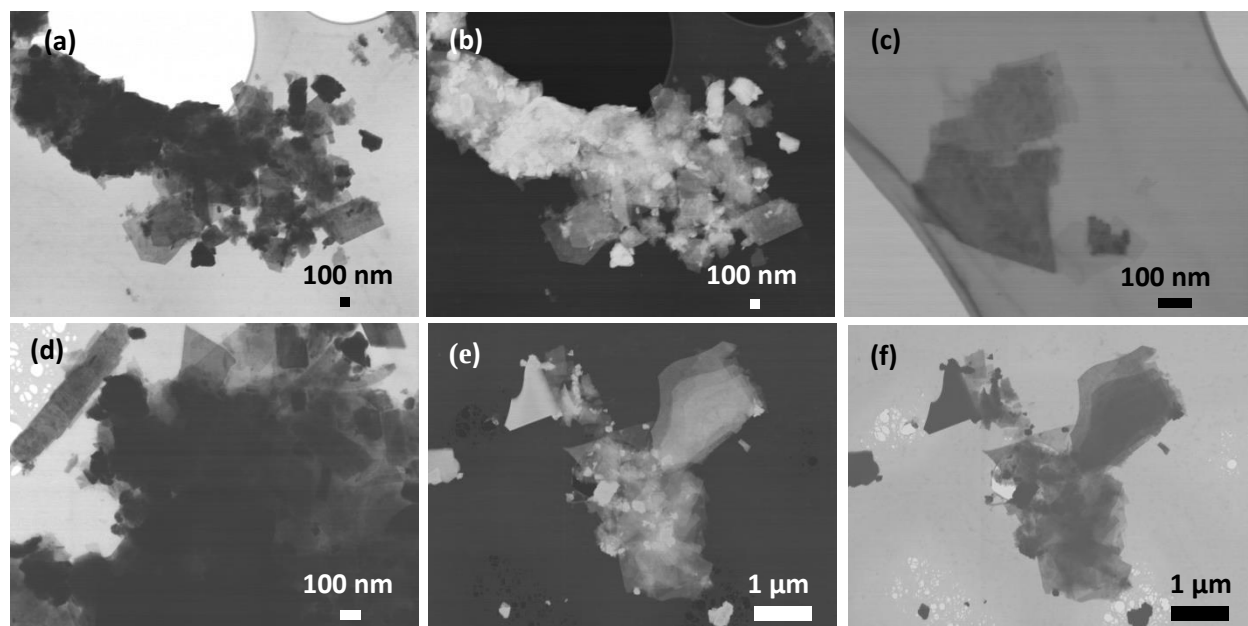
Figure 15: SEM images of (a) to (c) \text{BenzSC}_2\text{O-HST} (d) to (f) \text{C}_{10}\text{PO}_3\text{-HST} nanomaterials resulting from the exfoliation with the PEG600.
