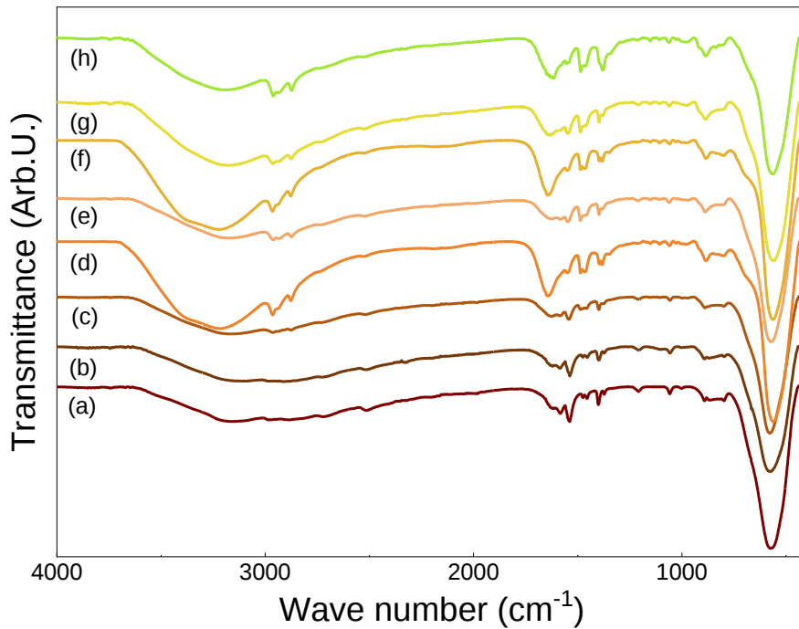
Figure 6: FTIR spectra of (a) \text{C}_2\text{N-HST} and (b) to (h) bottoms from exfoliated \text{C}_2\text{N-HST} solution with a ratio \text{TBA}^+/\text{H}^+ = 0, 0.5, 1, 3, 5, 7, 10 respectively .
