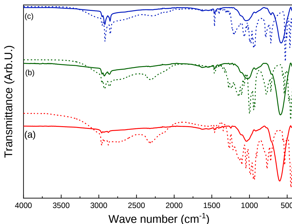
Figure 11 : FTIR spectra of (a) \text{C}_3\text{PO}_3\text{-HST} , (b) \text{C}_6\text{PO}_3\text{-HST} and (c) \text{C}_{10}\text{PO}_3\text{-HST} in solid line and their corresponding molecule 1-propylphosphonic acid, 1-hexylphosphonic acid and 1-decylphosphonic acid in dot line respectively.
