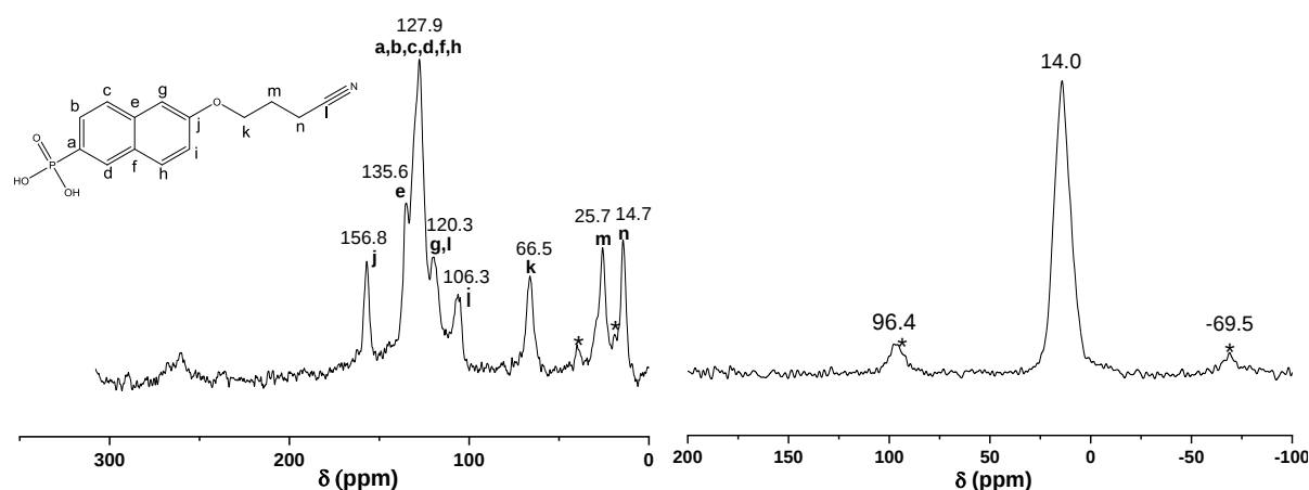
Figure 19: (a) 13 C CP/MAS NMR spectrum and (b) 31 P MAS NMR spectrum of NCaArPO 3 -HST (the signals with asterisks are attributed to spinning sidebands).
