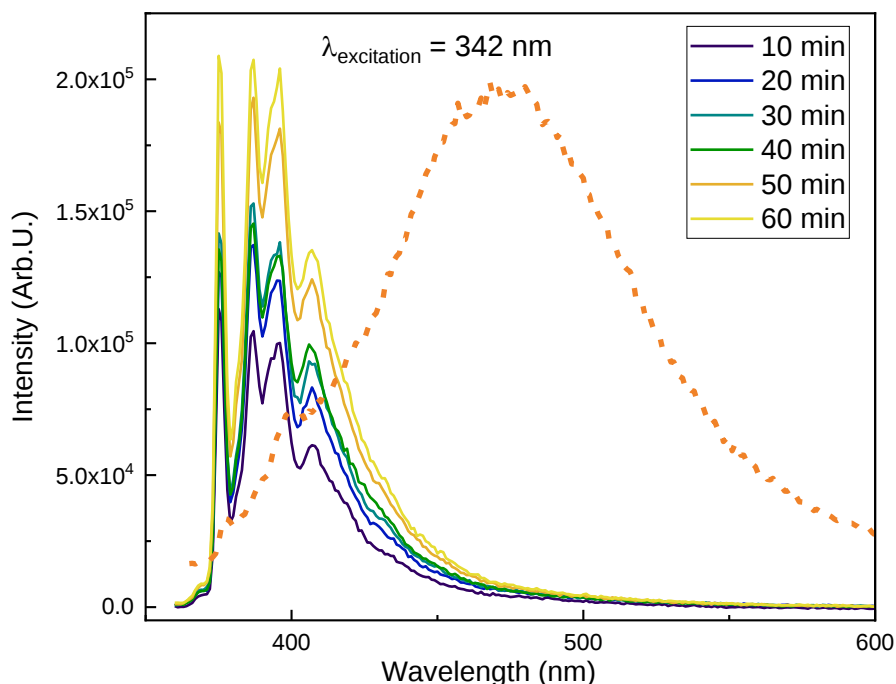
Figure 4: Emission spectra of bulk PyrC 4 O-HST (orange dot line) and suspension of PyrC 4 O-HST over the shear-exfoliation process from 10 minutes to 60 minutes.
