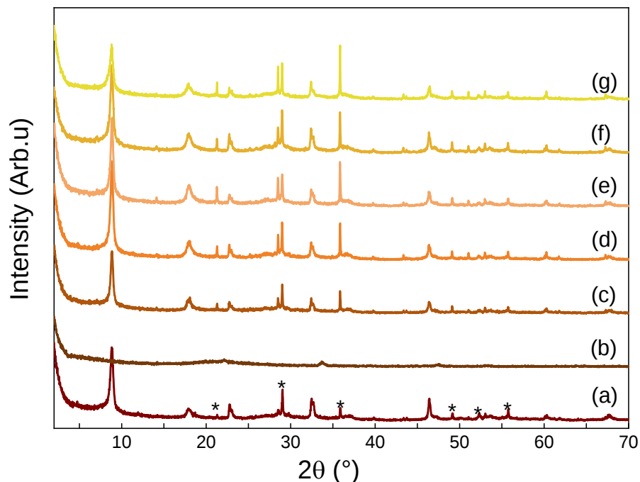
Figure 4: XRD patterns of (a) HST, (b) exfoliated HST from classical ion-exchange mechanism and (c) to (g) bottoms of exfoliated HST solution with a ratio \text{TBA}^+/\text{H}^+ = 0, 1, 3, 5, 10 respectively. Peaks with an asterisk correspond to an impurity of BST, present in the batch of HST for this peculiar set of experiments.
