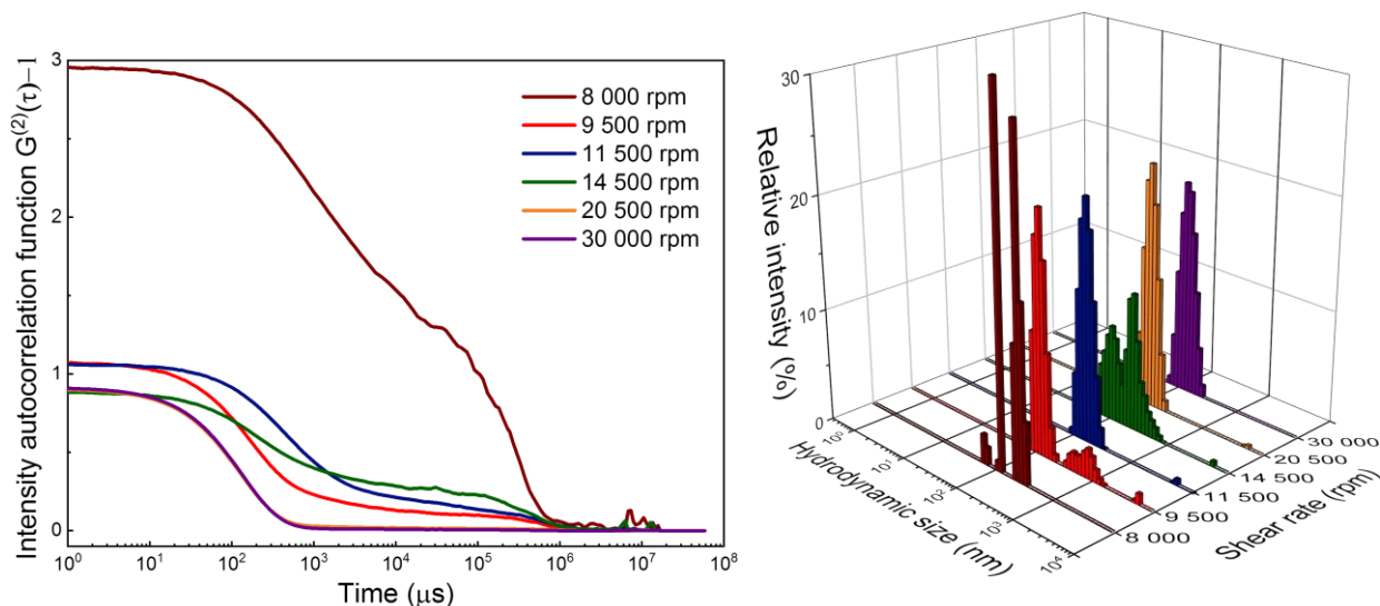
Figure 5: (Left) Intensity auto-correlation functions from suspension of exfoliated C_{12}O -HST in acetonitrile, obtained after exfoliation at different shear rates and (right) their corresponding size distribution determined using the Zetasizer.
