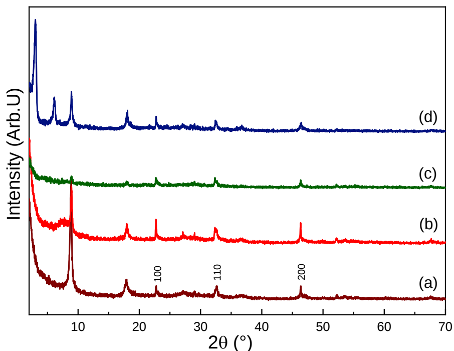
Figure 16: XRD patterns of bottoms of (a) C_4N -HST, (b) C_{12}O -HST, (c) BenSC_2O -HST and (d) C_{10}PO_3 -HST after exfoliation with PEGN5000.
