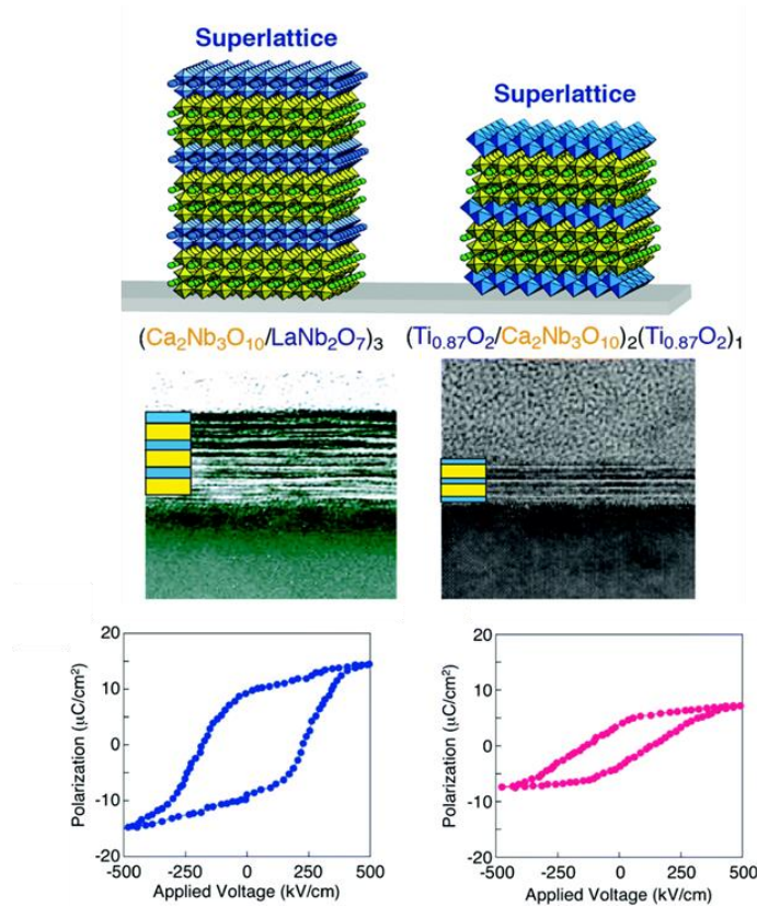
Figure 6: Two alternate structures composed of distinct charged oxide nanosheets. The two architectures display artificial ferroelectric behavior. 123
