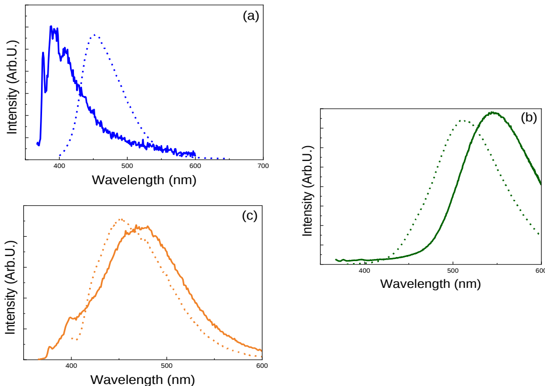
Figure 2: Emission spectra of (a) PyrO-HST, (b) PyrC 1 O-HST and (c) PyrC 4 O-HST (solid line) and their corresponding molecules (dot line) ( \lambda_{\text{excitation}} = 320 \text{ nm} ).
