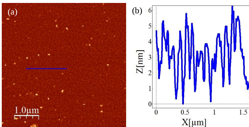
Figure 10: (a) AFM image of MPTS-HST nanosheets, deposited on a gold substrate. (b) Z-profile of the bare substrate, showing its roughness.
