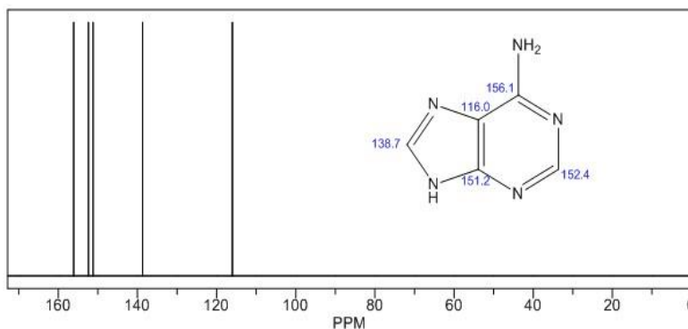
Figure 35: Simulated ^{13}\text{C} NMR spectrum of Adenine.
