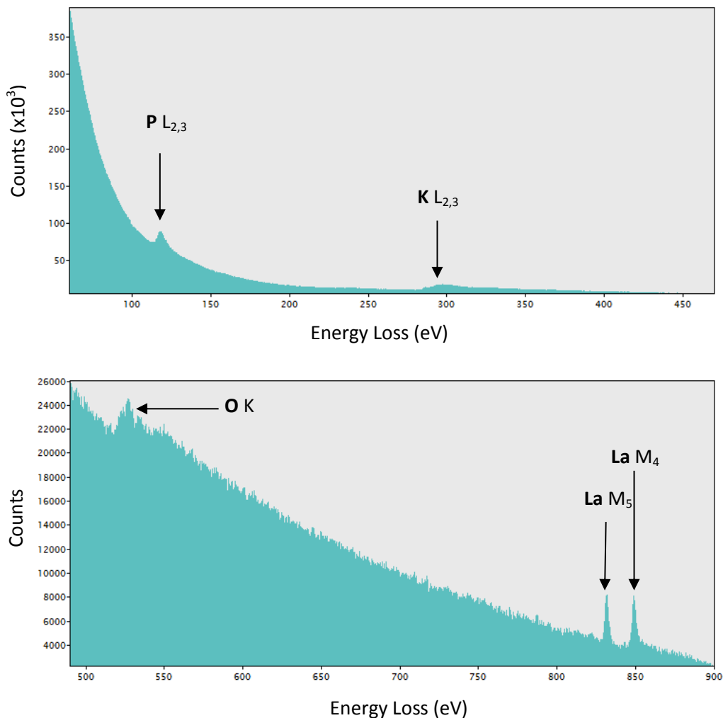
Figure 9: EELS spectrum of \text{C}_{10}\text{PO}_3\text{-HLN} nanosheets, obtained at 200 kV.
