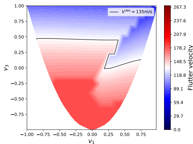
(d) Minimum critical velocity of the three first modes
