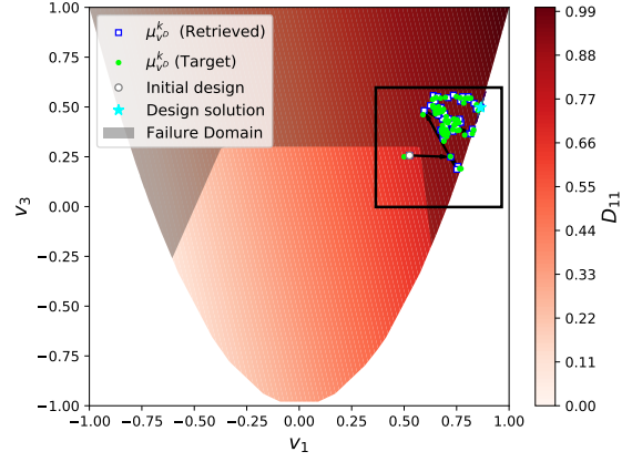
(b) Optimization path of the squared initial design from Figure 4.7a.
