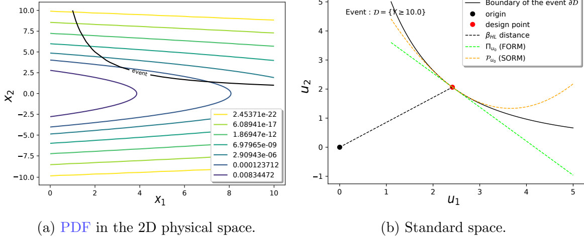
Figure 3.3: Schematic representation of FORM and SORM approximations with the mapping from the physical to the standard space.
