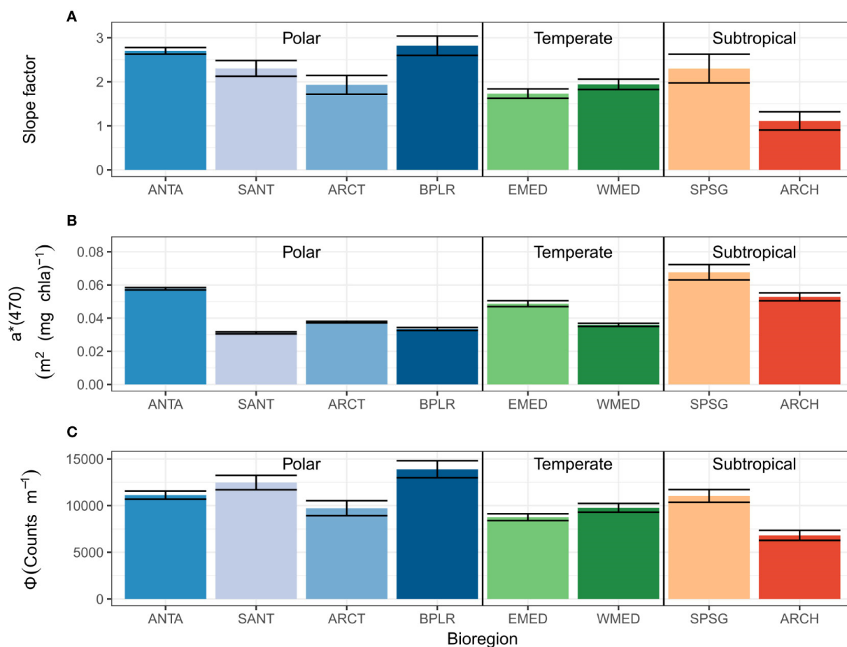
Figure 3.8: (A) Distribution of the slope factor, defined as the coefficient of the regression between [Chla]_{Fluo} and [Chla]_{HPLC} , (B) Chla -specific absorption coefficient at 470 nm, a^*(470) ( m^2(mg\ Chla)^{-1} ), and (C) fluorescence quantum yield, \Phi (counts m^{-1} ), for the eight bioregions of the Glo-Argo dataset (ANTA, Antarctic Province; ARCH, Archipelagic Deep Basin Province; ARCT, Atlantic arctic Province; BPLR, Boreal Polar Province; EMED, Eastern Mediterranean Sea; SANT, Subantarctic Province; SPSG, South Pacific Subtropical Gyre Province; WMED, Western Mediterranean Sea). The error bars indicate 95% confidence limits.
