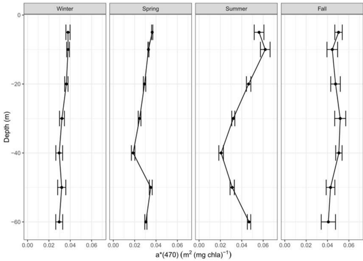
Figure 3.6: Vertical distribution of the phytoplankton chlorophyll-specific absorption coefficient at 470 nm, a^*(470) in \text{m}^2 (\text{mg Chla})^{-1} , for each season and sampling depth of the Med-Bouss dataset.
