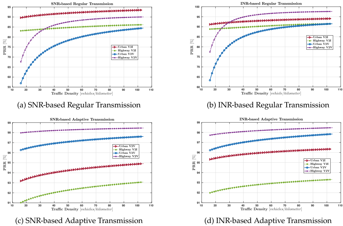
Figure 5.12: Packet Reception Ratio
