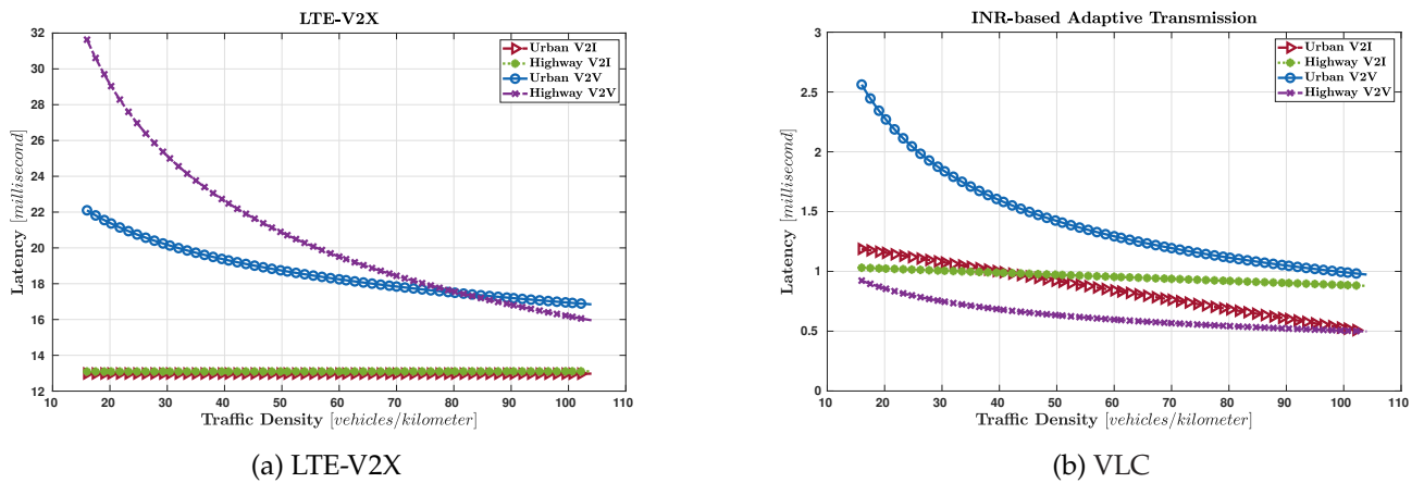
Figure 5.14: Latency
