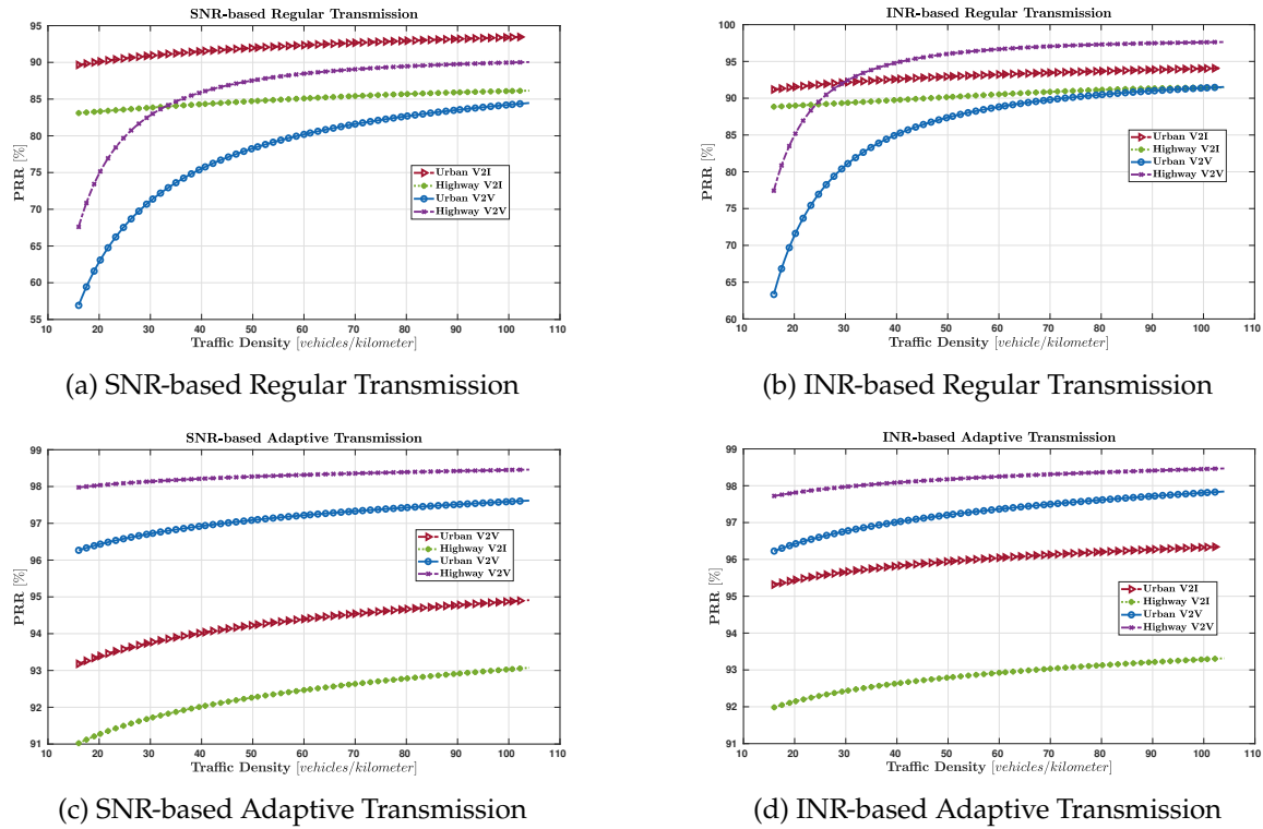
Figure 5.12: Packet Reception Ratio
