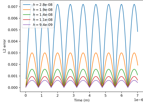
Figure 4.32: Evolution of the relative error \mathfrak{E}_{J,rel} for increasing mesh refinement in the ideal case \mathbf{E} = \tilde{\mathbf{E}} .
