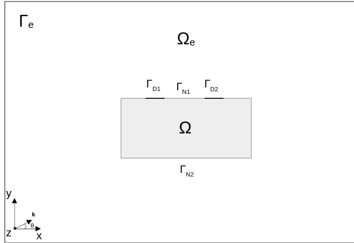
Figure 2.2: A two-dimensional representation of the original semiconductor domain \Omega immersed in a bounded dielectric domain \Omega_e and subject to an incident field – typically a plane wave of vector \mathbf{k} forming an angle \theta with the x axis.
