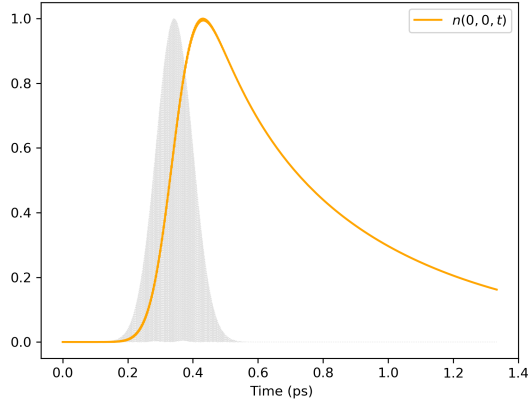
Figure 5.16: The evolution of generation and electron concentration throughout the simulation window t \in [0, t_f] , observed at the center of the semiconductor (x, y) = (0, 0) .
