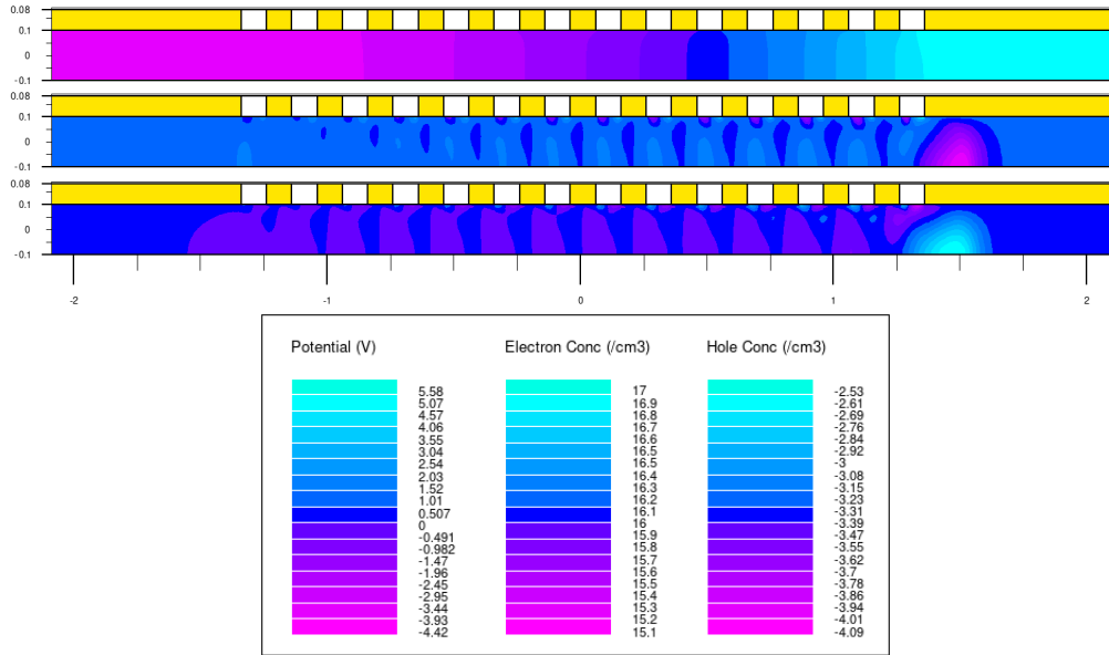
Figure 5.25: From the top to the bottom: the electrostatic potential (linear scale), electron concentration (logarithmic scale), hole concentration (logarithmic scale) calculated in Atlas.
