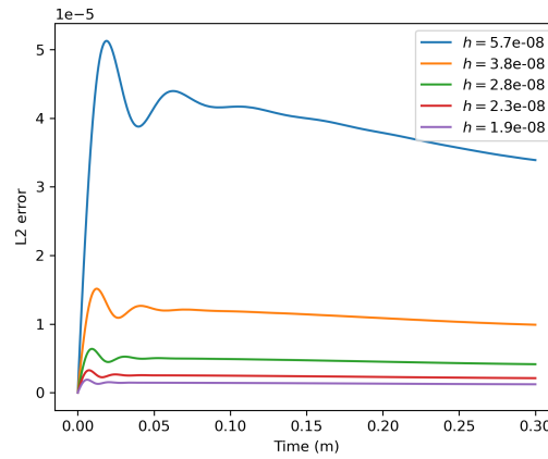
Figure 4.19: Evolution of \mathfrak{E}_{EM} in the considered meshes – RK2, \mathcal{P}_2
