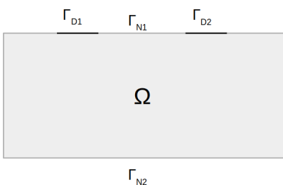
Figure 2.1: A two-dimensional bounded semiconductor domain \Omega with \partial\Omega = \Gamma_D \cup \Gamma_N , \Gamma_D = \Gamma_{D1} \cup \Gamma_{D2} representing metal contacts ideally connected to a voltage source, \Gamma_N = \Gamma_{N1} \cup \Gamma_{N2} representing electrically insulating boundaries.
