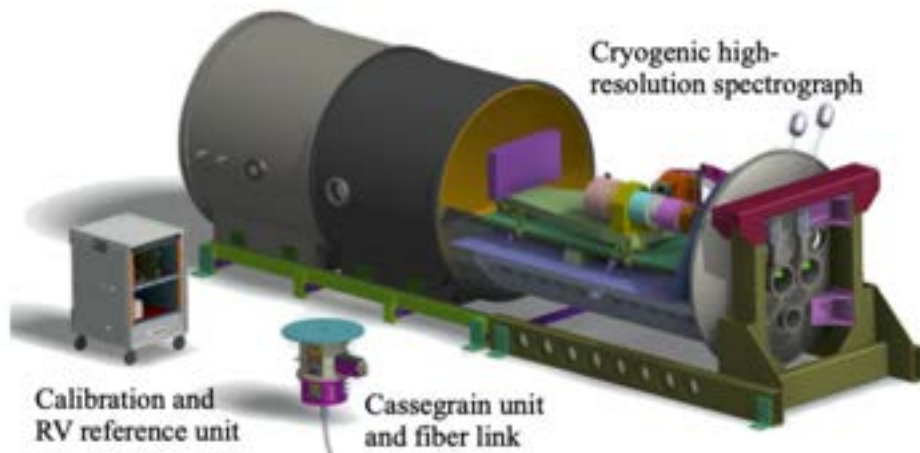
FIGURE 1.4. Computer aided design of SPIRou, taken from Donati et al. (2020) .
