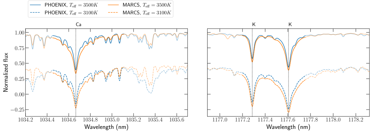
FIGURE 4.9. Comparison between line profiles computed from PHOENIX (blue) and MARCS (orange) model atmospheres. In each panel, models are plotted for two temperatures: 3100 K (dashed lines) and 3500 K (solid lines). The regions selected for our analysis are plotted in bold. For all models, the values of \log g and [M/H] are fixed to 5.0 dex and 0.0 dex respectively.
