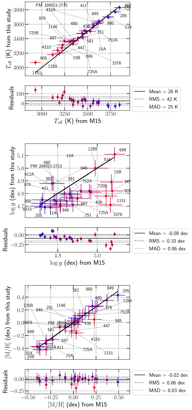
Figure A2. Same as Fig. 4 with labels identifying the stars.
