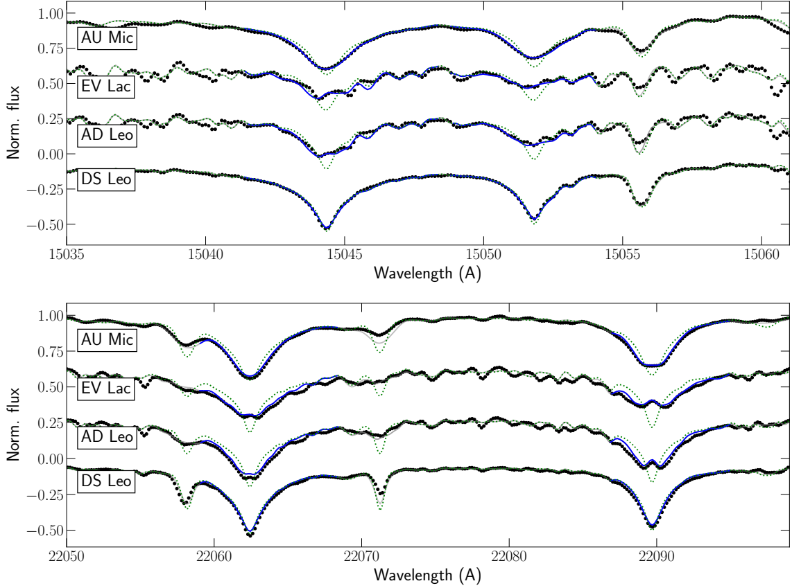
FIGURE 6.12. Best fit obtained for AU Mic, EV Lac, AD Leo and DS Leo with ZeeTurbo for two Mg lines (15044.3 & 15051.8 Å), and two Na lines (22062.4 & 22089.7 Å). Black points present the data. The gray solid line shows the best fit, and the blue solid blue line presents the part of the windows used for the fit. The green dotted line shows the model obtained for the same atmospheric parameters but with a zero magnetic field.
