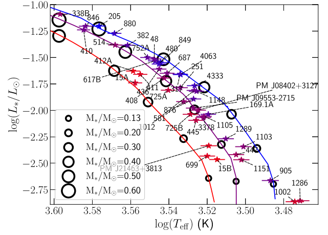
Figure A4. Same as Fig. 7 with labels identifying the stars.
