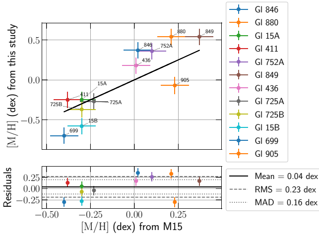
Figure 11. Same as Fig. 10 but for [M/H] .
