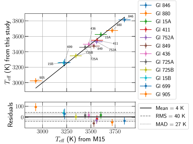
Figure 10. Retrieved T_{\text{eff}} using the grid of PHOENIX (left-hand panel) and MARCS (right-hand panel) spectra plotted against values published by M15. The bottom plot presents the residuals, i.e. the retrieved values minus literature values. RMS and MAD values are computed after application of a sigma clipping function on the residuals with a threshold at 5\sigma .
