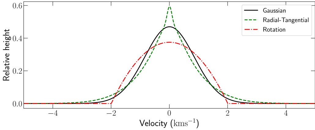
FIGURE 3.3. Comparison between the broadening kernels typically considered. All profiles were normalized. A value of 2 \text{ km s}^{-1} was assumed for the rotation velocity, radial-tangential macroturbulent velocity and for the full width at half maximum of the Gaussian profile.
