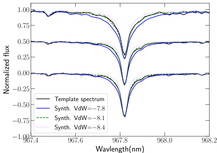
FIGURE 5.7. Effect of the Van der Waals parameters on the line shape. The spectra of our 3 references stars are displayed (GI 699, GI 15A, GI 411 from top to bottom), with the associated models computed for different values of the Van der Waals parameters.
