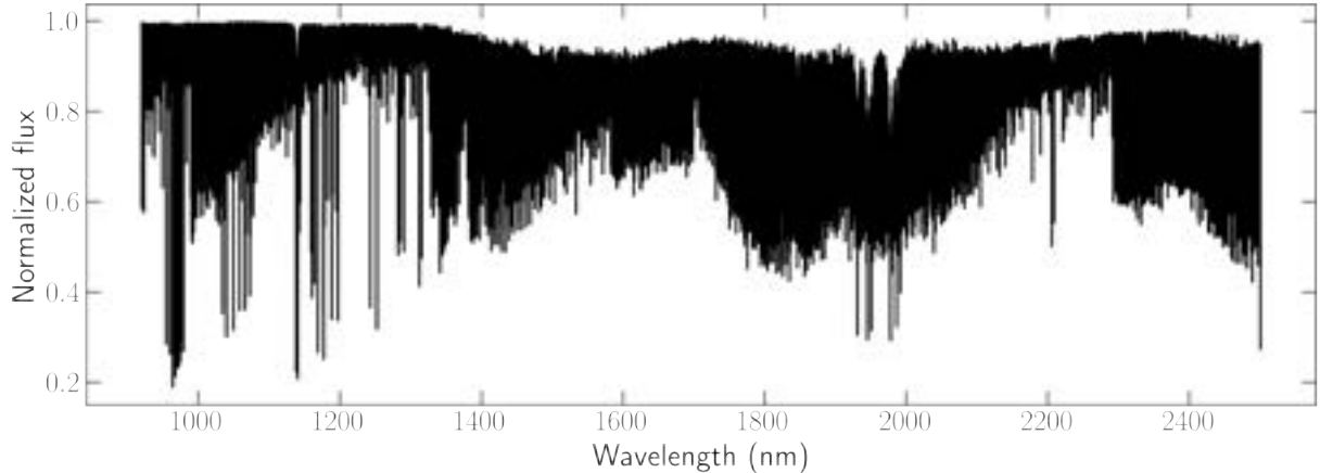
FIGURE 4.2. Example for normalized spectrum computed with Turbospectrum from a MARCS model atmosphere for the full SPIRou wavelength range. This model was computed for T_{\text{eff}} = 3200 K, \log g = 5.0 dex and [M/H] = -0.5 dex.
