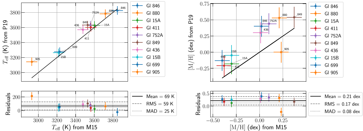
Figure 2. Comparison between parameters published by P19 (using near-infrared regions only) and M15. Top plots present the values retrieved by P19 plotted against the values retrieved by M15 for effective temperature (left-hand panel) and metallicity (right-hand panel). Bottom plots present the residuals, i.e. values retrieved by P19 minus values retrieved by M15. We additionally display the mean value, standard deviation, and median absolute deviation of the residuals.
