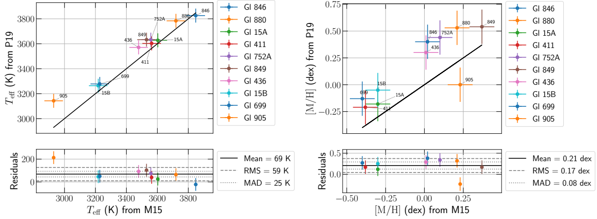
FIGURE 4.14. Same as Fig. 4.13 comparing results reported by Passegger et al. (2019) (P19) and Mann et al. (2015) (M15).
