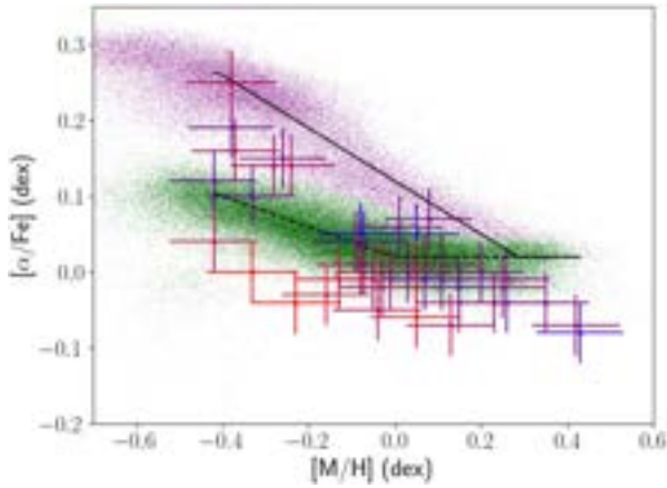
Figure 5. Retrieved [\alpha/\text{Fe}] plotted against [\text{M}/\text{H}] for the 44 targets in our sample. The solid and dashed black lines mark empirical thick and thin disc [\text{M}/\text{H}]-[\alpha/\text{Fe}] relations, respectively. The coloured pixels mark the position of giants studied by APOGEE, with the purple and green colours marking those expected to be from the thick and thin disc, respectively. An alternative figure with labels identifying the stars is presented in Fig. A3.
