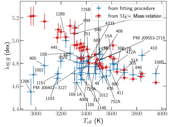
Figure A6. Same as Fig. 9 with labels identifying the stars.
