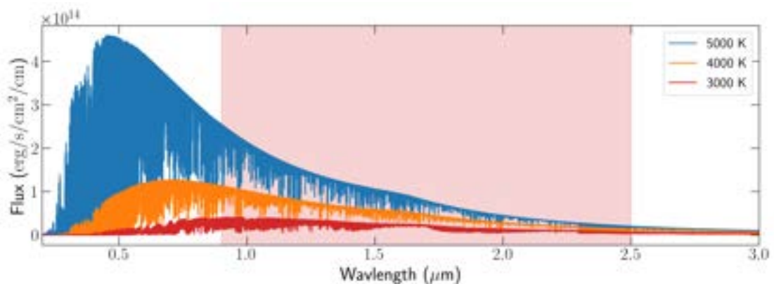
FIGURE 1.3. PHOENIX-ACES synthetic spectra (see Sec. 3.3) for 3 effective temperatures. The red band marks the wavelength domain covered by SPIRou.
