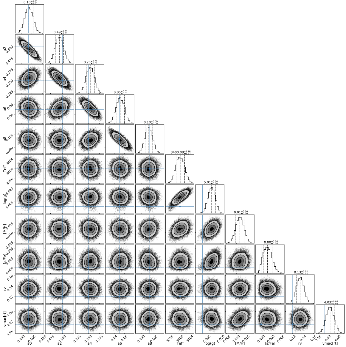
FIGURE 6.7. Corner plots showing the posterior distribution on all fitted parameters. The input parameters are located by the blue lines.
