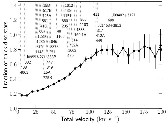
FIGURE 5.4. Fraction of thick disk stars per velocity bin estimated from APOGEE data for giants. The position of each target in our sample is marked on the horizontal axis.
