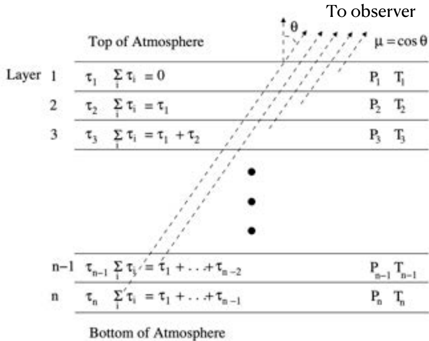
FIGURE 3.1. Schematic representation of a plane parallel atmosphere. Adapted from Dr. Brigitte Emily Hesman's PhD thesis.
