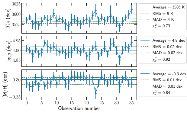
Figure 14. Optimal estimates and corresponding error bars retrieved for a series of SPIRou spectra of Gl 411. The mean value, standard deviation, and median absolute deviation are indicated for each series. We also compute the reduced \chi^2 to the mean value of each series.
