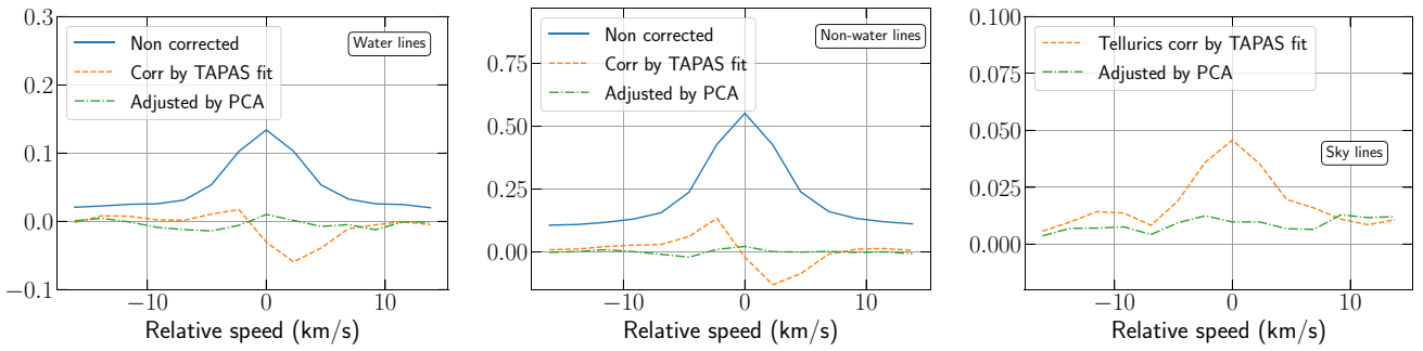
Figure 4. Left-hand panel: cross-correlation profile computed between the residuals for one of our G1 699 spectra and a mask of water absorption lines. Middle: same as left-hand panel but with a mask containing lines for all the telluric absorbers but water. Right-hand panel: same as left-hand panel but with a mask containing OH emission lines.
