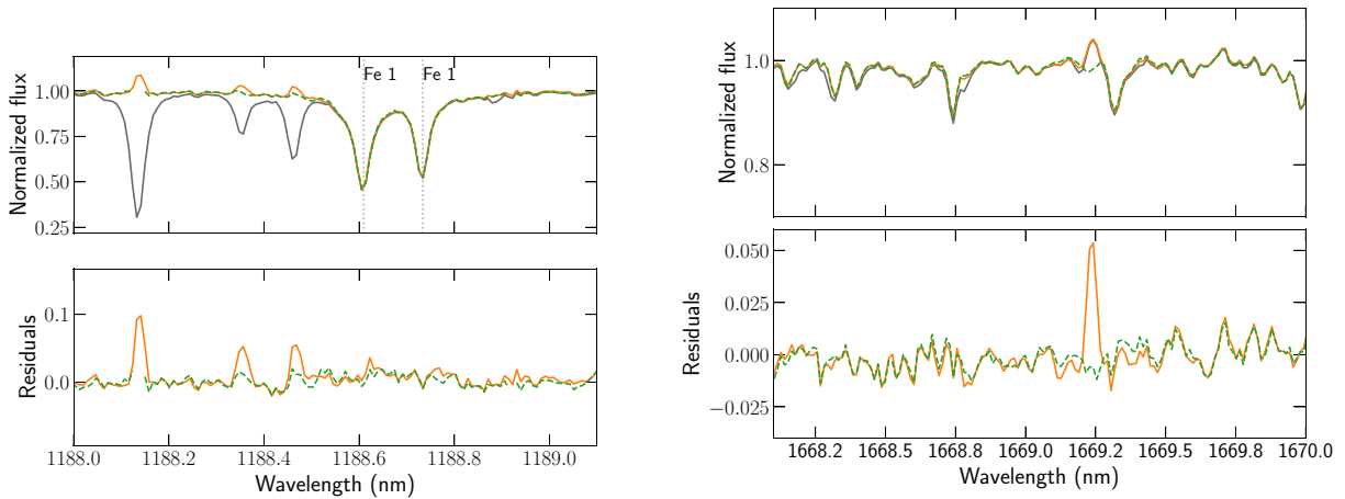
Figure 5. Examples of one of our G1 15A spectra before and after correction of telluric and sky lines, the left-hand and right-hand panels showing examples of telluric and sky line correction, respectively. Top panel: The uncorrected spectrum (grey) features telluric lines approximately removed following the TAPAS correction (orange). Applying PCA on the residuals yields an improved correction (green). Spectral points with telluric absorption larger than 60 per cent of the local continuum (like those around 1188.14 nm) are excluded prior to applying PCA, to optimize correction on the weak to medium-strength telluric features. Bottom panel: Corresponding residuals before (orange) and after (green) applying PCA.
