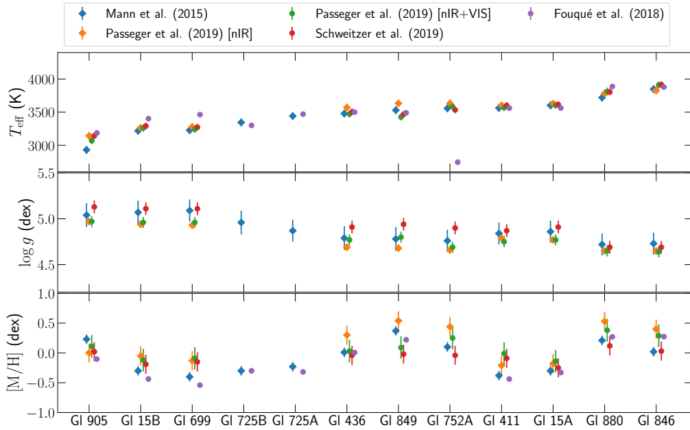
FIGURE 4.1. Parameters reported by several studies ( Mann et al., 2015 ; Fouqué et al., 2018 ; Passegger et al., 2019 ; Schweitzer et al., 2019 ) for 12 M dwarfs observed in the context of the SLS.
