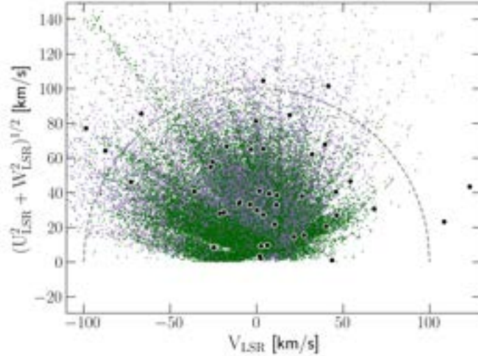
FIGURE 5.3. Toomre diagram for the giants studied with APOGEE. Green points presents \alpha -poor thin disk stars, while the purple points present \alpha -rich thick disk stars. Black dots present the position of the 44 M dwarfs included in our sample (see Fig. A1 of Cristofari et al., 2022b, for a figure with the star names). The dashed circle marks the fiducial boundary at 100 \text{ km s}^{-1} .
