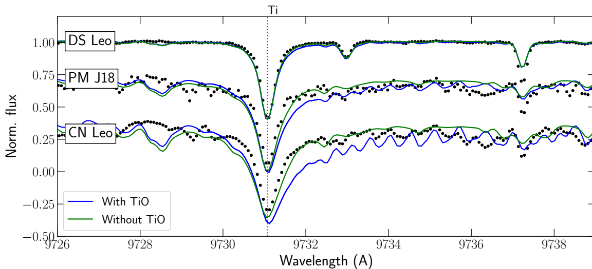
Figure 5. Best obtained fit with synthetic spectra computed with and without TiO for the two coolest stars in our sample (CN Leo and PM J18482+0741) and DS Leo. The black points show the SPIRou templates.
