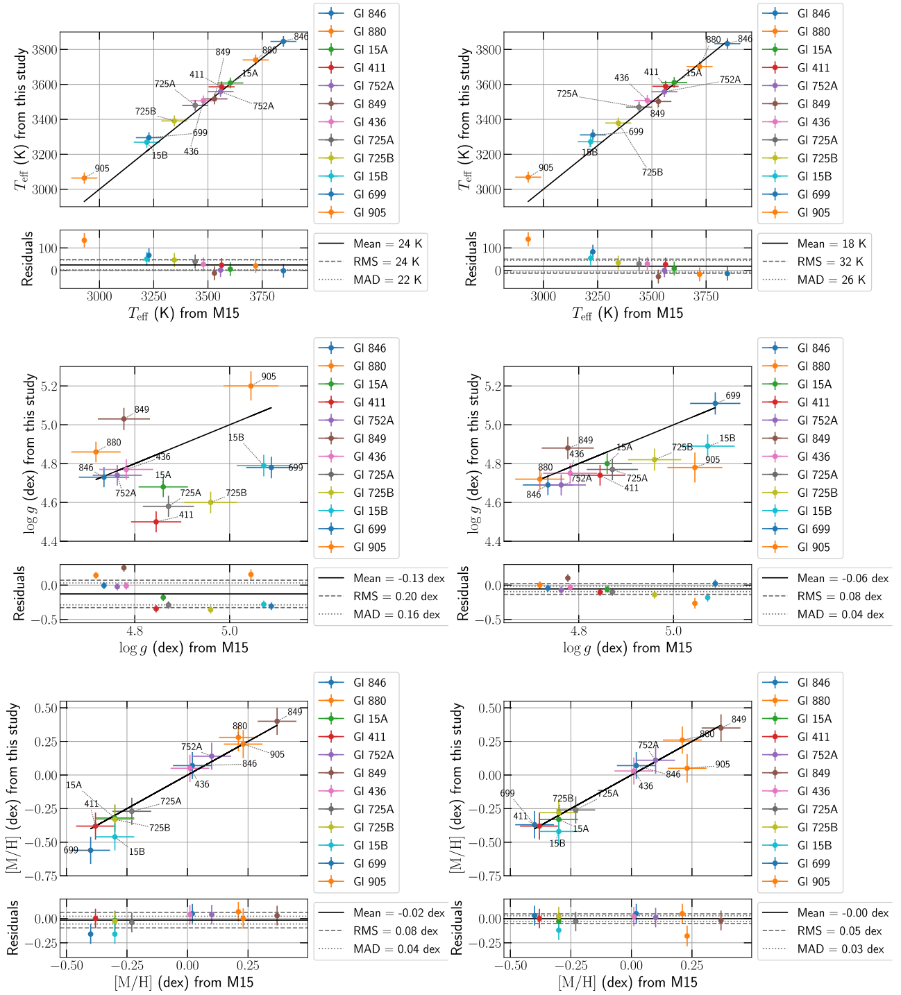
Figure B3. Same as Fig. B1 but comparing the results obtained with [\alpha/Fe] = 0 dex (left-hand panels) and while fitting [\alpha/Fe] (right-hand panels). These results are obtained with corrections of the line list described in Section 5.
