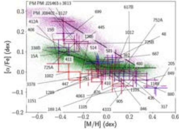
Figure A3. Same as Fig. 5 with labels identifying the stars.
