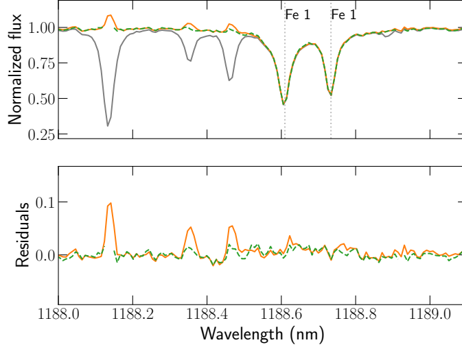
FIGURE 2.6. Example of correction for one of G1 15A spectrum before and after correction of the telluric and sky lines. Top panel: The uncorrected spectrum (grey) features telluric lines removed following the TAPAS-based correction (orange). The PCA adjusted correction is shown in green. Telluric lines with absorption larger than 60 % are excluded prior to applying the PCA. Bottom panel: Corresponding residuals before (orange) and after (green) applying PCA.
