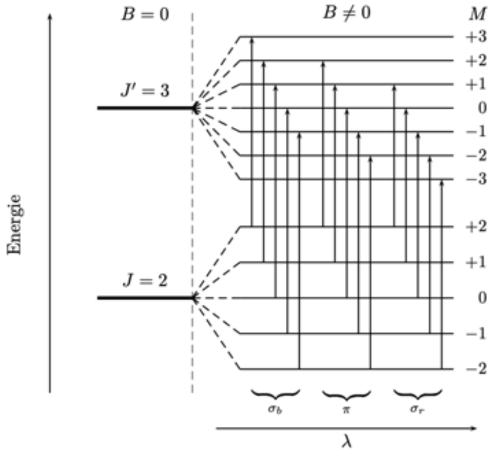
FIGURE 6.1. Splitting of energy levels within a magnetic field. Taken from Dr. Julien Morin's PhD thesis ( http://thesesups.ups-tlse.fr/816/ ). The resulting line profile is illustrated in Fig. 6.2.
