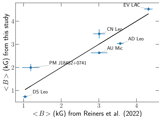
Figure 9. Comparison between our derived \langle B \rangle values and those of Reiners et al. (2022). The black line marks the equality
