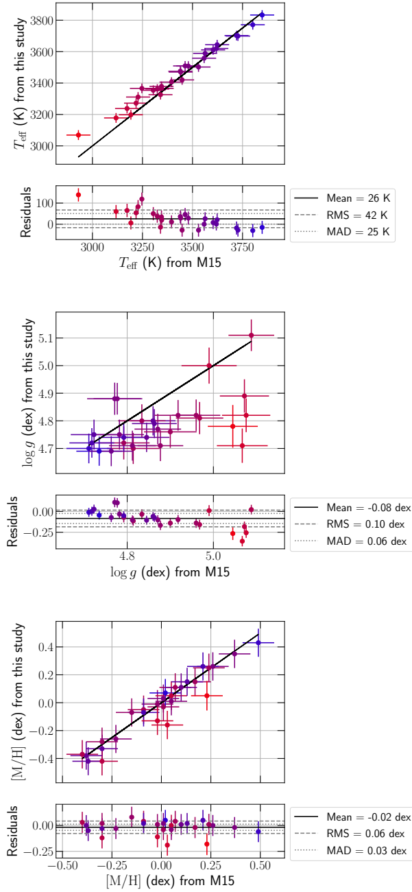
FIGURE 5.8. Retrieved parameters of our stellar sample plotted against those of Mann et al. (2015, M15). The color of the points codes the temperature from cold (red) to hot (blue). The bottom plots show the residuals with the associated average value, RMS and median absolute deviation (MAD).
