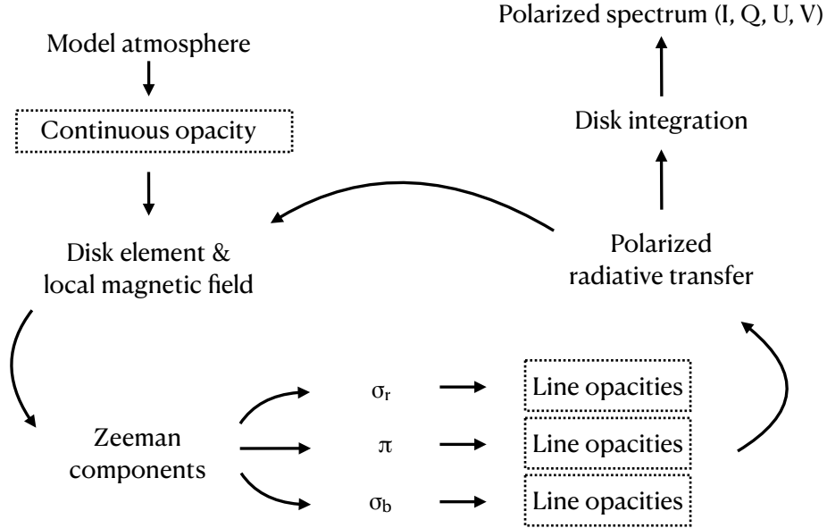
FIGURE 6.4. ZeeTurbo schematic. The dashed boxes indicate the Turbospectrum routines.
