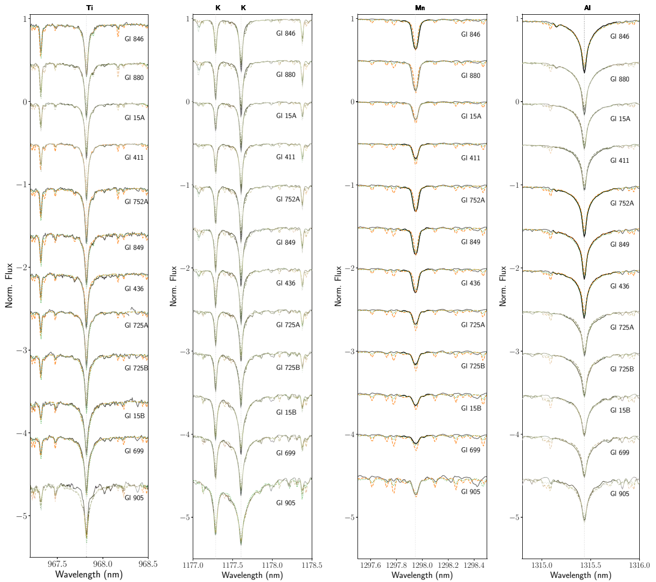
Figure A1. Template spectra (grey) along with the fitted PHOENIX model (dashed orange) and MARCS model (dotted green) for four spectral windows. Selected regions of the template spectra over which the comparison was carried out are shown in black. From top to bottom: GI 846, GI 880, GI 15A, GI 411, GI 752A, GI 849, GI 436, GI 725A, GI 725B, GI 15B, GI 699, and GI 905. Every spectrum but the first one is shifted by a multiple of 0.5 for better readability. Fig. A2 (available as supplementary material) shows all the spectral windows used for the analysis.
