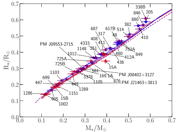
Figure A5. Same as Fig. 8 with labels identifying the stars.
