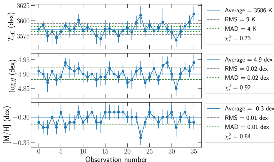
FIGURE 4.12. Optimal estimates and corresponding formal error bars retrieved for a series spectra of Gl 411. For each parameter we display the average, RMS, median absolute deviation(MAD) and \chi^2 on the series of points.
