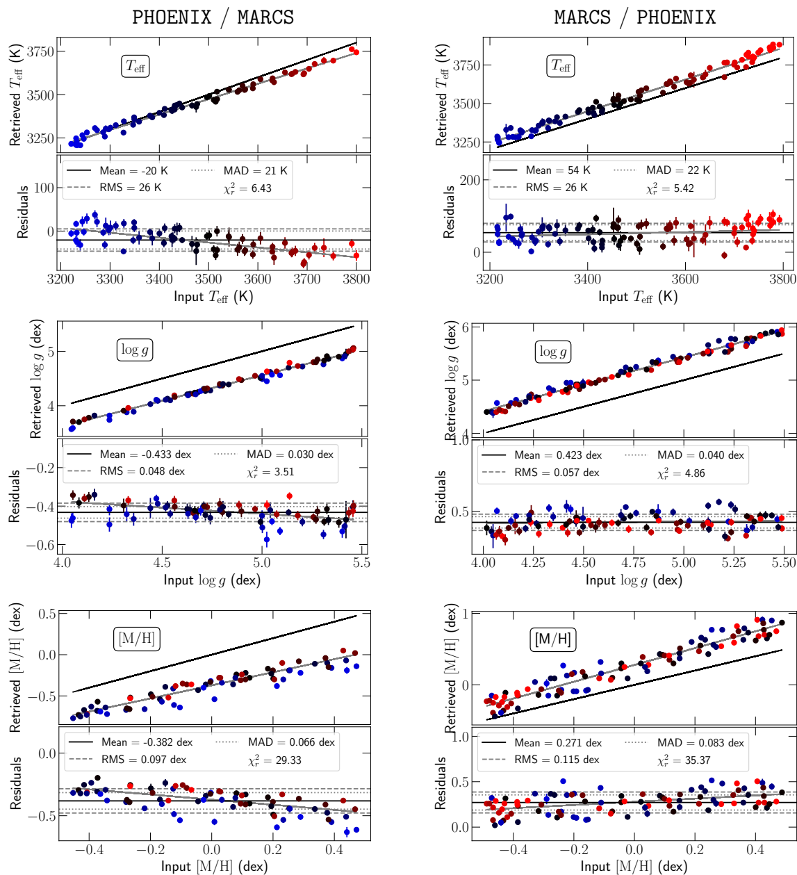
FIGURE 4.8. Same as Fig. 4.7 but using the PHOENIX models to generate input models analyzed with the grid of MARCS spectra (left), and using the MARCS models to generate input models analyzed with the grid of PHOENIX spectra (right).
