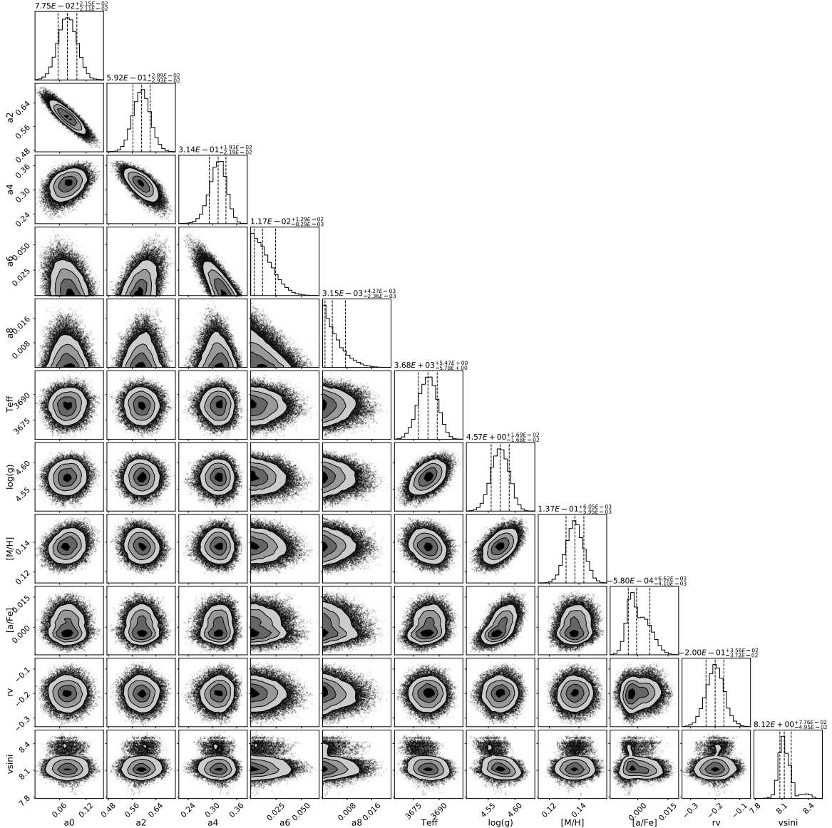
FIGURE 6.10. Same as Fig. 6.7 for AU Mic
