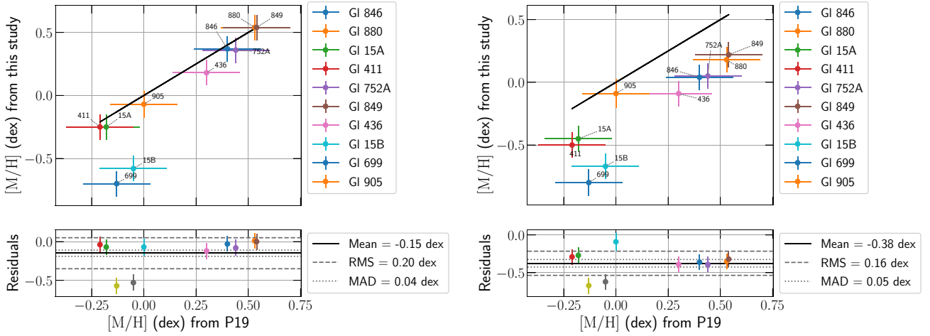
Figure B3. Same as Fig. 10 but for [M/H] .
