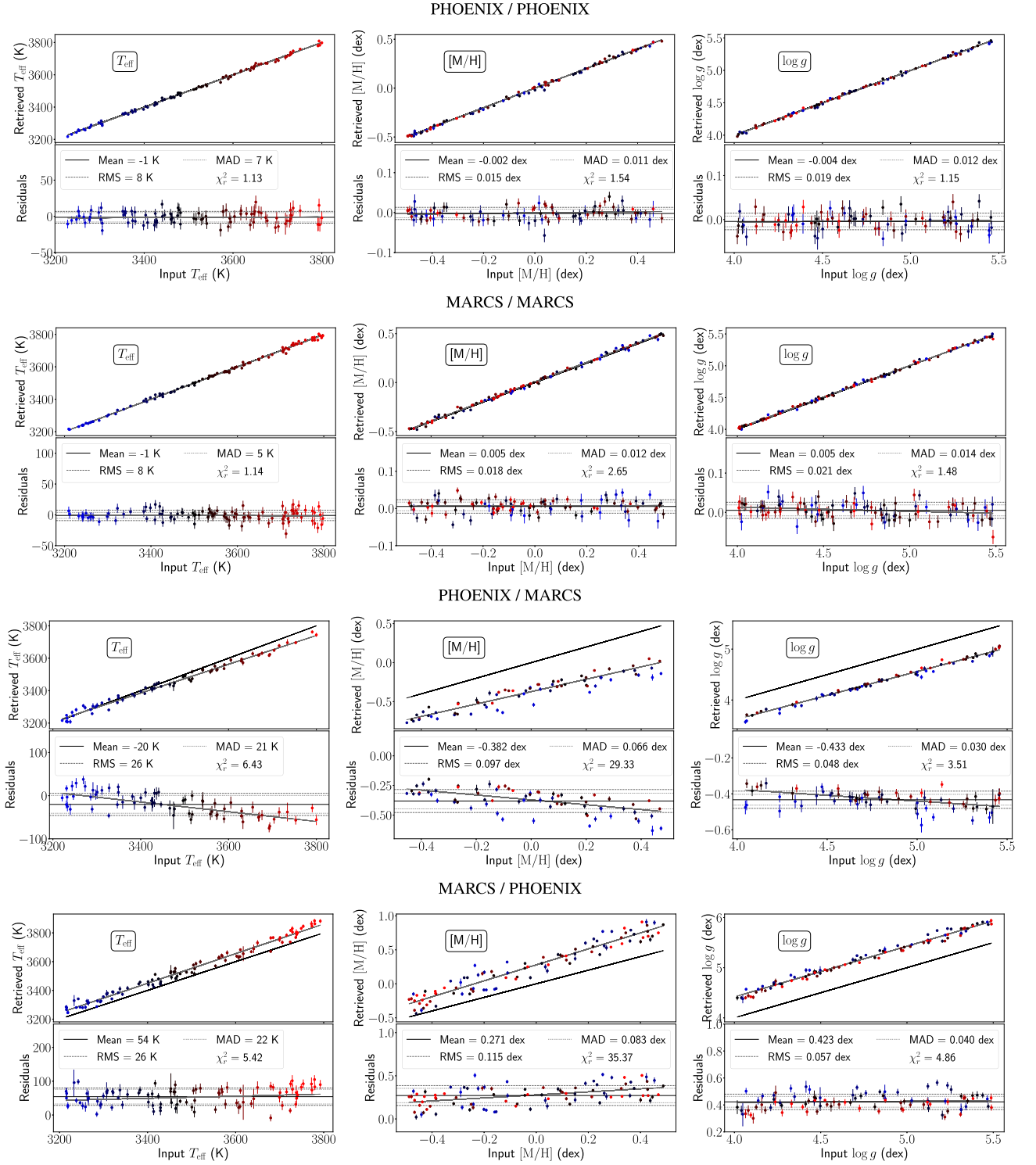
Figure 9. Simulations of parameters determination. The recovered T_{\text{eff}} , \log g , and [M/H] are plotted against the values used to generate the model spectra. The black solid line marks the equality, and a grey solid line is the result of the linear fit performed on the data points. The coefficients and intercepts of the fits are reported in Table 5. All data points are colour coded as a function of T_{\text{eff}} , blue corresponding to the smallest temperature (3200 K), red to the highest temperature (3800 K), and black corresponding to the median T_{\text{eff}} of 3500 K. RMS and MAD values are given with respect to the average of the residuals. The models are generated either from PHOENIX (first and third rows) or MARCS (second and fourth rows) synthetic spectra, which parameters chosen randomly, and a Gaussian noise is added to simulate an SNR of \sim 100 in the H -band, accounting for both the blaze function in each order and the SPIRou throughput. For each model the analysis was performed with either the PHOENIX or MARCS grid of synthetic spectra.
