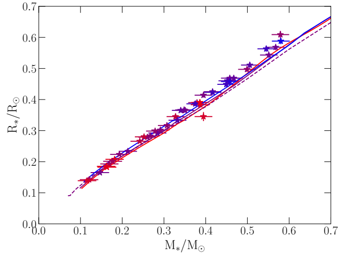
FIGURE 5.12. Comparison between our estimated masses and mass – radius relations derived from evolutionary models. The color of the points codes the temperature from coldest (red) to hottest (blue). The red, purple and blue solid lines present the relations predicted by the DSEP models for [M/H] = -0.5 dex, [M/H] = 0.0 dex and [M/H] = +0.5 dex respectively. The dashed purple line presents the relation computed by the models of Baraffe et al. (2015) at solar metallicity.
