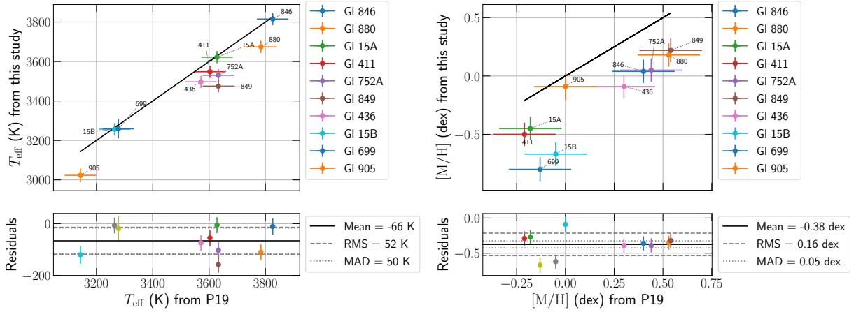
FIGURE 4.13. Comparison between our retrieved T_{\text{eff}} (left panel) and [M/H] (right panel) to those reported by Passegger et al. (2019) (P19). The solid black line marks the equality. The bottom panels show the residuals.
