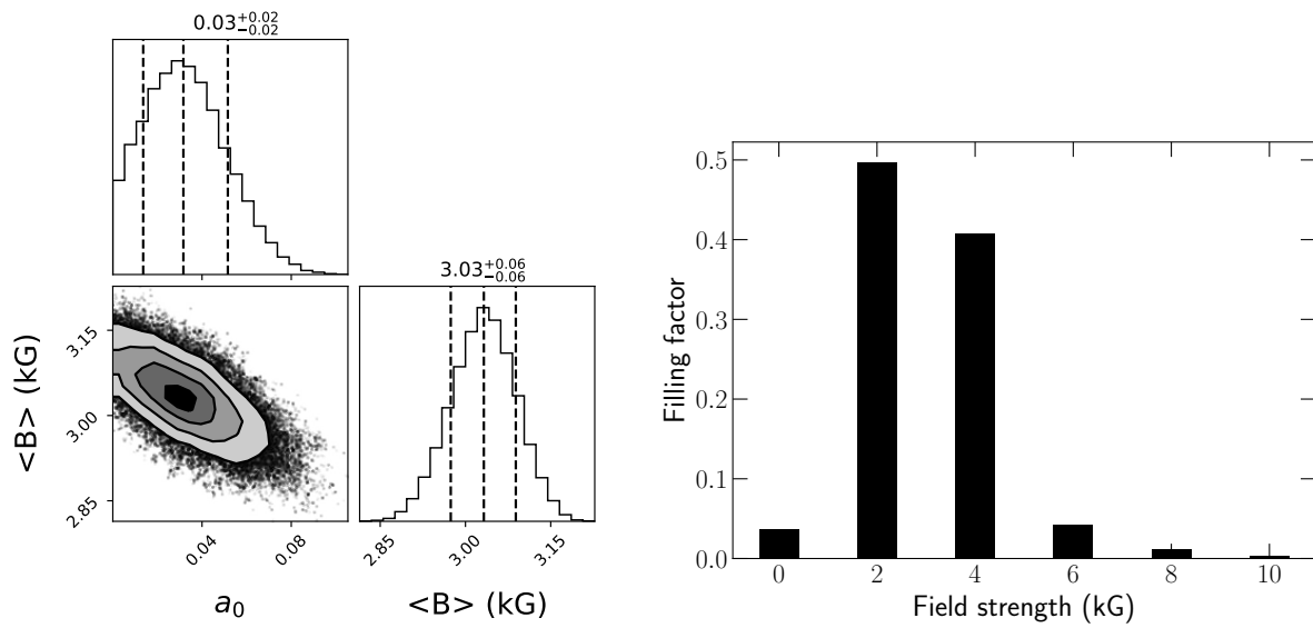
Figure A2. Same as 8 for AD Leo.
