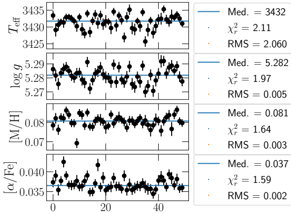
Figure 4. Same as Fig. 3 but with no magnetic field considered for the analysis.
