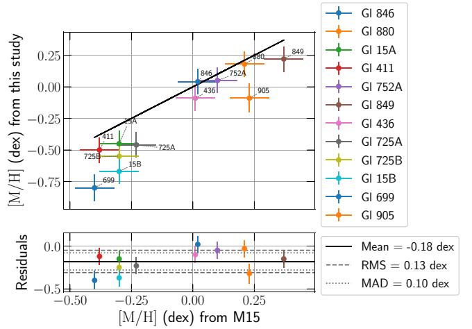
Figure 11. Same as Fig. 10 but for [M/H] .
