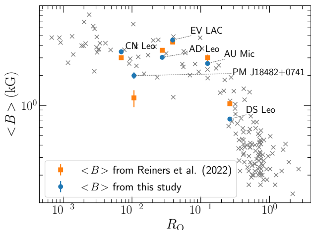
Figure 10. Comparison Rossby number ( R_O ) and \langle B \rangle values derived from our study (blue dots) and reported by Reiners et al. (2022, orange squares). The grey symbols mark the position of all the stars studied by Reiners et al. (2022).
