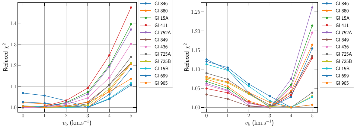
Figure 13. Reduced \chi^2 as a function of the FWHM of the considered Gaussian profile, v_b , obtained with the grid of PHOENIX (left-hand panel) and MARCS (right-hand panel) synthetic spectra, for each target of our sample. The reduced \chi^2 for each star are rescaled to the minimum value reached over the range of v_b , to ease comparison.
