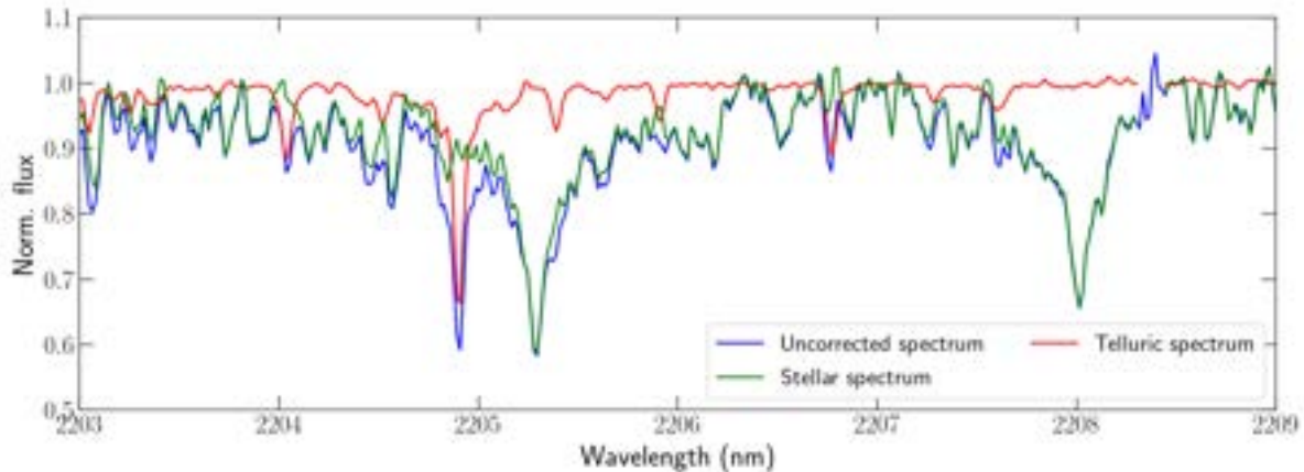
FIGURE 2.3. Same as Fig. 2.2 for small region of the K band featuring 2 Na lines at 2206.2 and 2208.9 nm.
