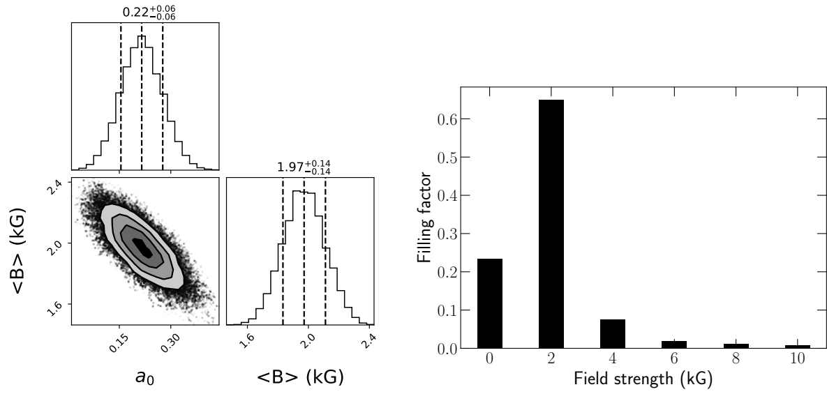
Figure A5. Same as 8 for PM J18482+0741.
