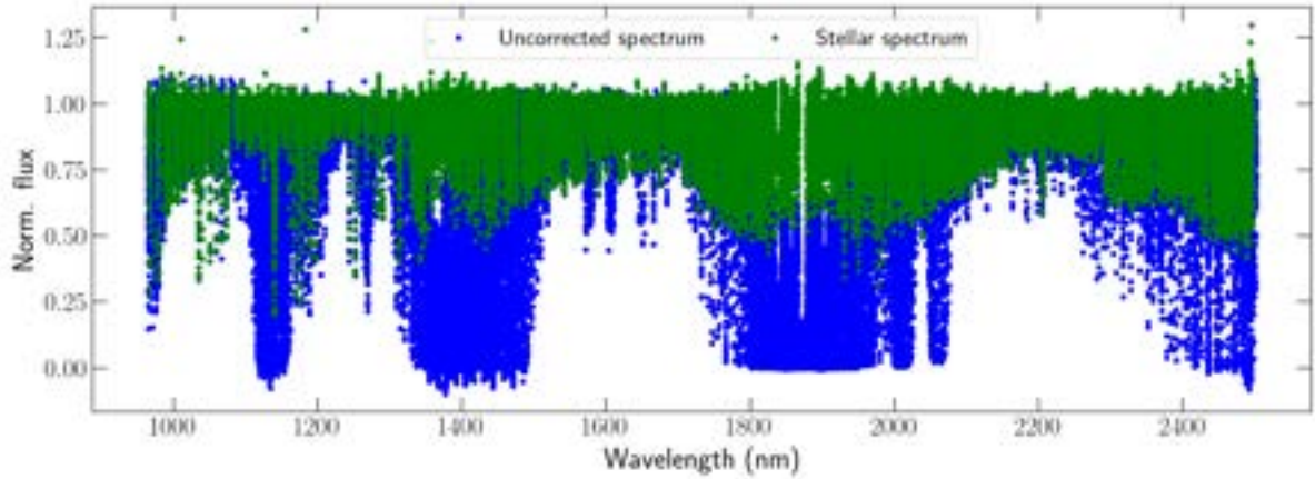
FIGURE 2.2. Typical SPIROU spectrum for Barnard’s star. The raw spectrum containing both the stellar and earth’s atmosphere contribution is plotted in blue, while the stellar spectrum obtained after correction of the telluric lines is plotted green.
