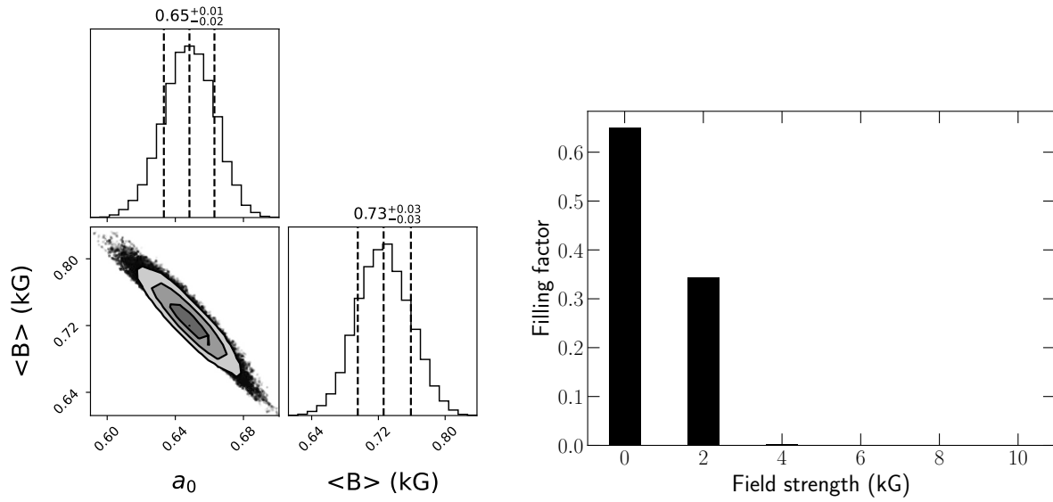
Figure A3. Same as 8 for DS Leo.
