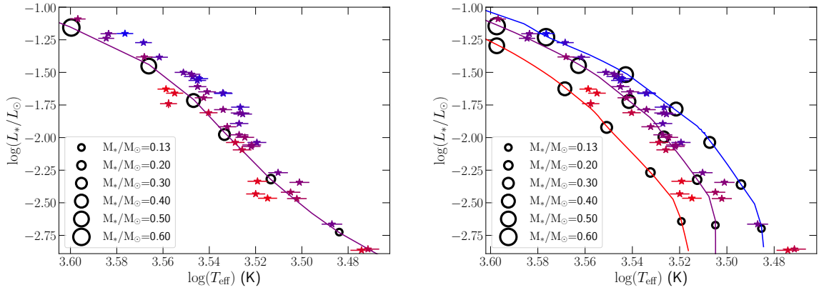
FIGURE 5.10. HR diagram showing the position of the stars in our sample. On both panels, the color of the points code the metallicity from red to blue (low to high metallicity respectively). On the left panel: comparison to the solar-metallicity isochrone computed by Baraffe et al. (2015) (purple line). On the right panel: comparison to the DSEP isochrones computed for [M/H] = -0.5 dex, [M/H] = 0.0 dex and [M/H] = +0.5 dex (red, purple and blue solid lines respectively). Black open circles mark the position of various stellar masses on each isochrone.
