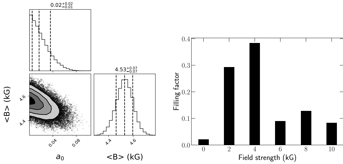
Figure A1. Same as 8 for EV Lac.
