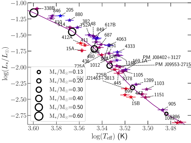
Figure A4. Same as Fig. 7 with labels identifying the stars.
