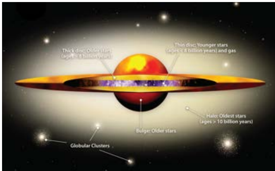
FIGURE 5.1. Schematic representation for the Milky way. Credit: Amanda Smith, IoA graphics officer. https://www.universetoday.com/83315/thick-stellar-disk-isolated-in-andromeda/
