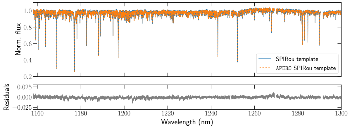
FIGURE 2.7. Comparison between our computed template spectrum and that obtained with APERO for Barnard's star (Gl 699). The bottom plot presents the residuals.
