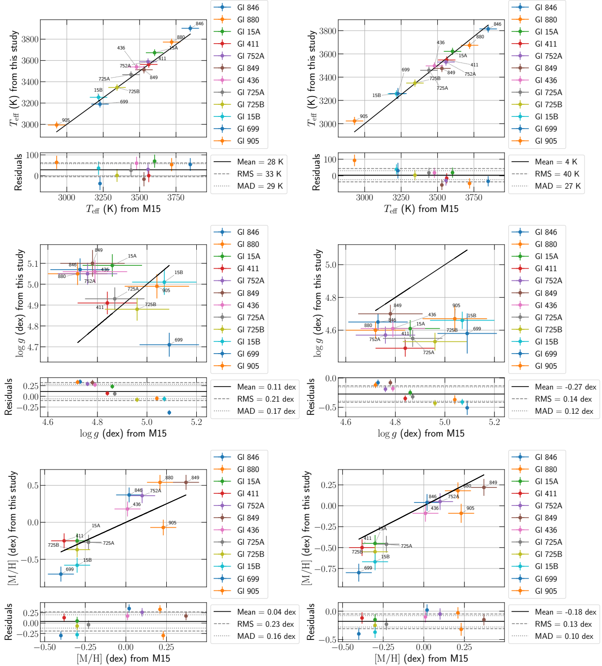
FIGURE 4.11. From top to bottom we present our retrieved T_{\text{eff}} , \log g and [M/H] using the grid of PHOENIX (left) and MARCS (right) spectra plotted against values published by Mann et al. (2015). The solid black line marks the equality. The bottom plots present the residuals, i.e. the retrieved values minus literature values. RMS and median absolute deviation (MAD) values are computed after application of a sigma clipping function on the residuals with a threshold at 5\sigma .
