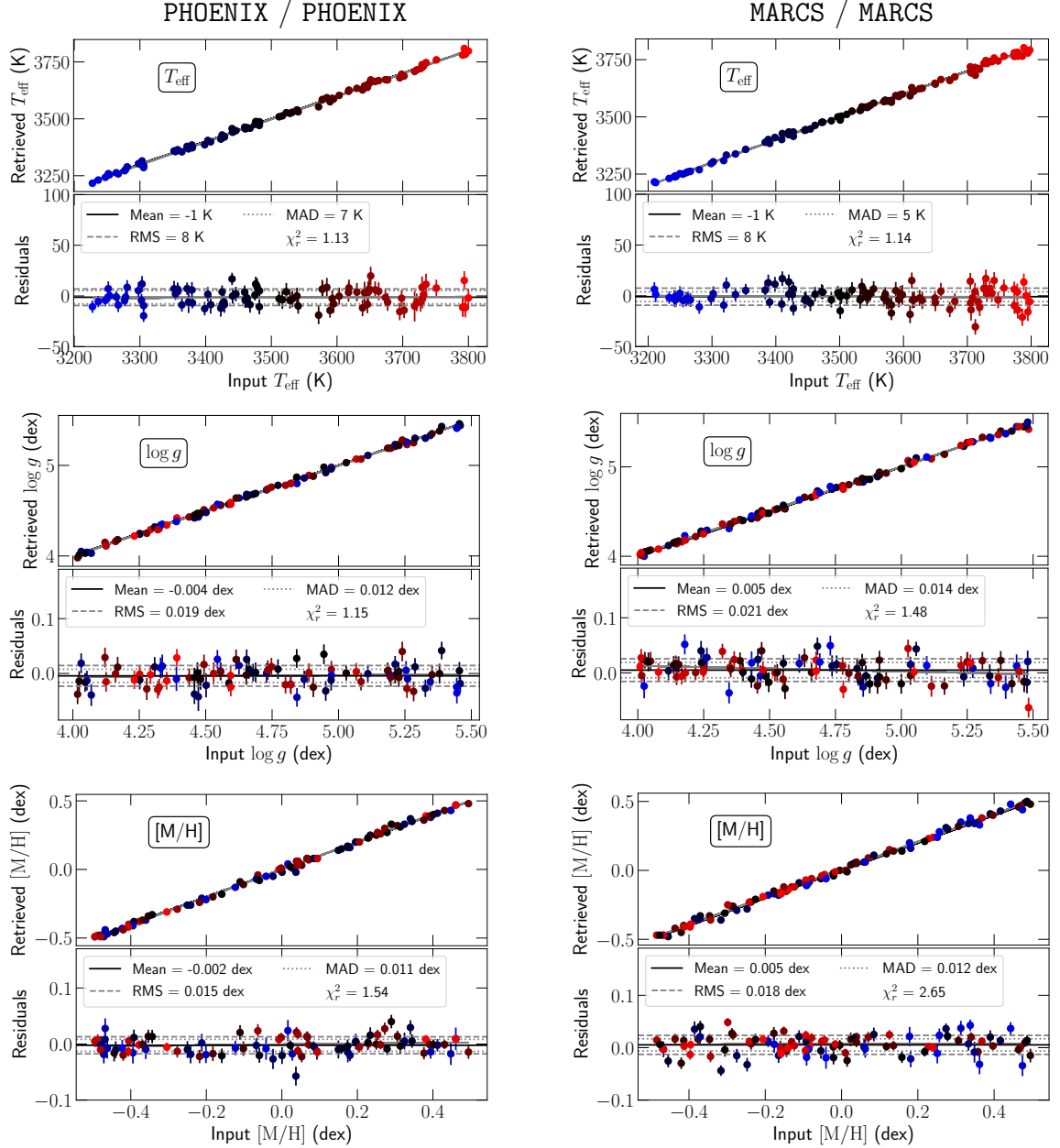
FIGURE 4.7. Simulation of parameters estimation. Retrieved T_{\text{eff}} , \log g and [M/H] are plotted against input parameters. The left column presents the results obtained with PHOENIX used to generate the input model and analyze the model templates. The right column presents the results obtained with the grid of MARCS models. Residuals are presented on the bottom plots, along with their average, RMS, median absolute deviation (MAD) and the reduced \chi^2 of series of points. Data points are color coded as a function of temperature, with blue the lowest temperature, and red the highest temperature.
