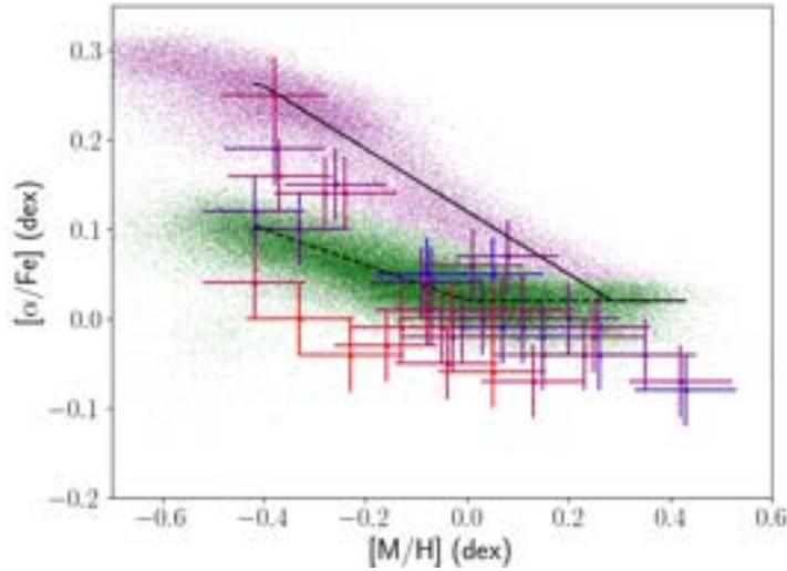
FIGURE 5.9. Estimated [\alpha/Fe] plotted against [M/H] . Purple and green points mark the position of thick and thin disk giants observed with APOGEE, respectively. The solid and dashed lines present fiducial relations for the thick and thin disk, respectively. The color of the points codes the temperature, from cold (red) to hot (blue).
