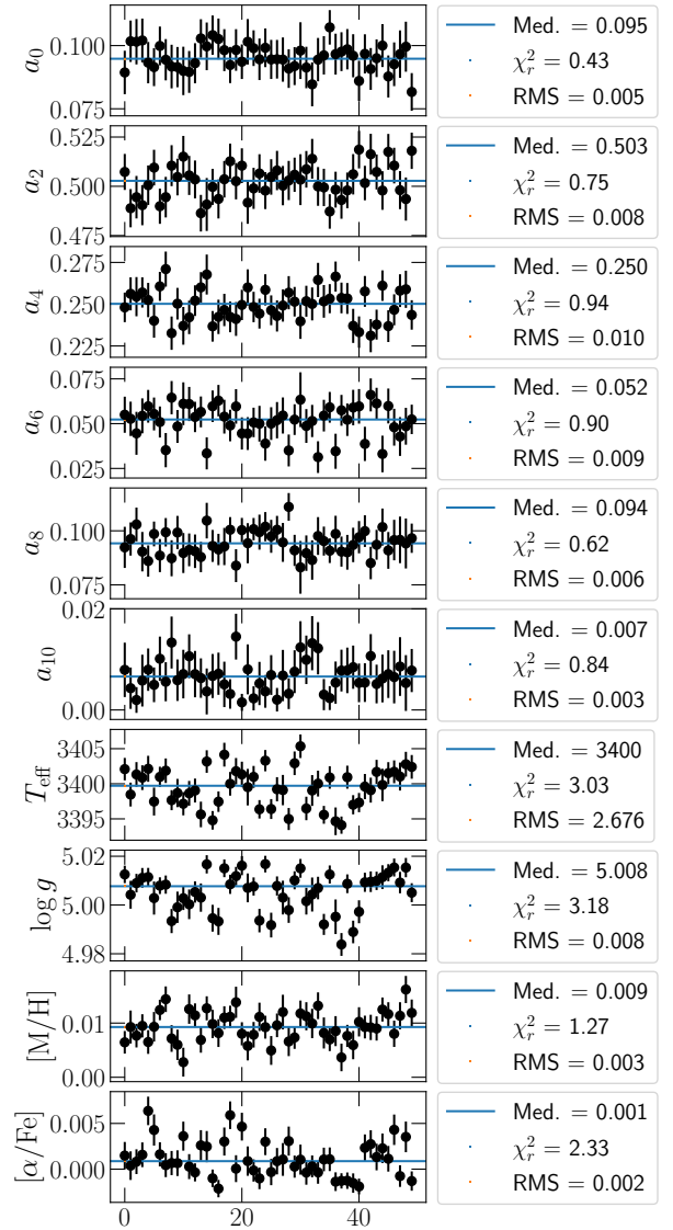
Figure 3. Example of comparison between input and output parameters. The blue horizontal solid line marks the median. For each parameter, we compute the \chi^2 of the series of points. The models were computed for T_{\text{eff}} = 3400 K, \log g = 5.0 dex, [\text{M}/\text{H}] = 0.00 dex and [\alpha/\text{Fe}] = 0.00 dex.
