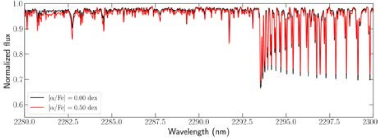
FIGURE 5.6. Example of spectra computed with [\alpha/\text{Fe}] = 0.00 dex and [\alpha/\text{Fe}] = 0.50 dex, with T_{\text{eff}} = 3200 K, \log g = 5.0 dex and [\text{M}/\text{H}] = 0.0 dex.
