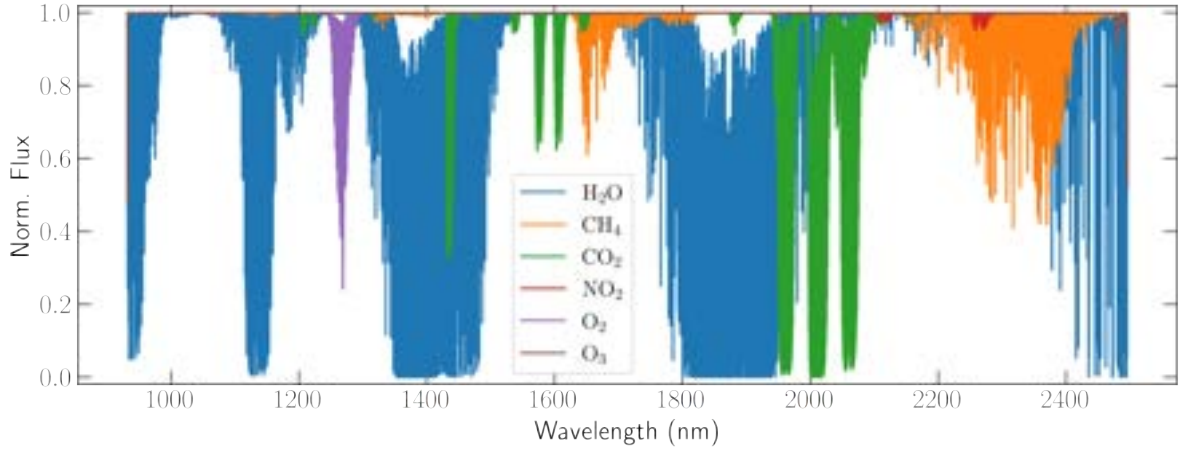
FIGURE 2.4. Typical TAPAS spectrum for each contributing molecule.
