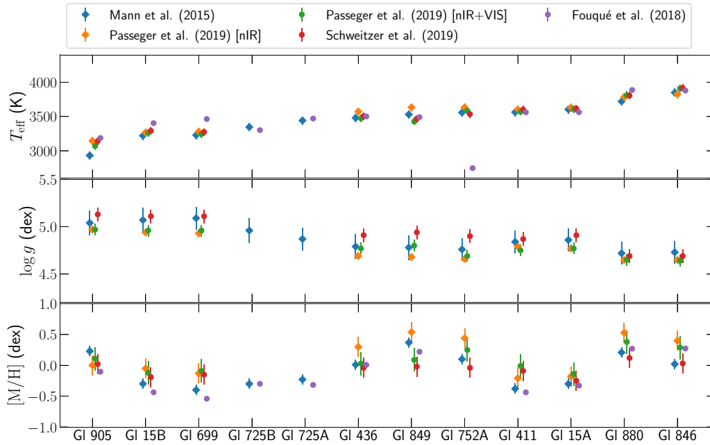
Figure 1. T_{\text{eff}} , \log g , and [M/H] values extracted from the reference studies of Mann et al. (2015), Passeger et al. (2019), Schweitzer et al. (2019), and Fouqué et al. (2018). The typical RMS with respect to the mean is of 45 K in T_{\text{eff}} , 0.07 dex in \log g , and 0.15 dex in [M/H] .
