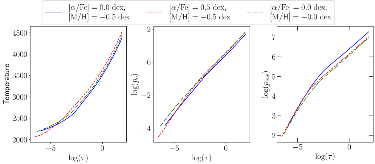
FIGURE 5.5. MARCS atmosphere model structure for different [\alpha/\text{Fe}] and [\text{M}/\text{H}] . The figure shows the temperature, electronic pressure and gas pressure (left, middle and right panels respectively), [\text{M}/\text{H}] = -0.5 dex & [\alpha/\text{Fe}] = 0.0 dex; [\text{M}/\text{H}] = -0.5 dex & [\alpha/\text{Fe}] = 0.5 dex and [\text{M}/\text{H}] = 0.0 dex & [\alpha/\text{Fe}] = 0.5 dex (solid blue, dashed red and dashed green lines respectively). All models are presented for T_{\text{eff}} = 3200 K and \log g = 5.0 dex.
