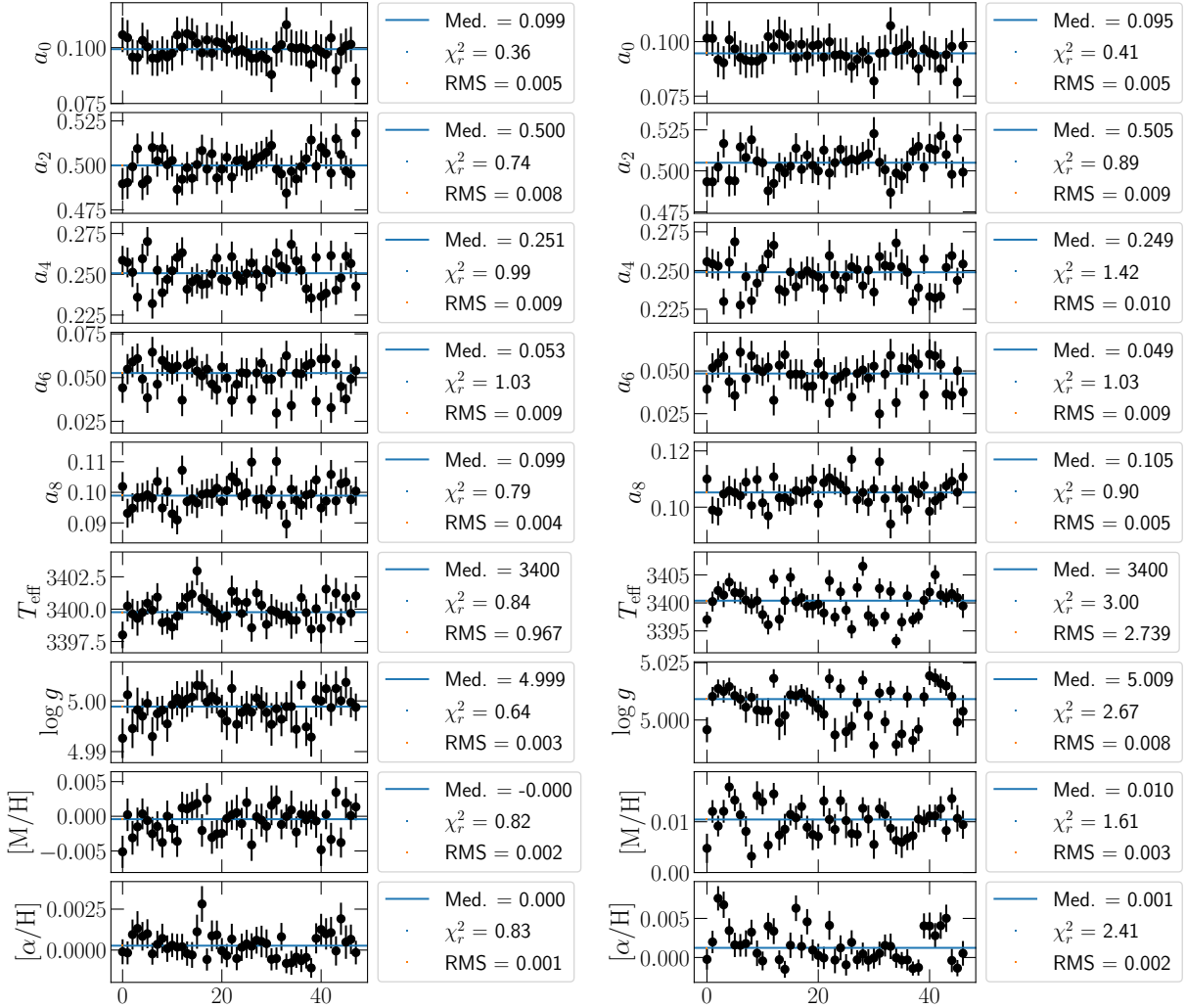
FIGURE 6.8. Results of 50 simulations. We present the residuals between the retrieved parameters and those used to generate the model. For each series of points, we compute the median and RMS. We also compute a reduced \chi^2 on the residuals. The left column presents the results of the analysis with no adjustment of the continuum, while the right column presents the results of the analysis performing the adjustment of the continuum.
