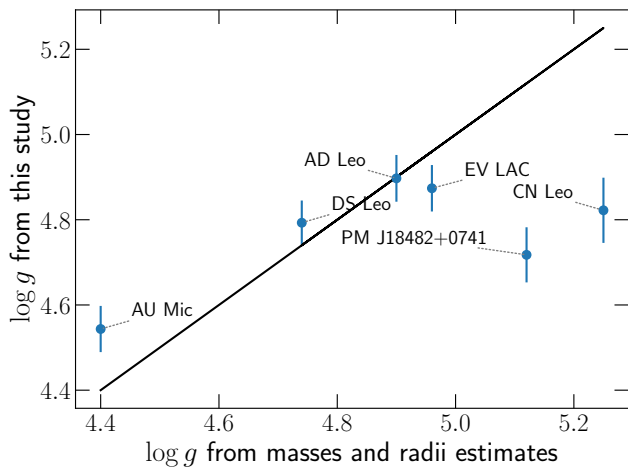
Figure C2. Retrieved \log g compared to estimates derived from masses and radii (see Table 3).
