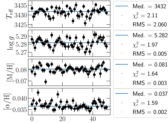
FIGURE 6.9. Same as Fig. 6.8 but with no field considered in the analysis.
