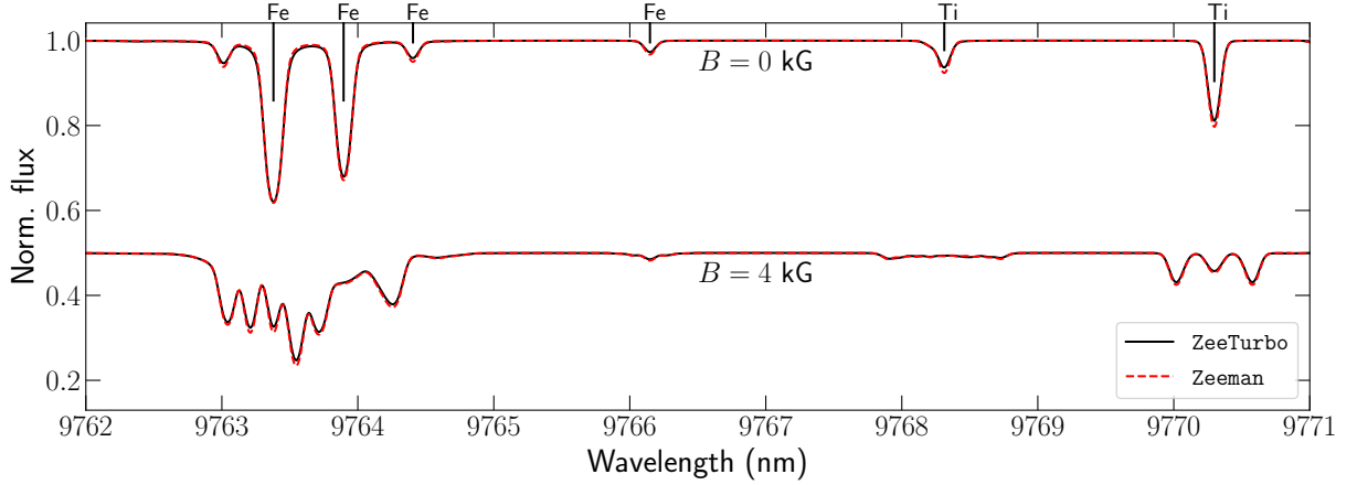
FIGURE 6.6. Comparison between ZeeTurbo and Zeeman spectra. Models were computed assuming T_{\text{eff}} = 6000 K, \log g = 4.5 dex and [M/H] = 0.0 dex.
