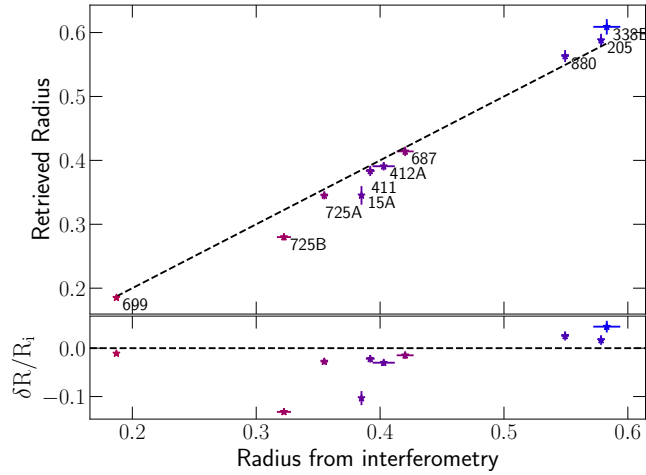
FIGURE 5.11. Comparison between our estimated radii and those computed from interferometric data. The dashed line marks the equality. The color of the points reflect the temperature from red (coolest) to blue (hottest).
