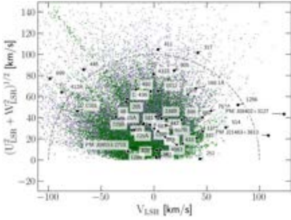
Figure A1. Same as Fig. 1 with labels identifying the stars.
