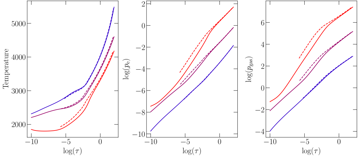
FIGURE 4.10. Comparison between the model atmosphere structure of PHOENIX-ACES (solid lines) and MARCS (dashed lines). Structures are displayed for a T_{\text{eff}} of 3000, 3400 and 3800 K, displayed in red, purple and blue respectively. Arbitrary offsets were applied on \log p_e and \log p_{\text{gas}} for better readability.
