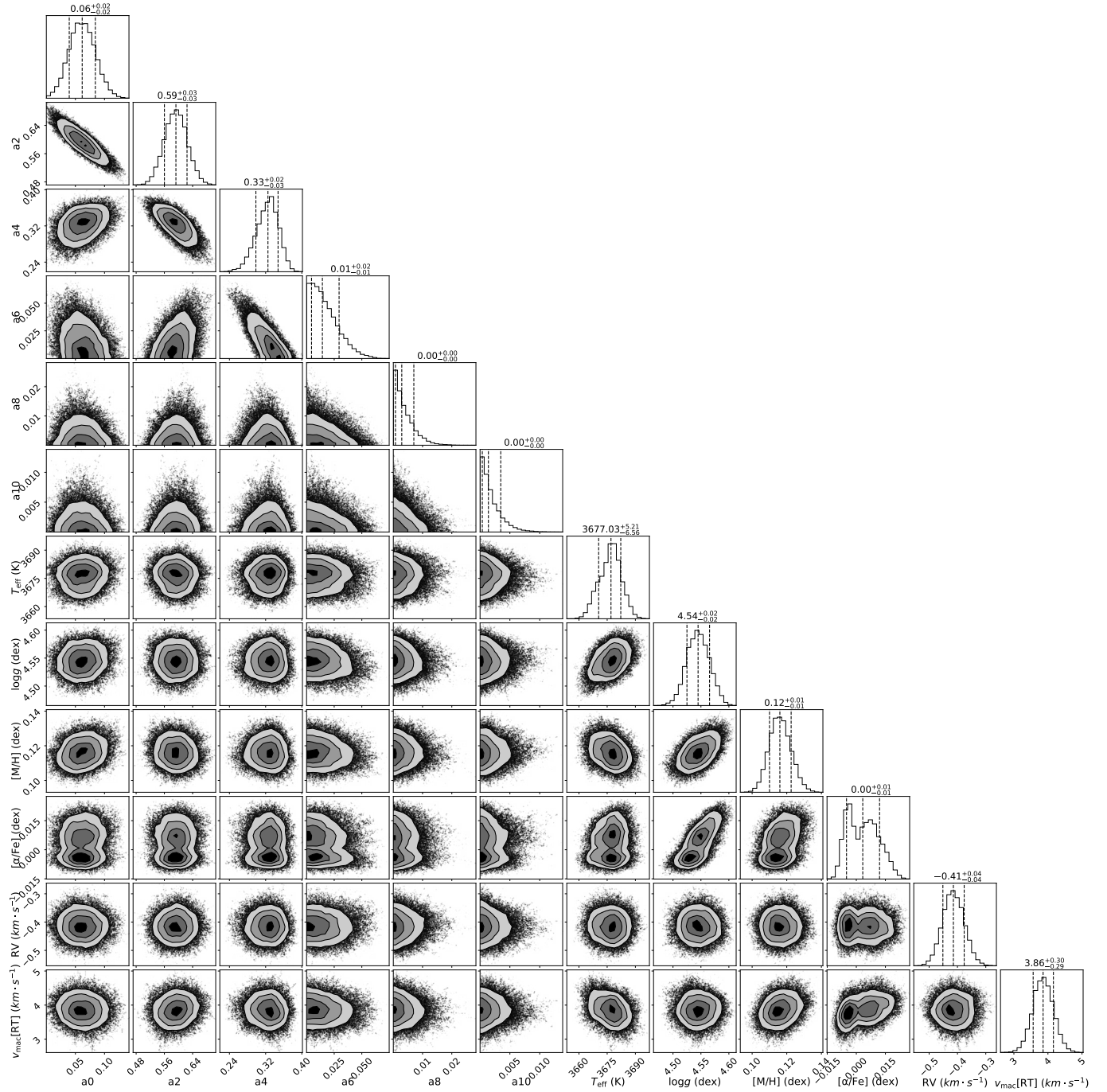
Figure 6. Corner plot presenting posterior distributions for filling factors and atmospheric parameters for AU Mic.
