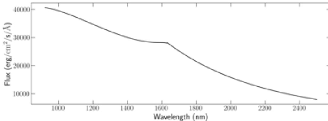
FIGURE 3.2. Example of continuum flux computed with Turbospectrum from a MARCS model atmosphere over the entire wavelength range covered by SPIRou. The discontinuity observed in the middle of the profile results from the end of H^- bound-free transitions.
