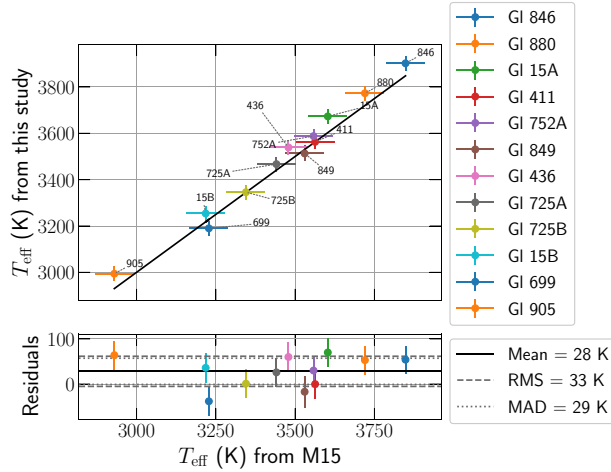
Figure 10. Retrieved T_{\text{eff}} using the grid of PHOENIX (left-hand panel) and MARCS (right-hand panel) spectra plotted against values published by M15. The bottom plot presents the residuals, i.e. the retrieved values minus literature values. RMS and MAD values are computed after application of a sigma clipping function on the residuals with a threshold at 5\sigma .
