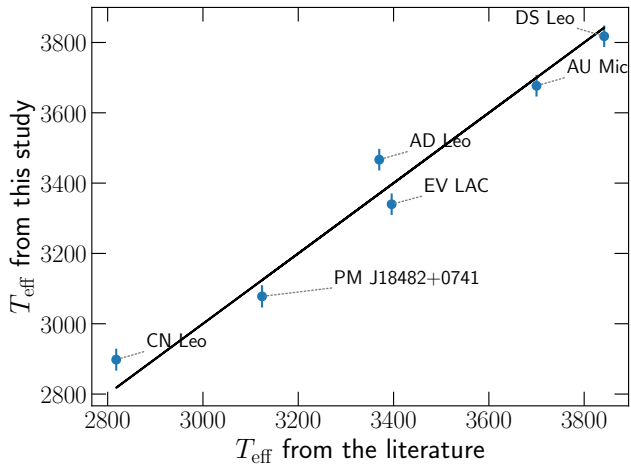
Figure C1. Retrieved T_{\text{eff}} compared to literature estimates taken from Afram & Berdyugina (2019, AU Mic) , Mann et al. (2015, AD Leo, CN Leo) , Maldonado et al. (2020, EV Lac) , Cristofari et al. (2022b, DS Leo) and Passegger et al. (2019, PM J18482+0741) .
