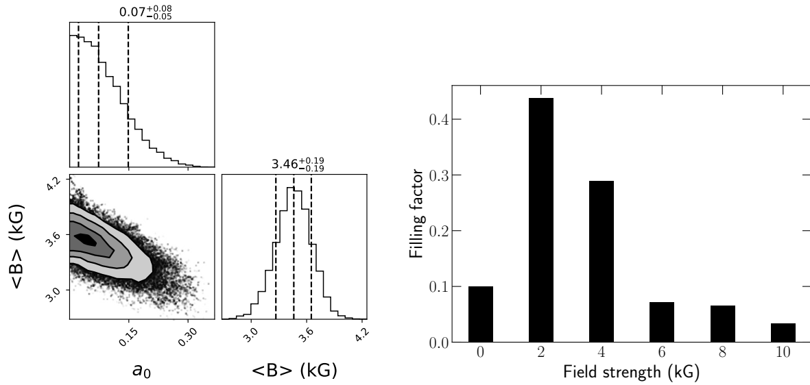
Figure A4. Same as 8 for CN Leo.
