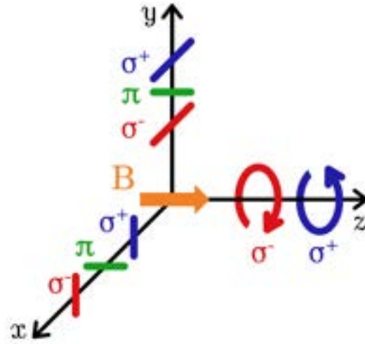
FIGURE 6.3. Polarization of the Zeeman components. Taken from Dr Lisa Lehmann's PhD thesis ( https://doi.org/10.17630/10023-20354 ).
