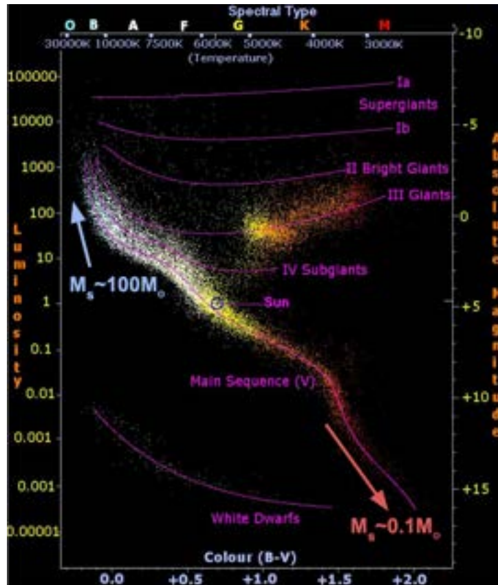
FIGURE 1.1. HR diagram for over 23000 stars from the Hipparcos and Gliese catalogues. Taken from Dr. Baptiste Klein PhD manuscript ( http://thesesups.ups-tlse.fr/5052/ ), adapted from R. Powell ( http://www.atlasoftheuniverse.com/hr.html )
