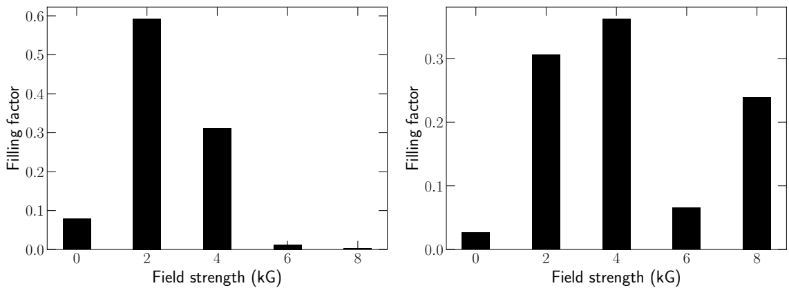
FIGURE 6.11. Retrieved filling factors for AU Mic (left) and EV Lac (right).
