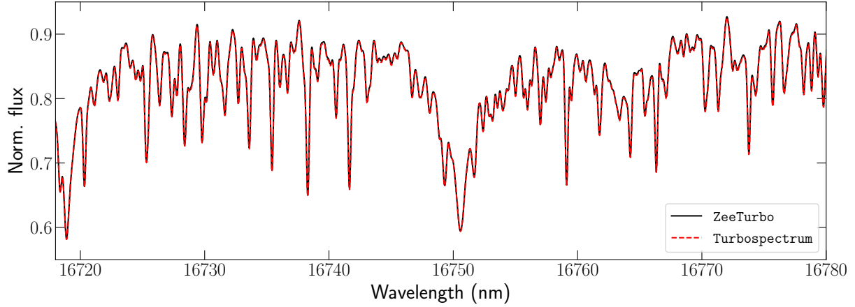
FIGURE 6.5. Comparison between ZeeTurbo and Turbospectrum spectra. Models were computed assuming T_{\text{eff}} = 3200 K, \log g = 5.0 dex and [M/H] = 0.0 dex.
