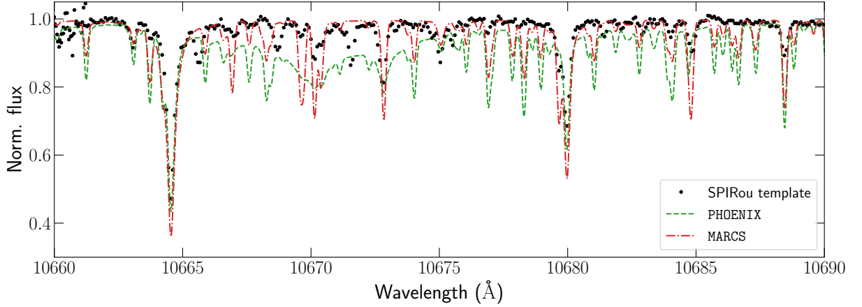
FIGURE 4.4. Gl 699 template spectrum compared to synthetic models for T_{\text{eff}} = 3200 K, \log g = 5.0 dex and [M/H] = -0.4 dex for a tiny chunk of the SPIRou domain (1066 – 1069 nm).
