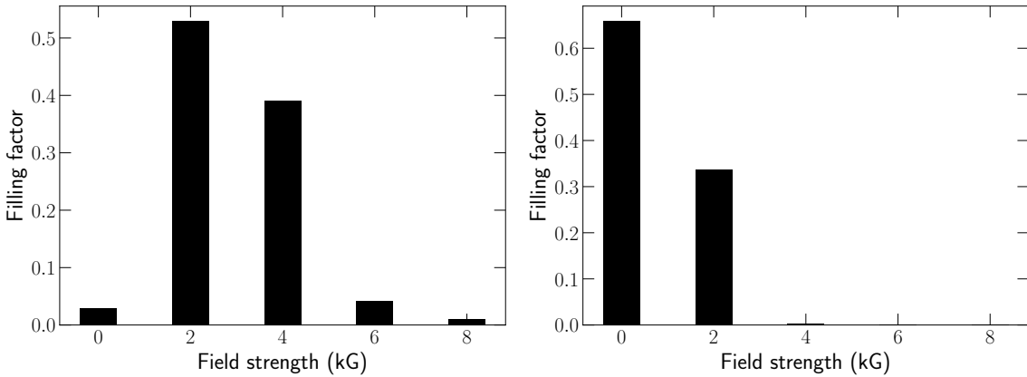
FIGURE 6.13. Same Fig. 6.11 for AD Leo (left) and DS Leo (right).
