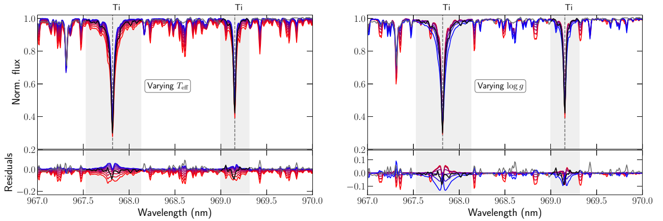
Figure 6. Comparison between PHOENIX synthetic spectra and the template spectrum of Gl 15A (grey). In the regions selected for the analysis, outlined with a grey background, the observed spectrum is displayed as a black line. The coloured spectra correspond to synthetic spectra for different values of the parameters, with red being the lowest and blue the highest. The associated parameters vary from 3000 K to 4000 K in steps of 100 K in T_{\text{eff}} (left-hand panel), and from 3. to 6.0 dex in steps of 0.5 dex in \log g (right-hand panel). The bottom plots show the residuals, i.e. the synthetic spectra and template spectrum minus the synthetic spectrum corresponding to the parameters of M15.
