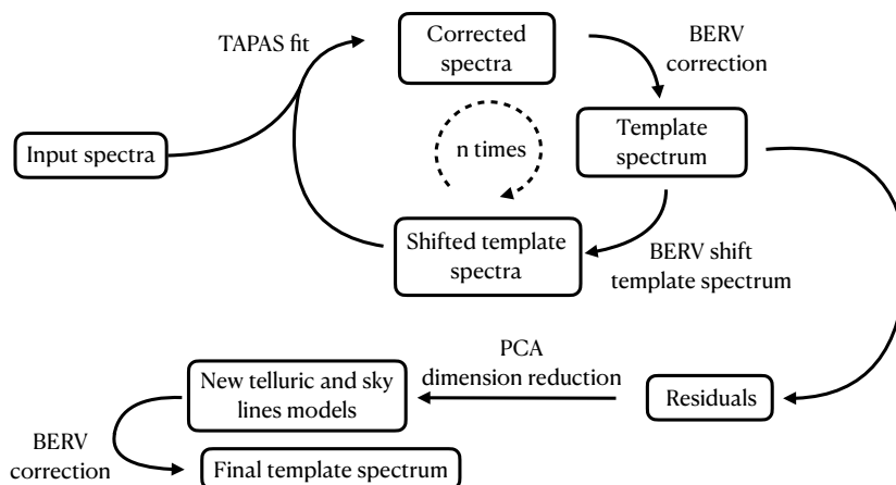
FIGURE 2.5. Iterative scheme used to derive template spectra from individual SPIRou spectra.
