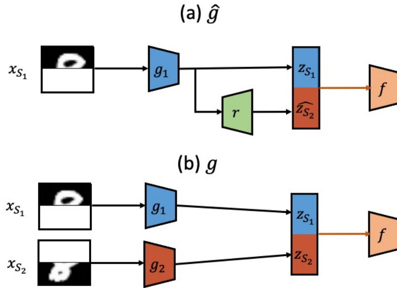
Figure 3.1. – Encoding of an input source digit \mathbf{x}_S = (\mathbf{x}_{S_1}, \mathbf{x}_{S_2}) with \hat{g} (a) and g (b). g_1 encodes the first part of the input \mathbf{x}_{S_1} into \mathbf{z}_{S_1} . The second latent component is either built by encoding \mathbf{x}_{S_2} with g_2 as \mathbf{z}_{S_2} (b) or with reconstruction via r \circ g_1 as \hat{\mathbf{z}}_{S_2} (a). These latent components \hat{\mathbf{z}}_S (a), \mathbf{z}_S (b) are fed directly into a classifier f .
