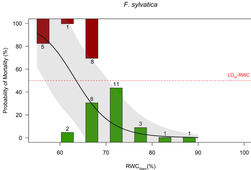
Figure S11. Logistic regression to determine the 50% lethal dose ( LD_{50} -RWC, dashed red line) of stem relative water content ( RWC_{Stem} ) during drought for Fagus sylvatica . LD_{50} -RWC was computed at 63.5 \pm 1.9\% . Bars represent the number of trees that survived (green bars) or died (red bars) from the drought event in each 5% RWC bin. The solid black line represents the logistic regression fit with a shaded grey area representing a 95% confidence interval for the logistic regression.
