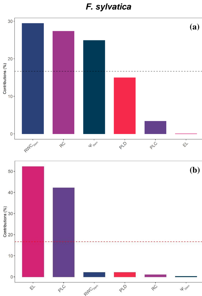
Figure 71. Contribution of each parameter measured right before re-watering to (a) Dimension 1 (Dim-1) and (b) Dimension 2 (Dim-2) of the PCA analysis run for Fagus sylvatica . Each colour represents one parameter.
