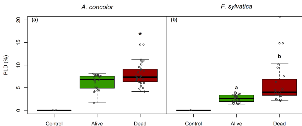
Figure 67. Percentage loss of stem diameter (PLD) for (a) Abies concolor and (b) Fagus sylvatica trees in control conditions (Control) and right before re-watering for trees that survived the experiment (Alive) and trees that died from drought (Dead). Stars (for A. concolor ) and letters (for F. sylvatica ) represent statistical differences between the groups ( \alpha=0.05 ).
