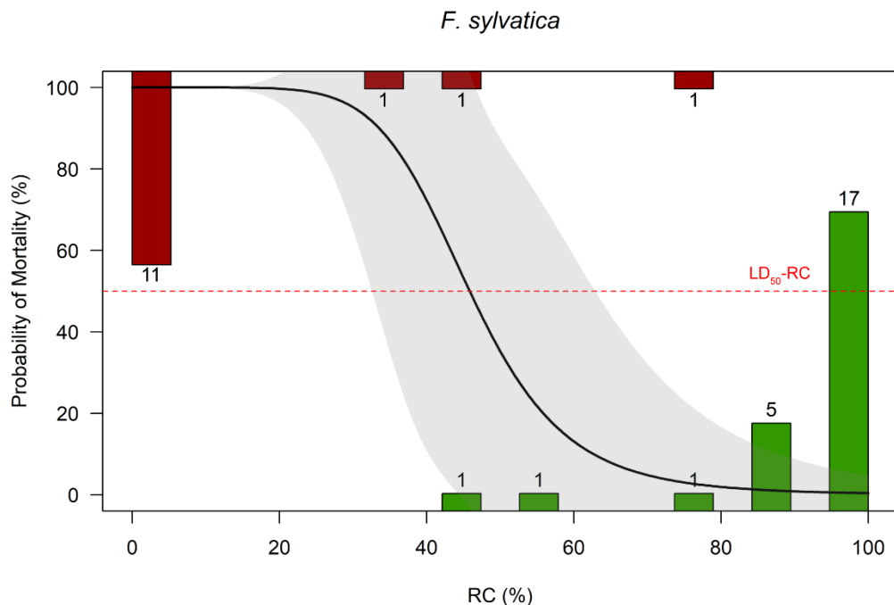
Figure S12. Logistic regression to determine the 50% lethal dose ( LD_{50} -RC, dashed red line) of stem recovery capacity (RC) during drought for Fagus sylvatica . LD_{50} -RC was computed at 45.9 \pm 4.4\% . Bars represent the number of trees that survived (green bars) or died (red bars) from the drought event in each 10% RC bin. The solid black line represents the logistic regression fit with a shaded grey area representing a 95% confidence interval for the logistic regression.
