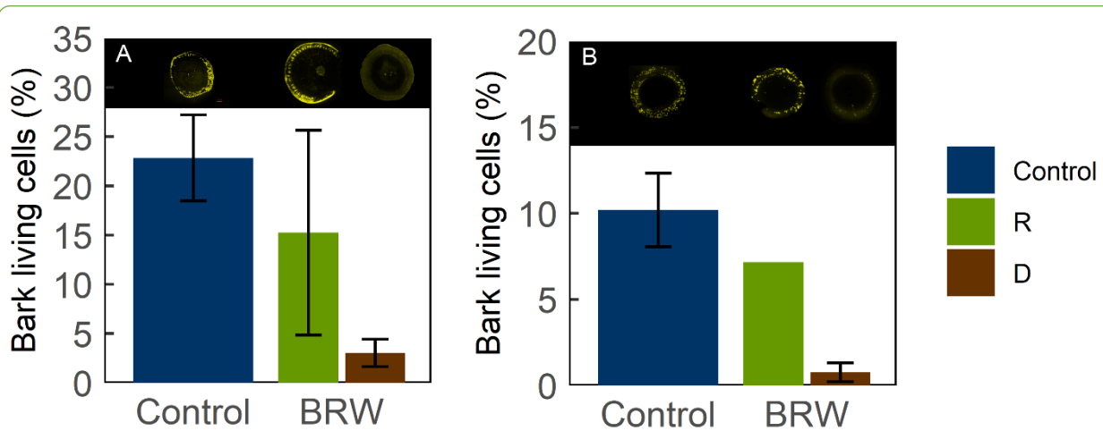
Figure 39. Percentage of bark living cells (%BLC) stained with FDA in stem cross-sections in Prunus lusitanica (panel A) and Pseudotsuga menziesii (panel B).
